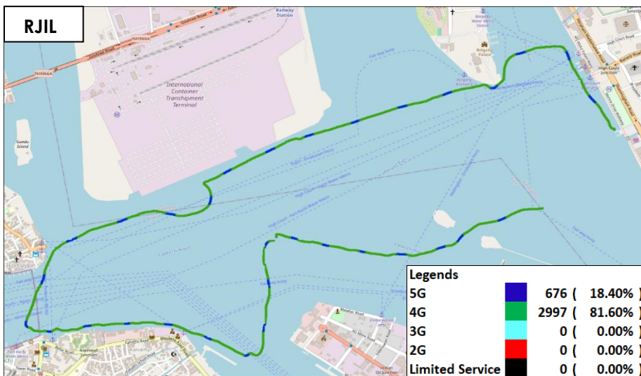
Figure-30: Serving technology plots in auto-selection mode (5G/4G/3G/2G)-RJIL.
