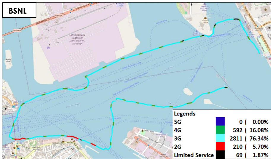
Figure-29: Serving technology plots in auto-selection mode (5G/4G/3G/2G)-BSNL.
