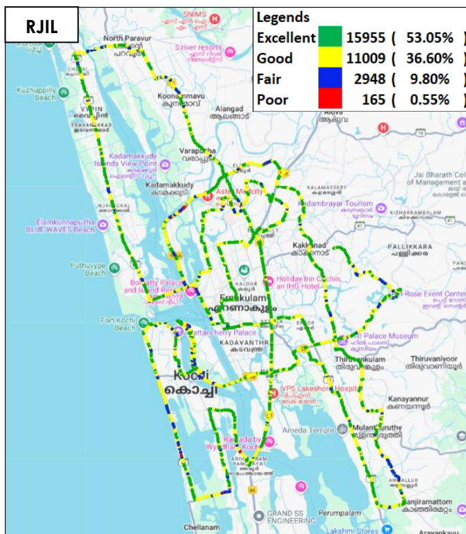
Figure-40: Signal strength auto-selection mode 5G/4G/3G/2G – RJIL.
