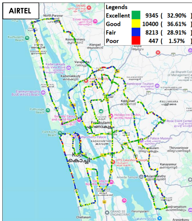
Figure-35: Signal strength 3G/2G network mode – AIRTEL.
