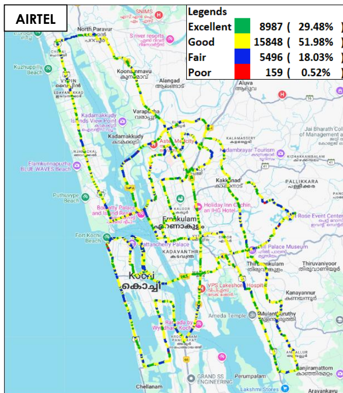
Figure-38: Signal strength auto-selection mode 5G/4G/3G/2G – AIRTEL.
