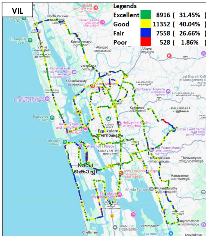
Figure-37: Signal strength 3G/2G network mode – VIL.
