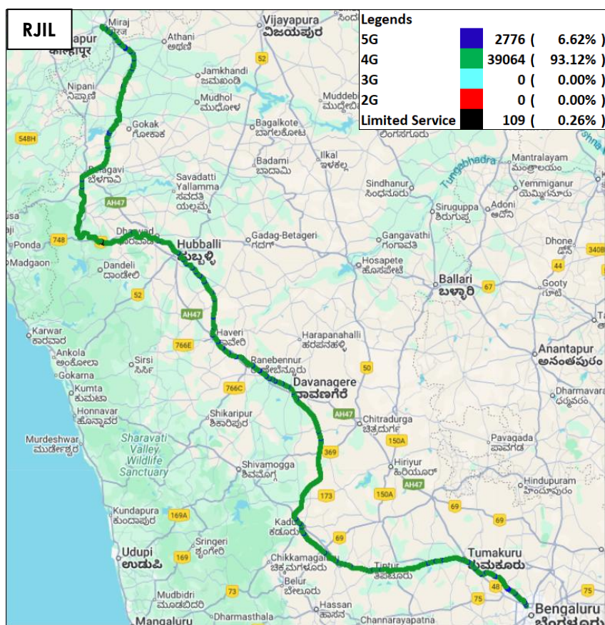
Figure-30: Serving technology plots in auto-selection mode (5G/4G/3G/2G)-RJIL.
