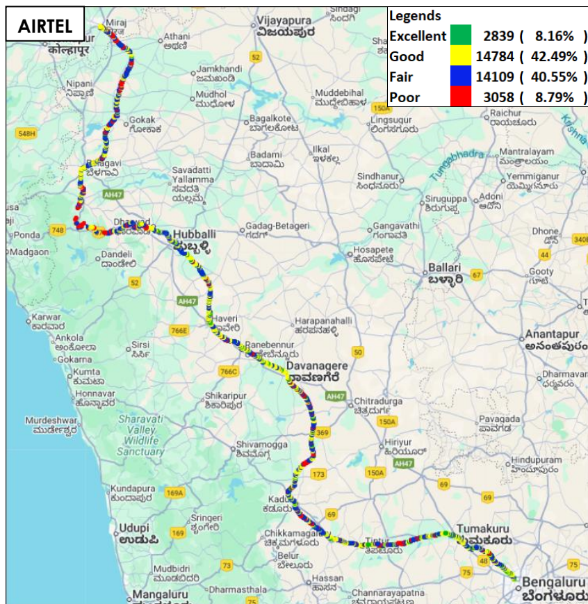
Figure-42: Signal strength auto-selection mode 5G/4G/3G/2G – AIRTEL.
