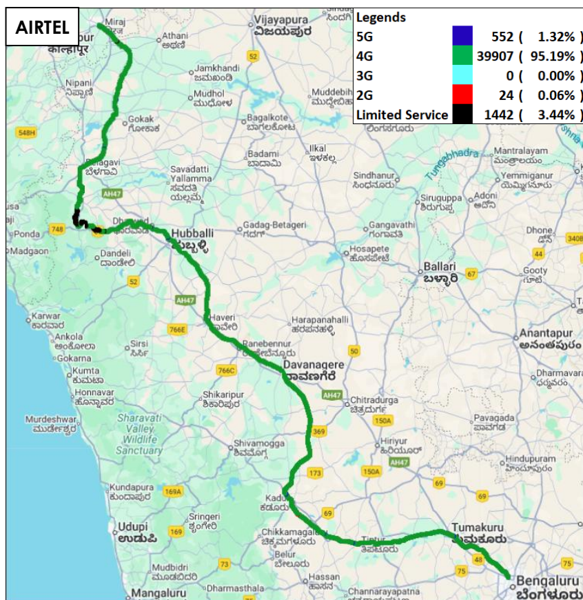
Figure-28: Serving technology plots in auto-selection mode (5G/4G/3G/2G)-AIRTEL.
