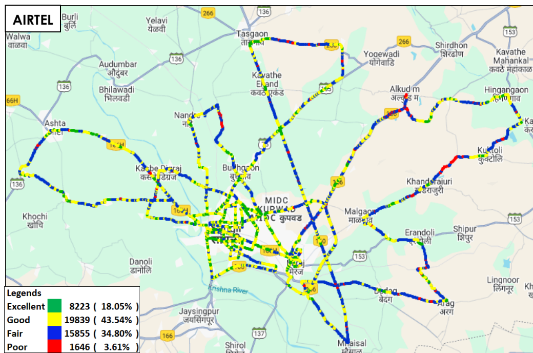
Figure-38: Signal strength auto-selection mode 5G/4G/3G/2G – AIRTEL.
