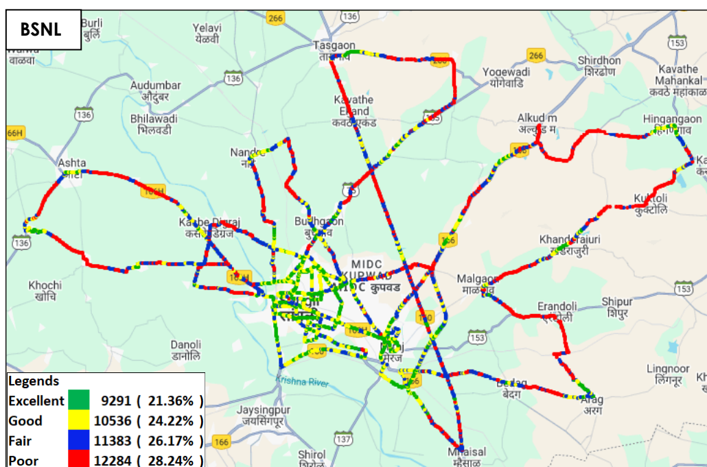
Figure-36: Signal strength 3G/2G network mode – BSNL.
