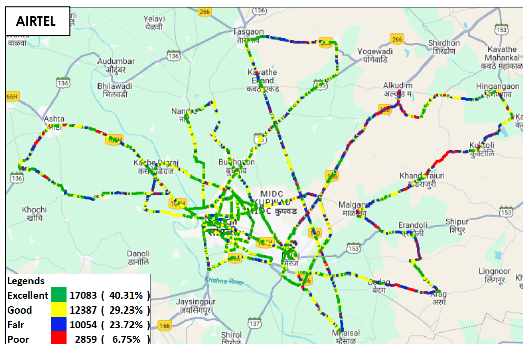
Figure-35: Signal strength 3G/2G network mode – AIRTEL.
