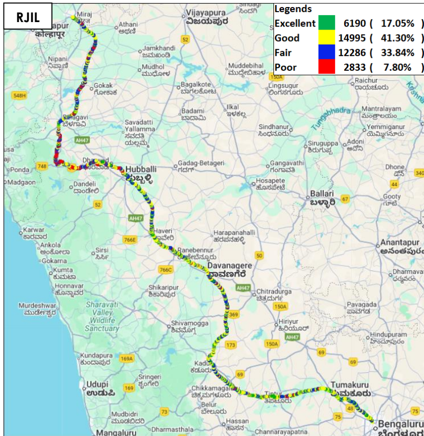
Figure-44: Signal strength auto-selection mode 5G/4G/3G/2G – RJIL.
