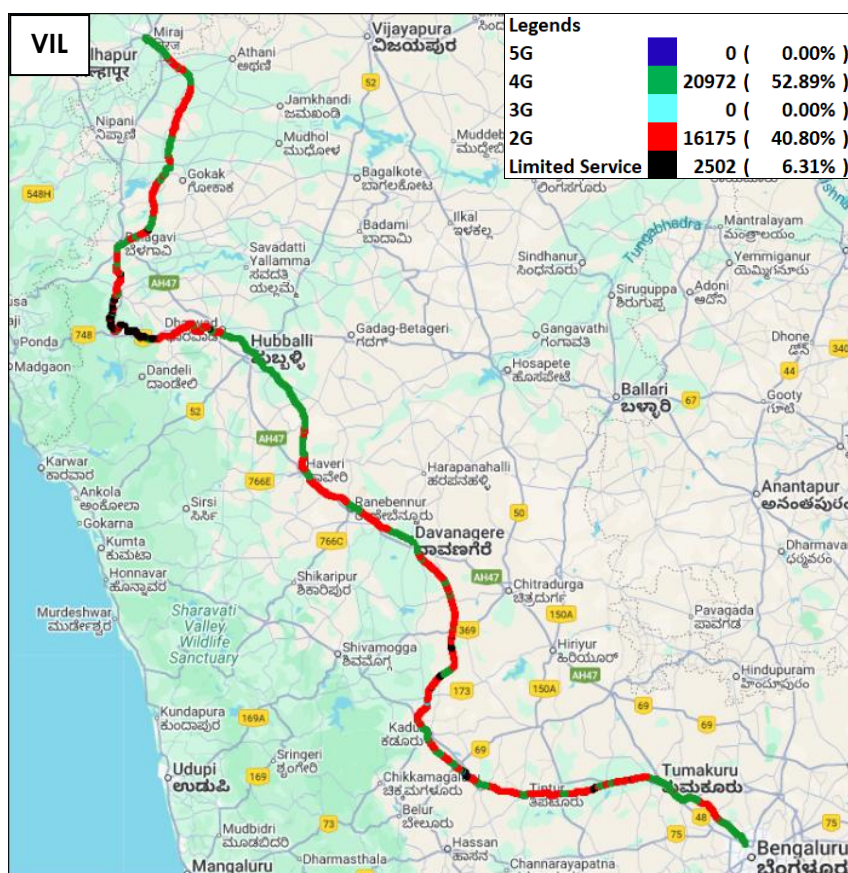
Figure-31: Serving technology plots in auto-selection mode (5G/4G/3G/2G) -VIL.
