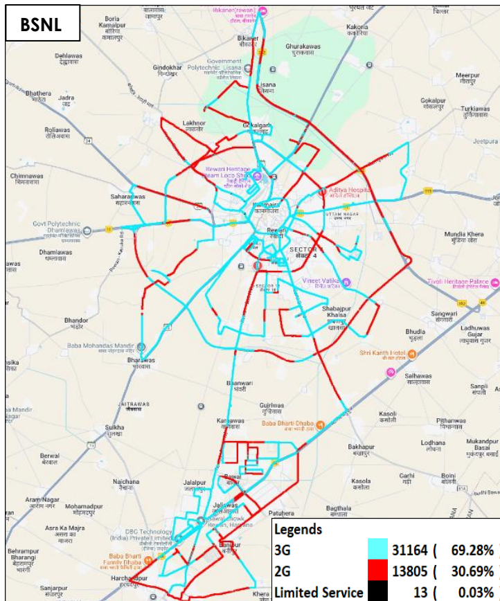
Figure-10: Serving technology plots 3G/2G network mode(4G services Being rolled out) –BSNL.
