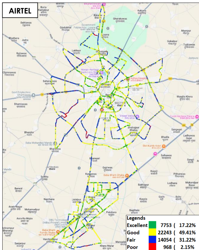
Figure-28: Signal strength auto-selection mode 5G/4G/3G/2G – AIRTEL.
