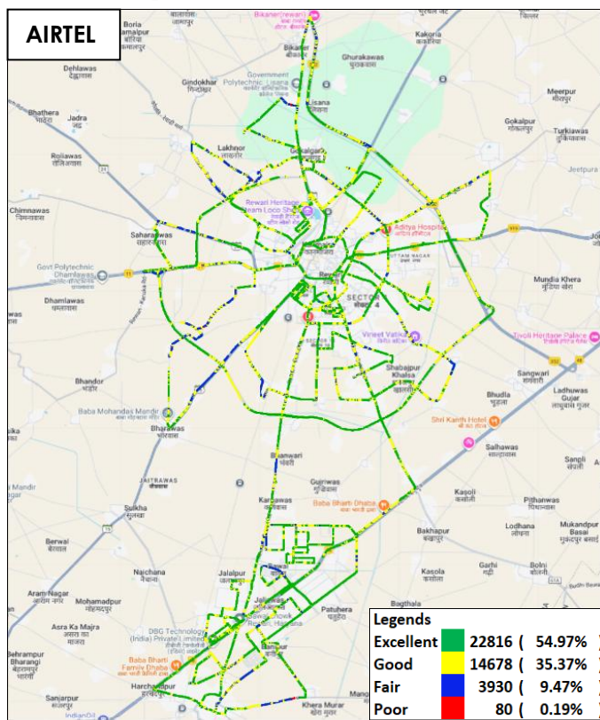
Figure-25: Signal strength 3G/2G network mode – AIRTEL.
