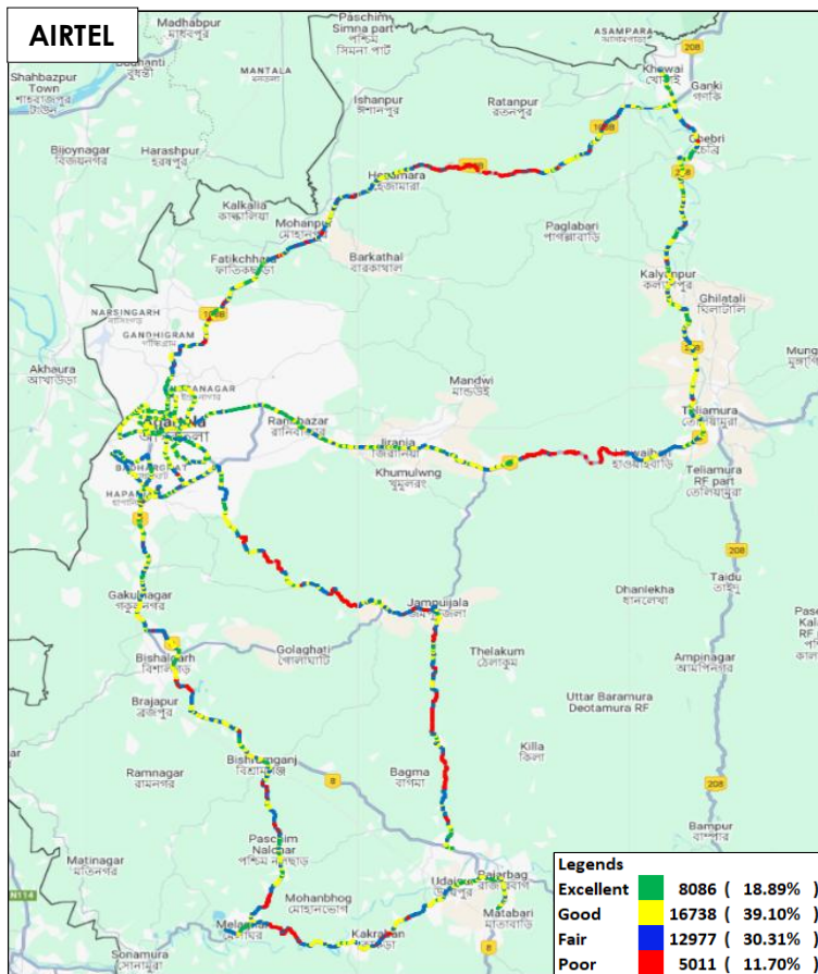
Figure-37: Signal strength auto-selection mode 5G/4G/3G/2G – AIRTEL.
