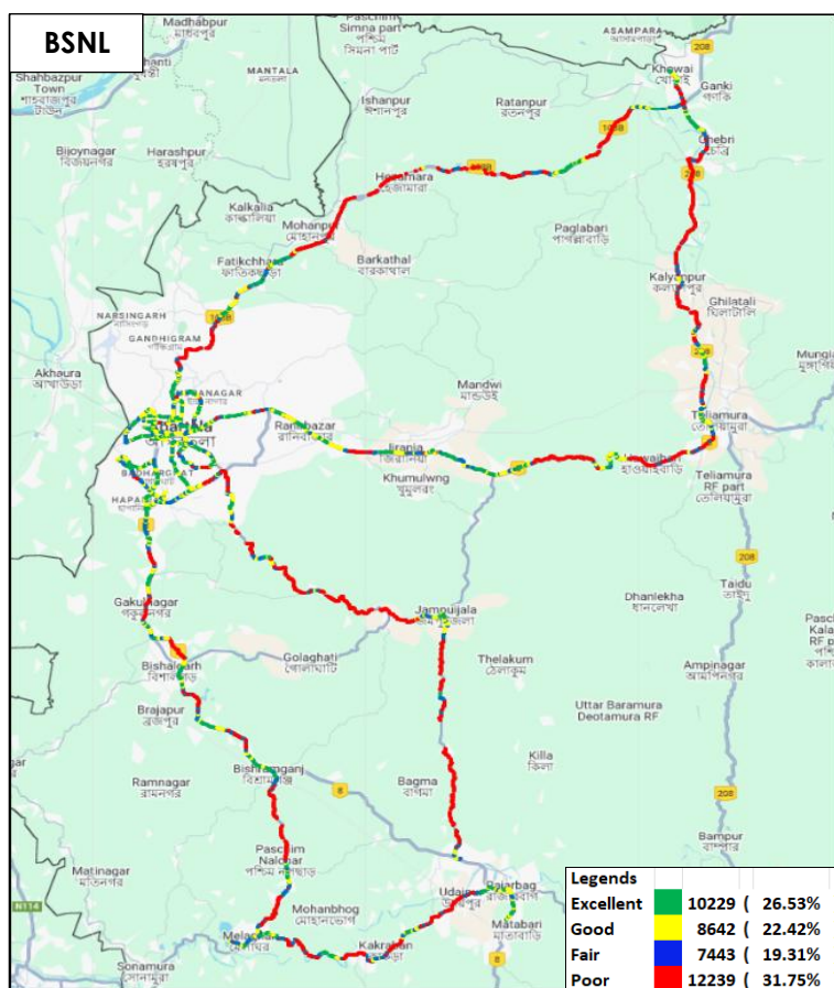
Figure-35: Signal strength 3G/2G network mode – BSNL.
