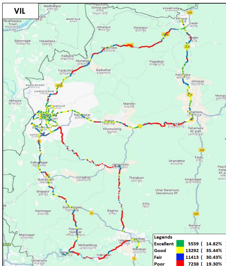
Figure-40: Signal strength auto-selection mode 5G/4G/3G/2G – VIL.
