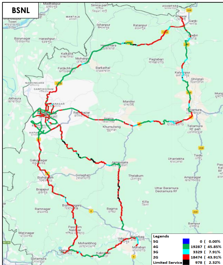
Figure-17: Serving technology plots in auto-selection mode (5G/4G/3G/2G) -BSNL (4G being rolled out)
