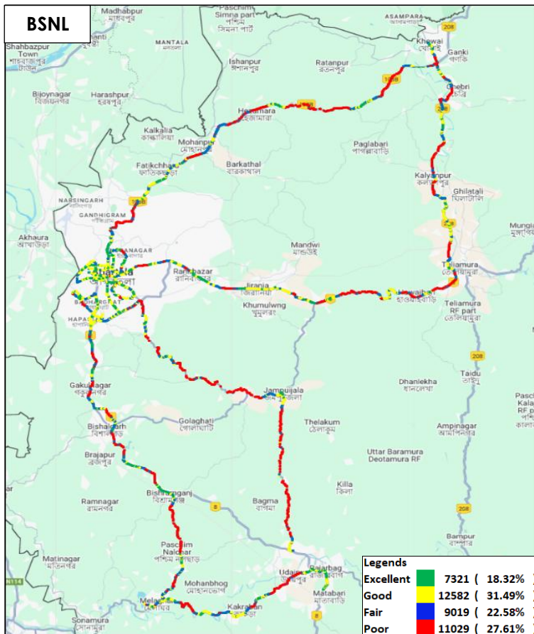
Figure-38: Signal strength auto-selection mode 5G/4G/3G/2G – BSNL (4G being rolled out)
