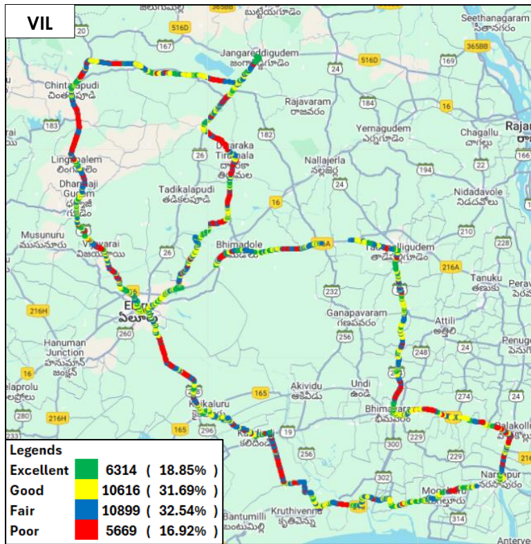
Figure-26: Signal strength 3G/2G network mode – VIL.
