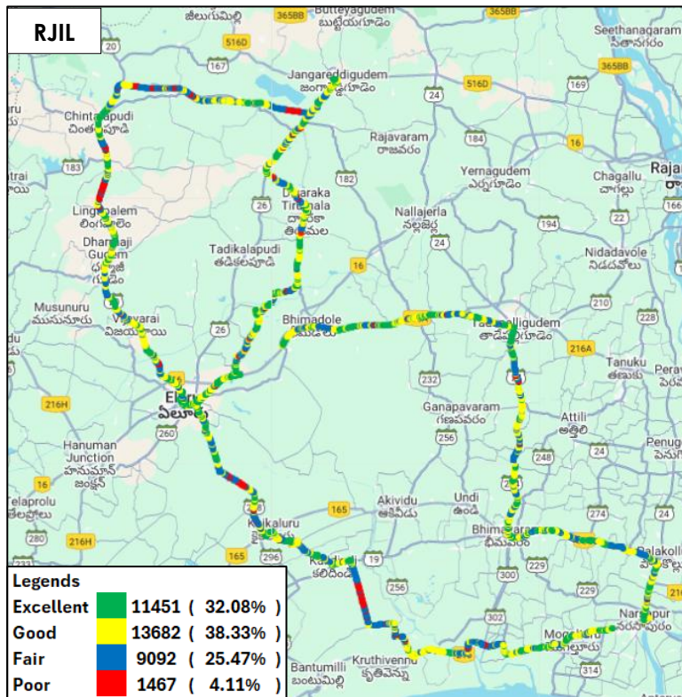
Figure-29: Signal strength auto-selection mode 5G/4G/3G/2G – RJIL.
