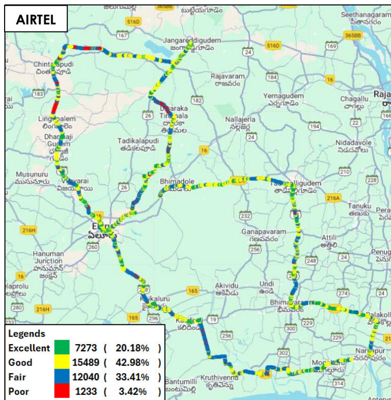
Figure-27: Signal strength auto-selection mode 5G/4G/3G/2G – AIRTEL.
