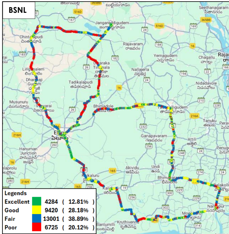
Figure-28: Signal strength auto-selection mode 5G/4G/3G/2G – BSNL.
