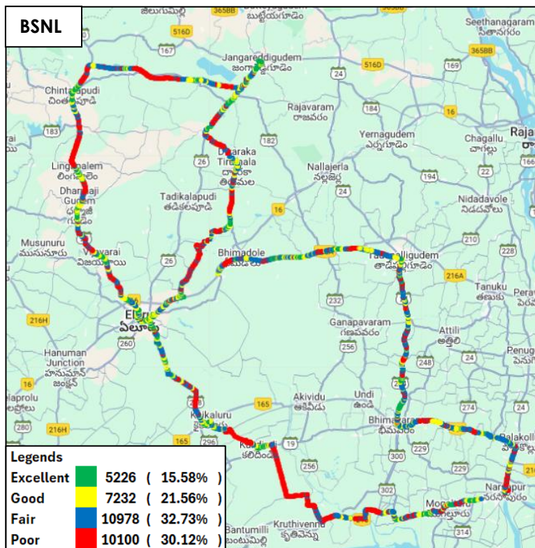
Figure-25: Signal strength 3G/2G network mode – BSNL.
