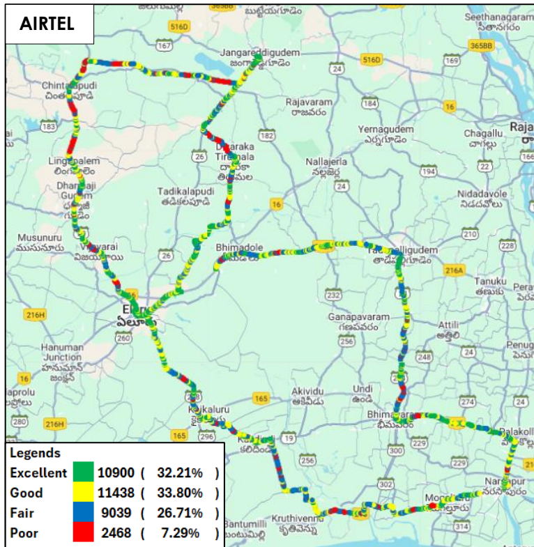
Figure-24: Signal strength 3G/2G network mode – AIRTEL.
