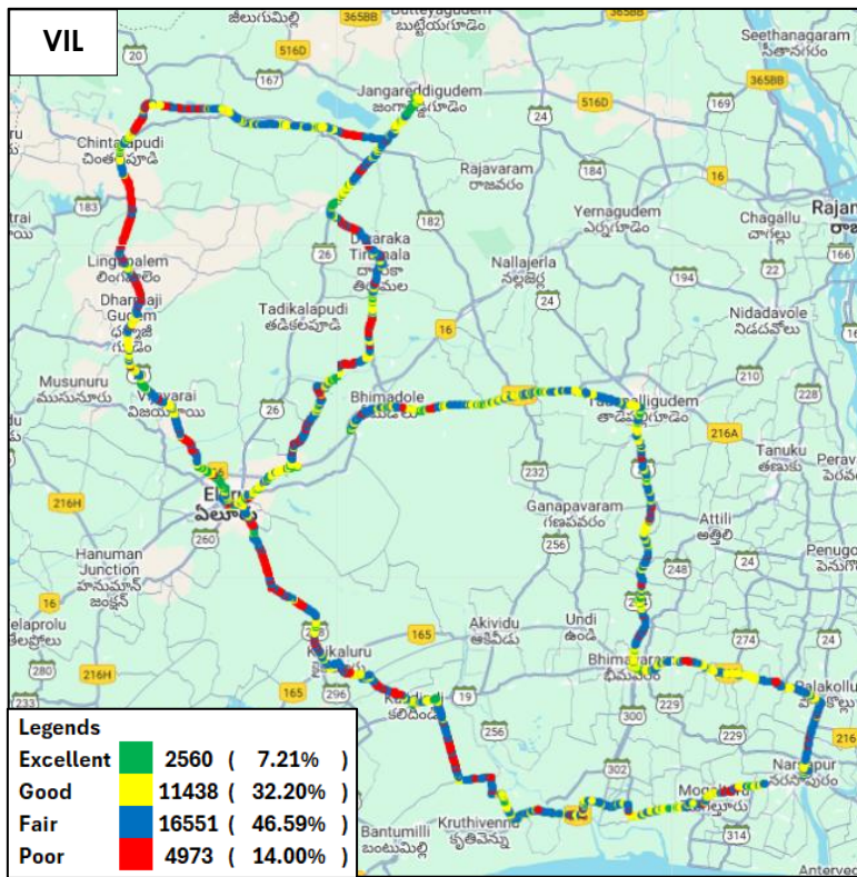
Figure-30: Signal strength auto-selection mode 5G/4G/3G/2G – VIL.
