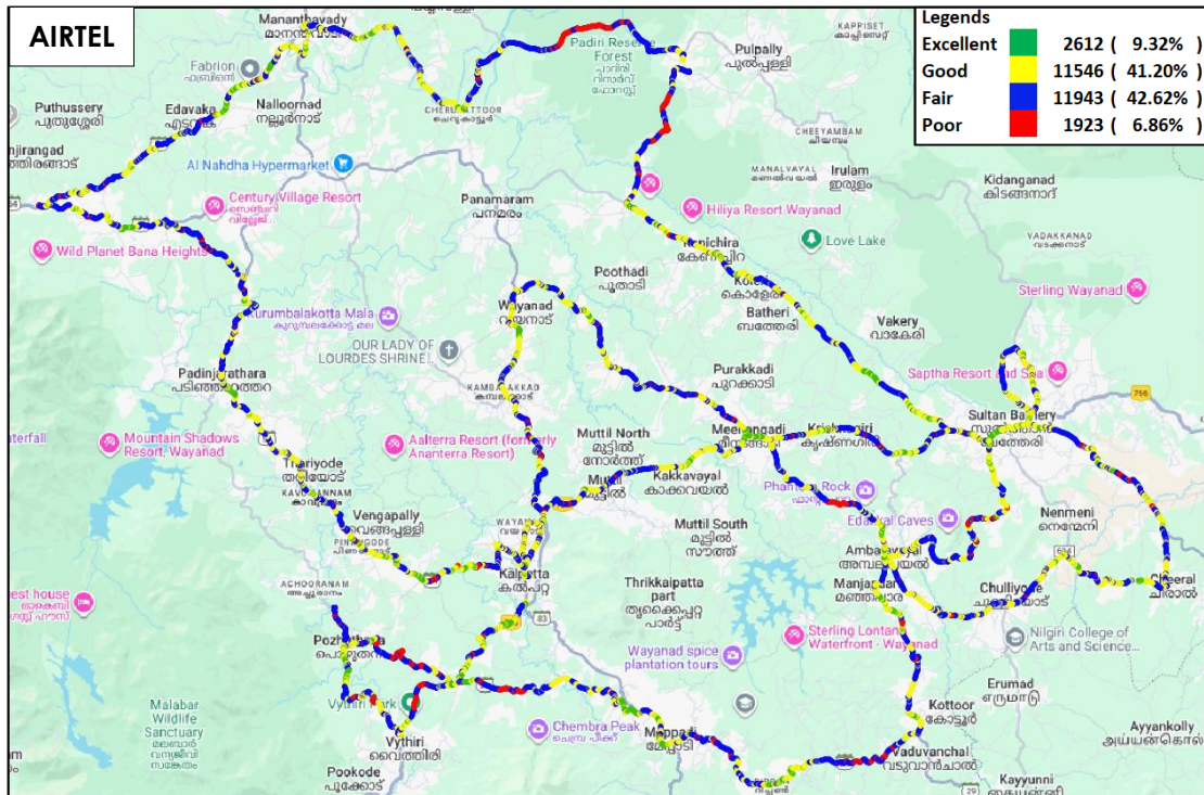
Figure-45: Signal strength auto-selection mode 5G/4G/3G/2G – AIRTEL.
