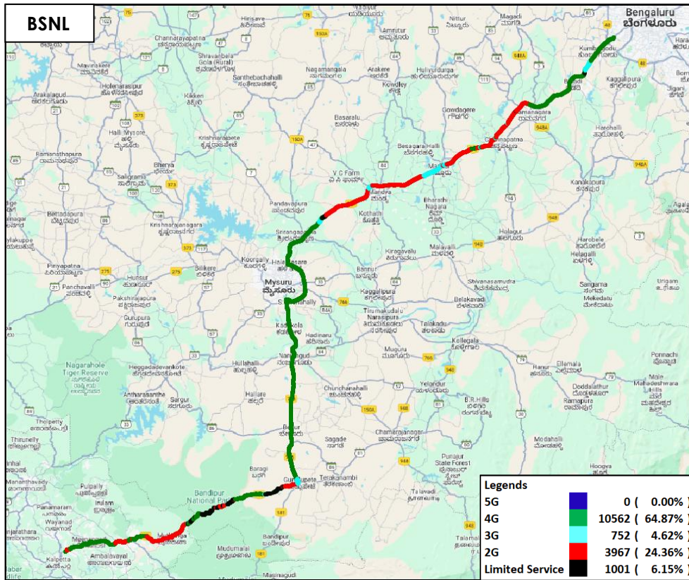
Figure-36: Serving technology plots in auto-selection mode (5G/4G/3G/2G)-BSNL.
