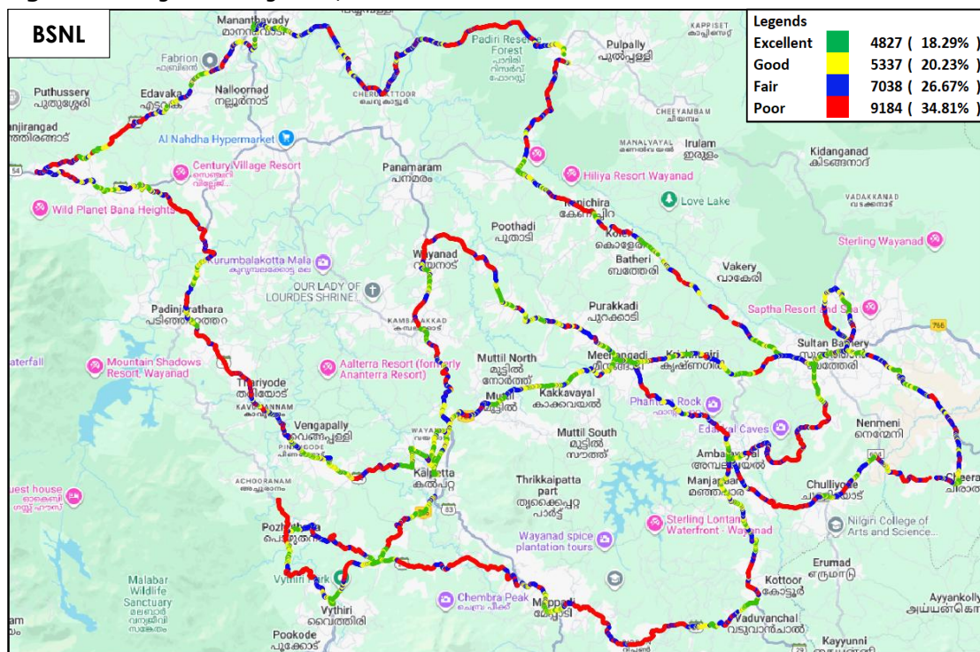
Figure-43: Signal strength 3G/2G network mode – BSNL.
