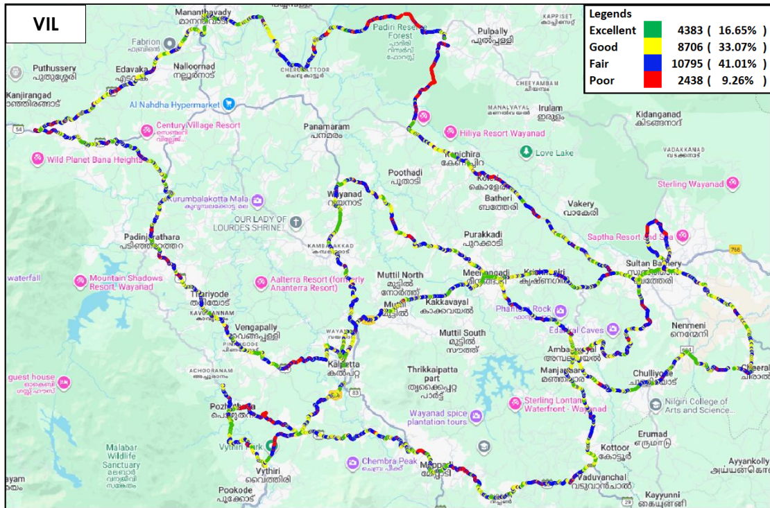
Figure-44: Signal strength 3G/2G network mode – VIL.
