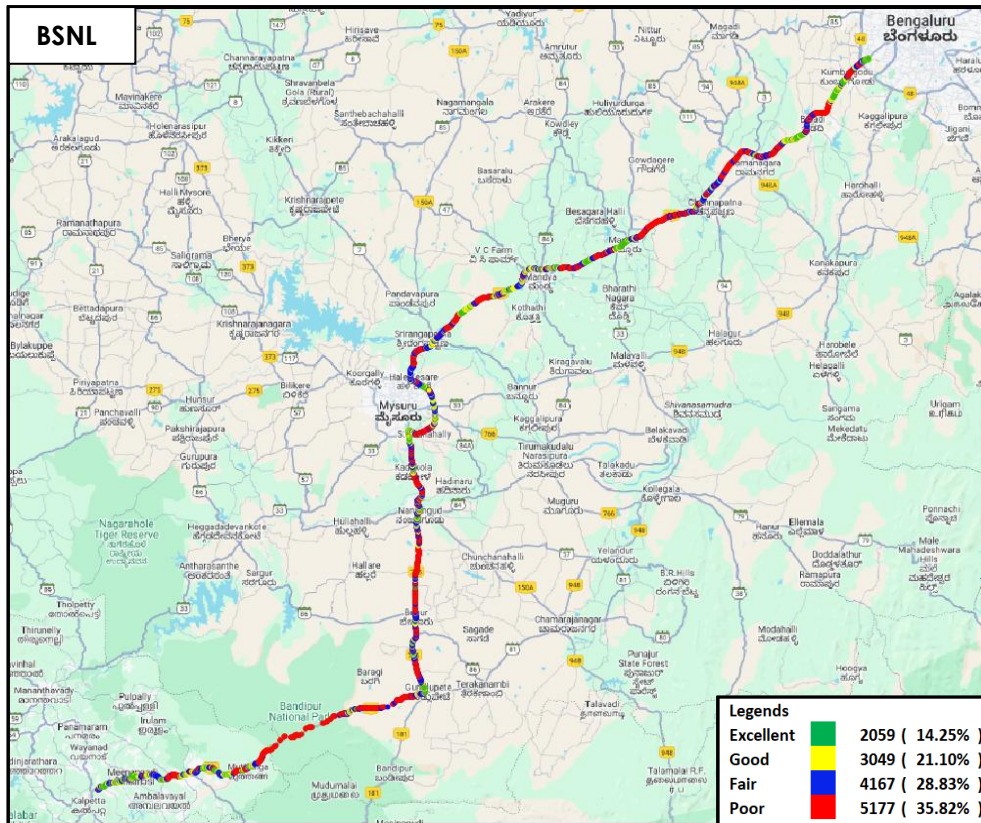
Figure-50: Signal strength 3G/2G network mode – BSNL.
