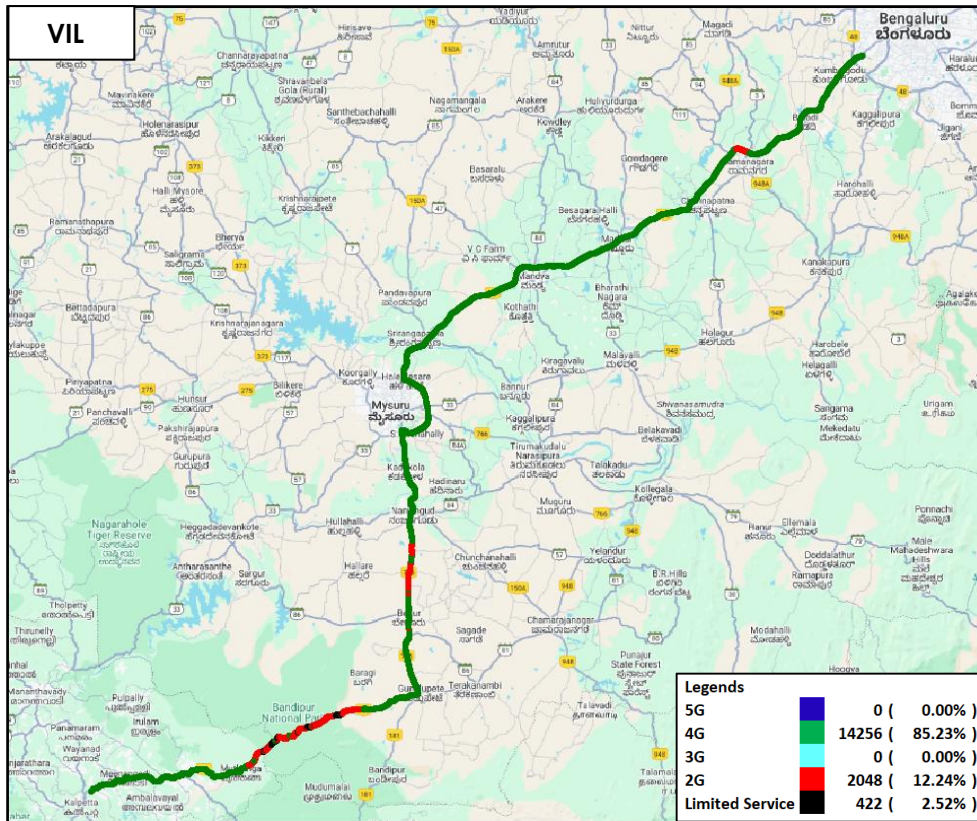
Figure-38: Serving technology plots in auto-selection mode (5G/4G/3G/2G)-VIL.
