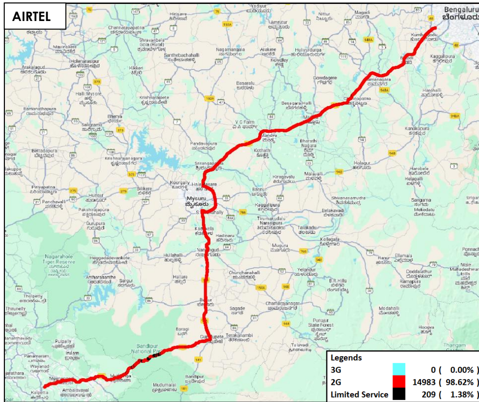
Figure-28: Serving technology plots 3G/2G network mode – AIRTEL.
