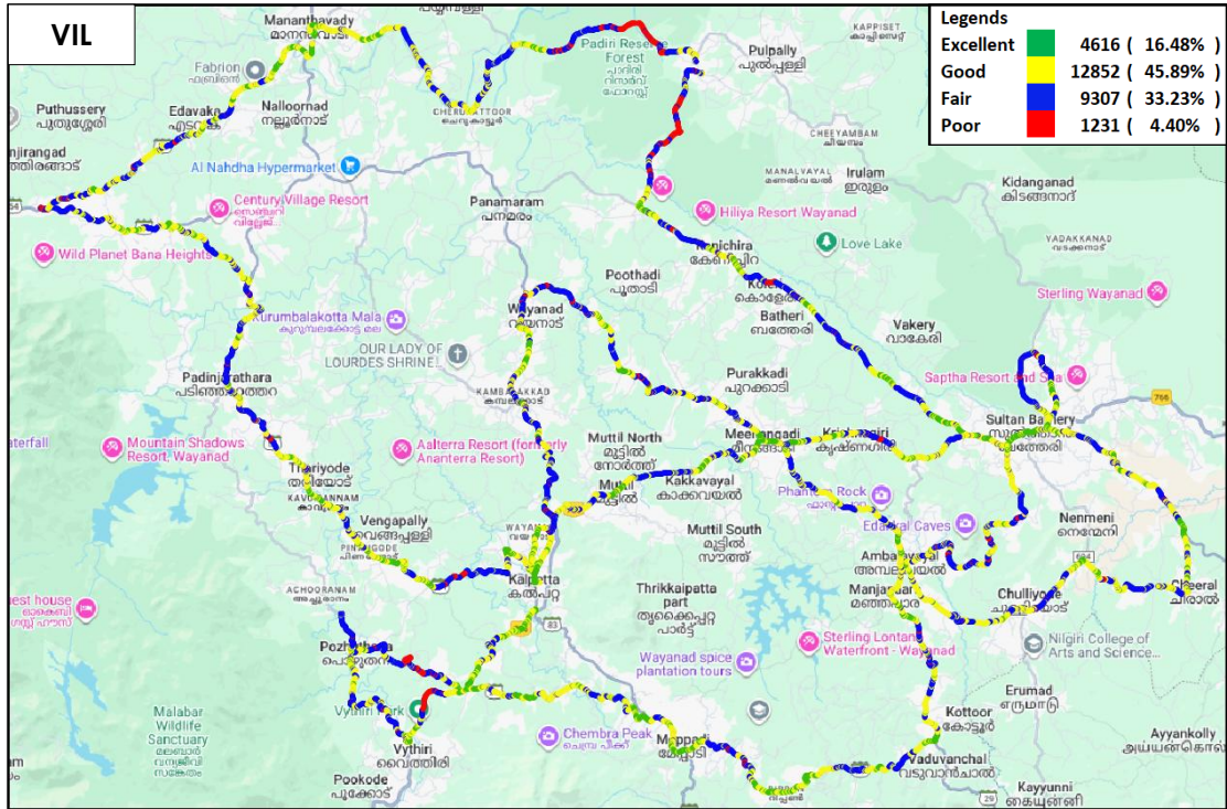
Figure-48: Signal strength auto-selection mode 5G/4G/3G/2G – VIL.
