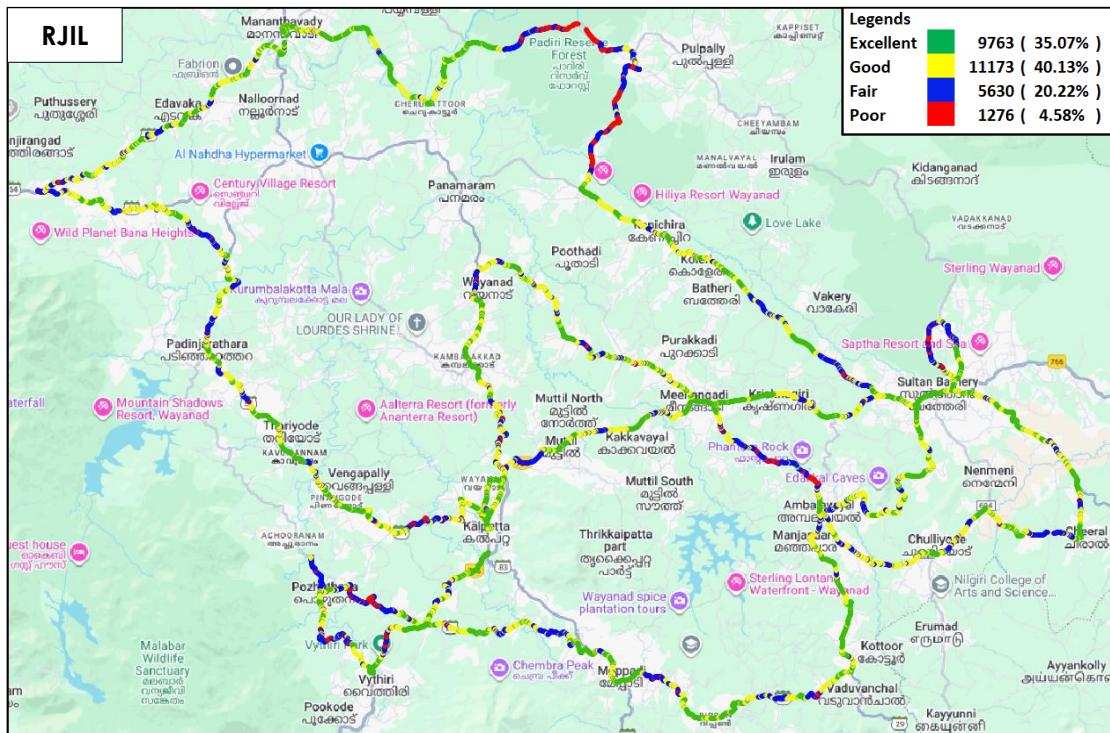
Figure-47: Signal strength auto-selection mode 5G/4G/3G/2G – RJIL.
