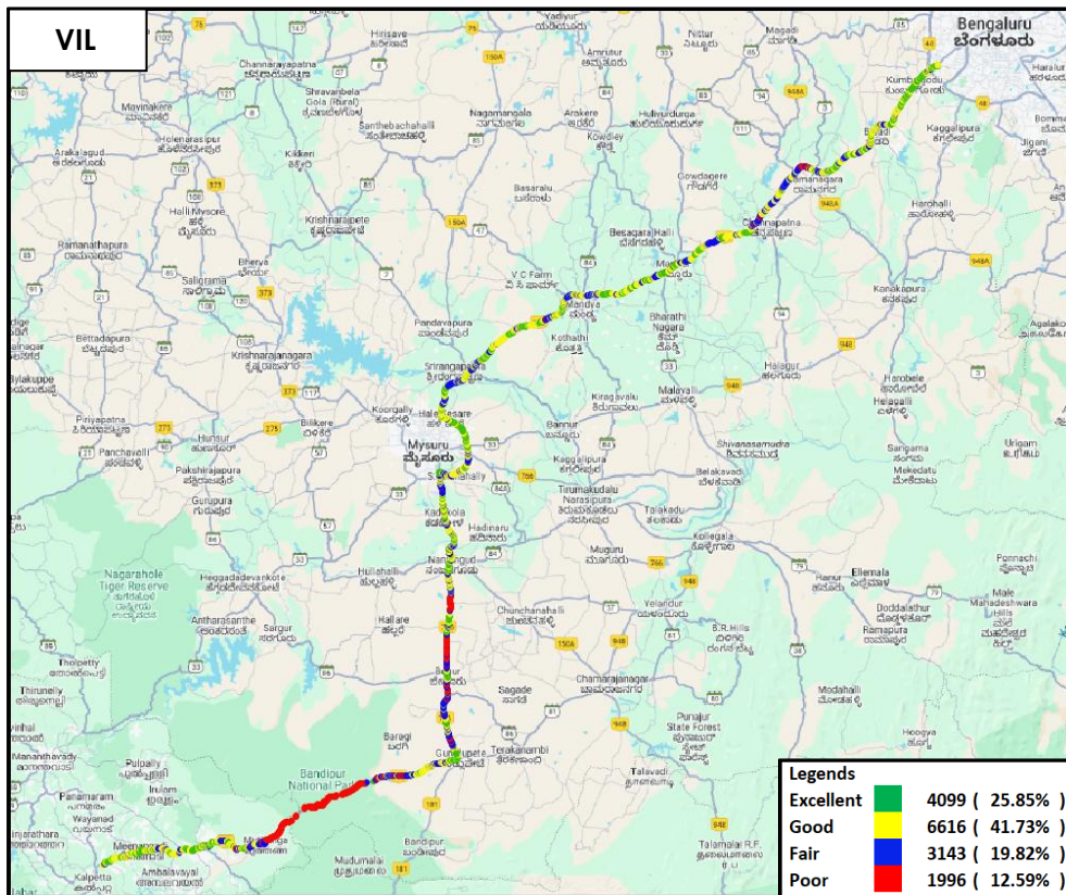
Figure-55: Signal strength auto-selection mode 5G/4G/3G/2G -VIL
