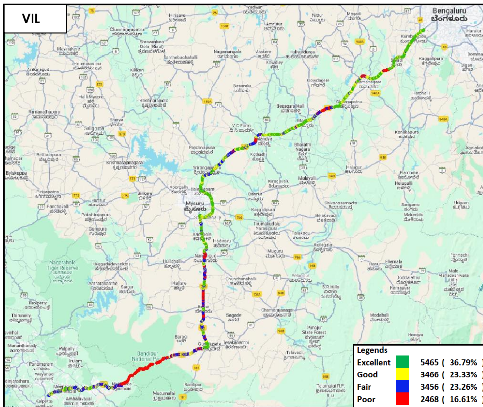
Figure-51: Signal strength 3G/2G network mode – VIL.
