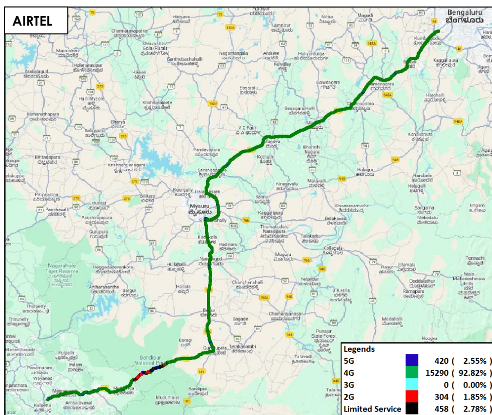
Figure-35: Serving technology plots in auto-selection mode (5G/4G/3G/2G)-AIRTEL
