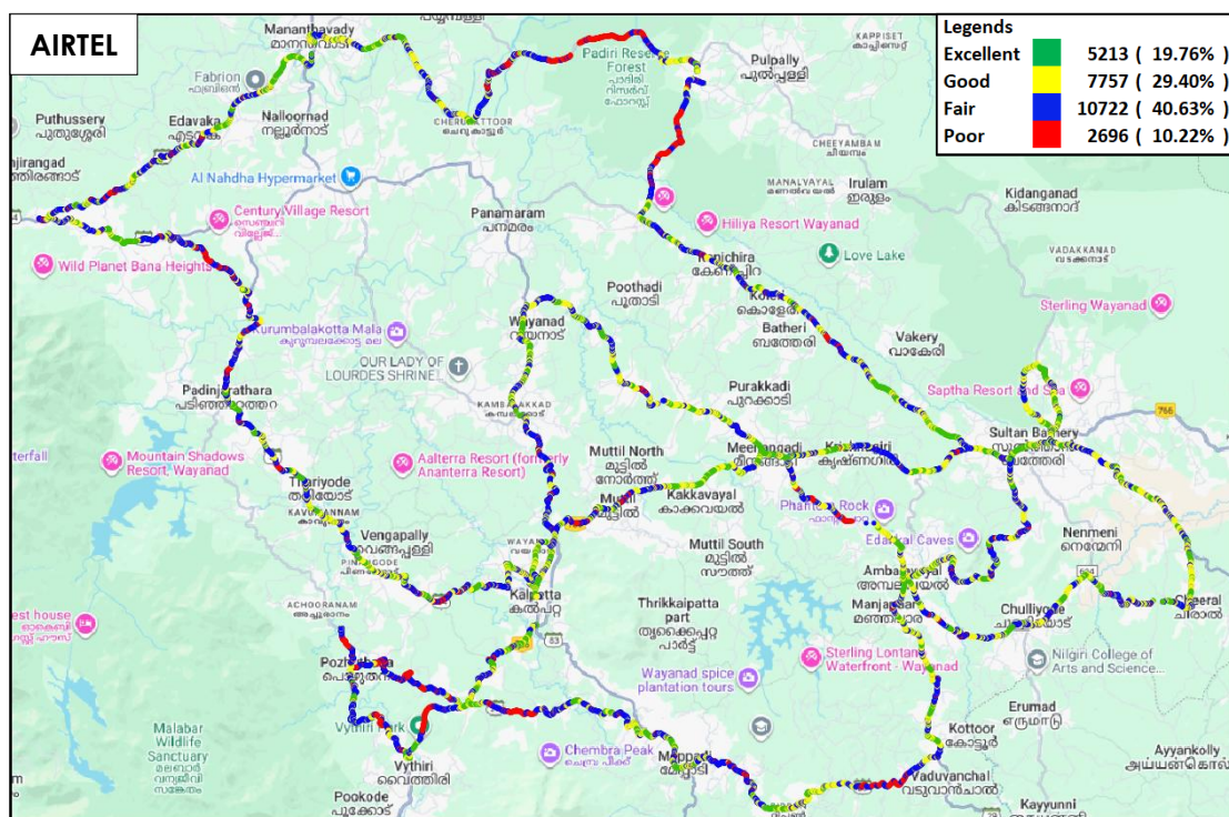
Figure-42: Signal strength 3G/2G network mode – AIRTEL.
