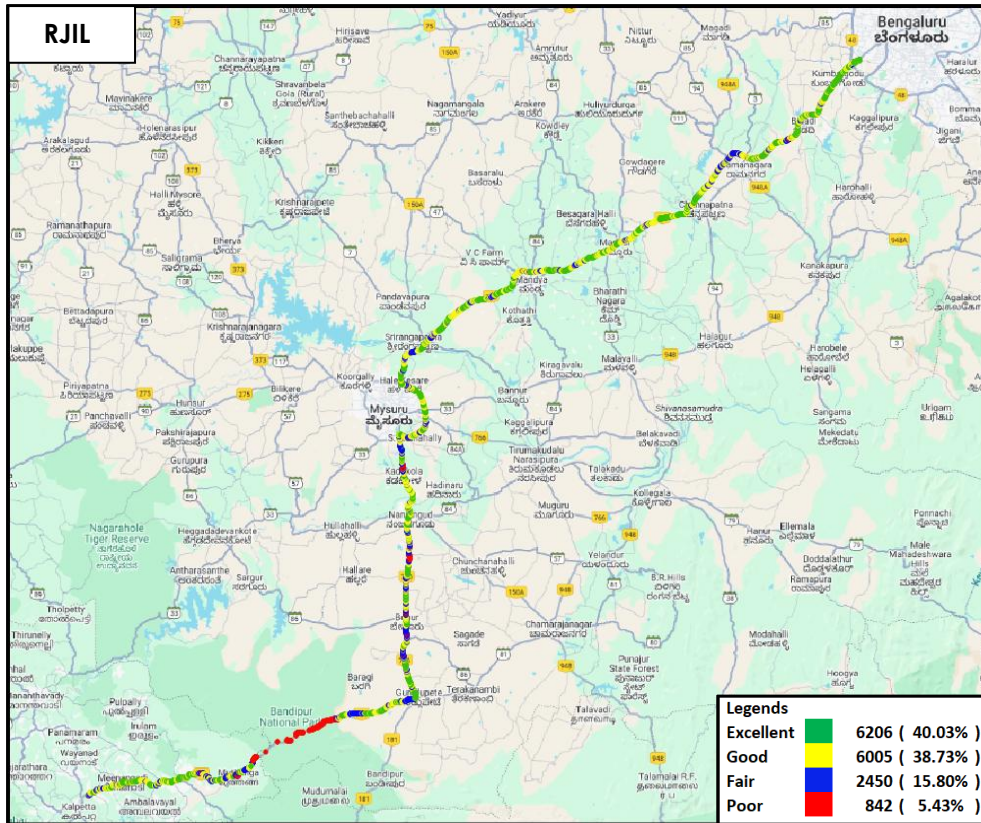
Figure-54: Signal strength auto-selection mode 5G/4G/3G/2G -RJIL
