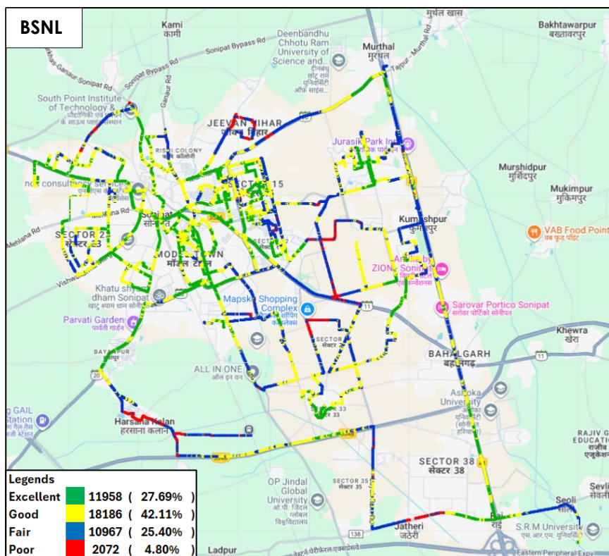
Figure-33: Signal strength auto-selection mode (5G/4G/3G/2G) voice - BSNL.
