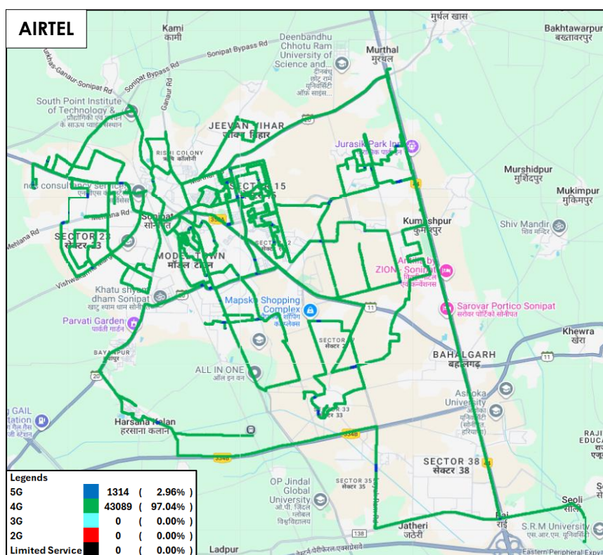
Figure-16: Serving technology plot in auto-selection mode (5G/4G/3G/2G) voice - AIRTEL.
