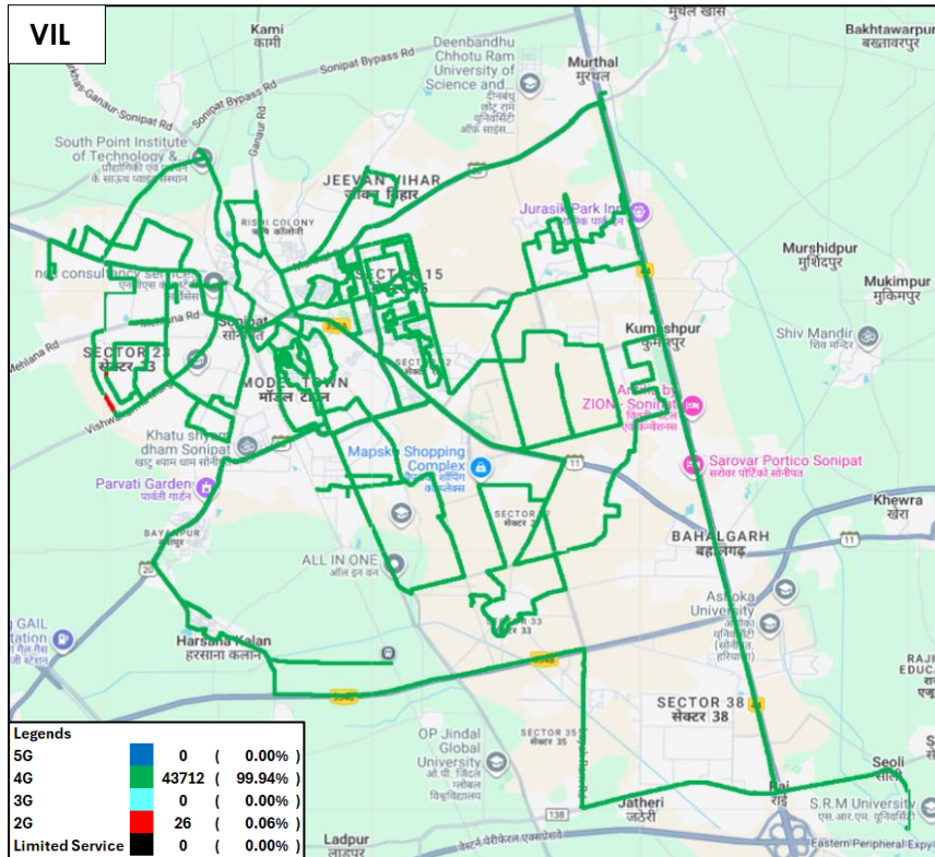
Figure-26: Serving technology plot in auto-selection mode (5G/4G/3G/2G) data - VIL
