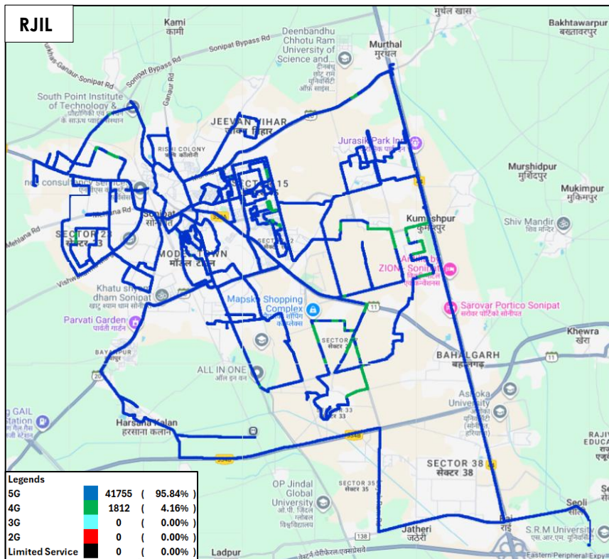
Figure-25: Serving technology plot in auto-selection mode (5G/4G/3G/2G) data - RJIL.
