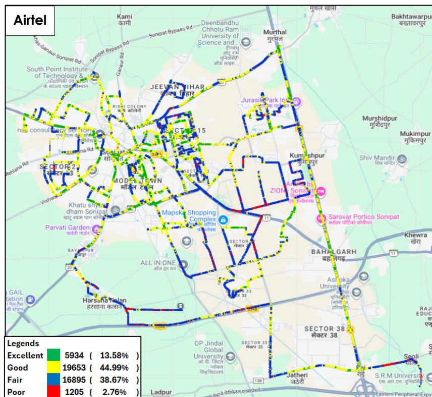
Figure-36: Signal strength auto-selection mode (5G/4G/3G/2G) data - AIRTEL.
