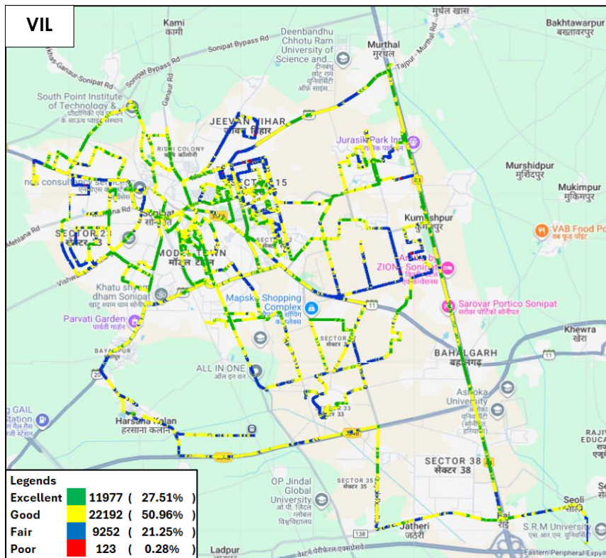
Figure-35: Signal strength auto-selection mode (5G/4G/3G/2G) voice - VIL.
