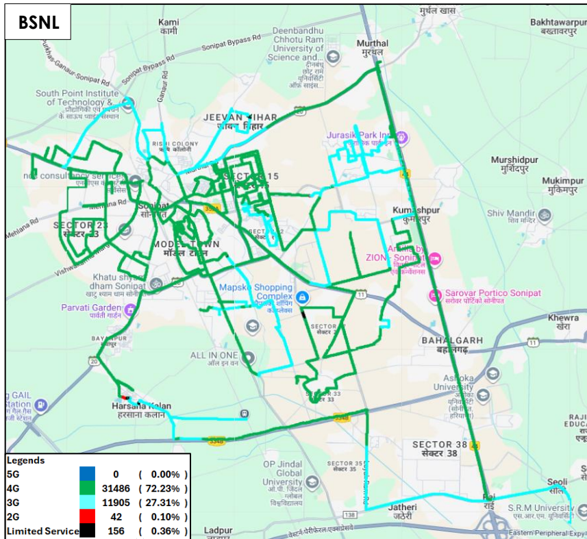
Figure-24: Serving technology plot in auto-selection mode (5G/4G/3G/2G) data - BSNL.
