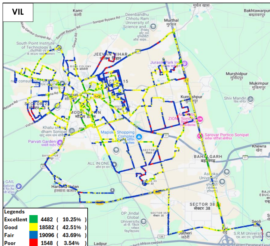
Figure-39: Signal strength auto-selection mode (5G/4G/3G/2G) data - VIL.
