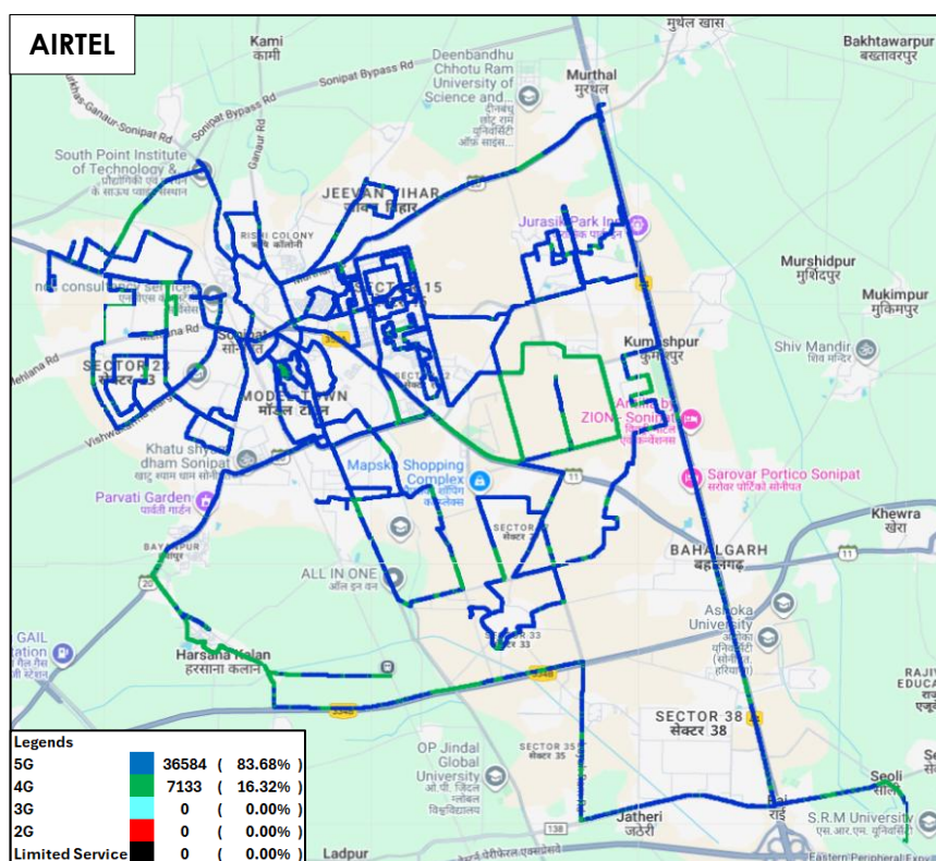
Figure-23: Serving technology plot in auto-selection mode (5G/4G/3G/2G) data - AIRTEL.
