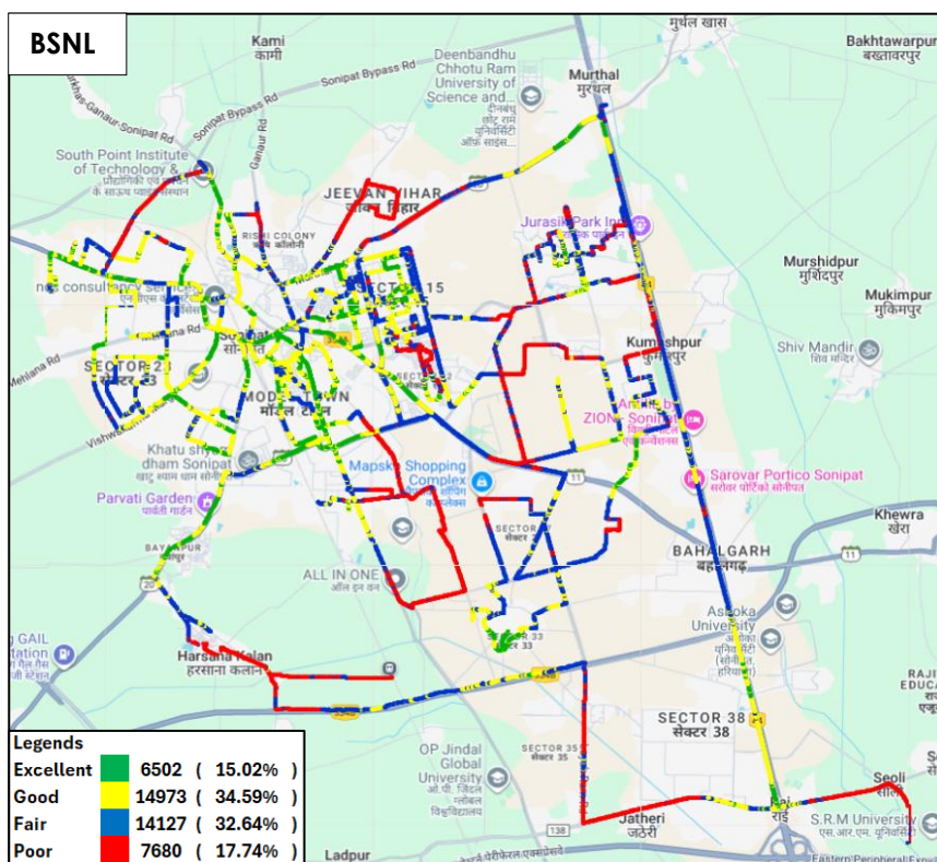
Figure-37: Signal strength auto-selection mode (5G/4G/3G/2G) data - BSNL.
