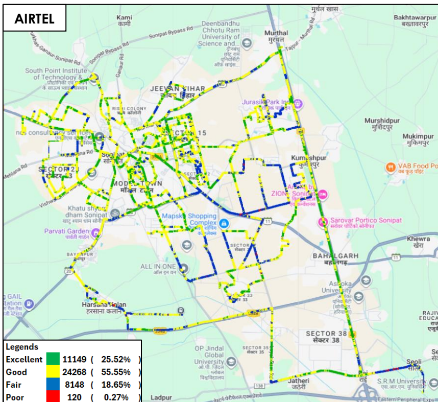
Figure-32: Signal strength auto-selection mode (5G/4G/3G/2G) voice - AIRTEL.
