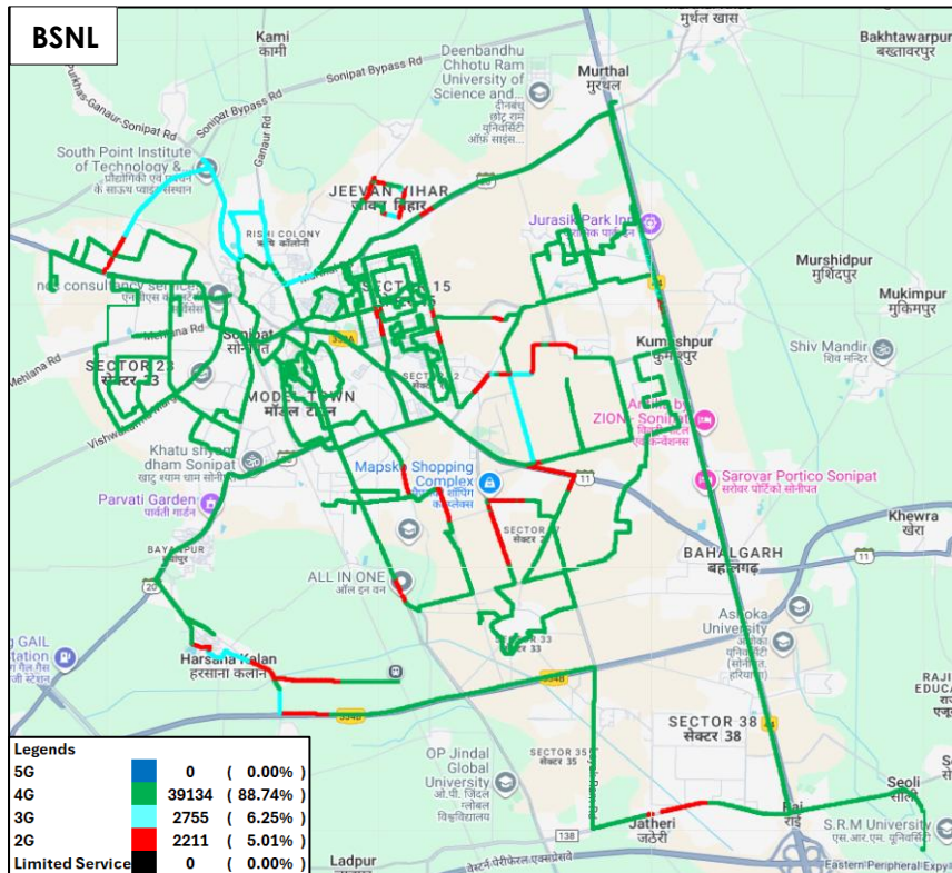
Figure-17: Serving technology plot in auto-selection mode (5G/4G/3G/2G) voice - BSNL.
