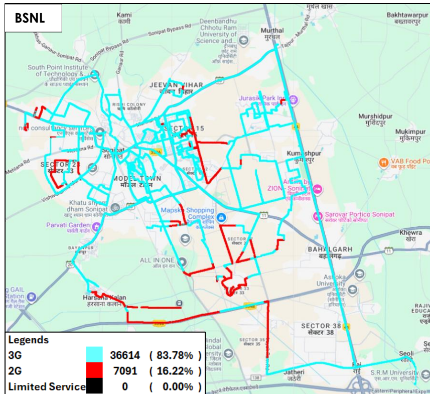
Figure-10: Serving technology plot 3G/2G network mode - BSNL.
