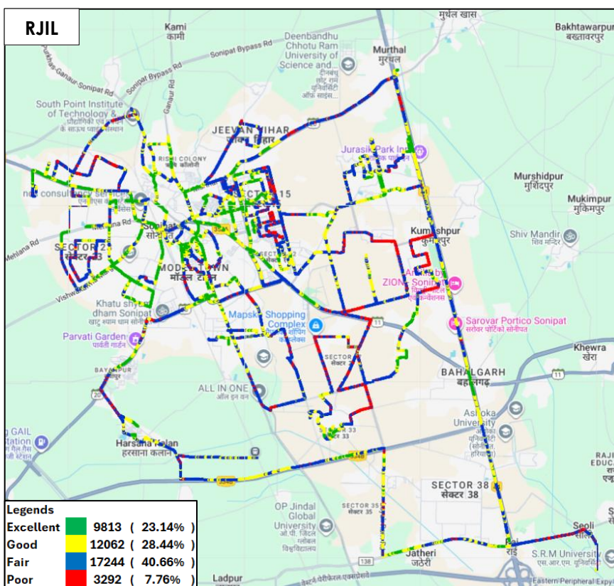
Figure-38: Signal strength auto-selection mode (5G/4G/3G/2G) data - RJIL.
