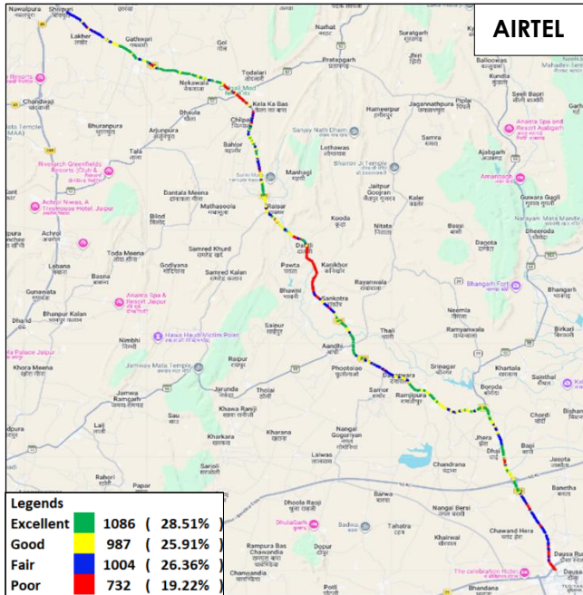
Figure-28: Signal strength 3G/2G network mode - AIRTEL.
