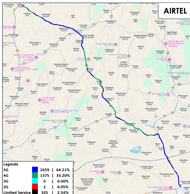
Figure-23: Serving technology plot in auto-selection mode (5G/4G/3G/2G) data - AIRTEL.
