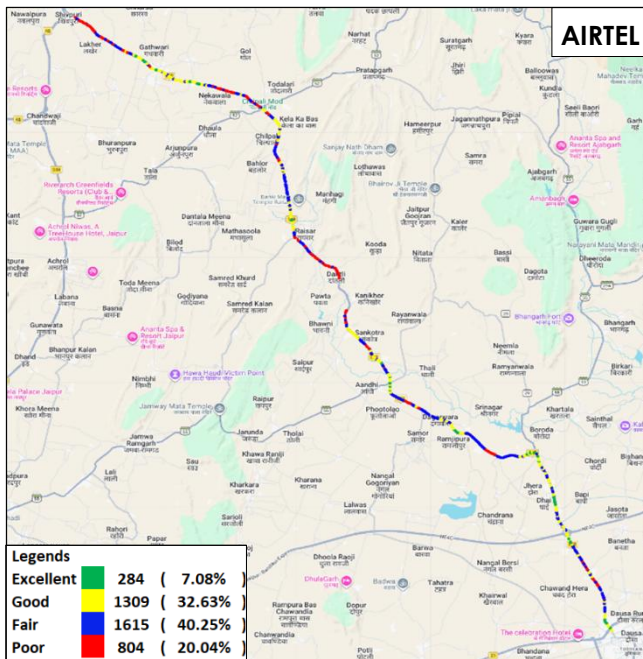
Figure-35: Signal strength auto-selection mode (5G/4G/3G/2G) data - AIRTEL.
