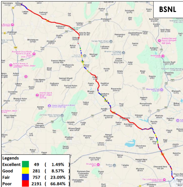
Figure-29: Signal strength 3G/2G network mode - BSNL.
