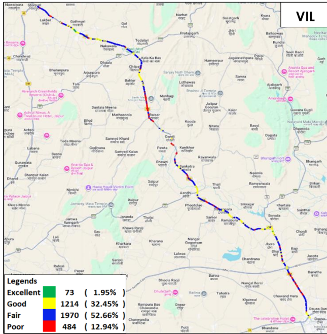
Figure-38: Signal strength auto-selection mode (5G/4G/3G/2G) data - VIL.
