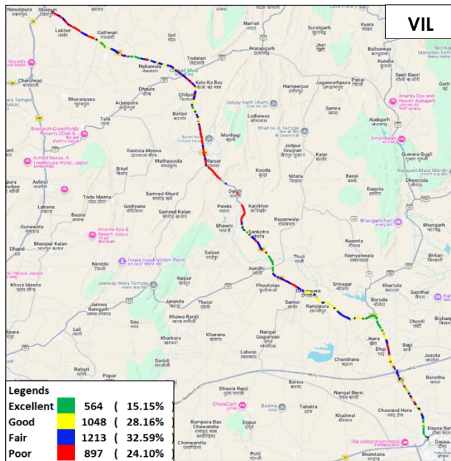
Figure-30: Signal strength 3G/2G network mode - VIL.
