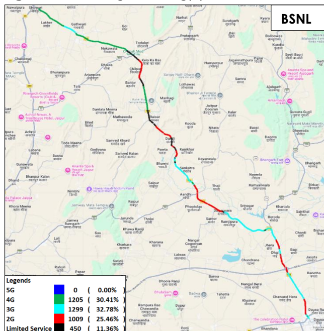
Figure-17: Serving technology plots in auto-selection mode (5G/4G/3G/2G) voice - BSNL.
