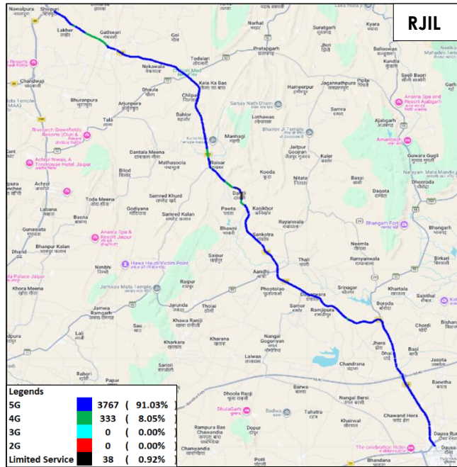
Figure-25: Serving technology plot in auto-selection mode (5G/4G/3G/2G) data - RJIL.
