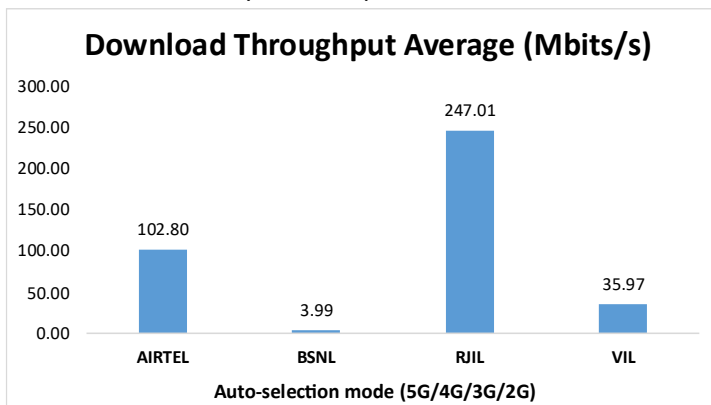
Figure 21: Download throughput.
