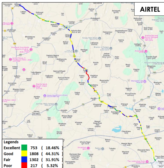
Figure-31: Signal strength auto-selection mode (5G/4G/3G/2G) voice - AIRTEL.
