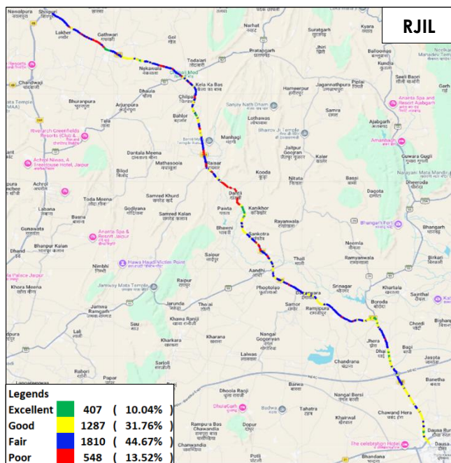
Figure-37: Signal strength auto-selection mode (5G/4G/3G/2G) data - RJIL.
