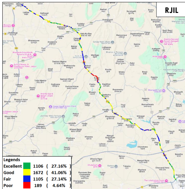
Figure-33: Signal strength auto-selection mode (5G/4G/3G/2G) voice - RJIL.
