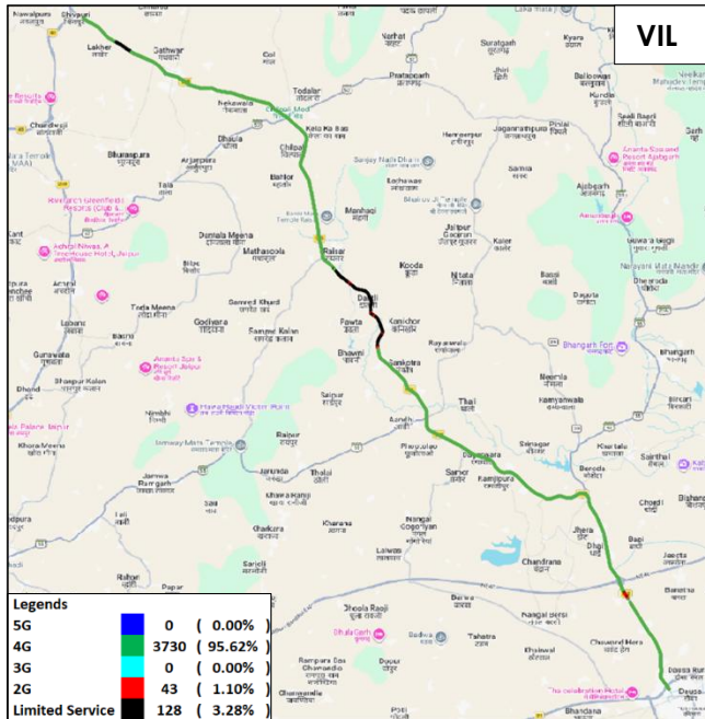
Figure-26: Serving technology plot in auto-selection mode (5G/4G/3G/2G) data - VIL.
