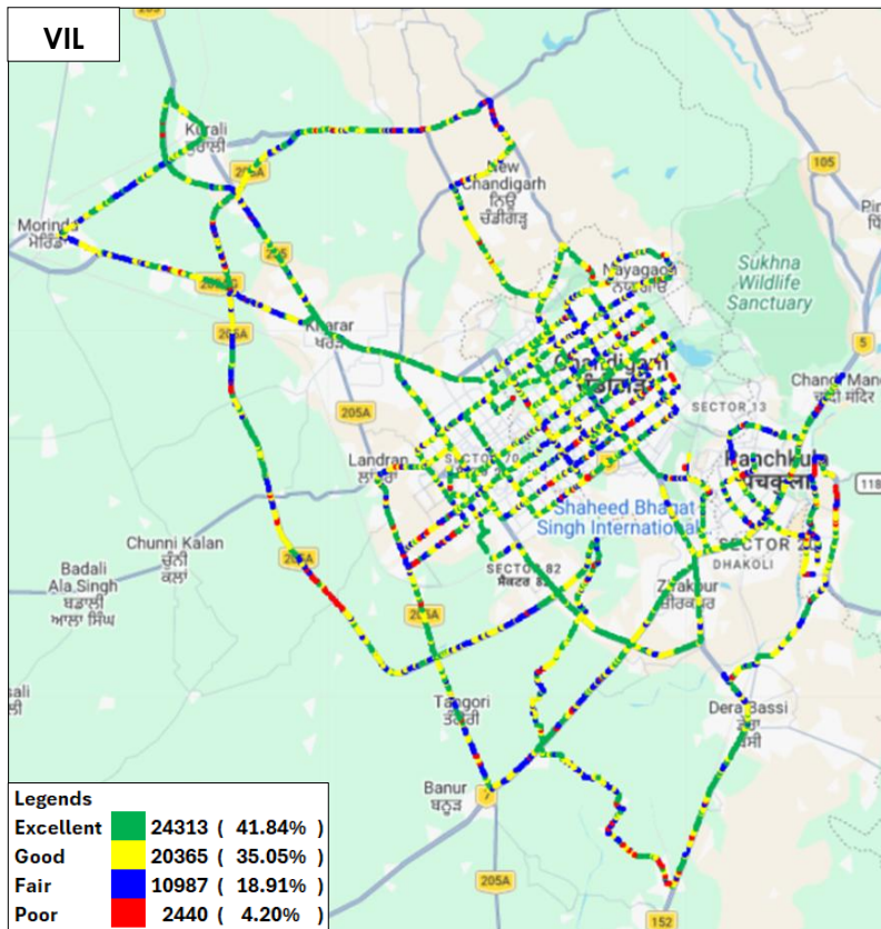
Figure-32: Signal strength 3G/2G network mode voice - VIL.
