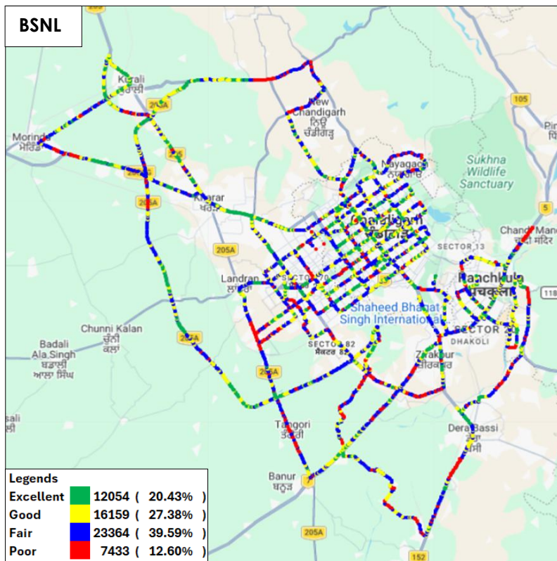
Figure-31: Signal strength 3G/2G network mode voice - BSNL.
