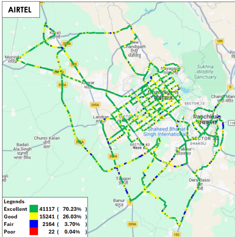
Figure-30: Signal strength 3G/2G network mode voice - AIRTEL.
