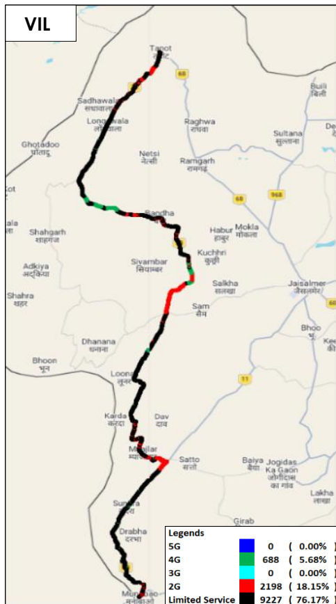
Figure-19: Serving technology plots in auto-selection mode (5G/4G/3G/2G) voice - VIL.
