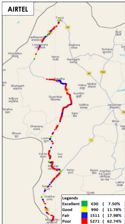
Figure-31: Signal strength auto-selection mode (5G/4G/3G/2G) voice - AIRTEL.
