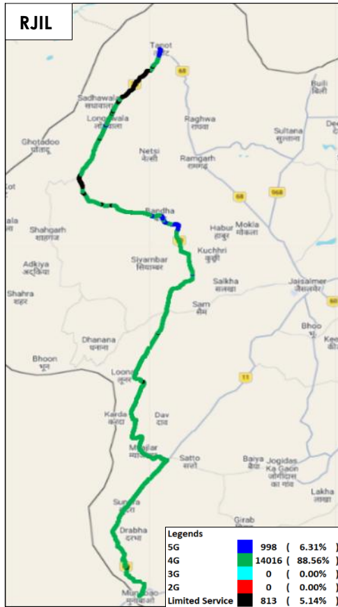
Figure-25: Serving technology plot in auto-selection mode (5G/4G/3G/2G) data - RJIL.
