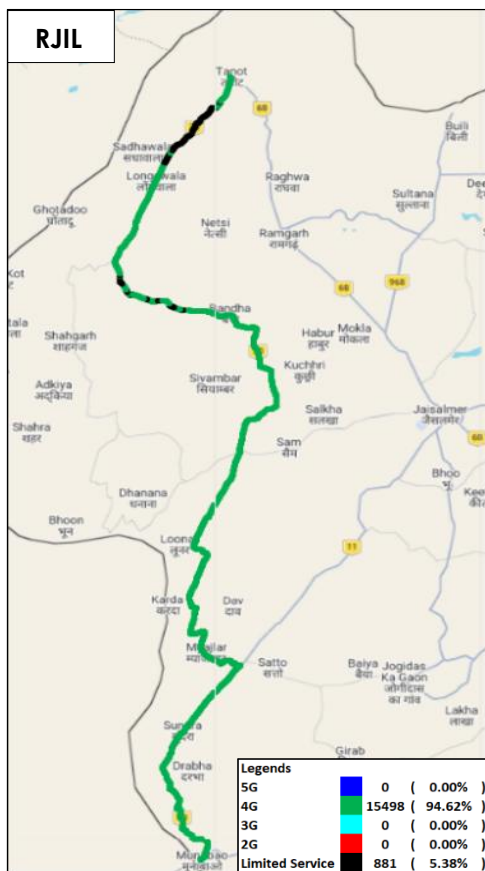
Figure-18: Serving technology plots in auto-selection mode (5G/4G/3G/2G) voice - RJIL.
