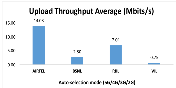
Figure-22: Upload throughput.
