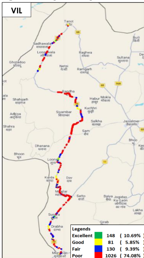
Figure-38: Signal strength auto-selection mode (5G/4G/3G/2G) data - VIL.
