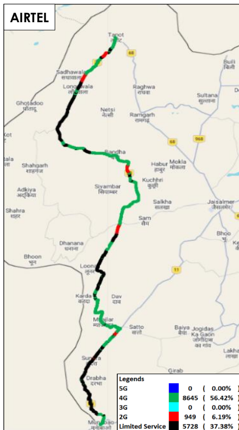
Figure-16: Serving technology plots in auto-selection mode (5G/4G/3G/2G) voice - AIRTEL.
