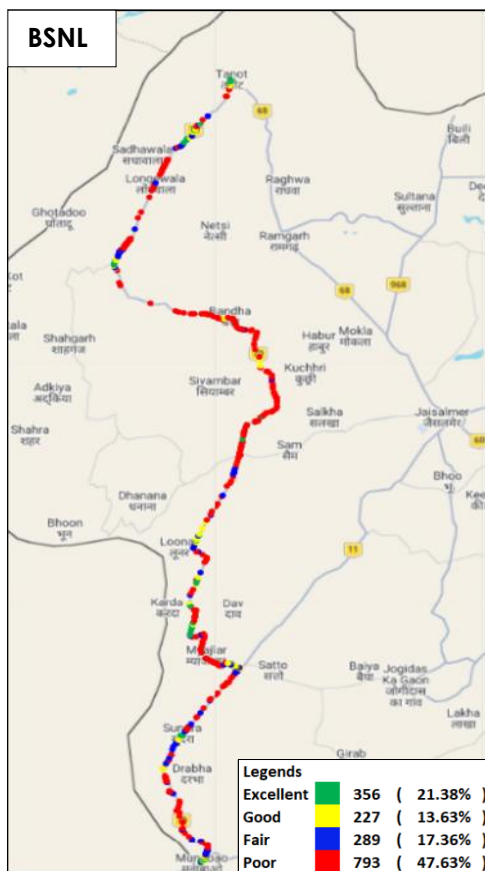
Figure-32: Signal strength auto-selection mode (5G/4G/3G/2G) voice - BSNL.
