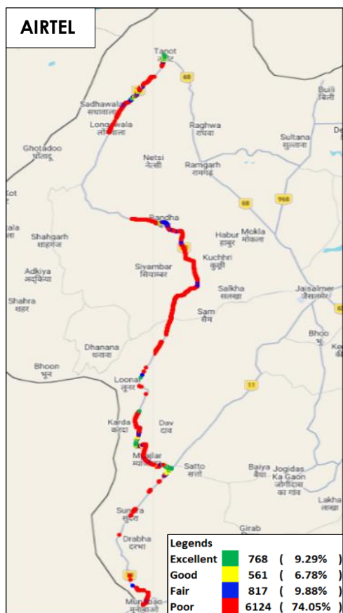
Figure-28: Signal strength 3G/2G network mode - AIRTEL.
