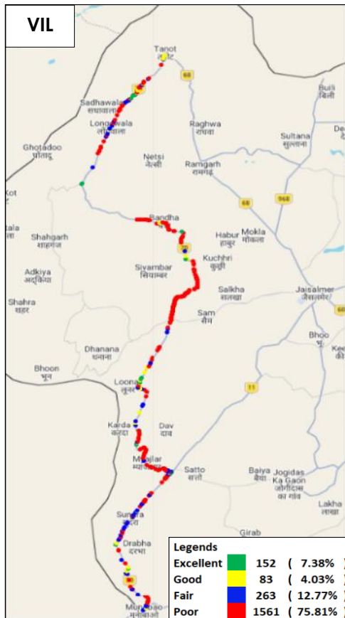
Figure-34: Signal strength auto-selection mode (5G/4G/3G/2G) voice - VIL.
