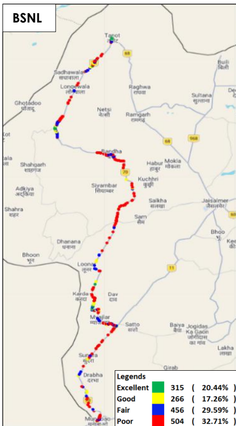
Figure-36: Signal strength auto-selection mode (5G/4G/3G/2G) data - BSNL.
