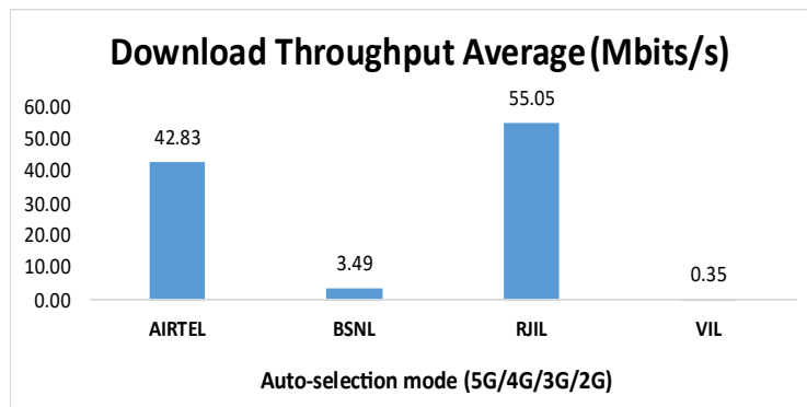
Figure 21: Download throughput.
