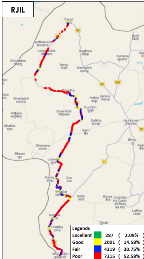
Figure-37: Signal strength auto-selection mode (5G/4G/3G/2G) data - RJIL.
