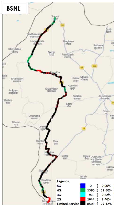
Figure-17: Serving technology plots in auto-selection mode (5G/4G/3G/2G) voice - BSNL.
