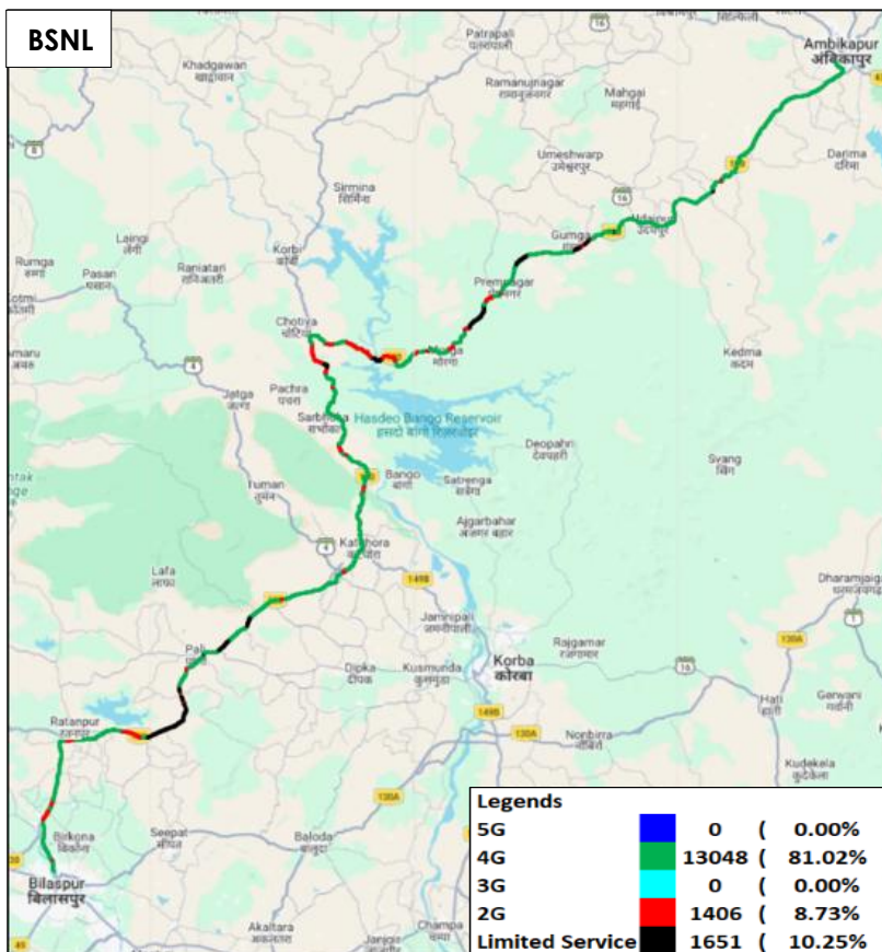
Figure-24: Serving technology plot in auto-selection mode (5G/4G/3G/2G) data - BSNL.
