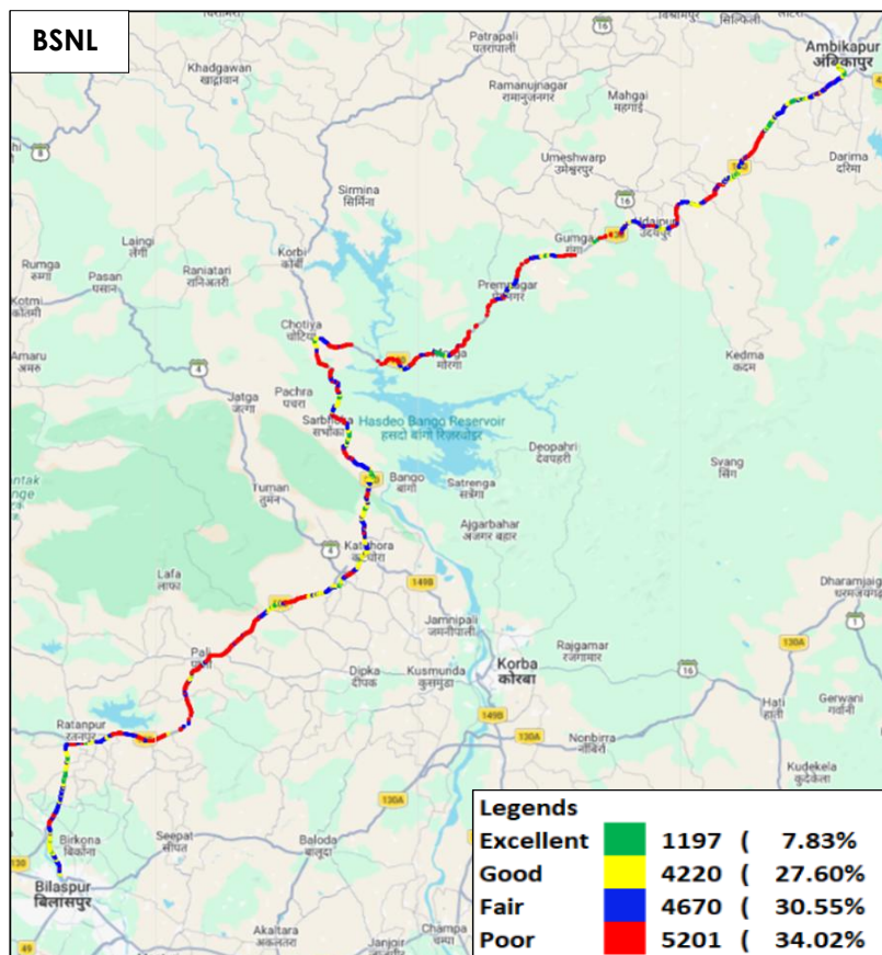
Figure-32: Signal strength auto-selection mode (5G/4G/3G/2G) voice - BSNL.
