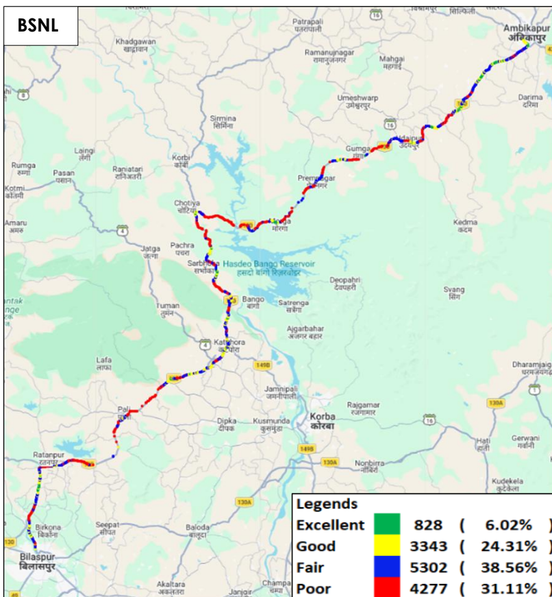
Figure-36: Signal strength auto-selection mode (5G/4G/3G/2G) data - BSNL.
