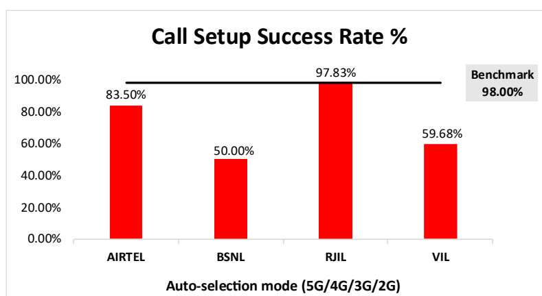
Figure-13: Performance for call setup success rate.
