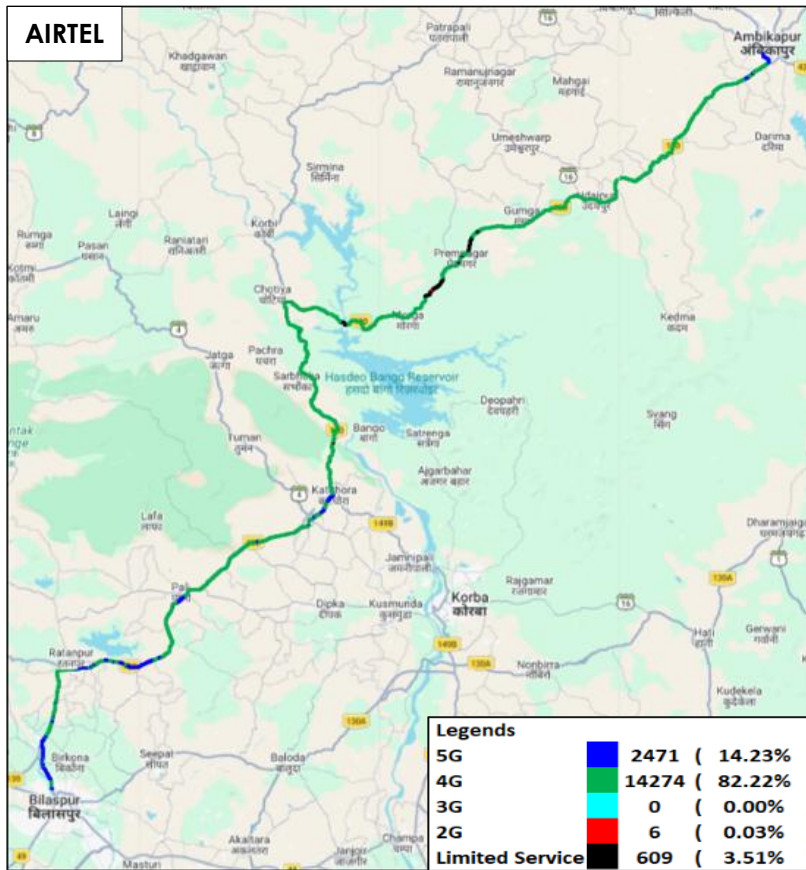
Figure-23: Serving technology plot in auto-selection mode (5G/4G/3G/2G) data - AIRTEL.
