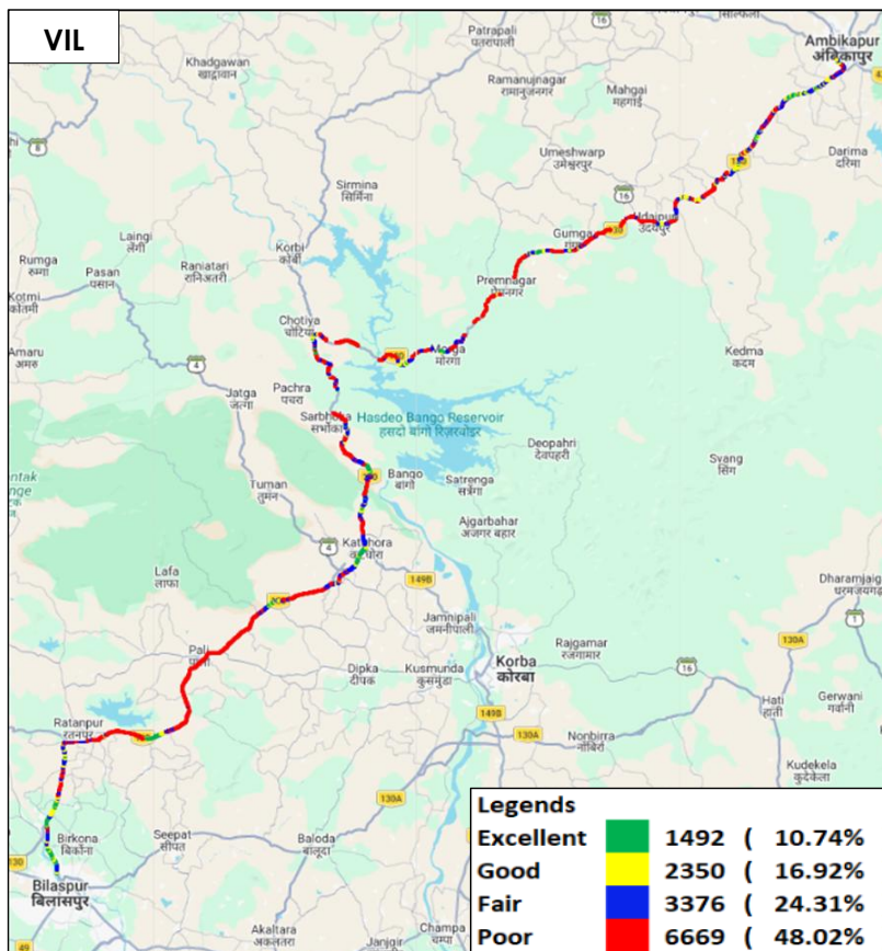
Figure-30: Signal strength 3G/2G network mode - VIL.
