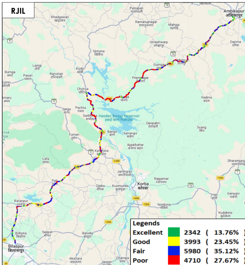
Figure-37: Signal strength auto-selection mode (5G/4G/3G/2G) data - RJIL.
