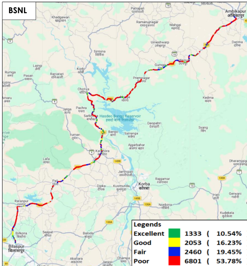
Figure-29: Signal strength 3G/2G network mode - BSNL.
