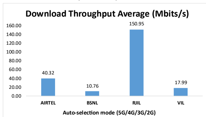
Figure 21: Download throughput.
