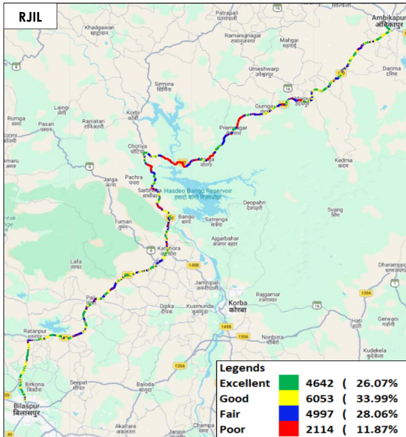
Figure-33: Signal strength auto-selection mode (5G/4G/3G/2G) voice - RJIL.
