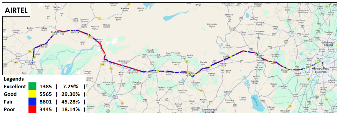
Figure-23: Signal strength auto-selection mode (5G/4G/3G/2G) data – AIRTEL.
