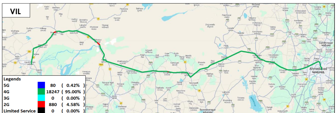
Figure-10: Serving technology plots in auto-selection mode (5G/4G/3G/2G) voice - VIL.
