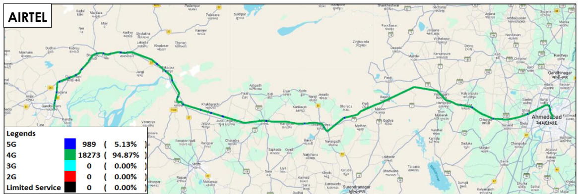
Figure-7: Serving technology plots in auto-selection mode (5G/4G/3G/2G) voice - AIRTEL.
