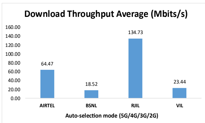
Figure 12: Download throughput.
