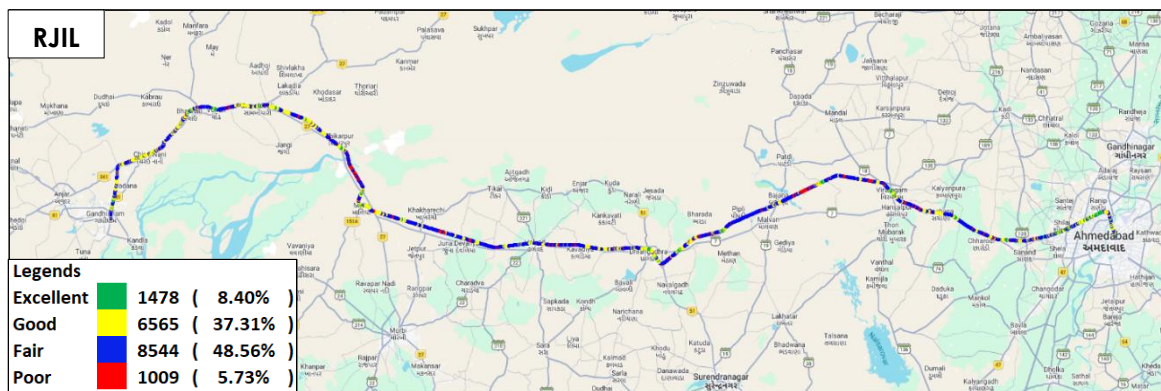
Figure-25: Signal strength auto-selection mode (5G/4G/3G/2G) data – RJIL.
