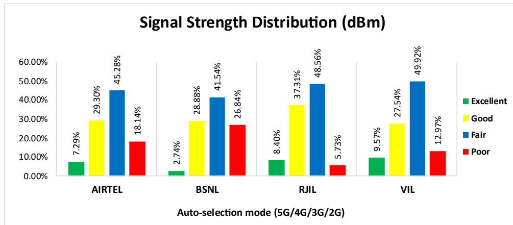
Figure-18: Signal strength distribution auto-selection mode (5G/4G/3G/2G) data.
