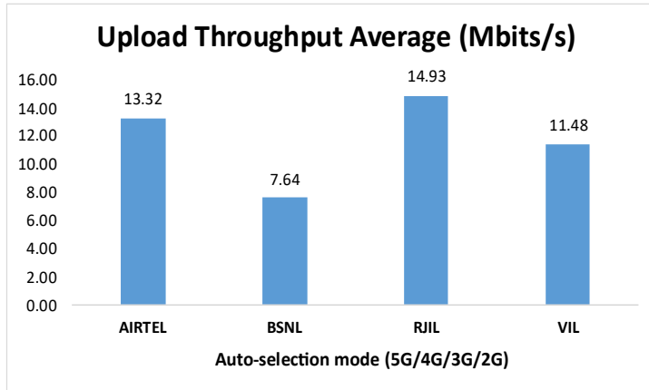
Figure-13: Upload throughput.
