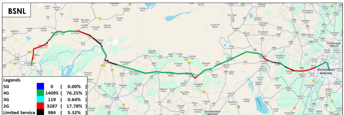
Figure-8: Serving technology plots in auto-selection mode (5G/4G/3G/2G) voice - BSNL.
