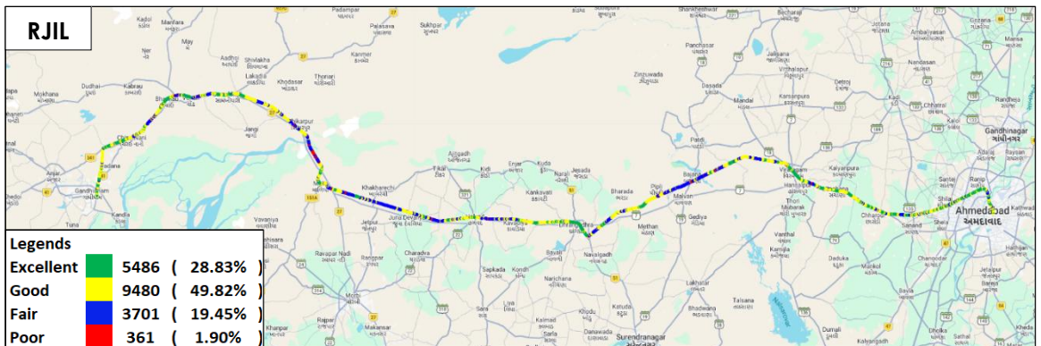
Figure-21: Signal strength auto-selection mode (5G/4G/3G/2G) voice - RJIL.
