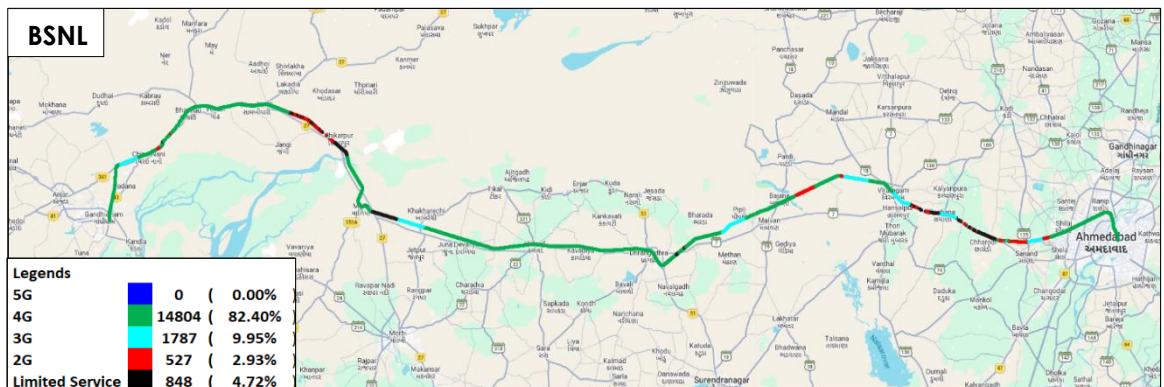
Figure-15: Serving technology plots in auto-selection mode (5G/4G/3G/2G) data - BSNL.
