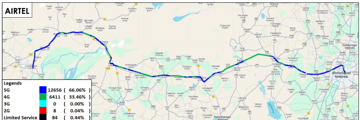
Figure-14: Serving technology plots in auto-selection mode (5G/4G/3G/2G) data - AIRTEL.
