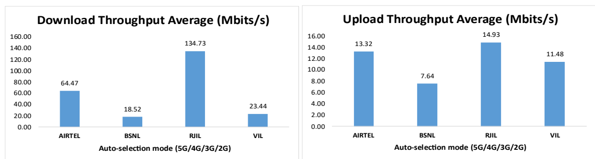
Figure- 3: Download and Upload throughput
