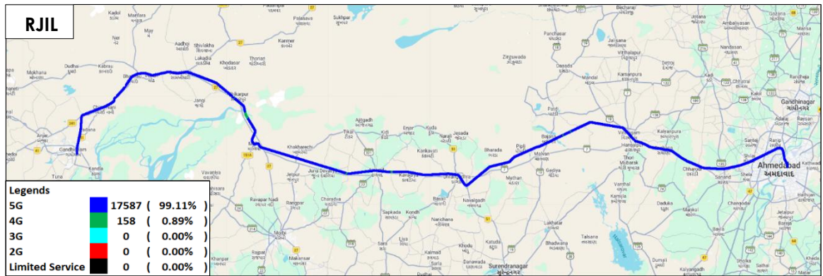
Figure-16: Serving technology plots in auto-selection mode (5G/4G/3G/2G) data - RJIL.
