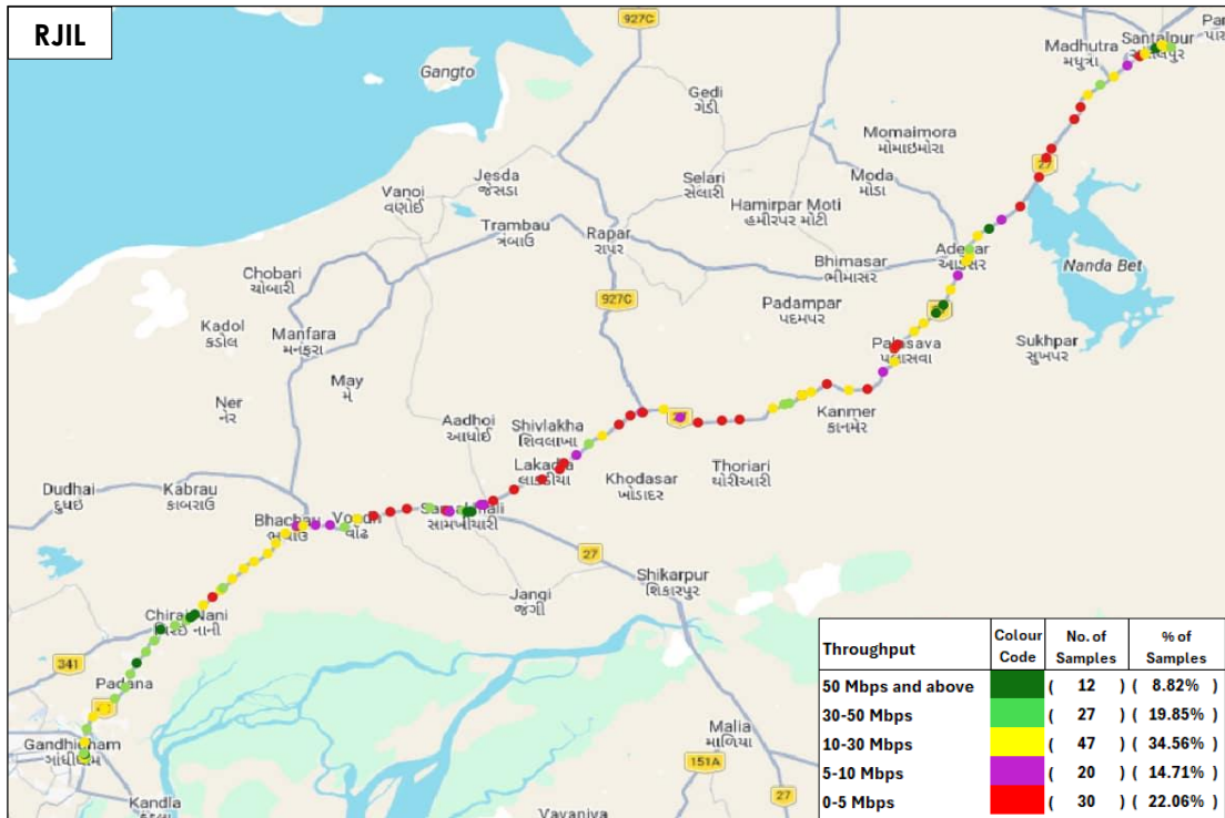
Figure-38: Upload throughput distribution auto-selection mode (5G/4G/3G/2G) - RJIL.
