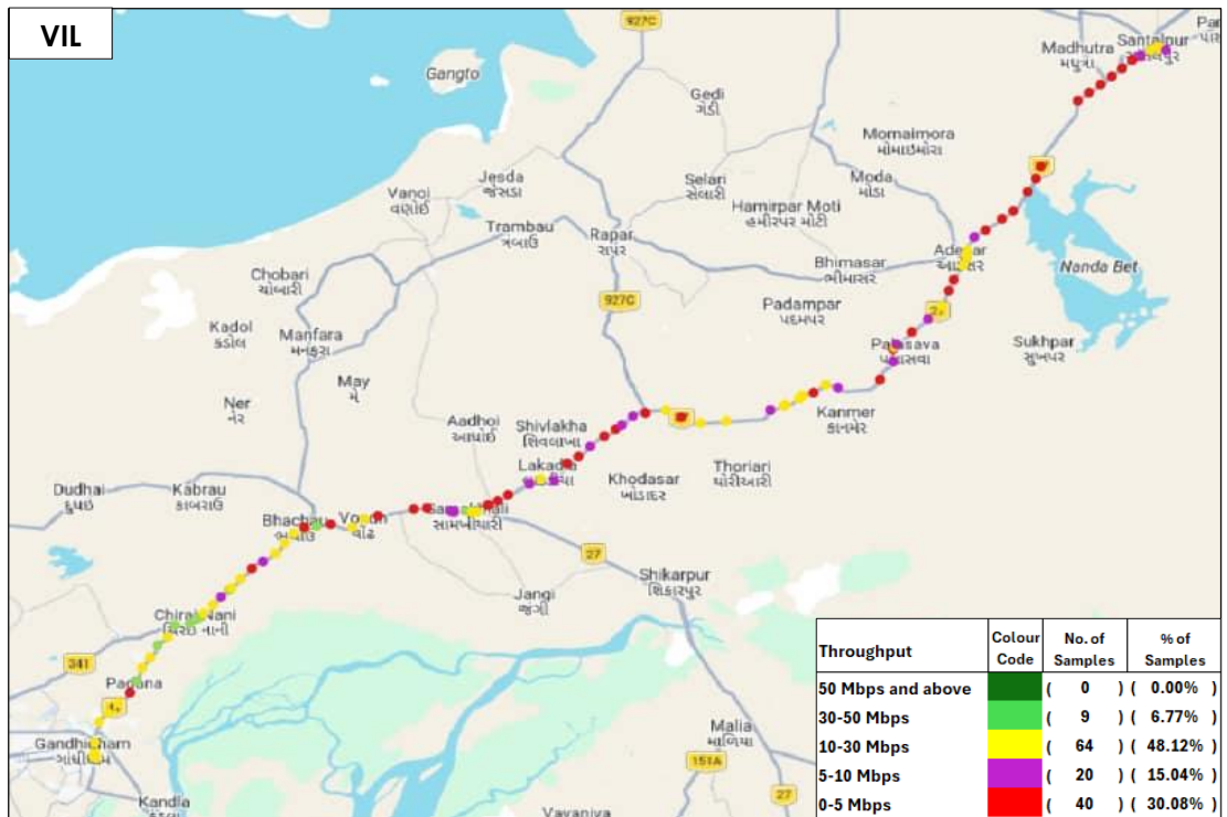
Figure-39: Upload throughput distribution auto-selection mode (5G/4G/3G/2G) - VIL.
