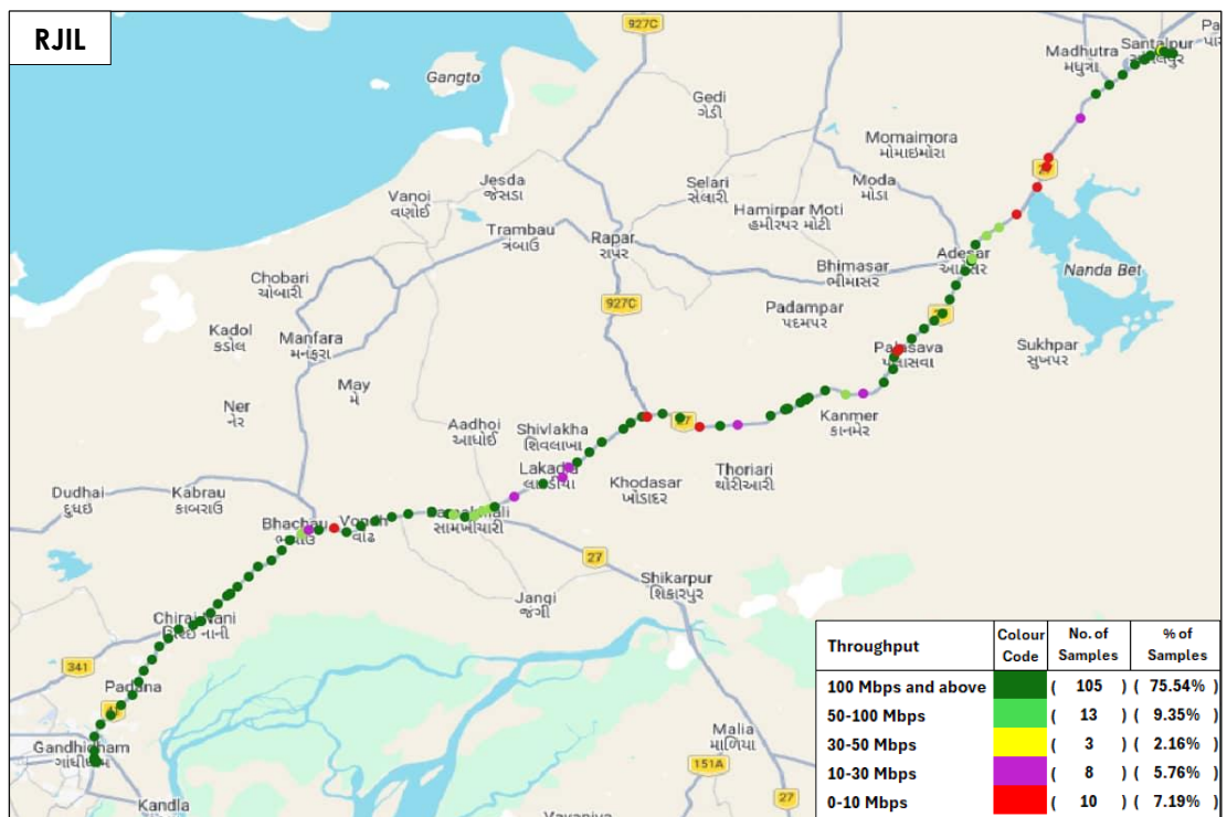
Figure-34: Download throughput distribution auto-selection mode (5G/4G/3G/2G) - RJIL.
