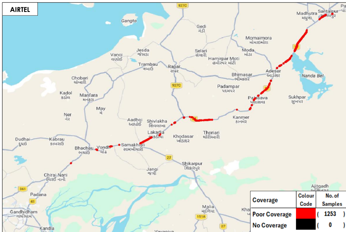
Figure-27: Poor coverage & no coverage locations in auto-selection mode (5G/4G/3G/2G) voice-Airtel.
