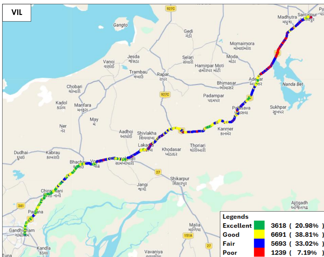
Figure-51: Signal strength auto-selection mode (5G/4G/3G/2G) voice - VIL.
