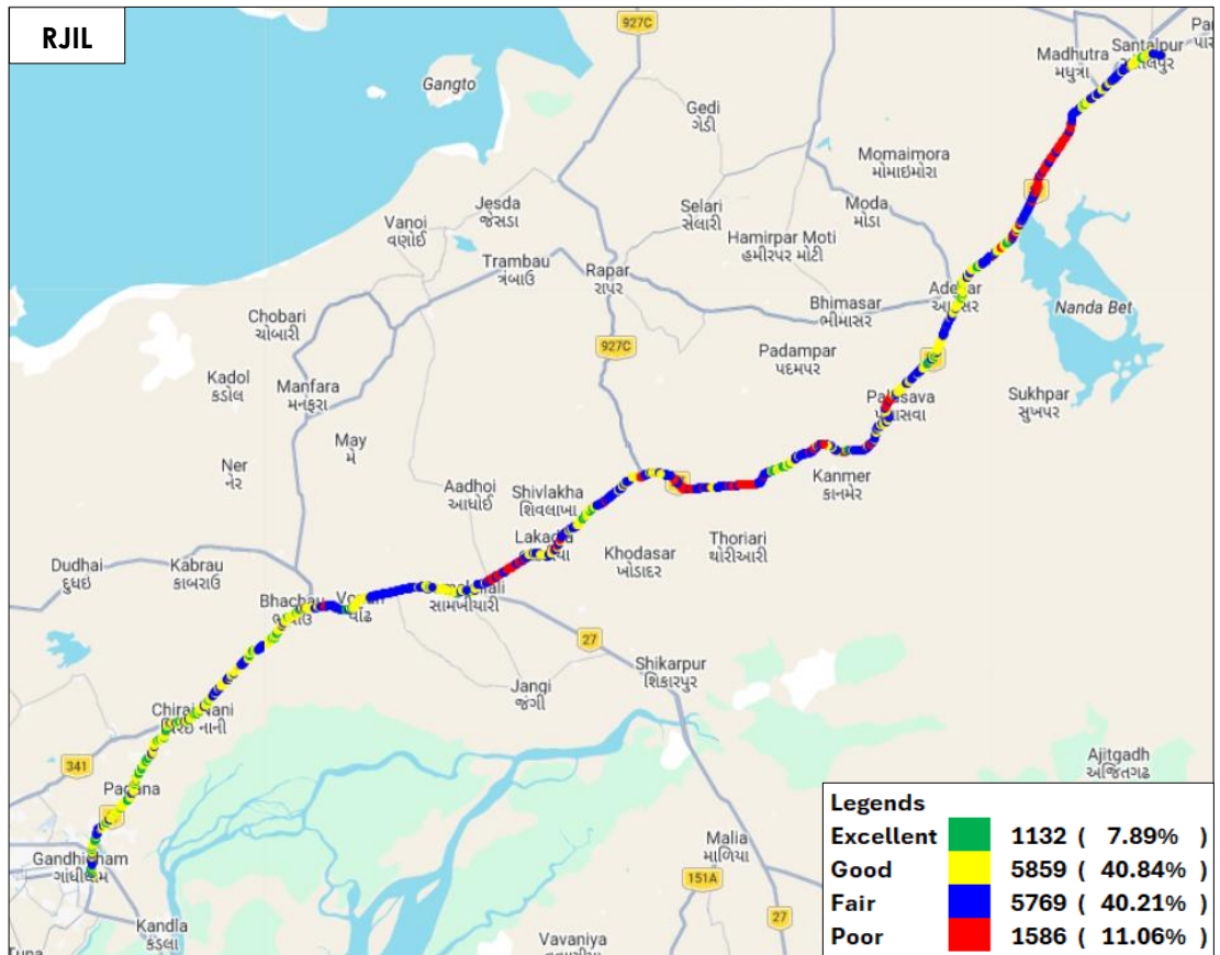
Figure-54: Signal strength auto-selection mode (5G/4G/3G/2G) data - RJIL.
