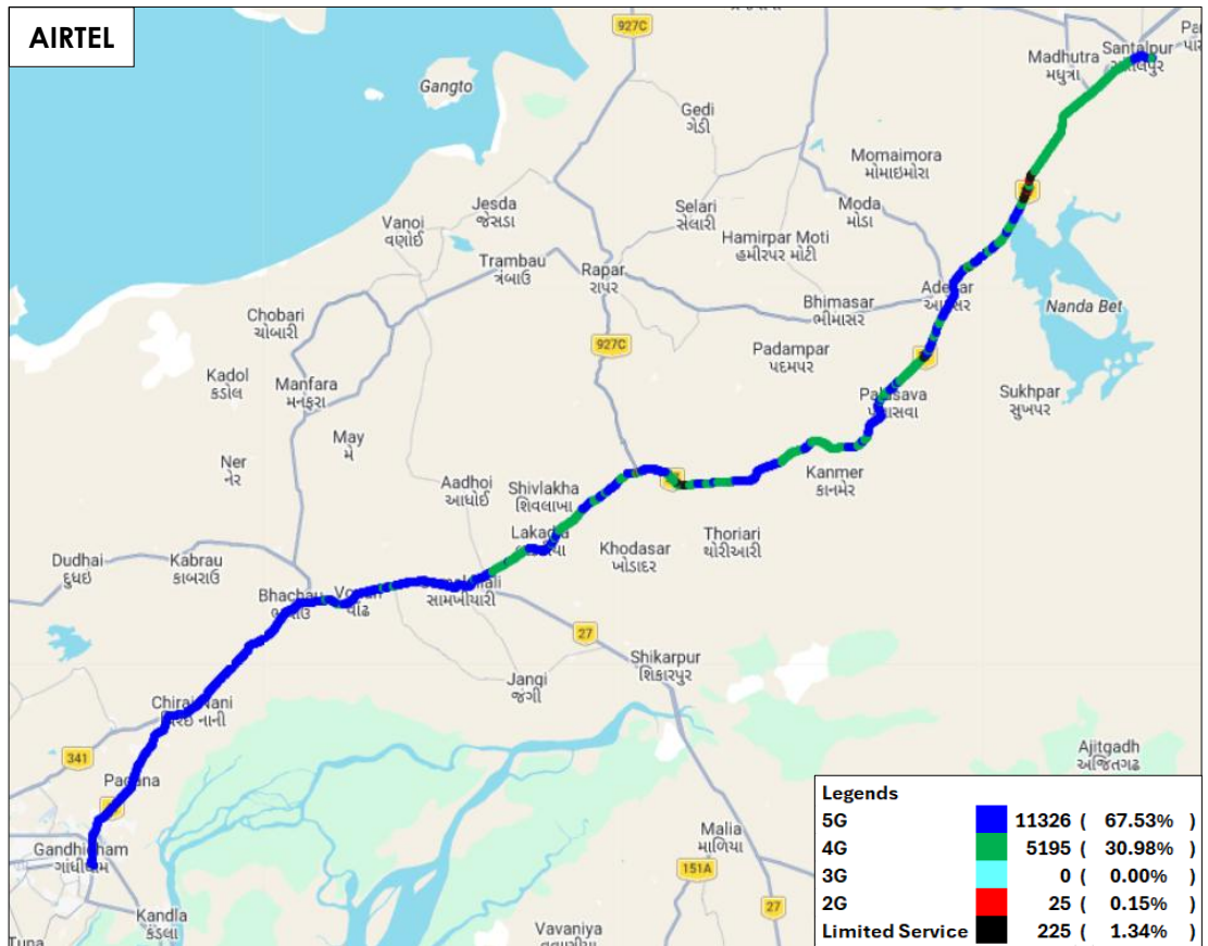
Figure-40: Serving technology plot in auto-selection mode (5G/4G/3G/2G) data - AIRTEL.
