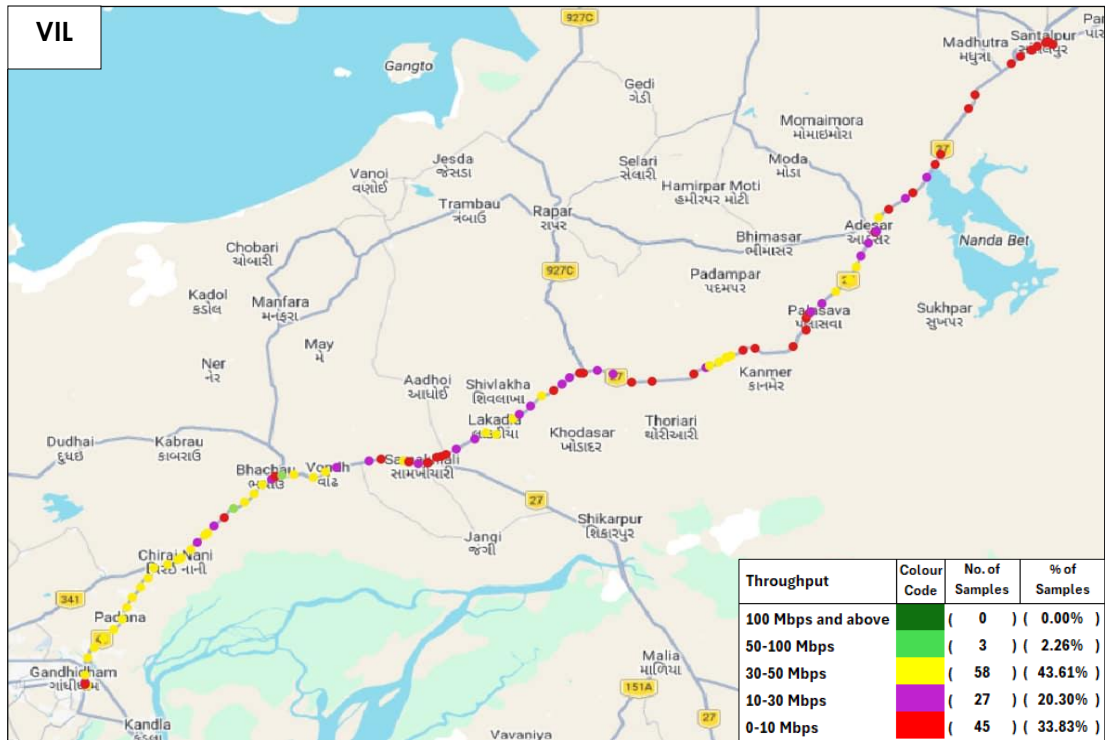
Figure-35: Download throughput distribution auto-selection mode (5G/4G/3G/2G) - VIL.
