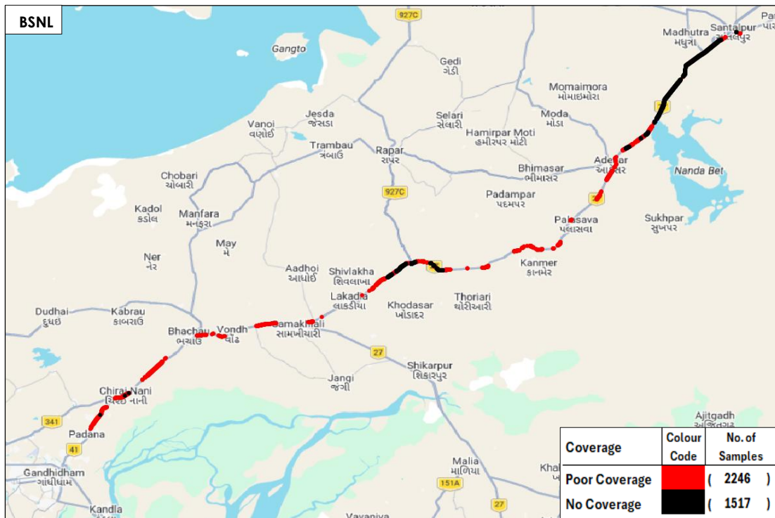
Figure-28: Poor coverage & no coverage locations in auto-selection mode (5G/4G/3G/2G) voice-BSNL.
