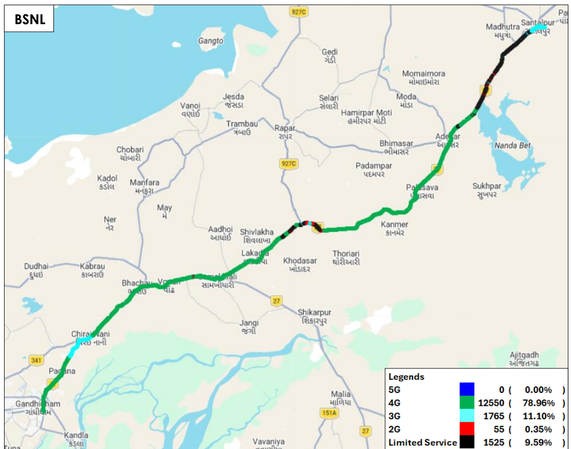
Figure-41: Serving technology plot in auto-selection mode (5G/4G/3G/2G) data - BSNL.
