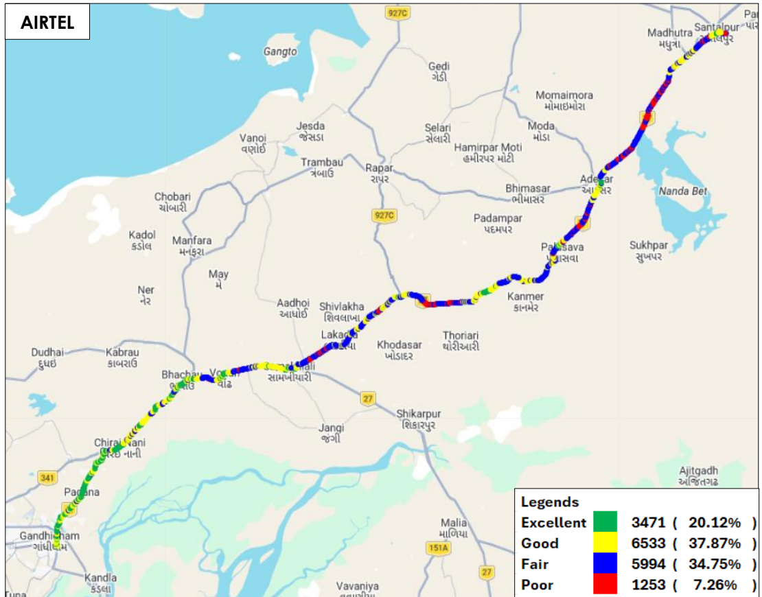
Figure-48: Signal strength auto-selection mode (5G/4G/3G/2G) voice - AIRTEL.
