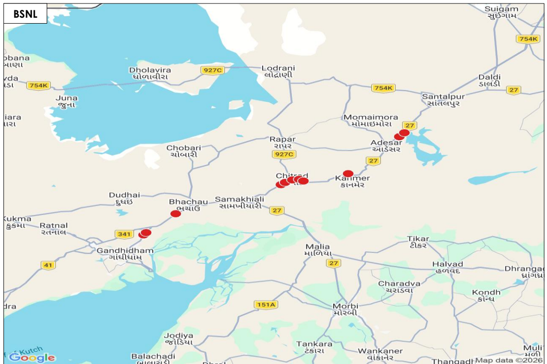
Figure-15: Drop call locations in auto-selection mode (5G/4G/3G/2G) voice - BSNL.
