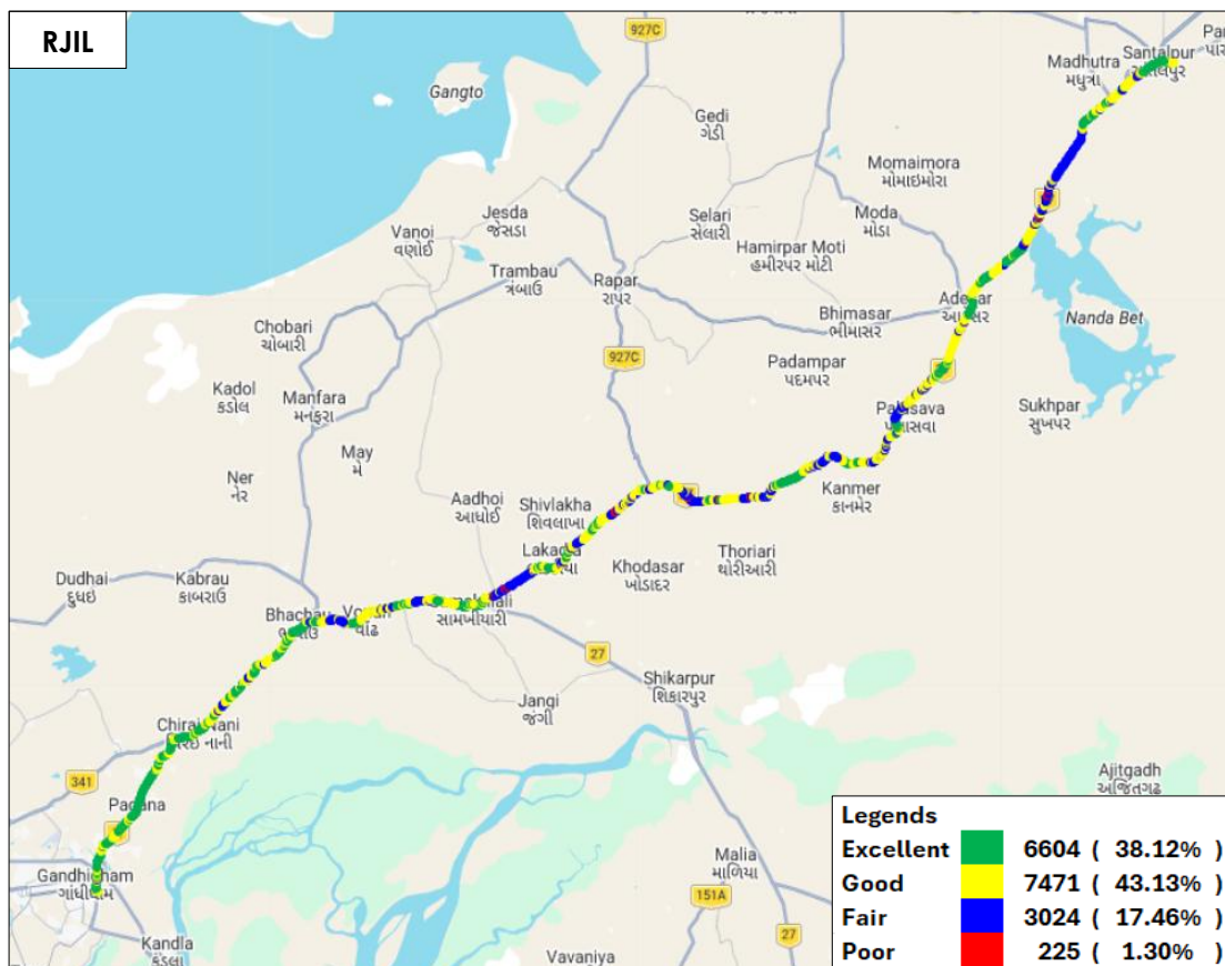
Figure-50: Signal strength auto-selection mode (5G/4G/3G/2G) voice - RJIL.
