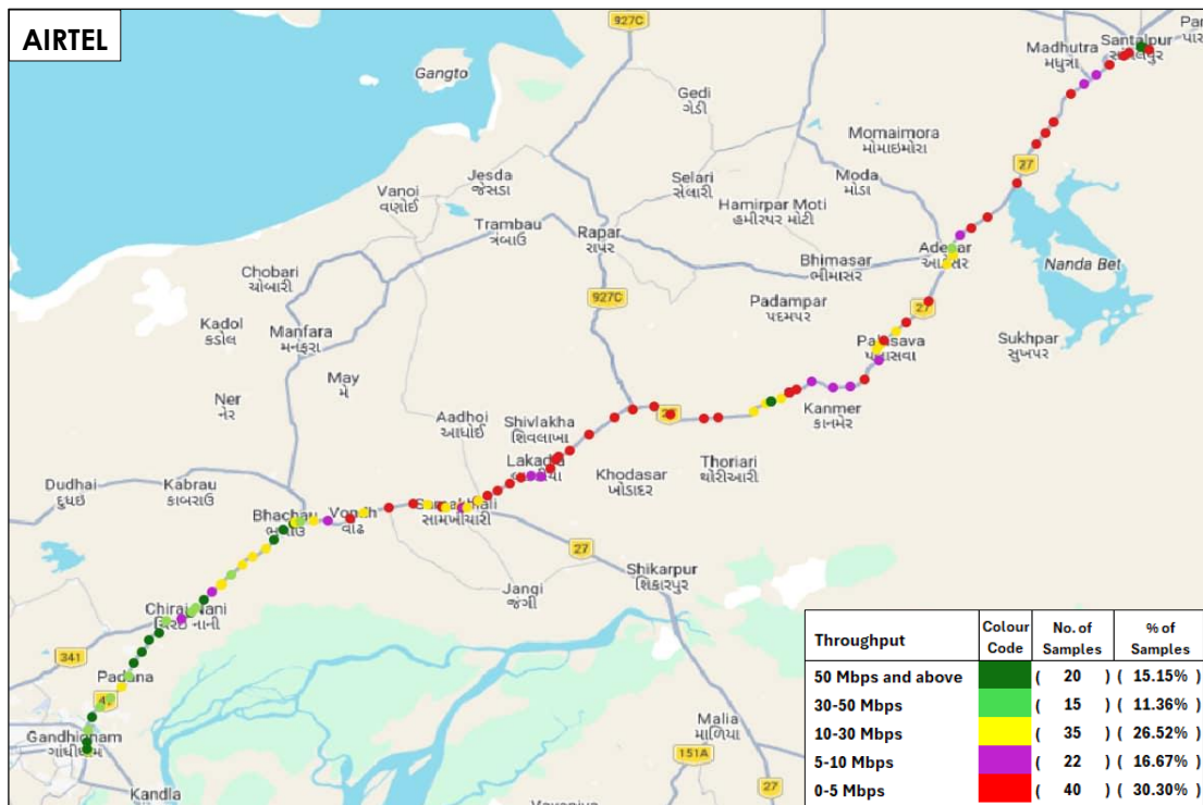
Figure-36: Upload throughput distribution auto-selection mode (5G/4G/3G/2G) - AIRTEL.
