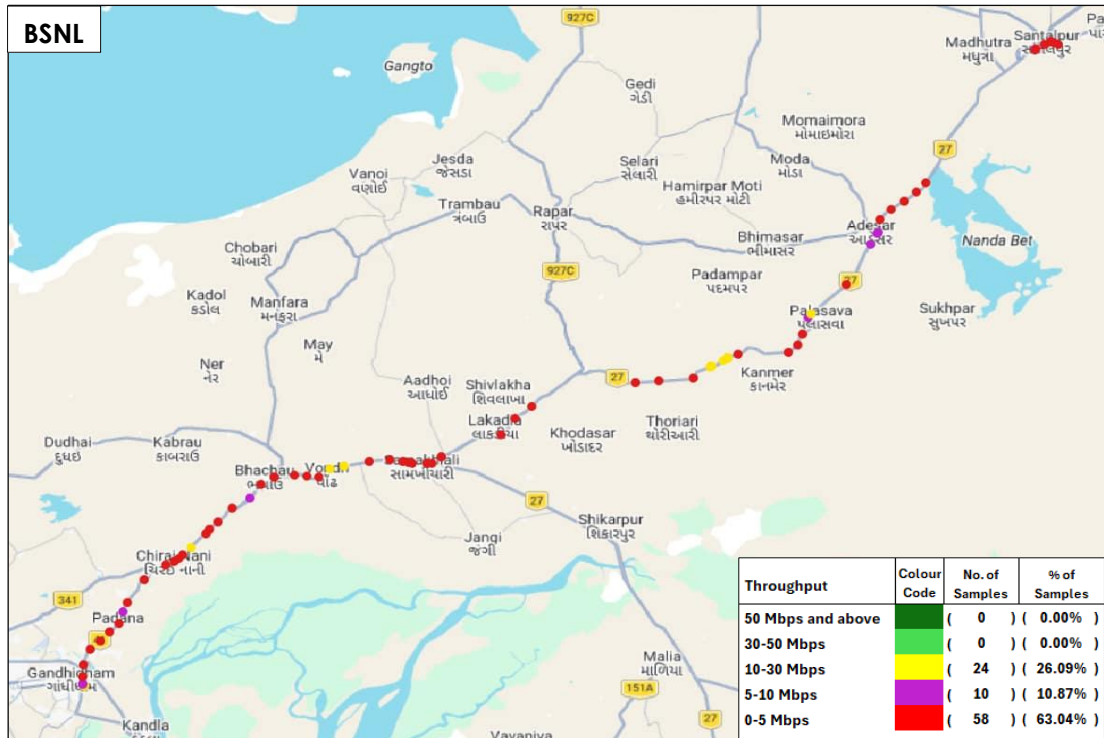
Figure-37: Upload throughput distribution auto-selection mode (5G/4G/3G/2G) - BSNL.
