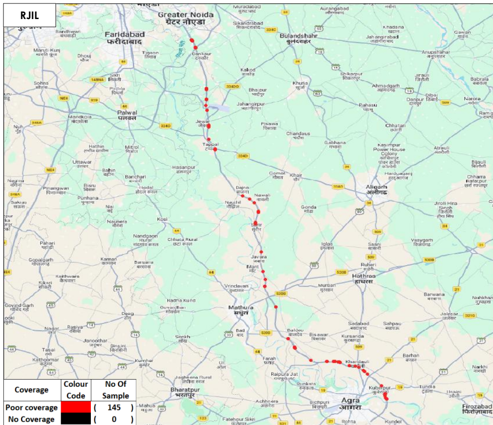
Figure-30: Poor coverage & no coverage locations in auto-selection mode (5G/4G/3G/2G) voice-RJIL.
