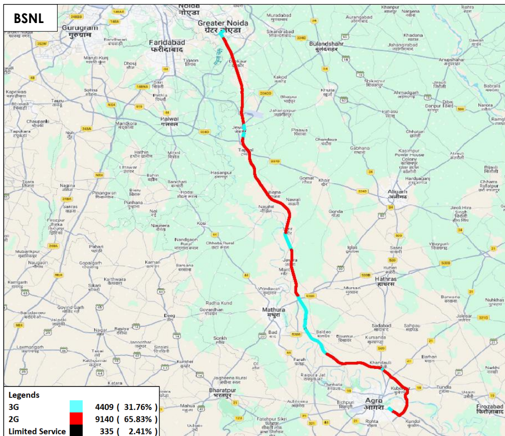
Figure-11: Serving technology plots 3G/2G network mode - BSNL.
