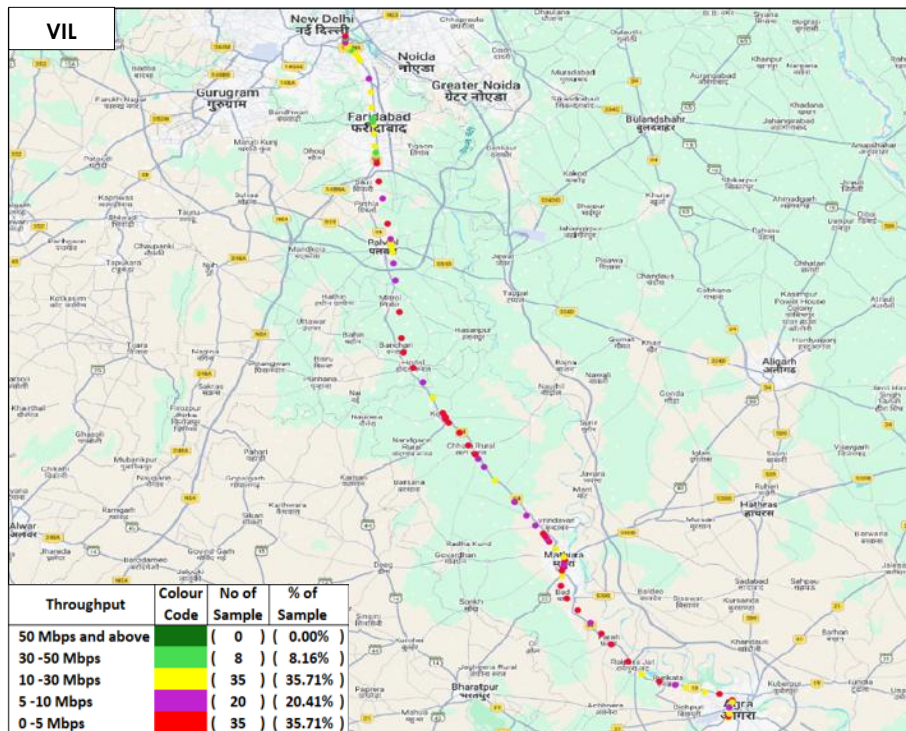
Figure-69: Upload throughput distribution auto-selection mode (5G/4G/3G/2G) - VIL.
