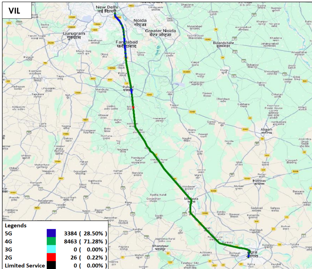
Figure-73: Serving technology plot in auto-selection mode (5G/4G/3G/2G) data - VIL.
