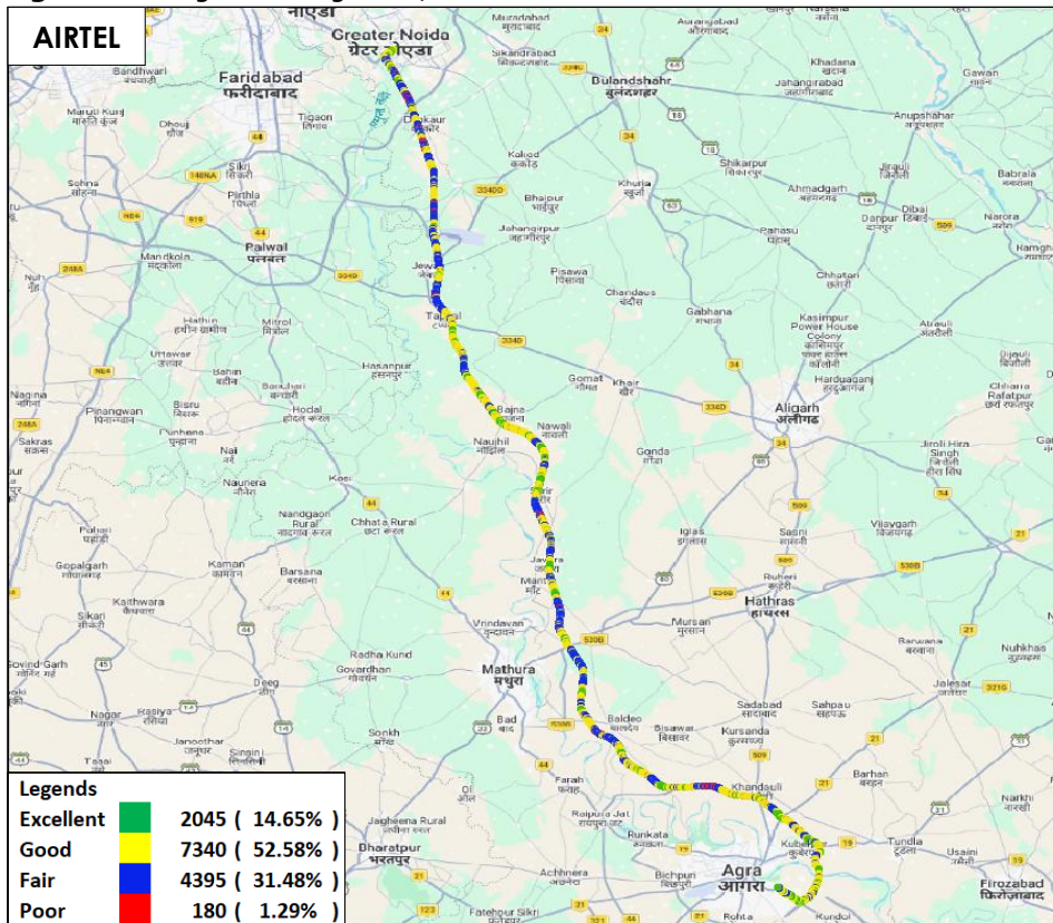
Figure-78: Signal strength auto-selection mode (5G/4G/3G/2G) voice - AIRTEL.
