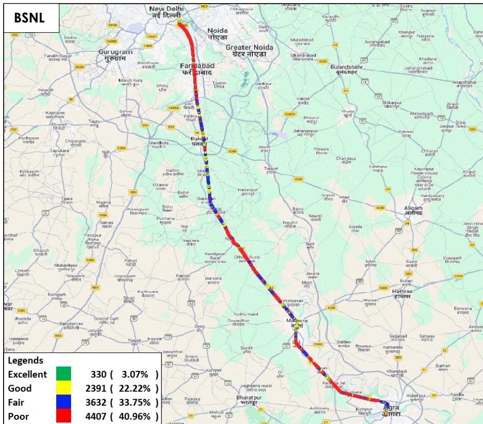
Figure-91: Signal strength auto-selection mode (5G/4G/3G/2G) data - BSNL.
