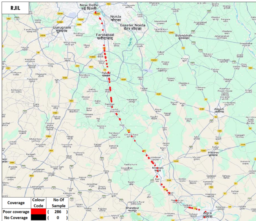
Figure-59: Poor coverage & no coverage locations in auto-selection mode (5G/4G/3G/2G) voice-RJIL.
