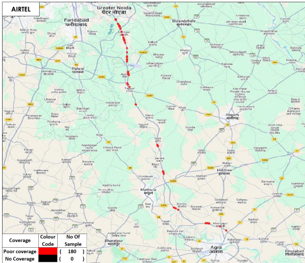
Figure-28: Poor coverage & no coverage locations in auto-selection mode (5G/4G/3G/2G) voice-Airtel.
