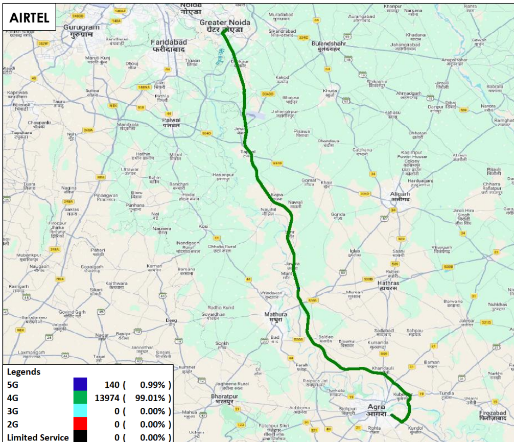
Figure-23: Serving technology plots in auto-selection mode (5G/4G/3G/2G) voice - AIRTEL.
