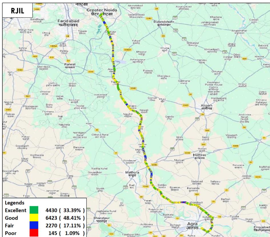
Figure-80: Signal strength auto-selection mode (5G/4G/3G/2G) voice - RJIL.
