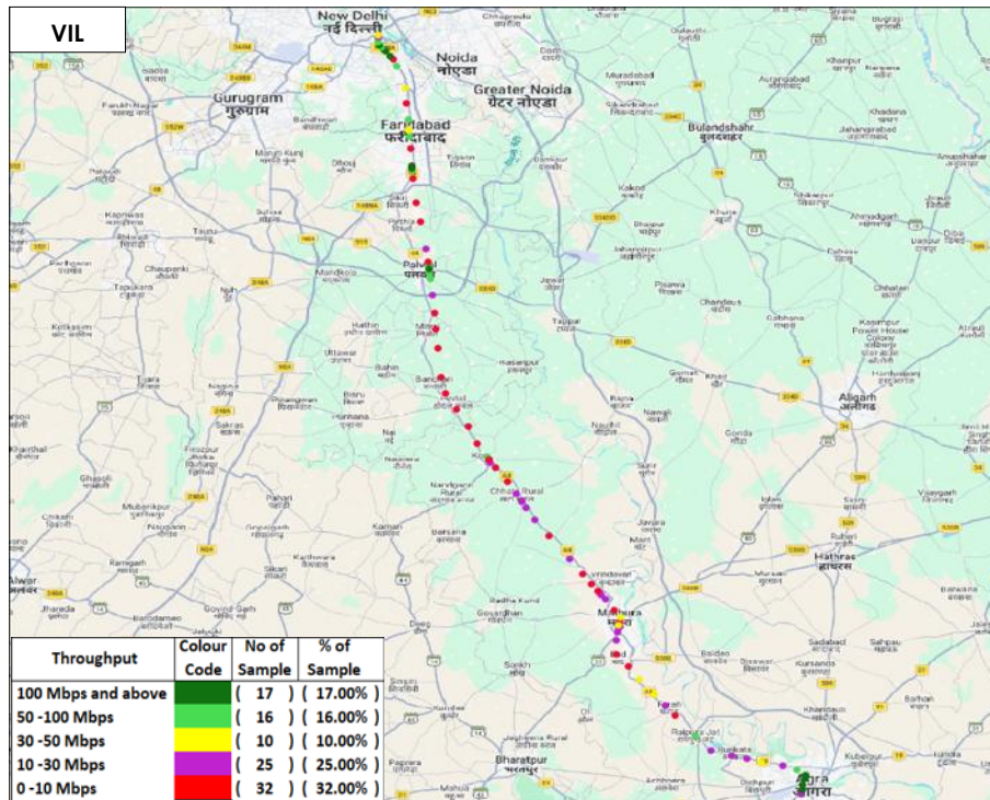
Figure-65: Download throughput distribution auto-selection mode (5G/4G/3G/2G) - VIL.
