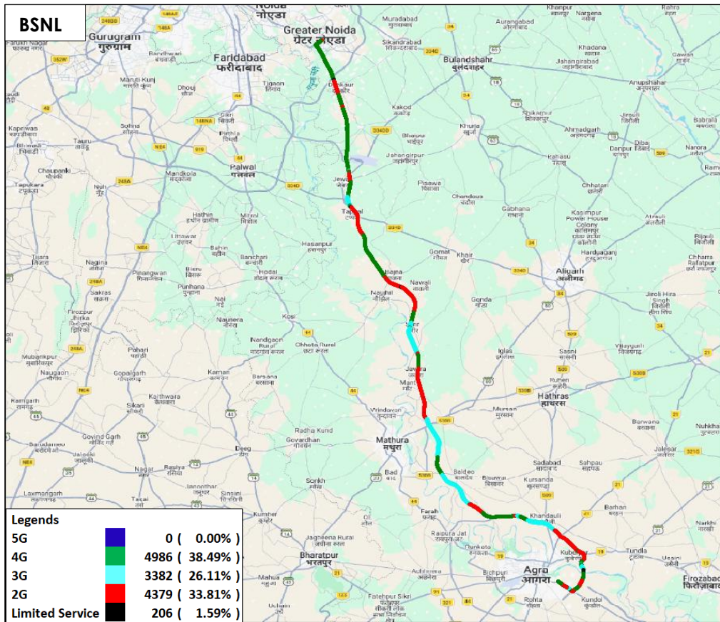
Figure-24: Serving technology plots in auto-selection mode (5G/4G/3G/2G) voice - BSNL.
