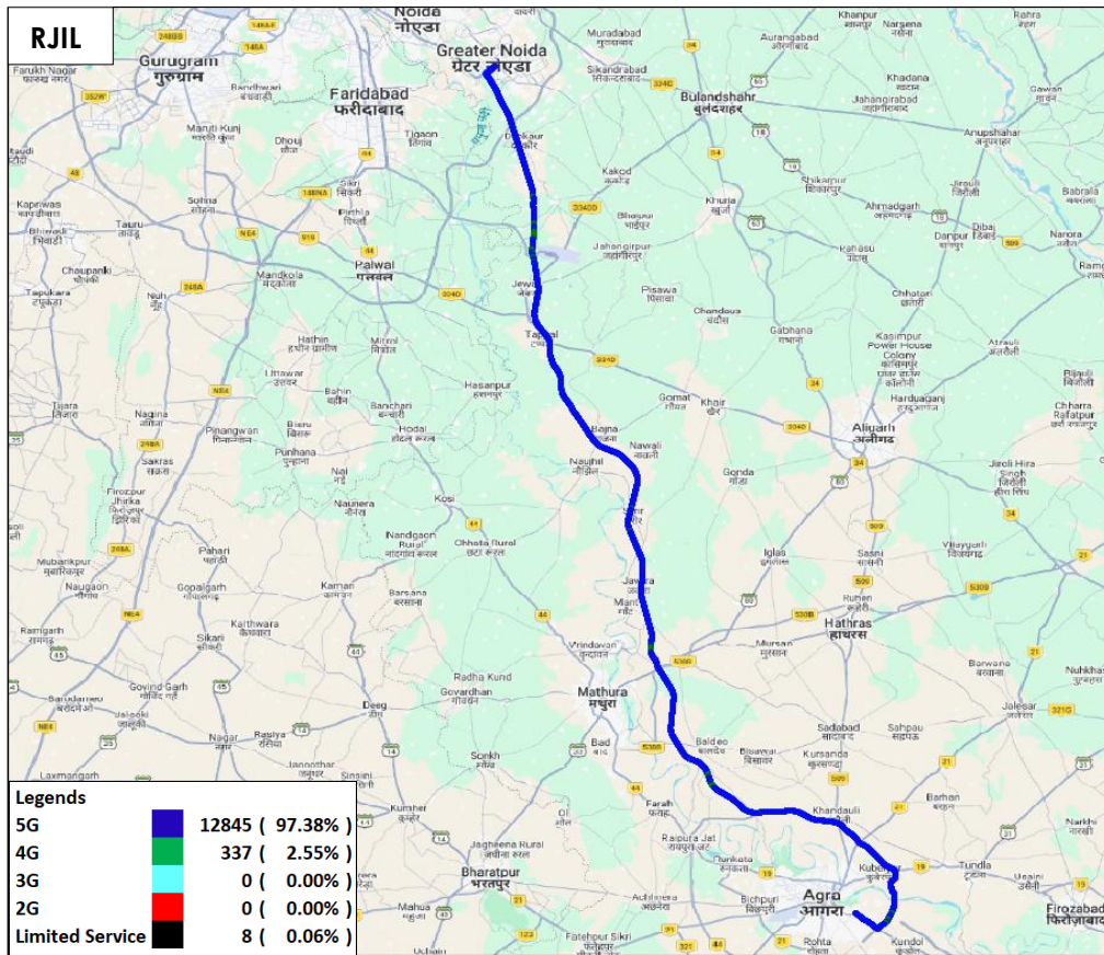
Figure-43: Serving technology plot in auto-selection mode (5G/4G/3G/2G) data - RJIL.
