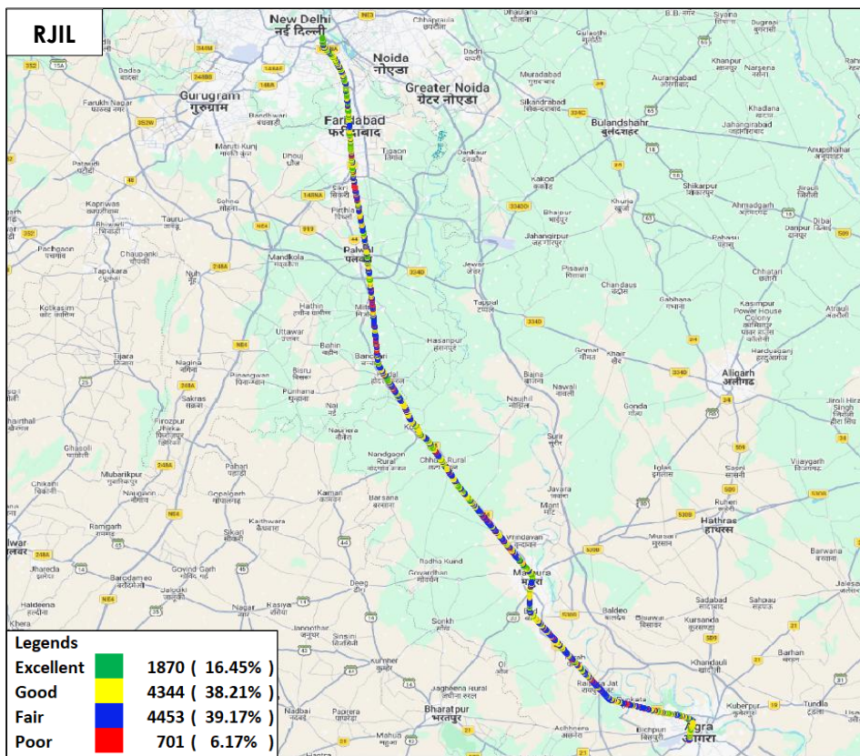
Figure-92: Signal strength auto-selection mode (5G/4G/3G/2G) data - RJIL.
