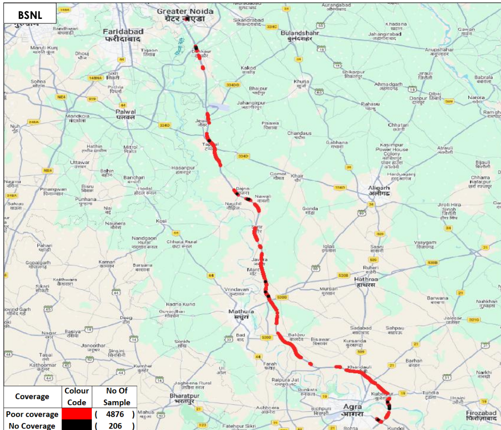
Figure-29: Poor coverage & no coverage locations in auto-selection mode (5G/4G/3G/2G) voice-BSNL.
