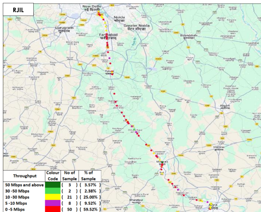
Figure-68: Upload throughput distribution auto-selection mode (5G/4G/3G/2G) - RJIL.
