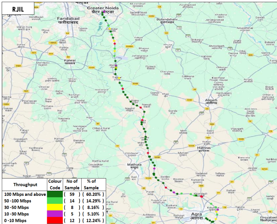
Figure-35: Download throughput distribution auto-selection mode (5G/4G/3G/2G) - RJIL.
