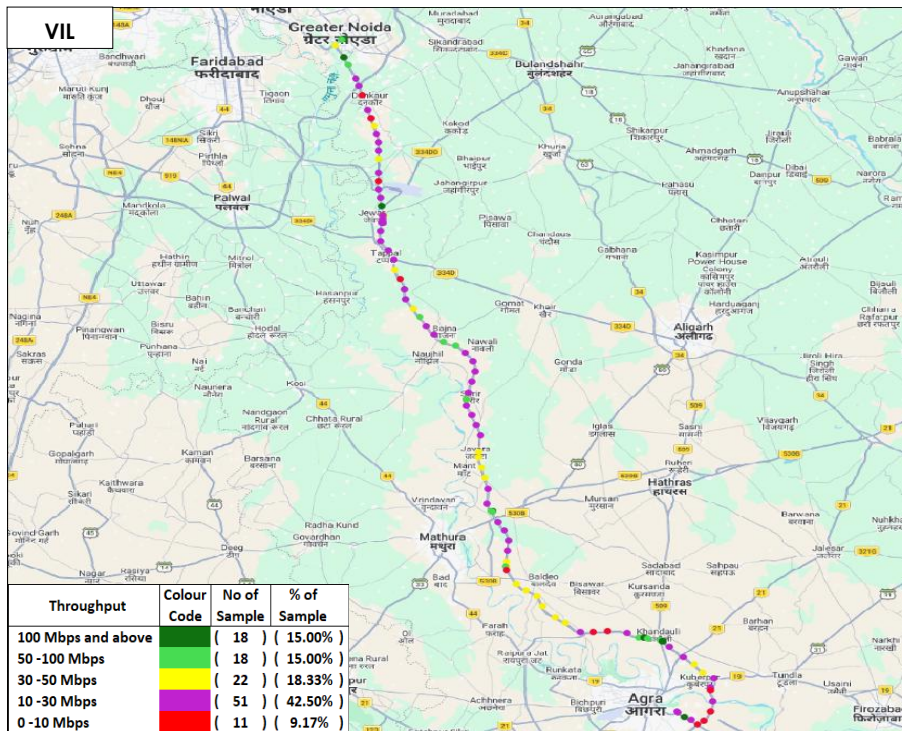
Figure-36: Download throughput distribution auto-selection mode (5G/4G/3G/2G) - VIL.
