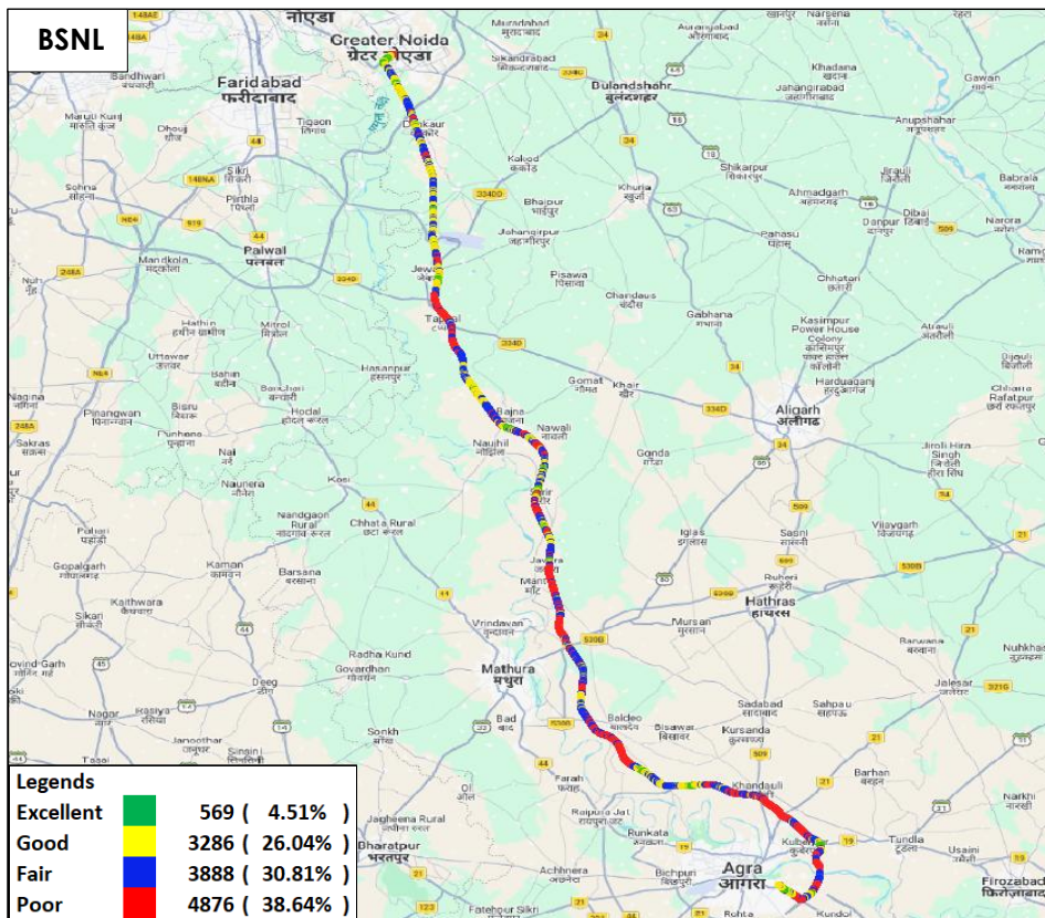
Figure-79: Signal strength auto-selection mode (5G/4G/3G/2G) voice - BSNL.
