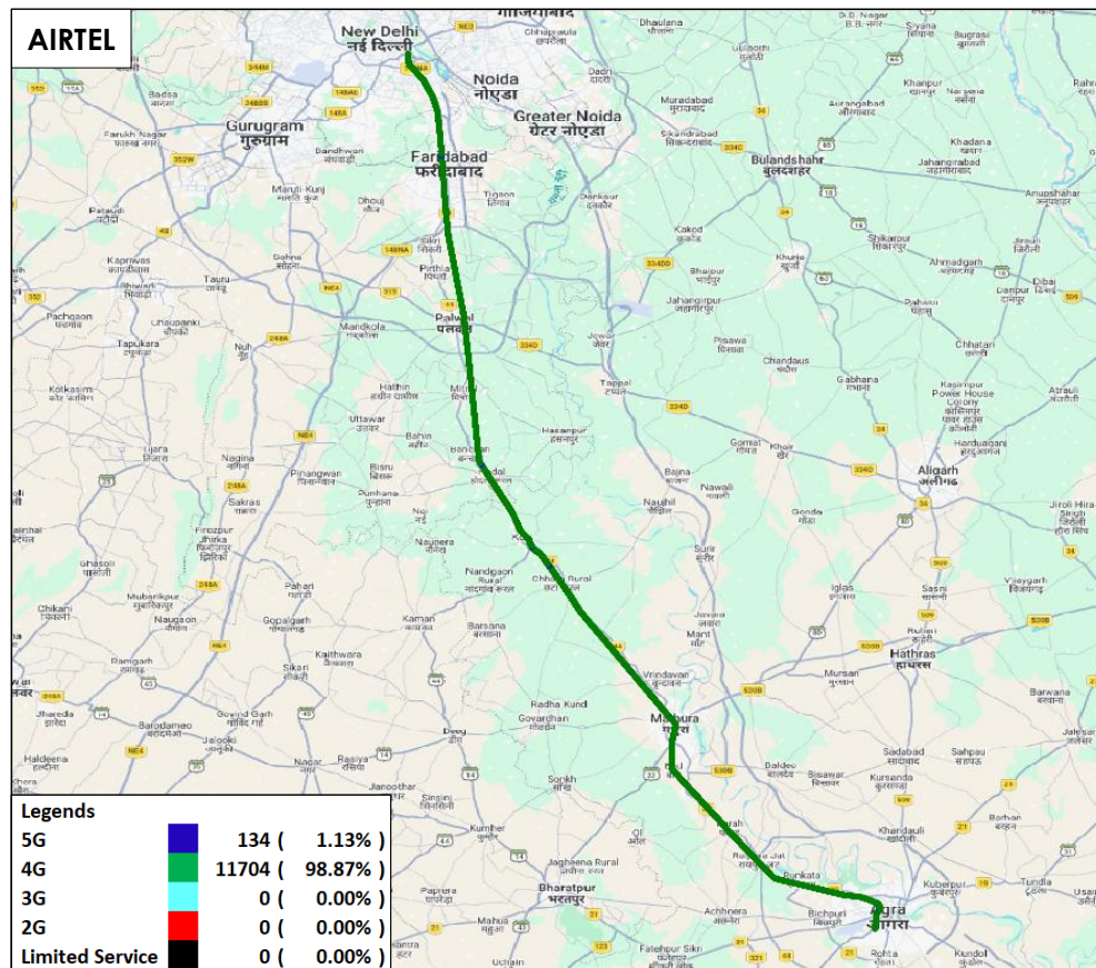
Figure-52: Serving technology plots in auto-selection mode (5G/4G/3G/2G) voice - AIRTEL.
