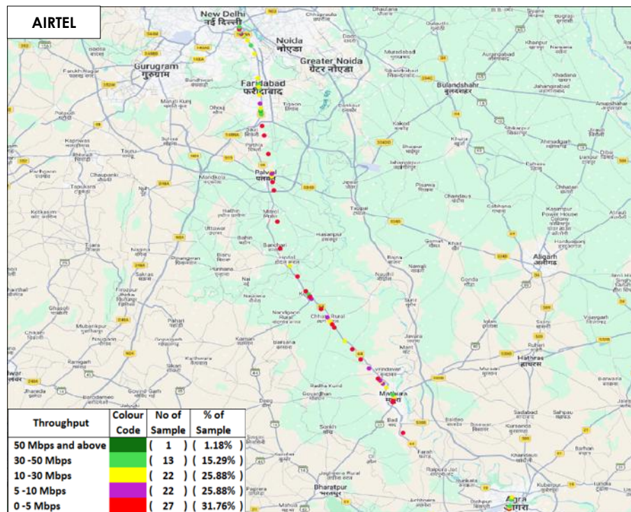
Figure-66: Upload throughput distribution auto-selection mode (5G/4G/3G/2G) - AIRTEL.
