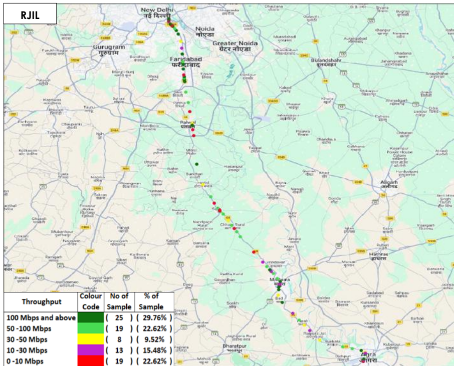
Figure-64: Download throughput distribution auto-selection mode (5G/4G/3G/2G) - RJIL.
