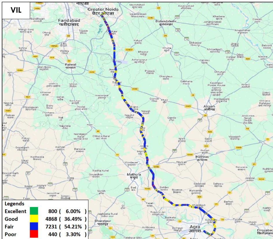
Figure-85: Signal strength auto-selection mode (5G/4G/3G/2G) data - VIL.
