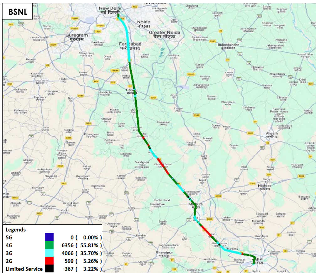
Figure-71: Serving technology plot in auto-selection mode (5G/4G/3G/2G) data - BSNL.
