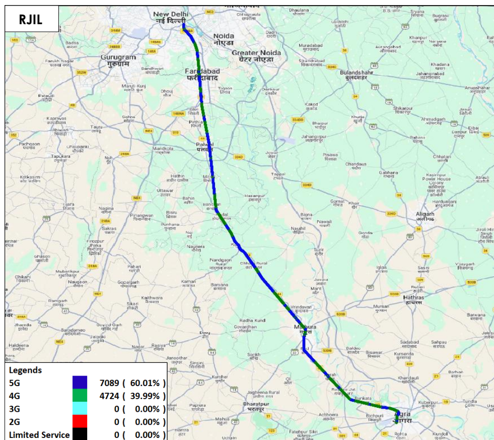
Figure-54: Serving technology plots in auto-selection mode (5G/4G/3G/2G) voice - RJIL.
