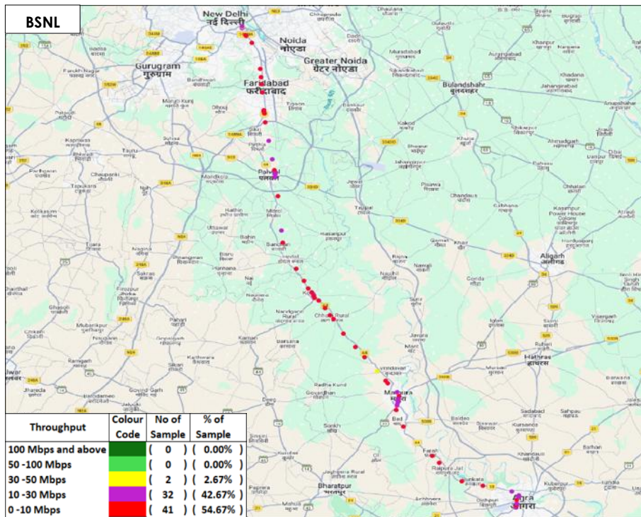
Figure-63: Download throughput distribution auto-selection mode (5G/4G/3G/2G) - BSNL.
