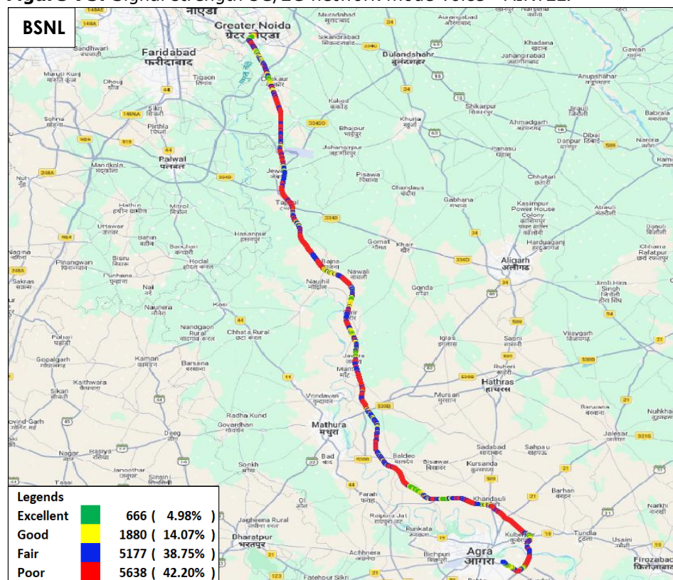
Figure-76: Signal strength 3G/2G network mode voice - BSNL.
