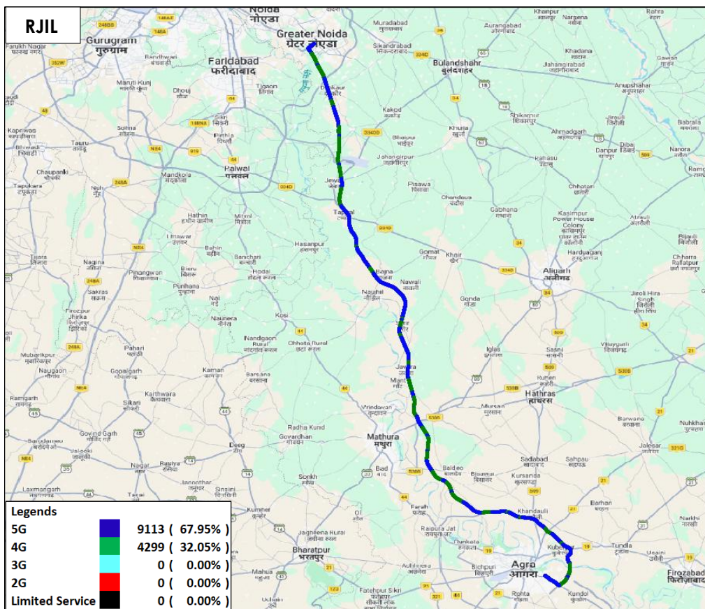
Figure-25: Serving technology plots in auto-selection mode (5G/4G/3G/2G) voice - RJIL.
