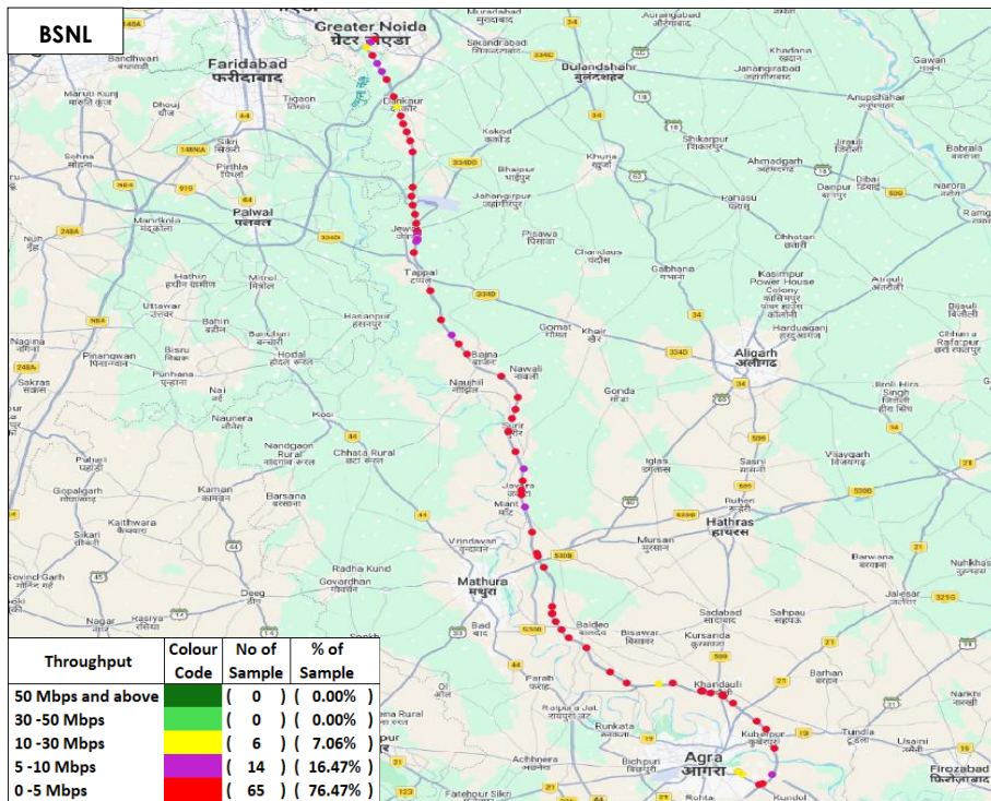
Figure-38: Upload throughput distribution auto-selection mode (5G/4G/3G/2G) - BSNL.
