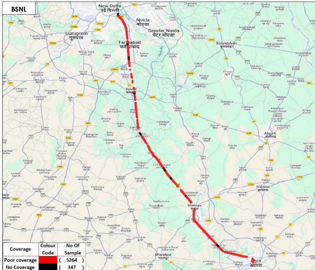
Figure-58: Poor coverage & no coverage locations in auto-selection mode (5G/4G/3G/2G) voice-BSNL.
