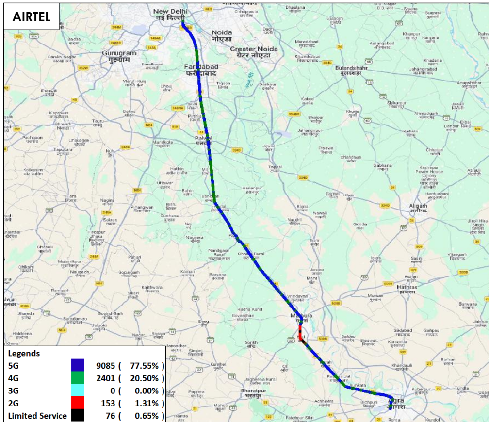
Figure-70: Serving technology plot in auto-selection mode (5G/4G/3G/2G) data - AIRTEL.
