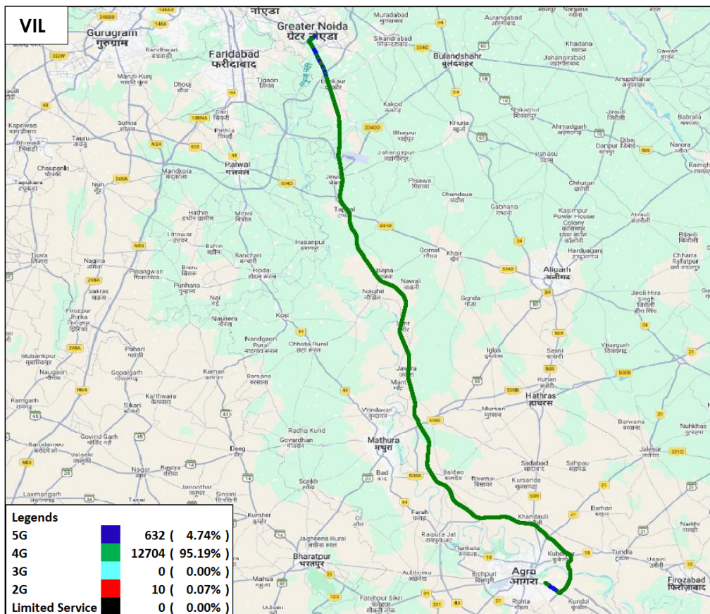
Figure-44: Serving technology plot in auto-selection mode (5G/4G/3G/2G) data - VIL.
