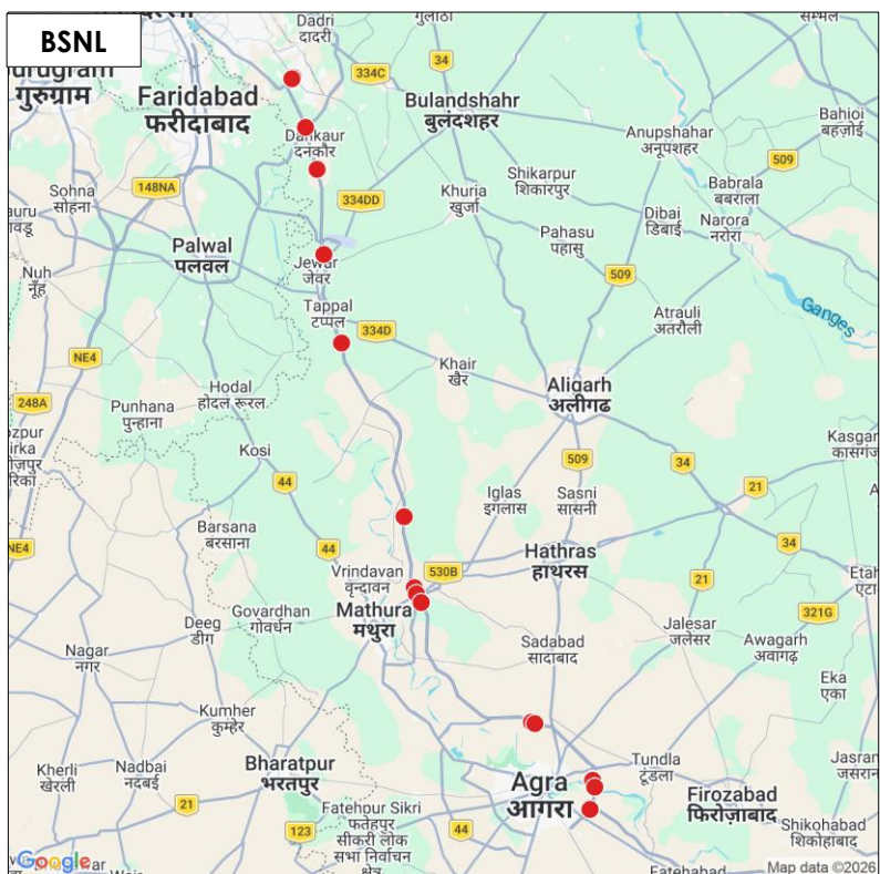
Figure-17: Drop call locations in auto-selection mode (5G/4G/3G/2G) voice - BSNL
