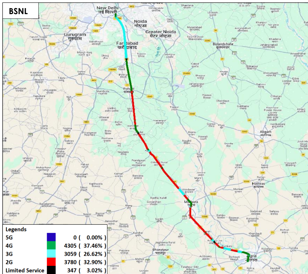
Figure-53: Serving technology plots in auto-selection mode (5G/4G/3G/2G) voice - BSNL.
