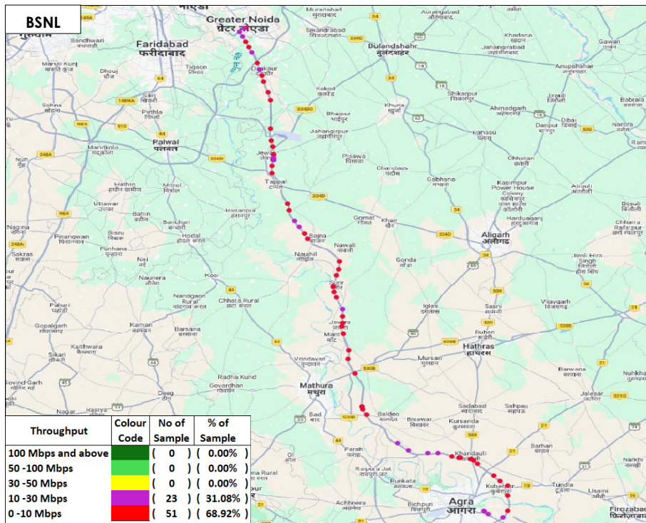
Figure-34: Download throughput distribution auto-selection mode (5G/4G/3G/2G) - BSNL.
