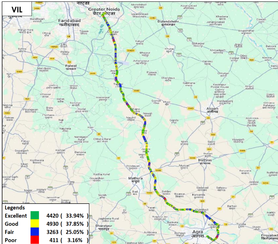
Figure-77: Signal strength 3G/2G network mode voice - VIL.
