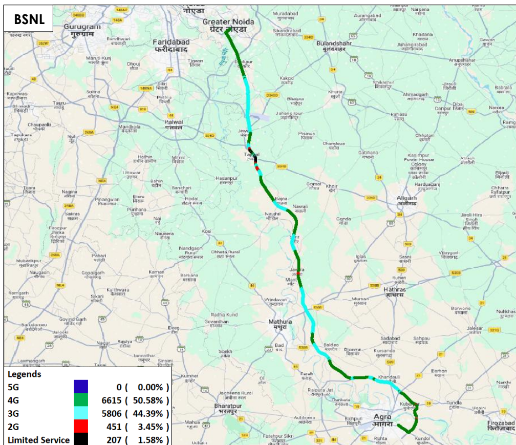
Figure-42: Serving technology plot in auto-selection mode (5G/4G/3G/2G) data - BSNL.
