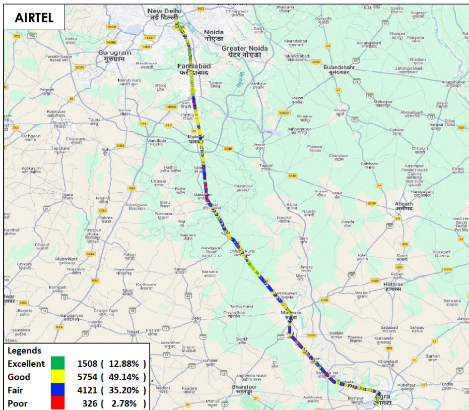
Figure-86: Signal strength auto-selection mode (5G/4G/3G/2G) voice - AIRTEL.
