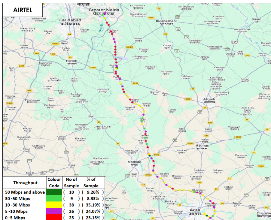
Figure-37: Upload throughput distribution auto-selection mode (5G/4G/3G/2G) - AIRTEL.
