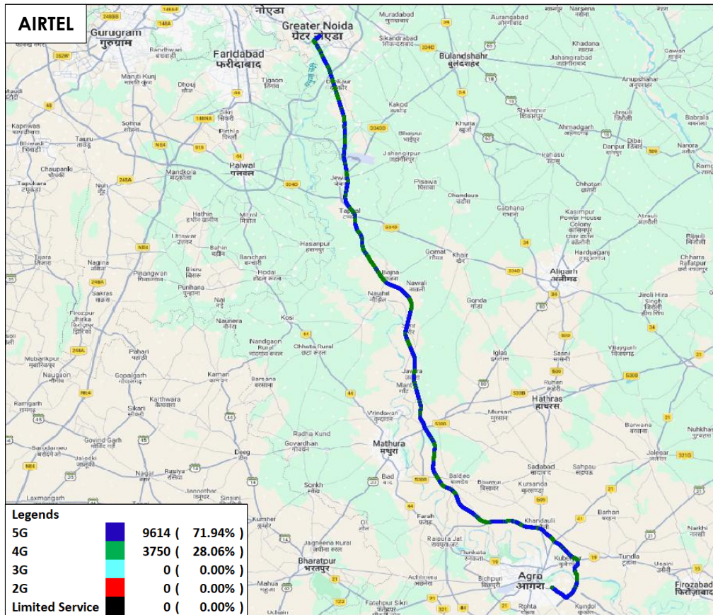
Figure-41: Serving technology plot in auto-selection mode (5G/4G/3G/2G) data - AIRTEL.
