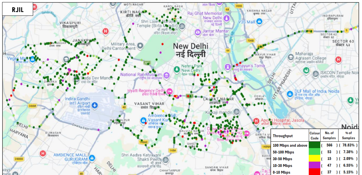
Figure-35: Download throughput distribution auto-selection mode (5G/4G/3G/2G) - RJIL
