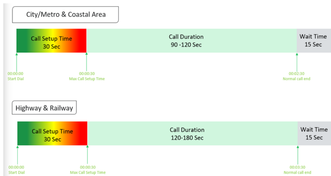
Figure-61: Voice test script for city/railway/metro/Airport route & coastal area
