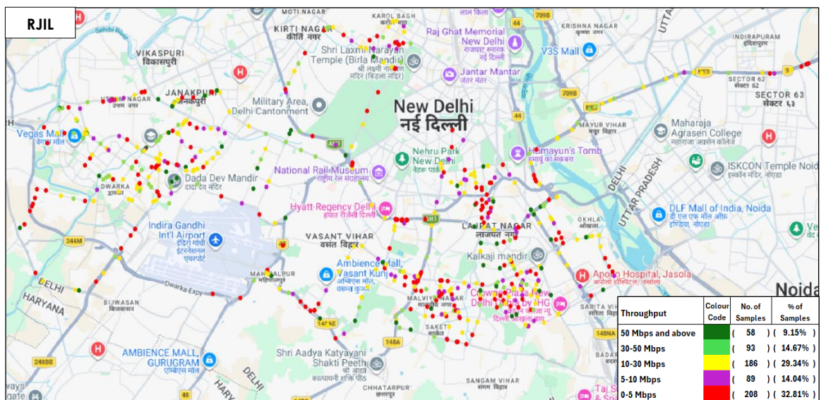
Figure-39: Upload throughput distribution auto-selection mode (5G/4G/3G/2G) - RJIL.
