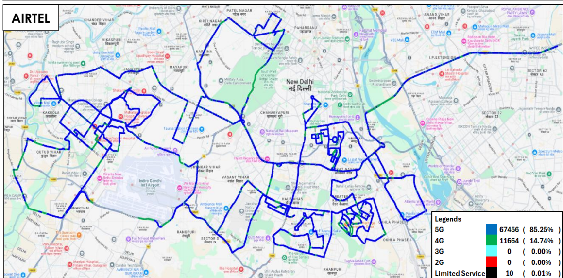
Figure-41: Serving technology plots in auto-selection mode (5G/4G/3G/2G) data - AIRTEL.
