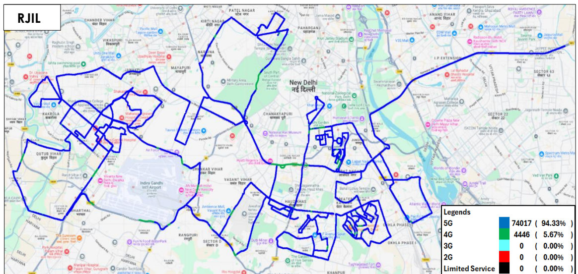
Figure-43: Serving technology plots in auto-selection mode (5G/4G/3G/2G) data - RJIL.
