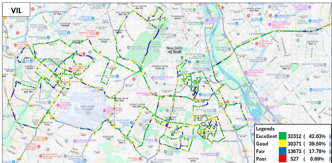
Figure-54: Signal strength auto-selection mode (5G/4G/3G/2G) voice - VIL.
