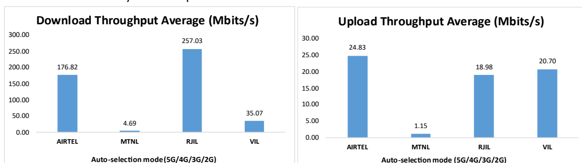
Figure- 32: Download & Upload throughput.
