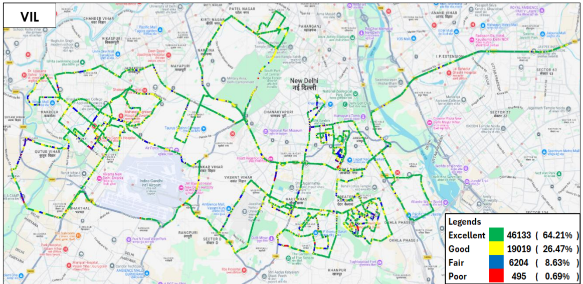
Figure-50: Signal strength 3G/2G network mode voice - VIL.
