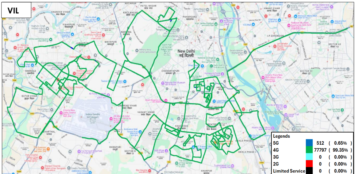
Figure-26: Serving technology plots in auto-selection mode (5G/4G/3G/2G) voice - VIL.
