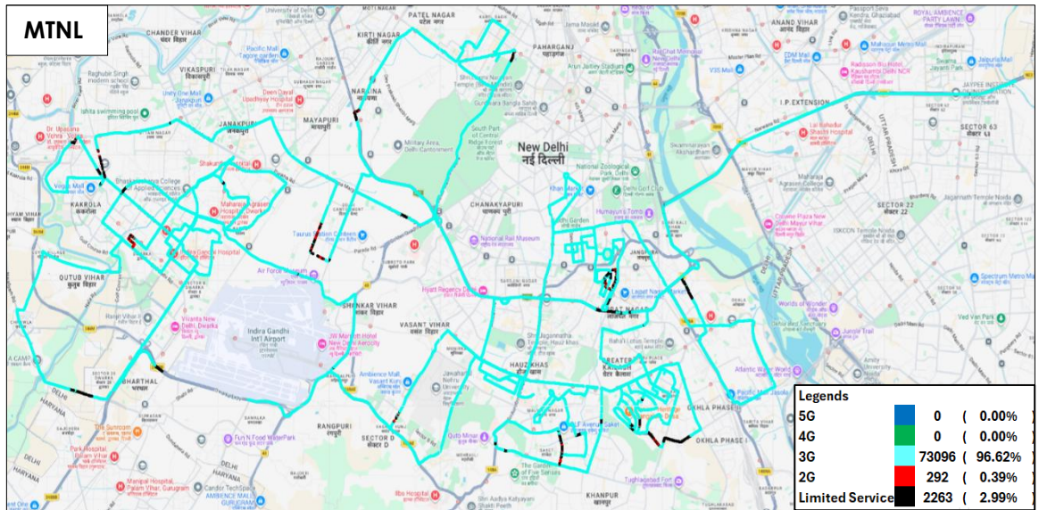
Figure-42: Serving technology plots in auto-selection mode (5G/4G/3G/2G) data - MTNL.
