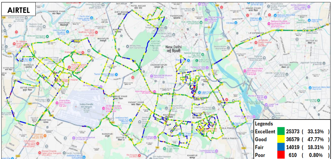
Figure-51: Signal strength auto-selection mode (5G/4G/3G/2G) voice - AIRTEL.
