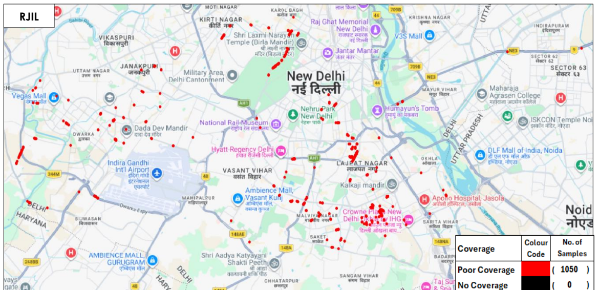
Figure-30: Poor coverage & no coverage locations in auto-selection mode (5G/4G/3G/2G) voice- RJIL.
