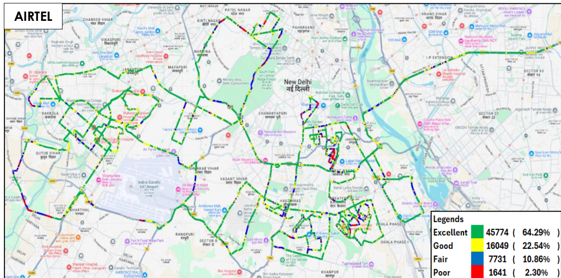
Figure-48: Signal strength 3G/2G network mode voice - AIRTEL.
