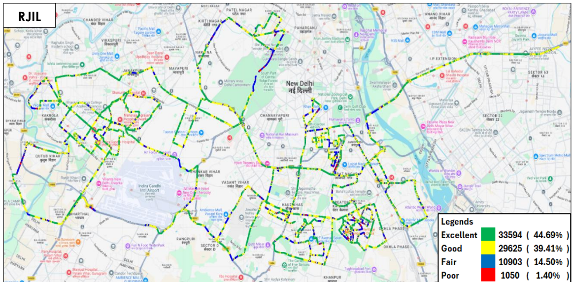
Figure-53: Signal strength auto-selection mode (5G/4G/3G/2G) voice - RJIL.
