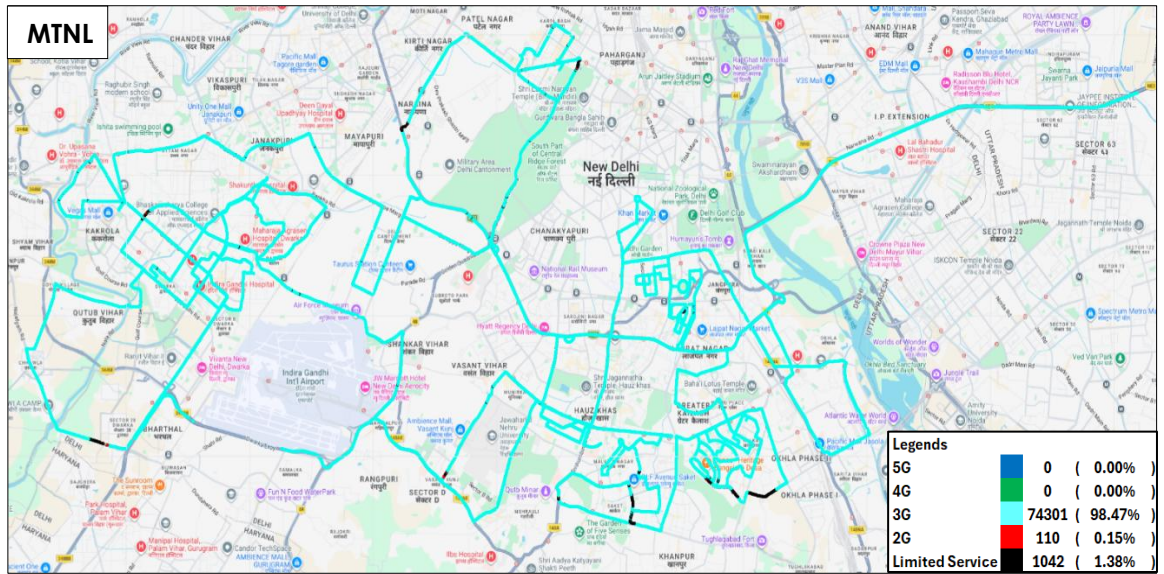
Figure-24: Serving technology plots in auto-selection mode (5G/4G/3G/2G) voice - MTNL.
