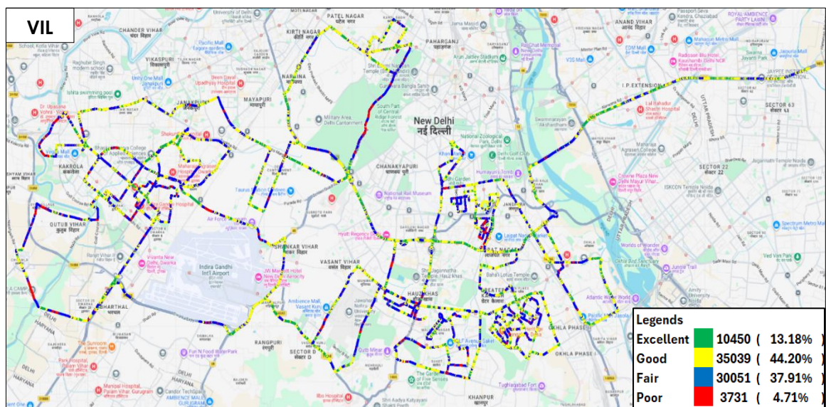
Figure-58: Signal strength auto-selection mode (5G/4G/3G/2G) data - VIL.
