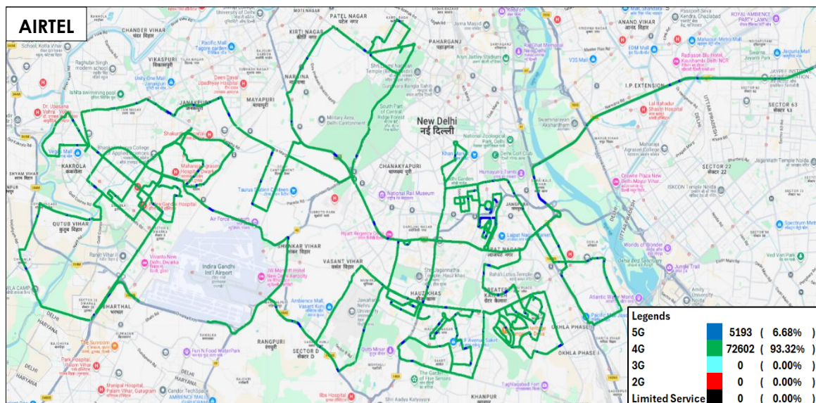
Figure-23: Serving technology plots in auto-selection mode (5G/4G/3G/2G) voice - AIRTEL.
