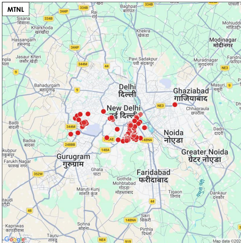
Figure-16: Drop call locations in auto-selection mode (5G/4G/3G/2G) voice - MTNL.
