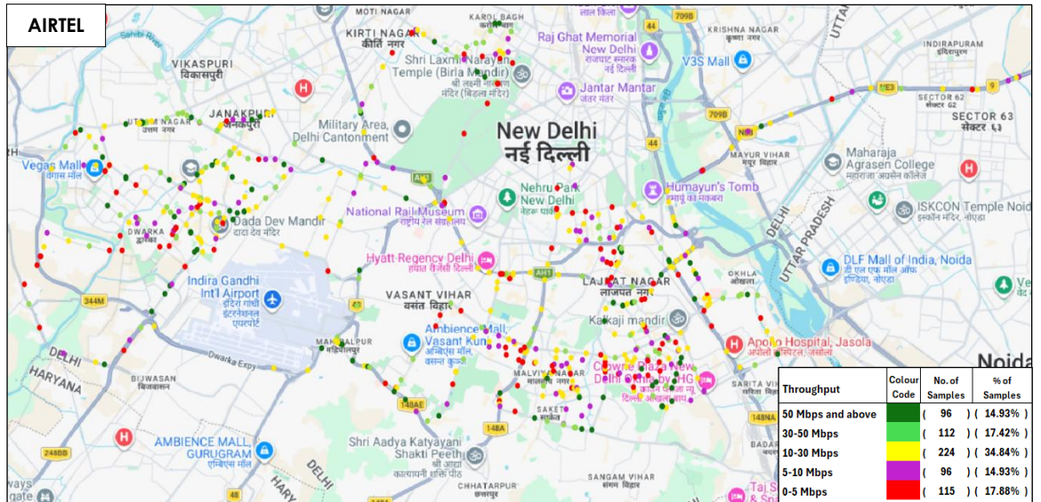
Figure-37: Upload throughput distribution auto-selection mode (5G/4G/3G/2G) - AIRTEL.
