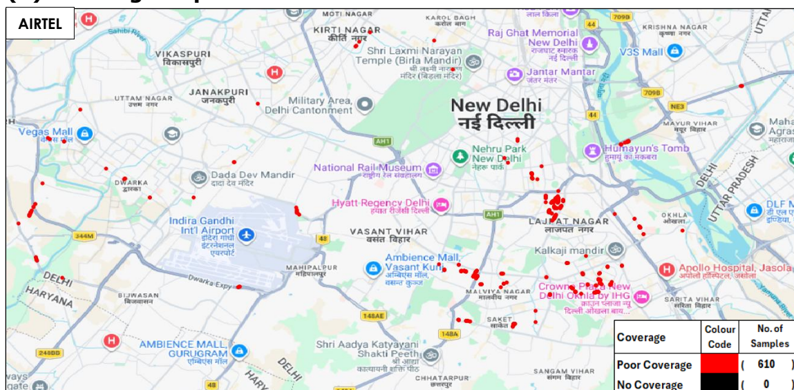
Figure-28: Poor coverage & no coverage locations in auto-selection mode (5G/4G/3G/2G) voice- Airtel.
