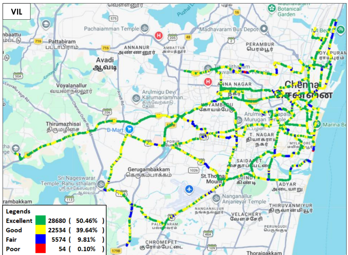
Figure-54: Signal strength auto-selection mode (5G/4G/3G/2G) voice - VIL.
