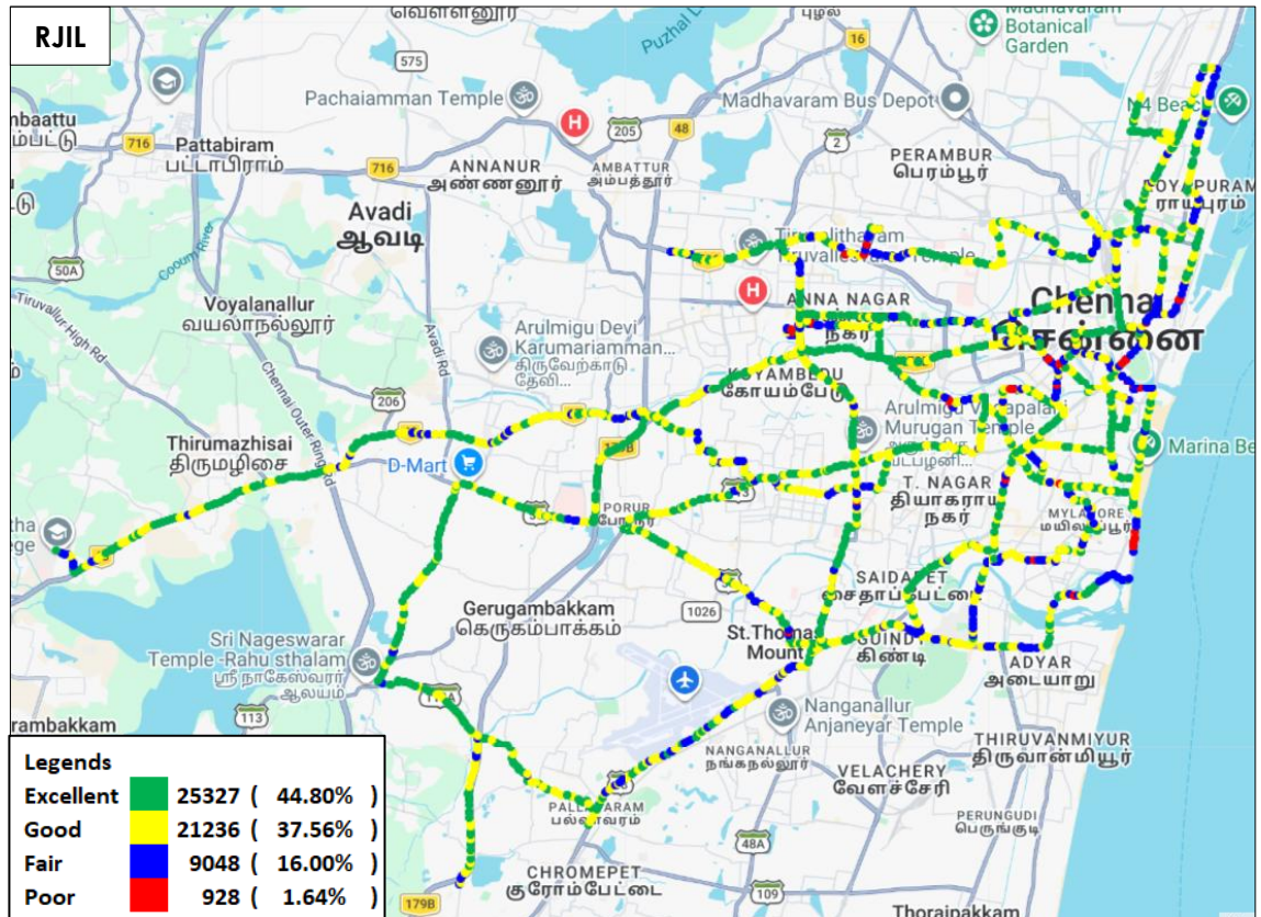
Figure-57: Signal strength auto-selection mode (5G/4G/3G/2G) data - RJIL.
