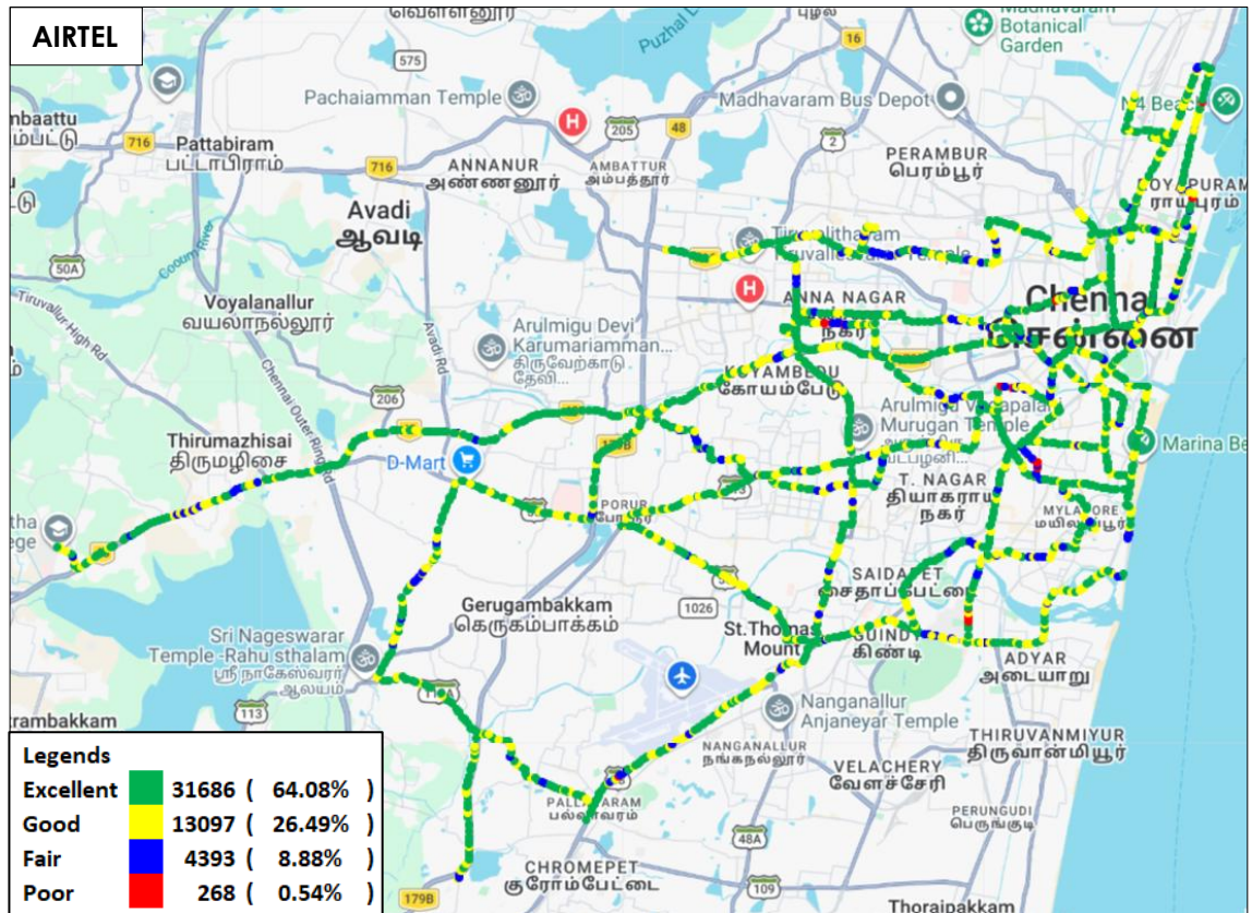
Figure-48: Signal strength 3G/2G network mode voice - AIRTEL.
