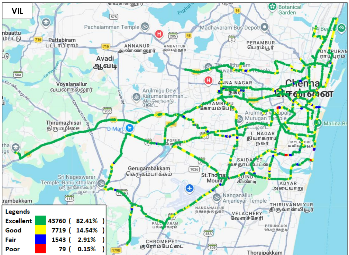
Figure-50: Signal strength 3G/2G network mode voice - VIL.
