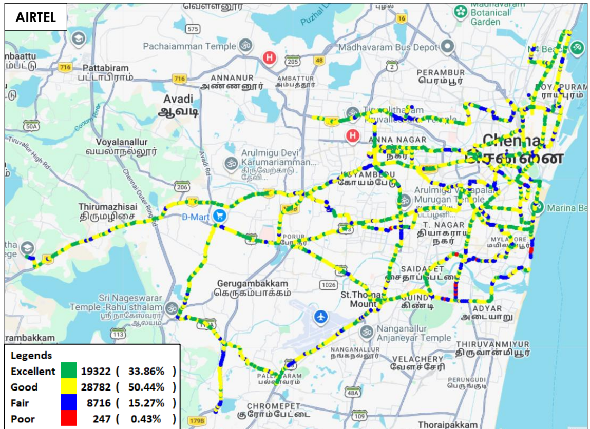
Figure-55: Signal strength auto-selection mode (5G/4G/3G/2G) data - AIRTEL.
