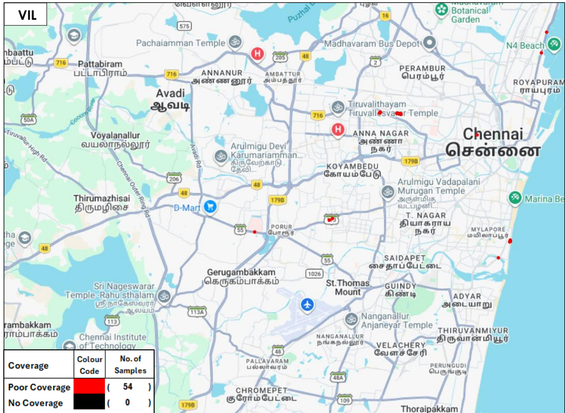
Figure-31: Poor coverage & no coverage locations in auto-selection mode (5G/4G/3G/2G) voice-VIL.
