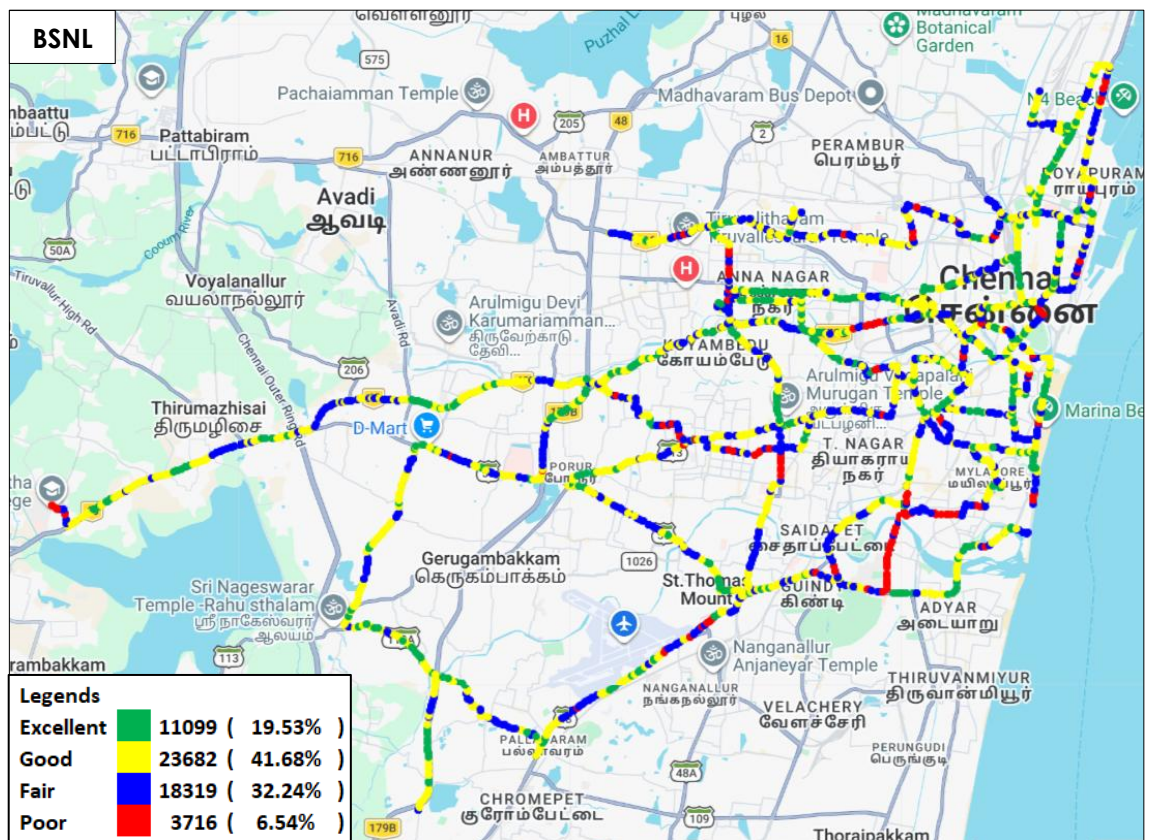
Figure-56: Signal strength auto-selection mode (5G/4G/3G/2G) data - BSNL.
