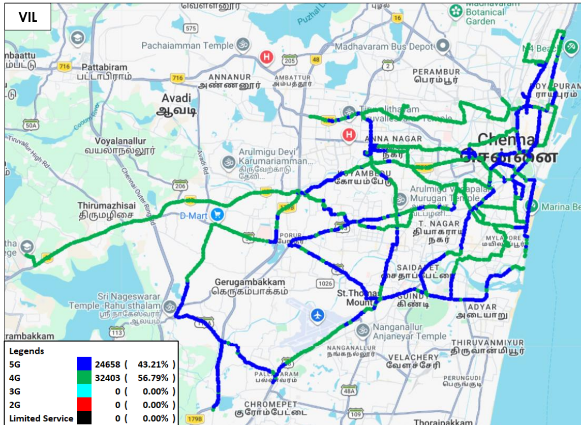
Figure-44: Serving technology plots in auto-selection mode (5G/4G/3G/2G) data- VIL.
