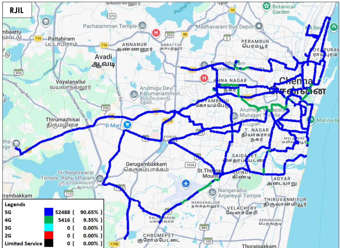
Figure-25: Serving technology plots in auto-selection mode (5G/4G/3G/2G) voice - RJIL.
