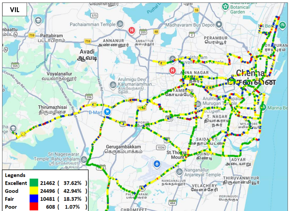
Figure-58: Signal strength auto-selection mode (5G/4G/3G/2G) data - VIL.
