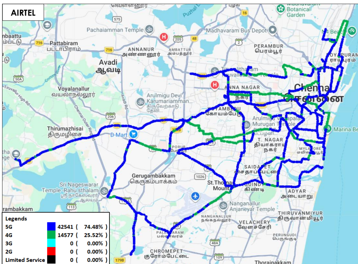
Figure-41: Serving technology plots in auto-selection mode (5G/4G/3G/2G) data -AIRTEL.
