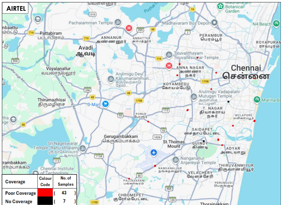
Figure-28: Poor coverage & no coverage locations in auto-selection mode (5G/4G/3G/2G) voice-Airtel.
