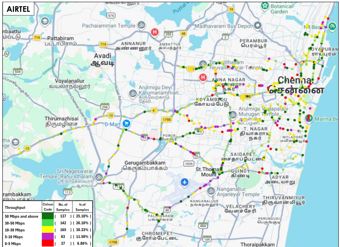
Figure-37: Upload throughput distribution auto-selection mode (5G/4G/3G/2G) – AIRTEL.
