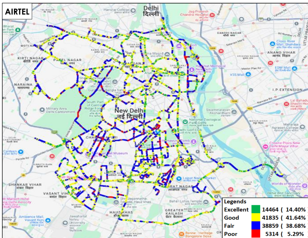
Figure-54: Signal strength auto-selection mode (5G/4G/3G/2G) data - AIRTEL.
