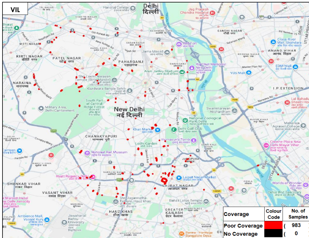
Figure-30: Poor coverage & no coverage locations in auto-selection mode (5G/4G/3G/2G) voice-VIL.
