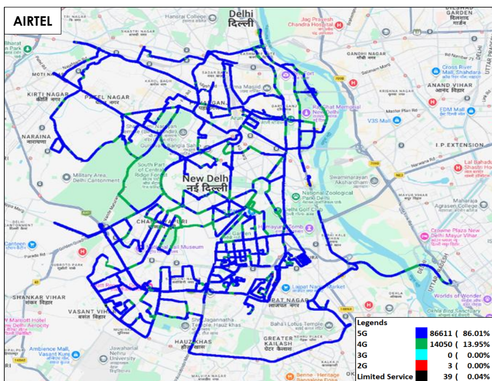
Figure-40: Serving technology plots in auto-selection mode (5G/4G/3G/2G) data - AIRTEL.
