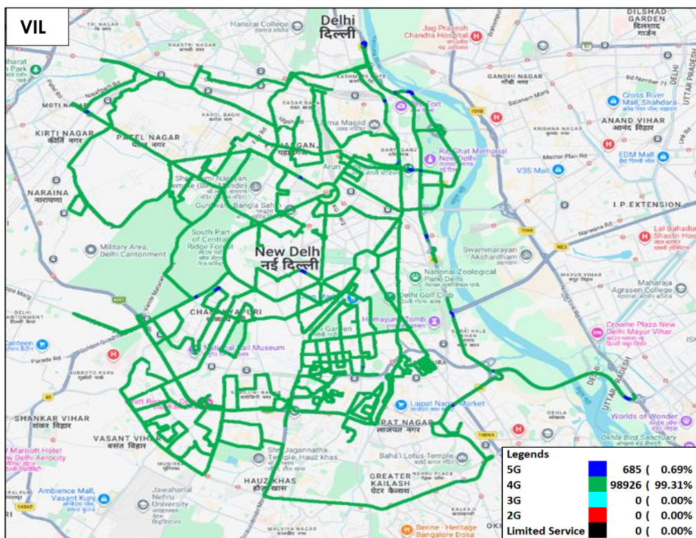
Figure-25: Serving technology plots in auto-selection mode (5G/4G/3G/2G) voice - VIL.
