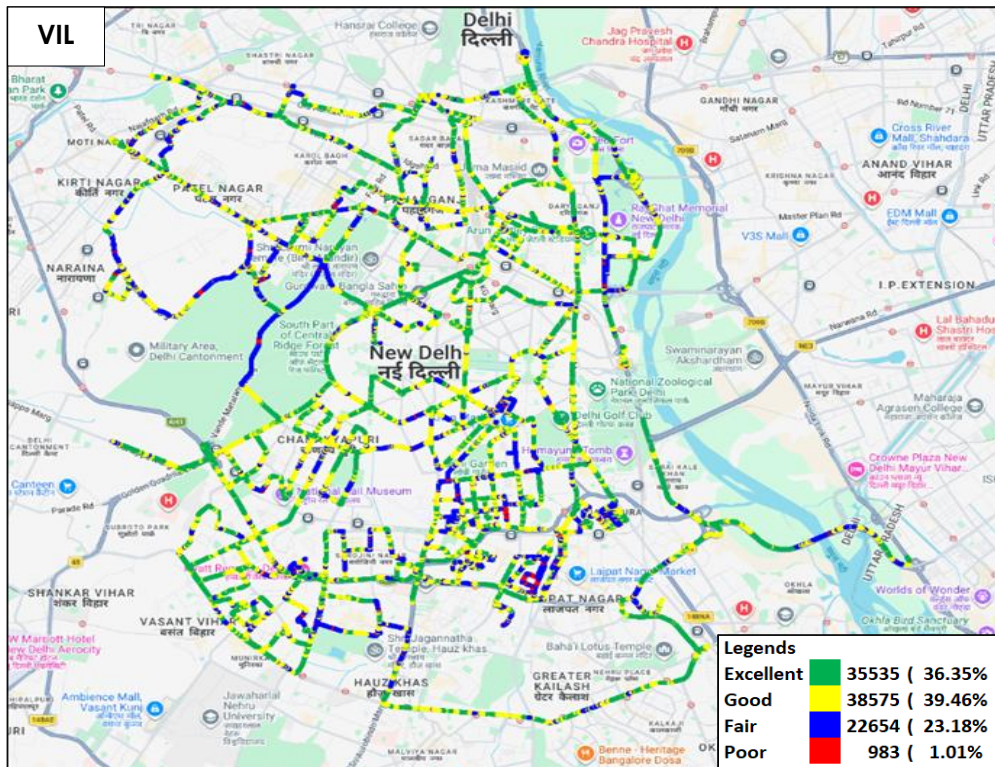
Figure-53: Signal strength auto-selection mode (5G/4G/3G/2G) voice - VIL.
