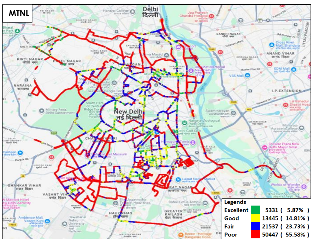
Figure-48: Signal strength 3G/2G network mode voice - MTNL.
