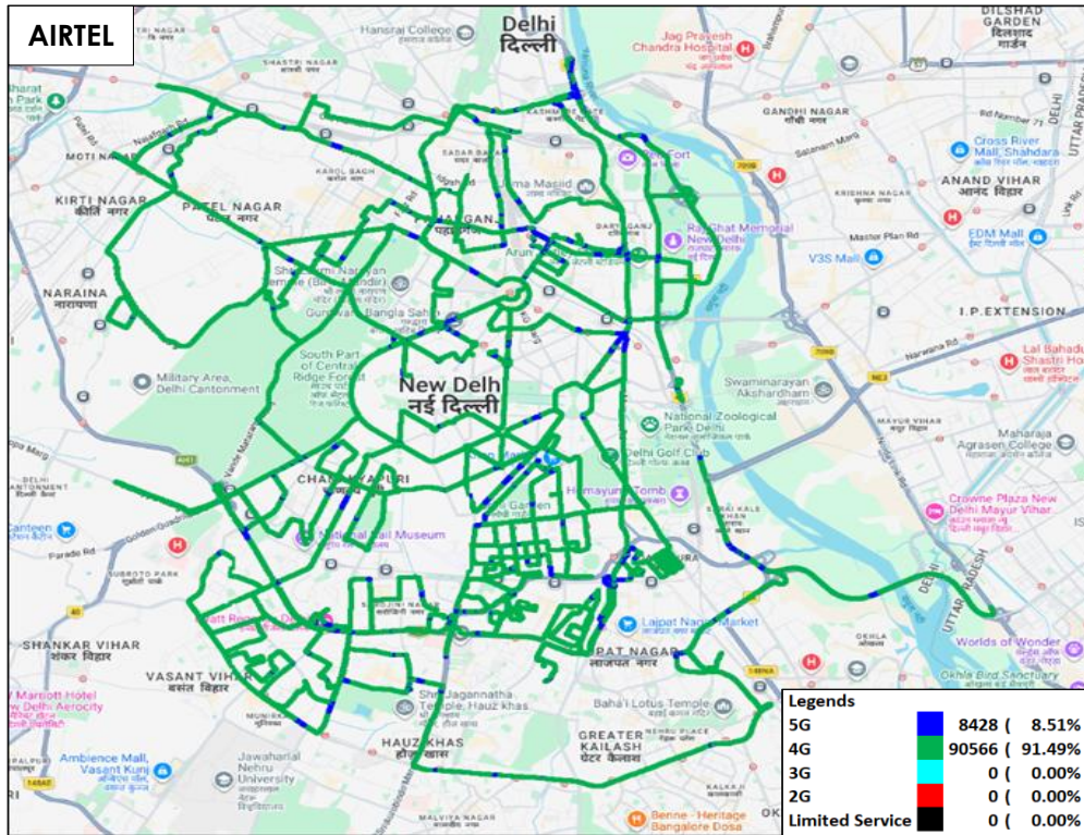
Figure-22: Serving technology plots in auto-selection mode (5G/4G/3G/2G) voice - AIRTEL.
