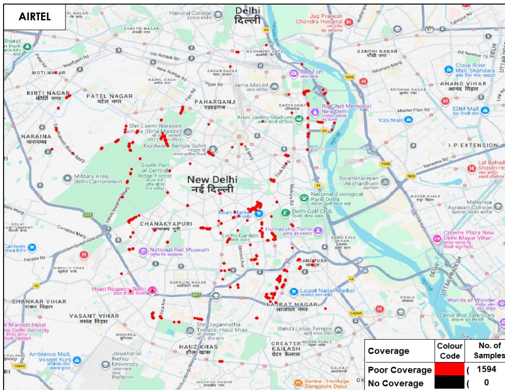
Figure-27: Poor coverage & no coverage locations in auto-selection mode (5G/4G/3G/2G) voice-AIRTEL.
