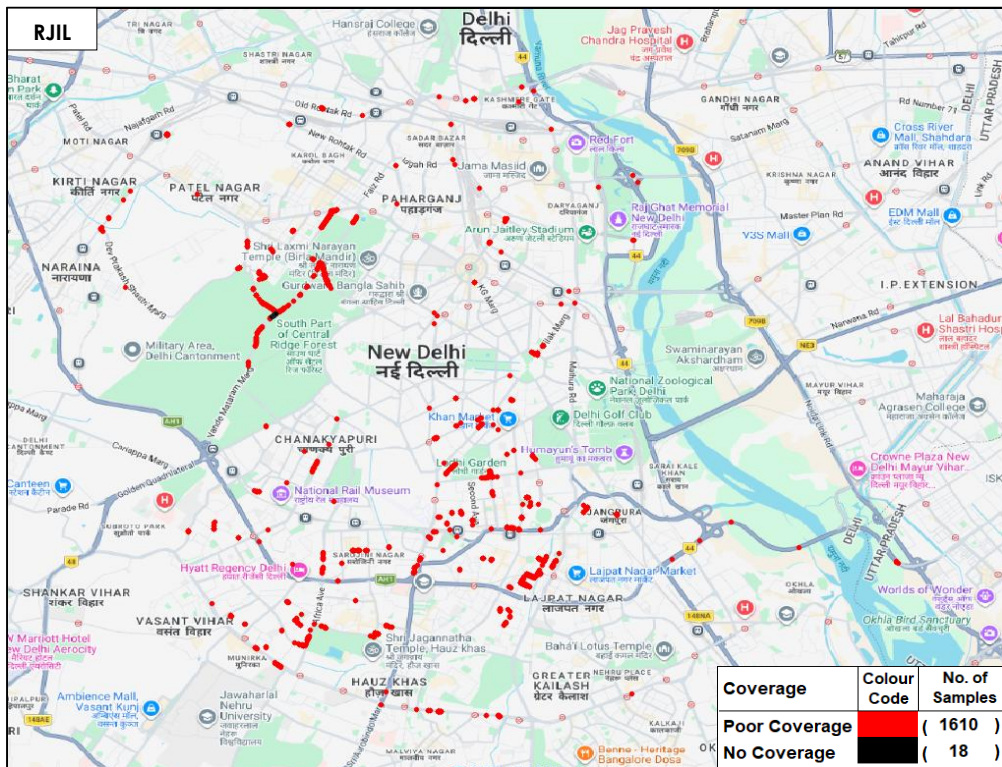
Figure-29: Poor coverage & no coverage locations in auto-selection mode (5G/4G/3G/2G) voice-RJIL.
