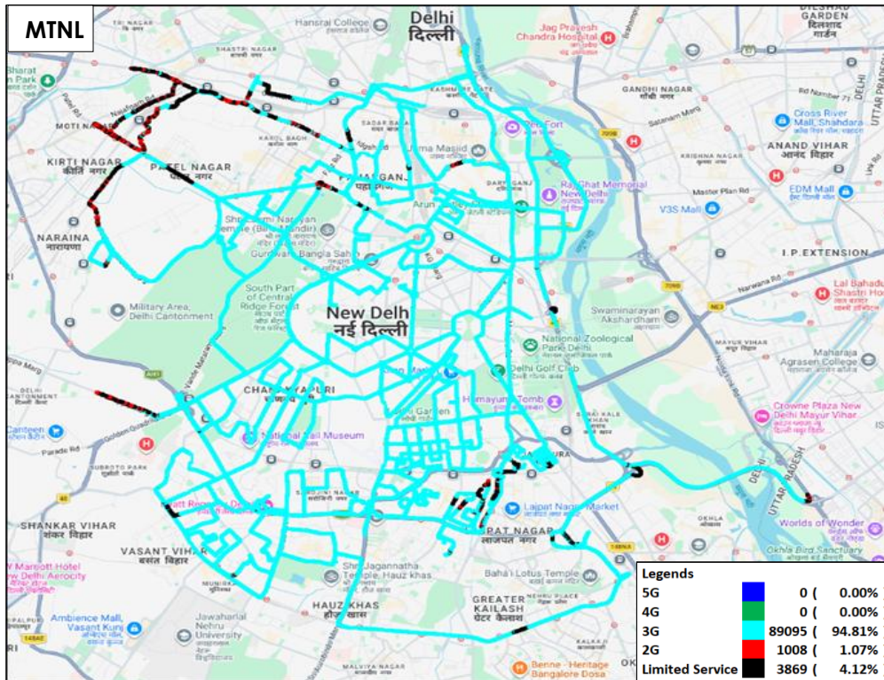
Figure-41: Serving technology plots in auto-selection mode (5G/4G/3G/2G) data - MTNL.
