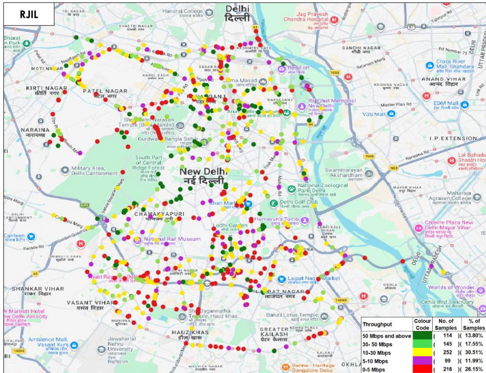
Figure-38: Upload throughput distribution auto-selection mode (5G/4G/3G/2G) - RJIL.
