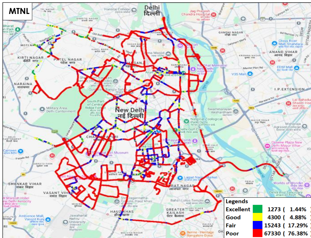
Figure-55: Signal strength auto-selection mode (5G/4G/3G/2G) data - MTNL.
