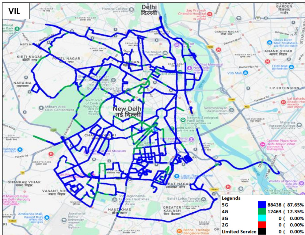
Figure-43: Serving technology plots in auto-selection mode (5G/4G/3G/2G) data - VIL.
