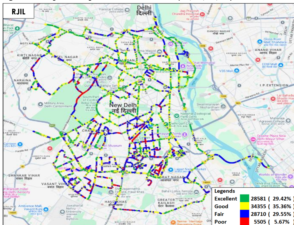
Figure-56: Signal strength auto-selection mode (5G/4G/3G/2G) data - RJIL.
