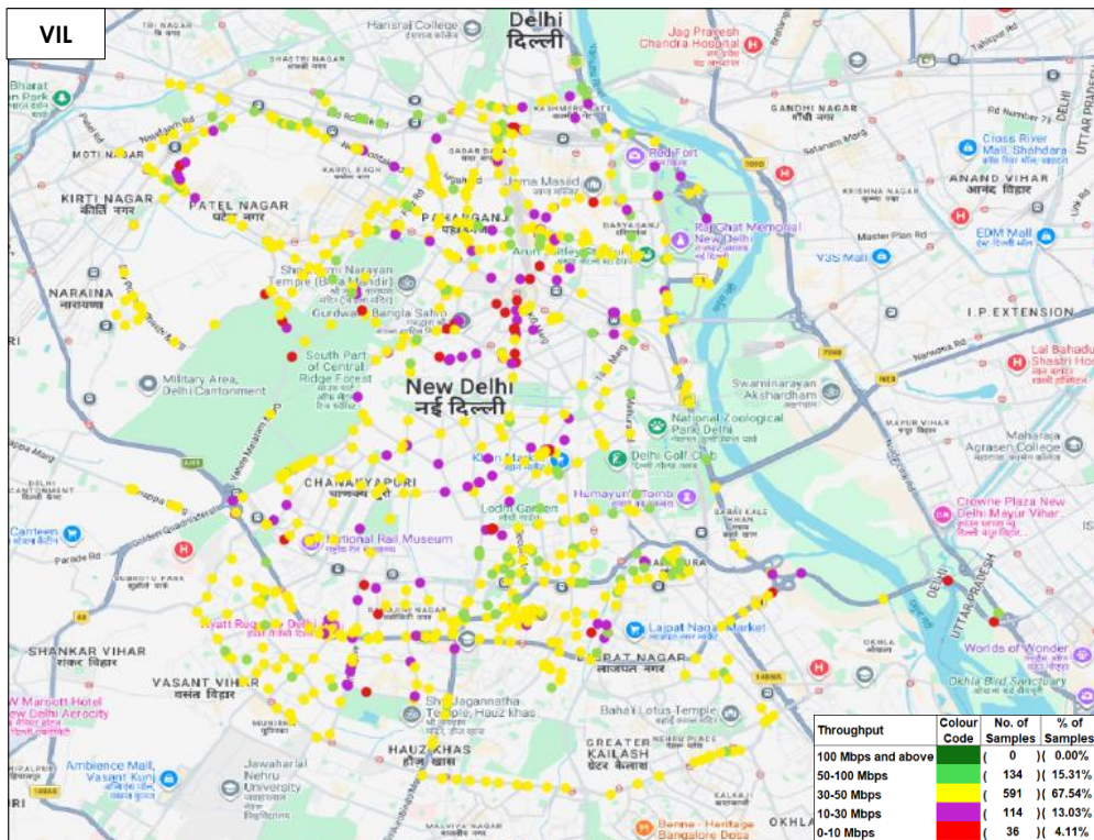
Figure-35: Download throughput distribution auto-selection mode (5G/4G/3G/2G) - VIL.
