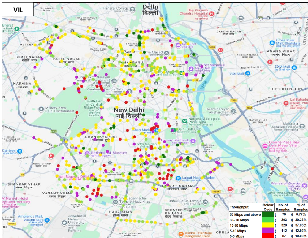
Figure-39: Upload throughput distribution auto-selection mode (5G/4G/3G/2G) - VIL.
