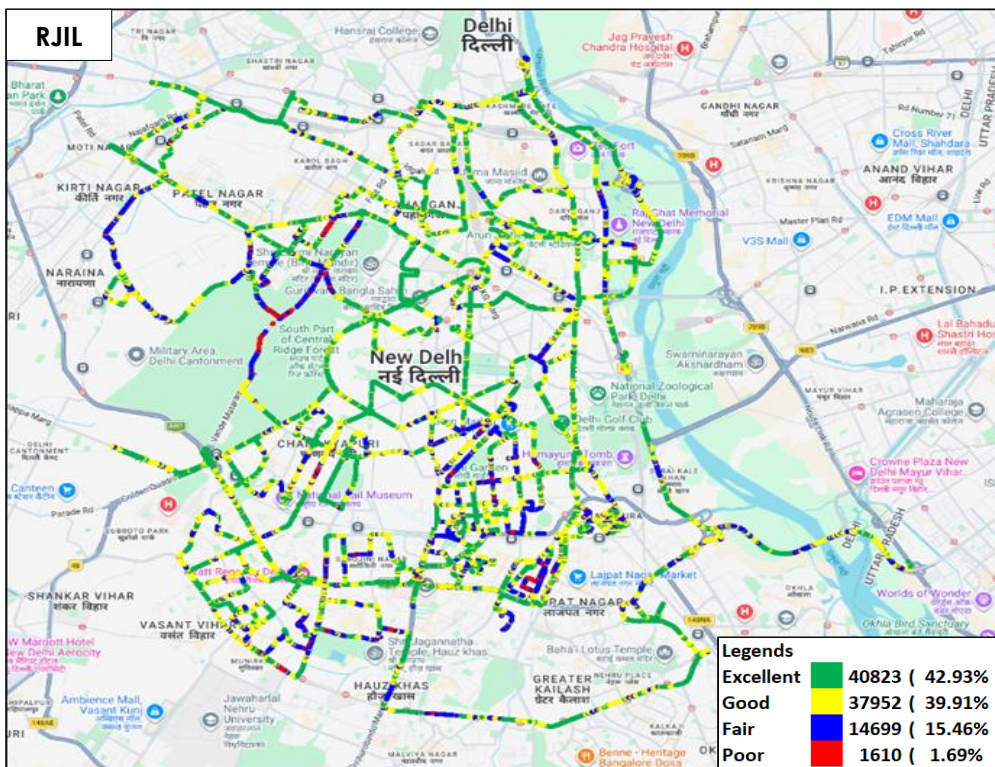
Figure-52: Signal strength auto-selection mode (5G/4G/3G/2G) voice - RJIL.
