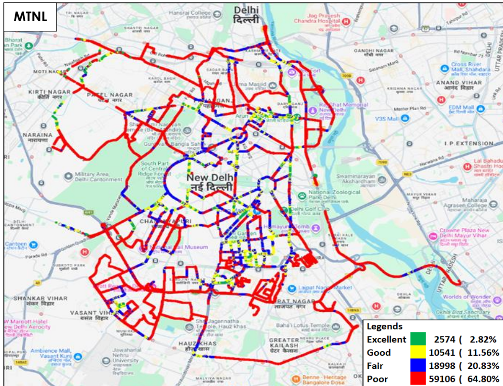
Figure-51: Signal strength auto-selection mode (5G/4G/3G/2G) voice - MTNL.
