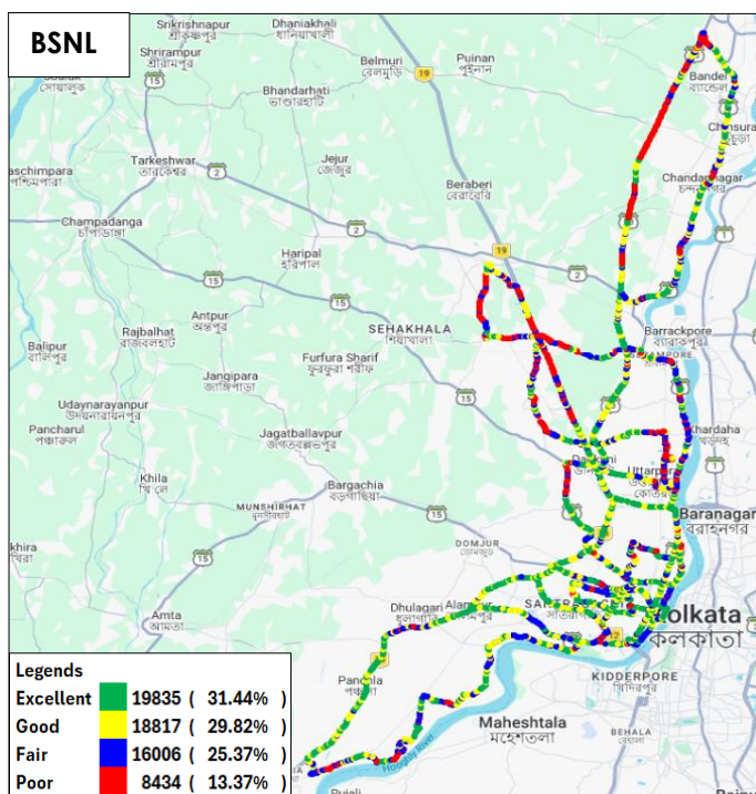
Figure-59: Signal strength 3G/2G network mode voice - BSNL.
