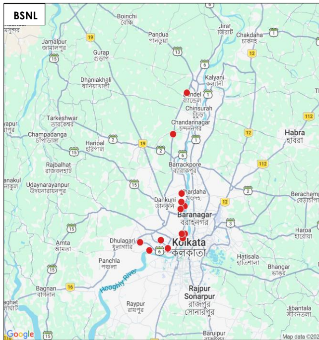
Figure-16: Drop call locations in auto-selection mode (5G/4G/3G/2G) voice - BSNL.
