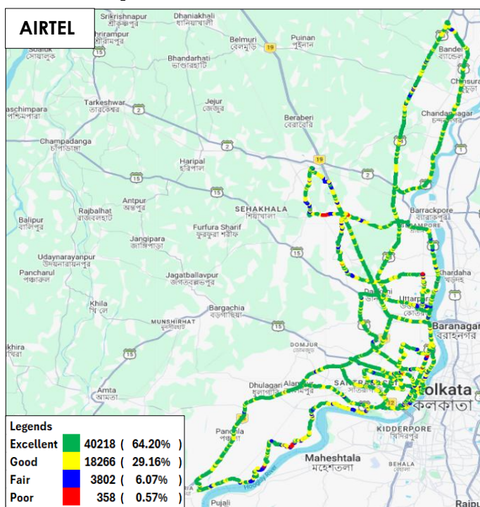
Figure-58: Signal strength 3G/2G network mode voice - AIRTEL.
