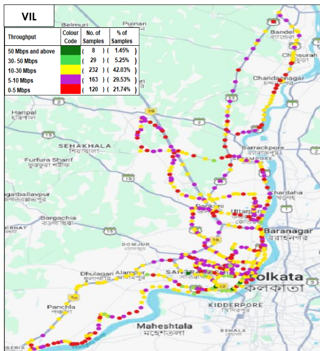
Figure-41: Upload throughput distribution auto-selection mode (5G/4G/3G/2G) - VIL.
