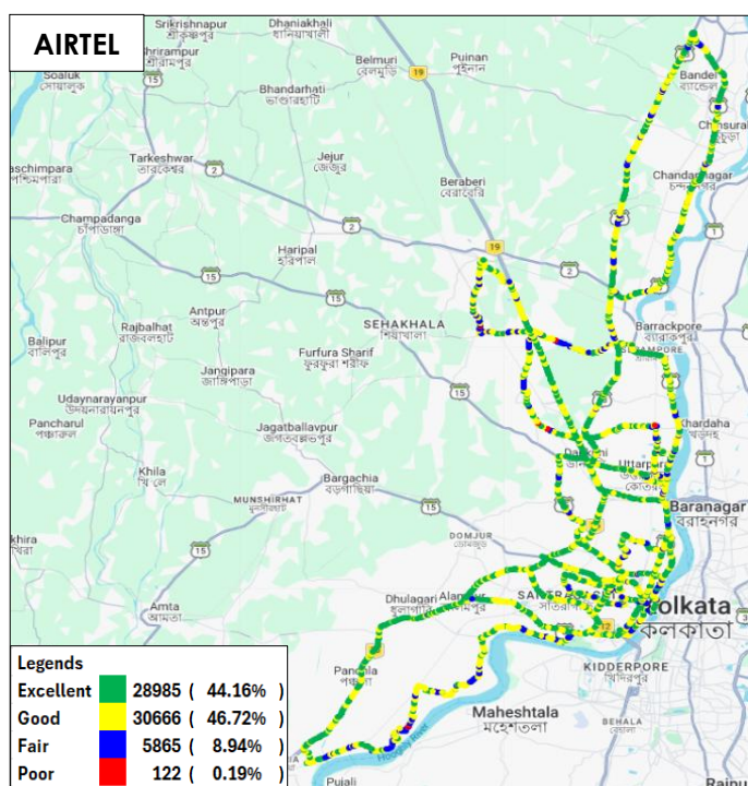
Figure-61: Signal strength auto-selection mode (5G/4G/3G/2G) voice - AIRTEL.
