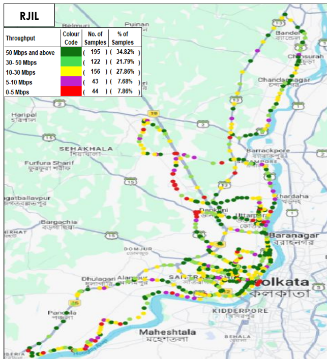
Figure-40: Upload throughput distribution auto-selection mode (5G/4G/3G/2G) - RJIL.
