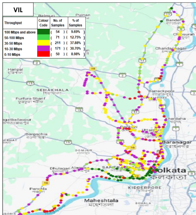
Figure-37: Download throughput distribution auto-selection mode (5G/4G/3G/2G) - VIL.
