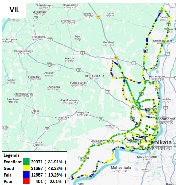
Figure-64: Signal strength auto-selection mode (5G/4G/3G/2G) voice - VIL.
