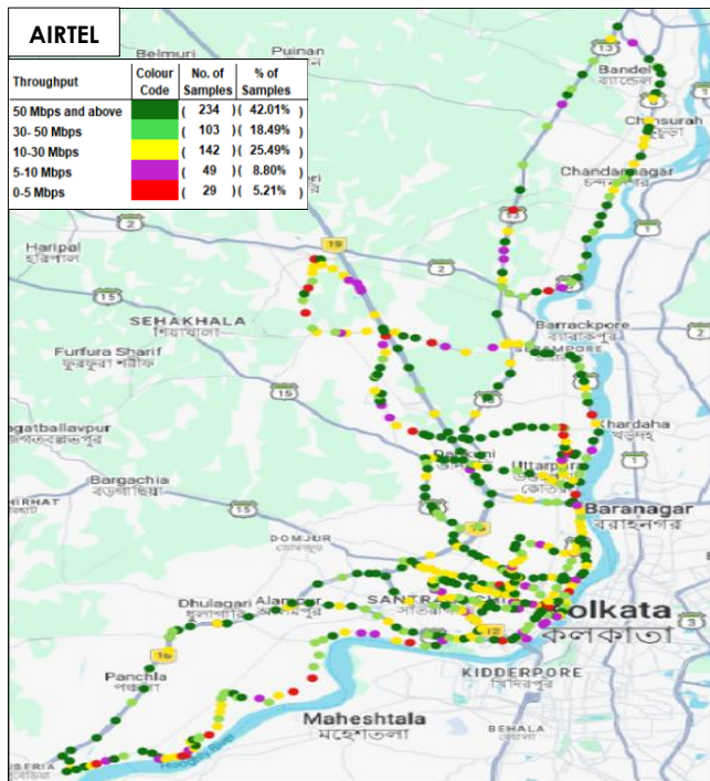
Figure-38: Upload throughput distribution auto-selection mode (5G/4G/3G/2G) - AIRTEL.
