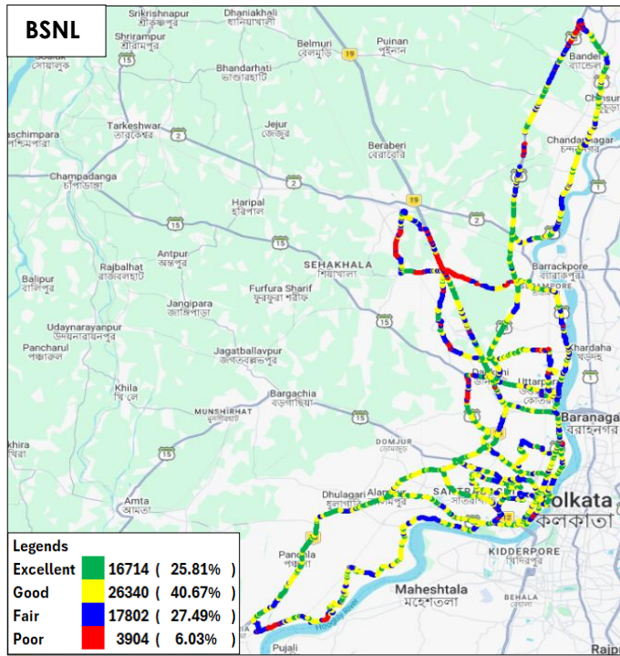
Figure-62: Signal strength auto-selection mode (5G/4G/3G/2G) voice - BSNL.
