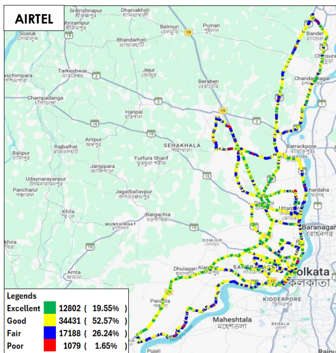
Figure-65: Signal strength auto-selection mode (5G/4G/3G/2G) data - AIRTEL.
