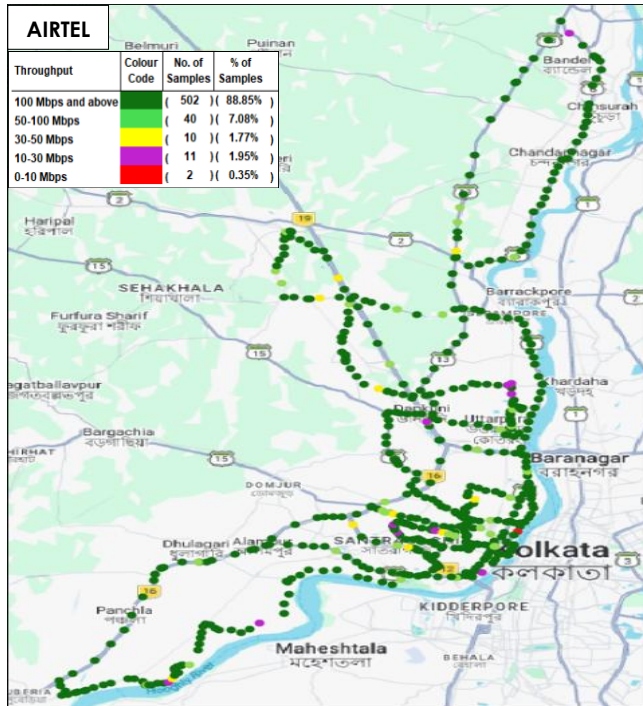
Figure-34: Download throughput distribution auto-selection mode (5G/4G/3G/2G) - AIRTEL.
