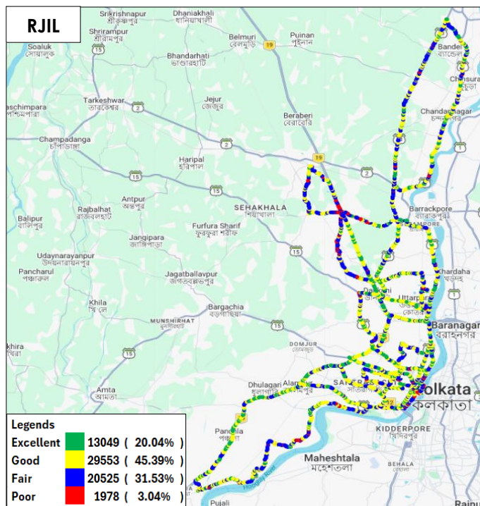
Figure-67: Signal strength auto-selection mode (5G/4G/3G/2G) data - RJIL.
