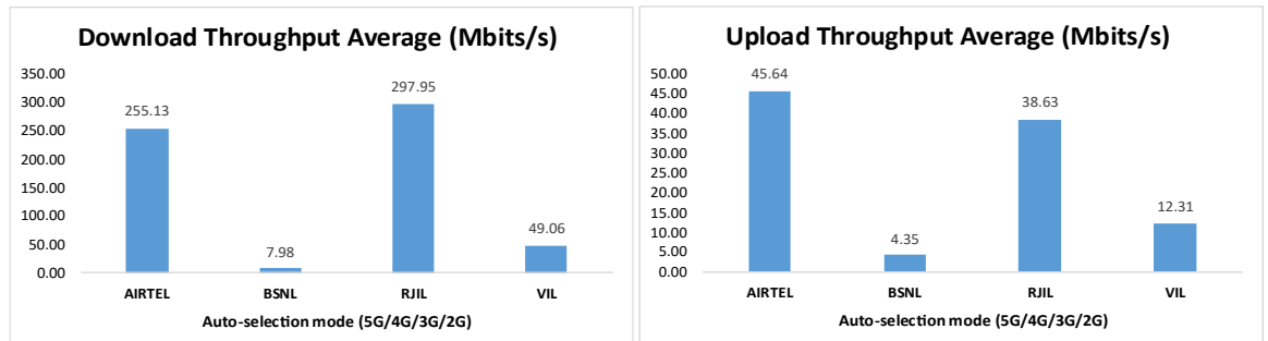
Figure- 33: Download & Upload throughput.
