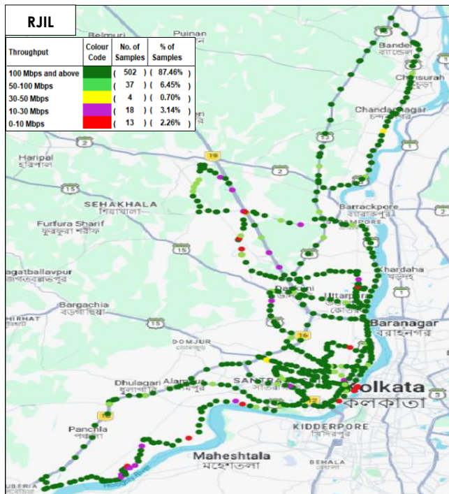
Figure-36: Download throughput distribution auto-selection mode (5G/4G/3G/2G) - RJIL.
