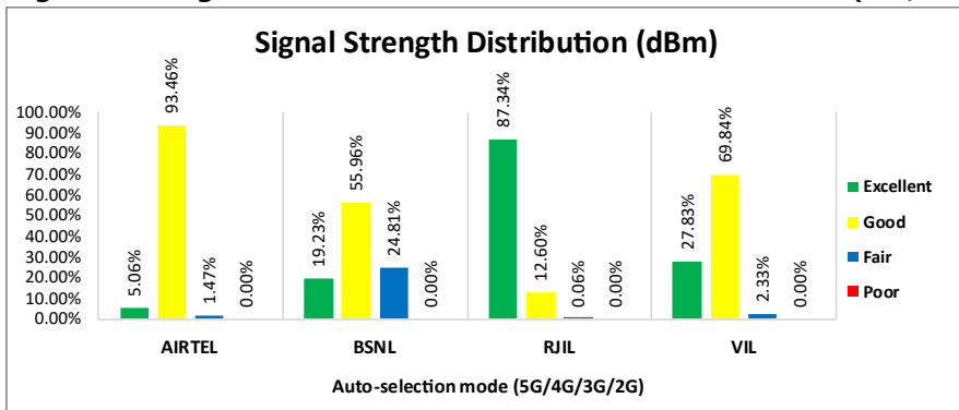
Figure-54: Signal strength distribution auto-selection mode (5G/4G/3G/2G).
