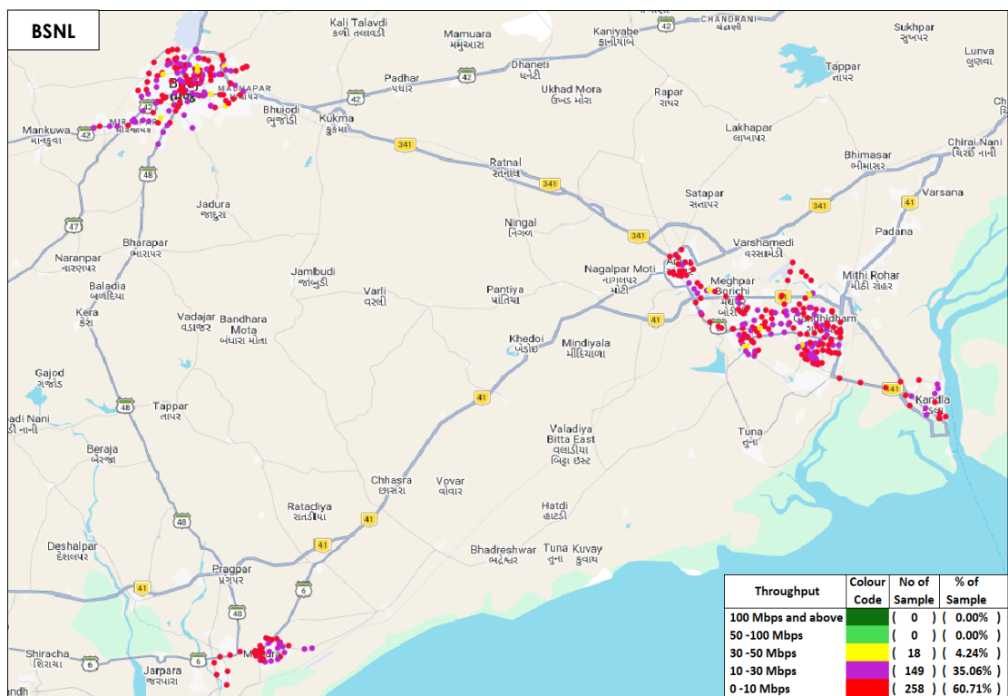
Figure-32: Download throughput distribution auto-selection mode (5G/4G/3G/2G) - BSNL.
