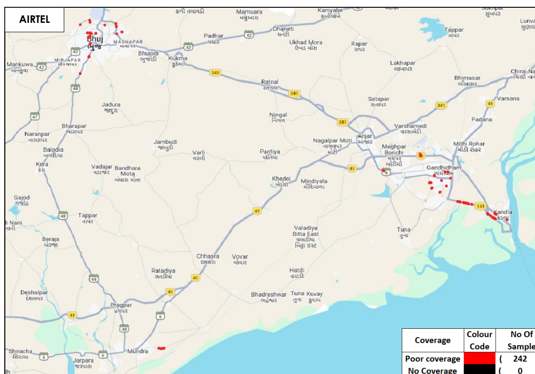
Figure-26: Poor coverage & no coverage locations in auto-selection mode (5G/4G/3G/2G) voice-AIRTEL.
