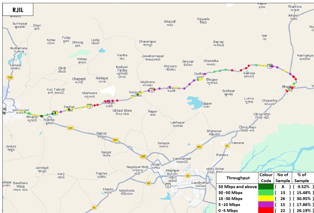
Figure-75: Upload throughput distribution auto-selection mode (5G/4G/3G/2G) - RJIL.
