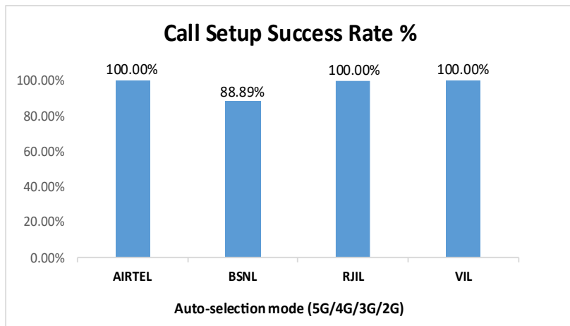
Figure-52: Performance for call setup success rate.
