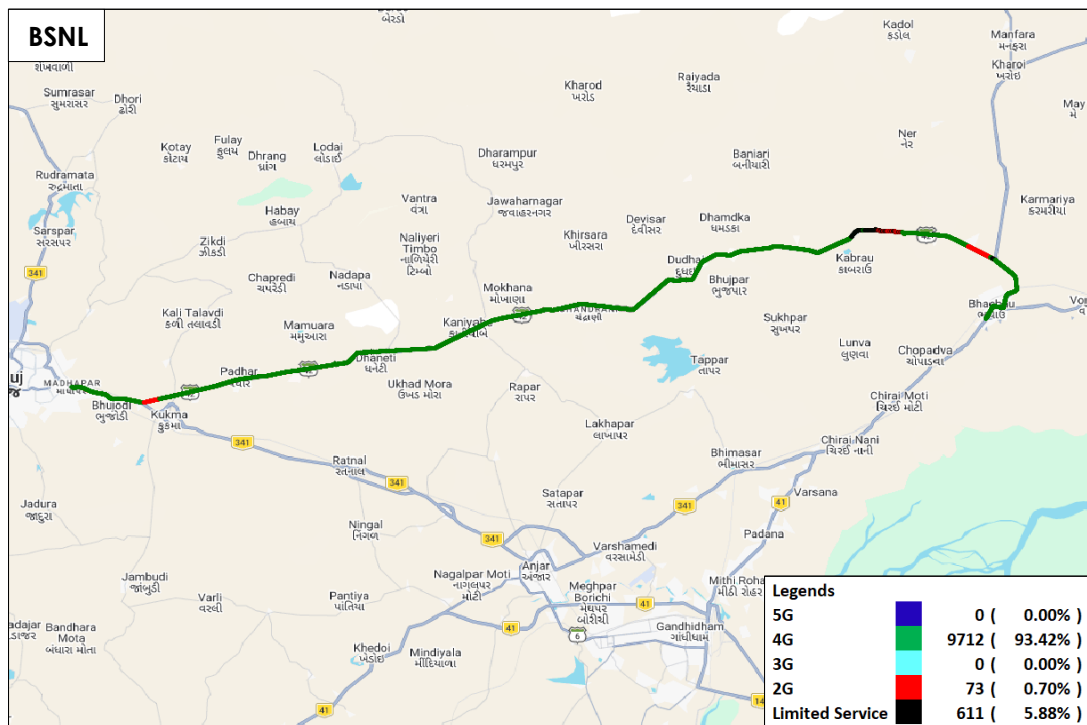
Figure-78: Serving technology plot in auto-selection mode (5G/4G/3G/2G) data - BSNL.
