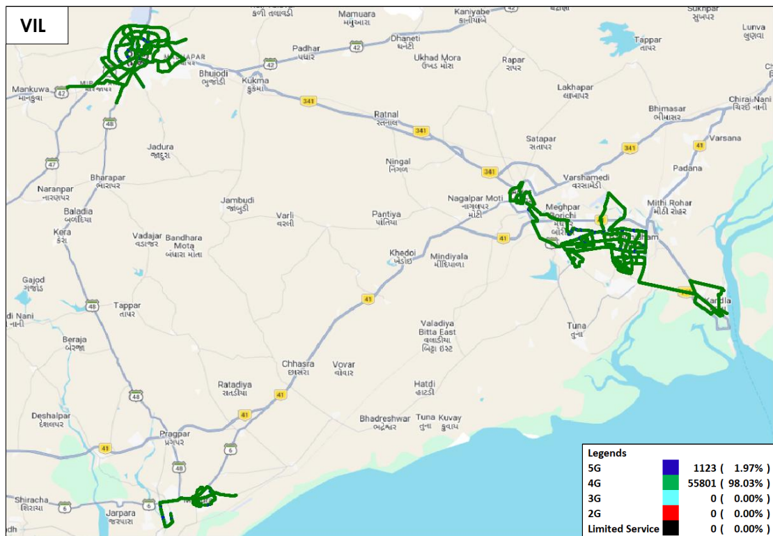
Figure-24: Serving technology plots in auto-selection mode (5G/4G/3G/2G) voice - VIL.
