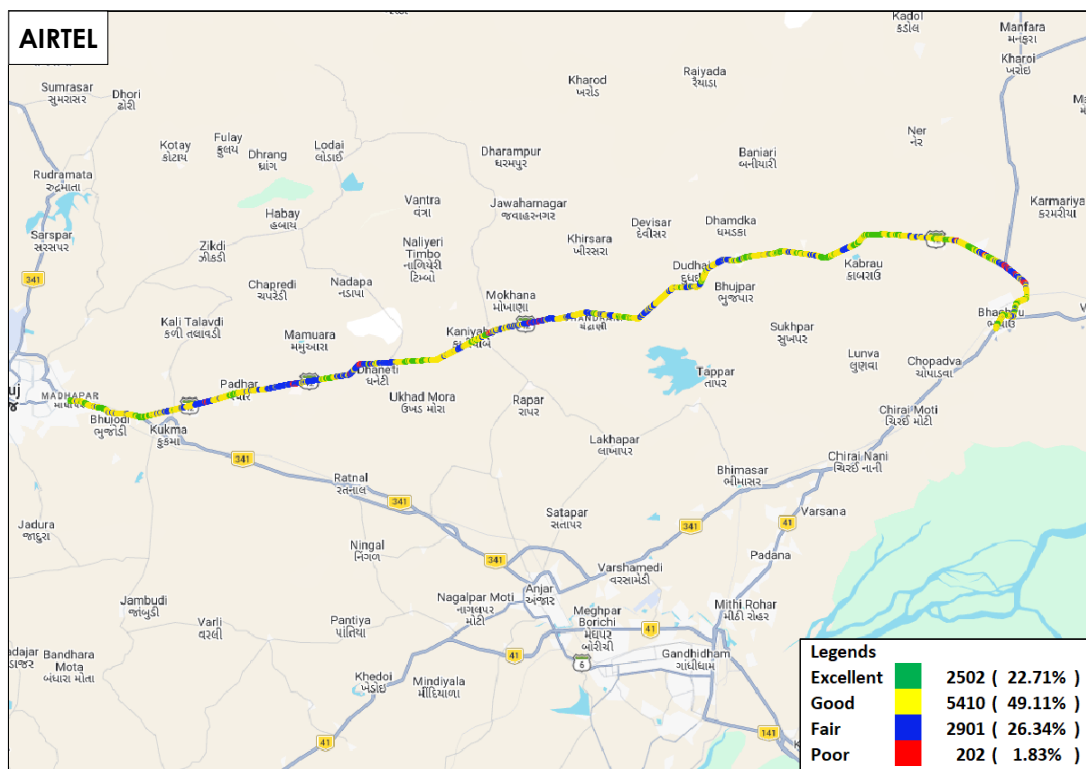
Figure-96: Signal strength auto-selection mode (5G/4G/3G/2G) voice - AIRTEL.
