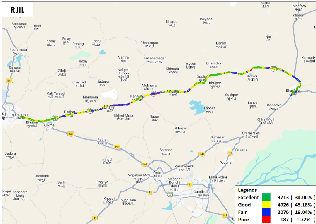
Figure-98: Signal strength auto-selection mode (5G/4G/3G/2G) voice - RJIL.
