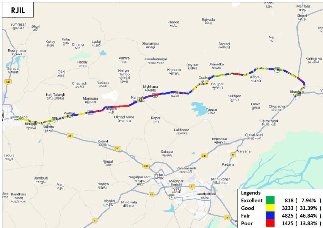
Figure-102: Signal strength auto-selection mode (5G/4G/3G/2G) data - RJIL.
