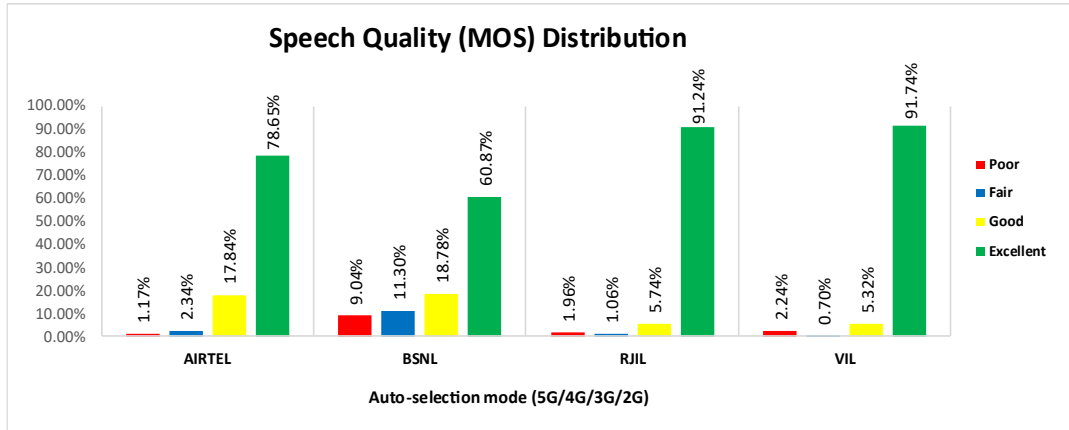
Figure-58: Distribution of samples in MOS range.
