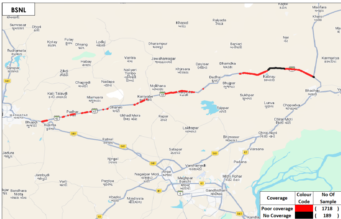
Figure-65: Poor coverage & no coverage locations in auto-selection mode (5G/4G/3G/2G) voice-BSNL.
