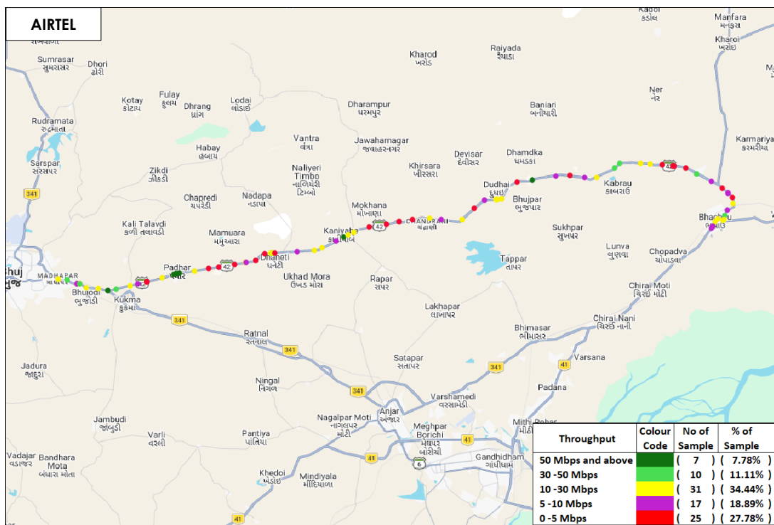
Figure-73: Upload throughput distribution auto-selection mode (5G/4G/3G/2G) - AIRTEL.
