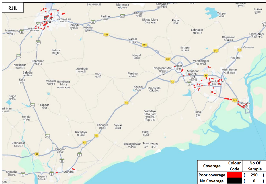
Figure-28: Poor coverage & no coverage locations in auto-selection mode (5G/4G/3G/2G) voice-RJIL.
