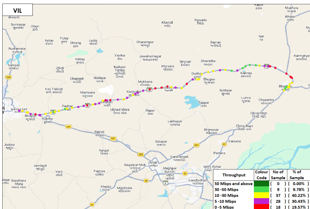
Figure-76: Upload throughput distribution auto-selection mode (5G/4G/3G/2G) - VIL.
