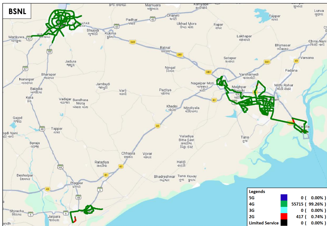
Figure-22: Serving technology plots in auto-selection mode (5G/4G/3G/2G) voice - BSNL.
