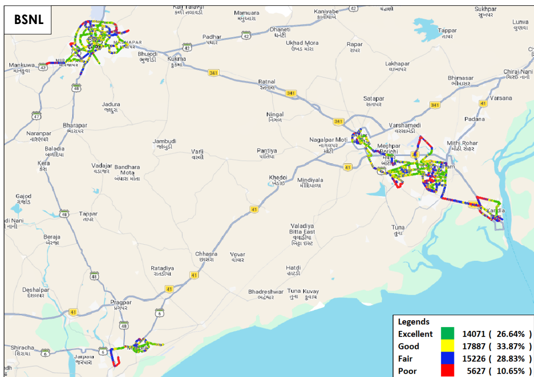
Figure-83: Signal strength 3G/2G network mode voice - BSNL.
