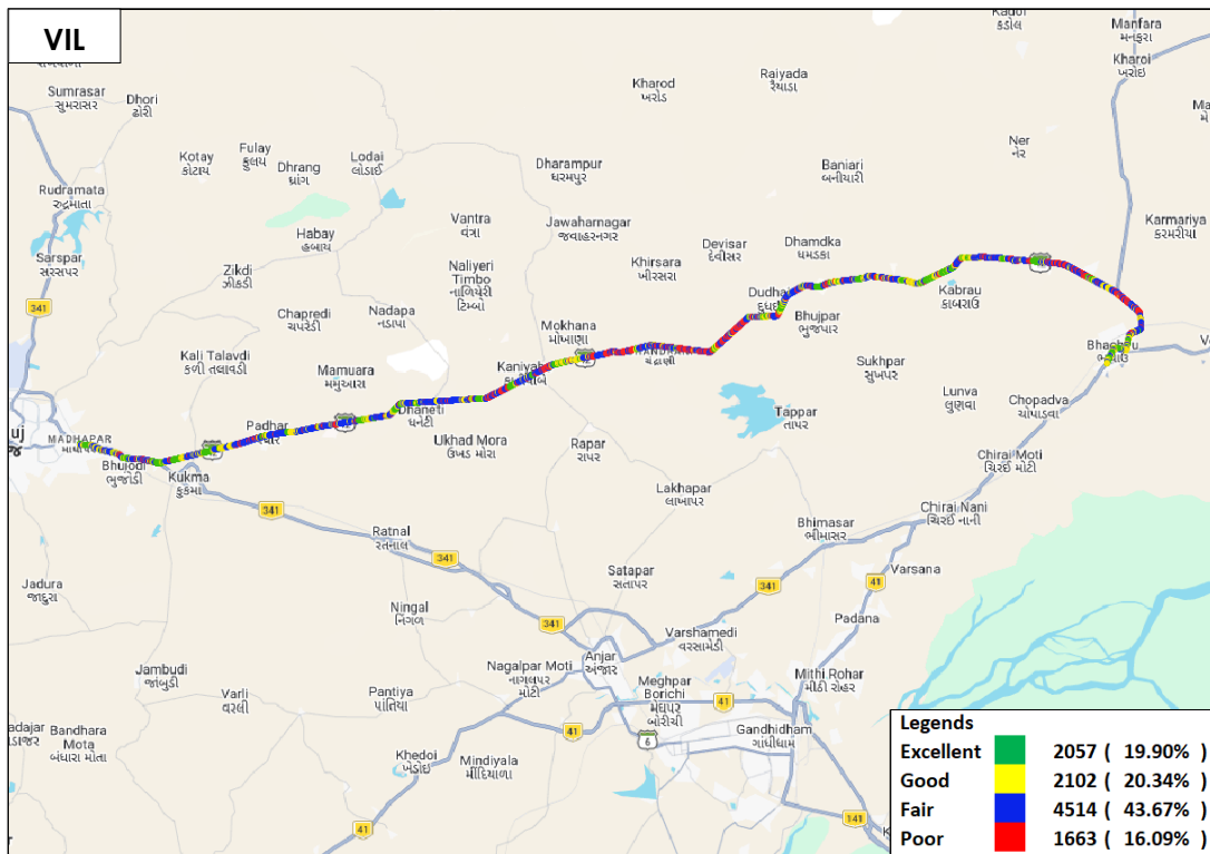
Figure-95: Signal strength 3G/2G network mode voice - VIL.
