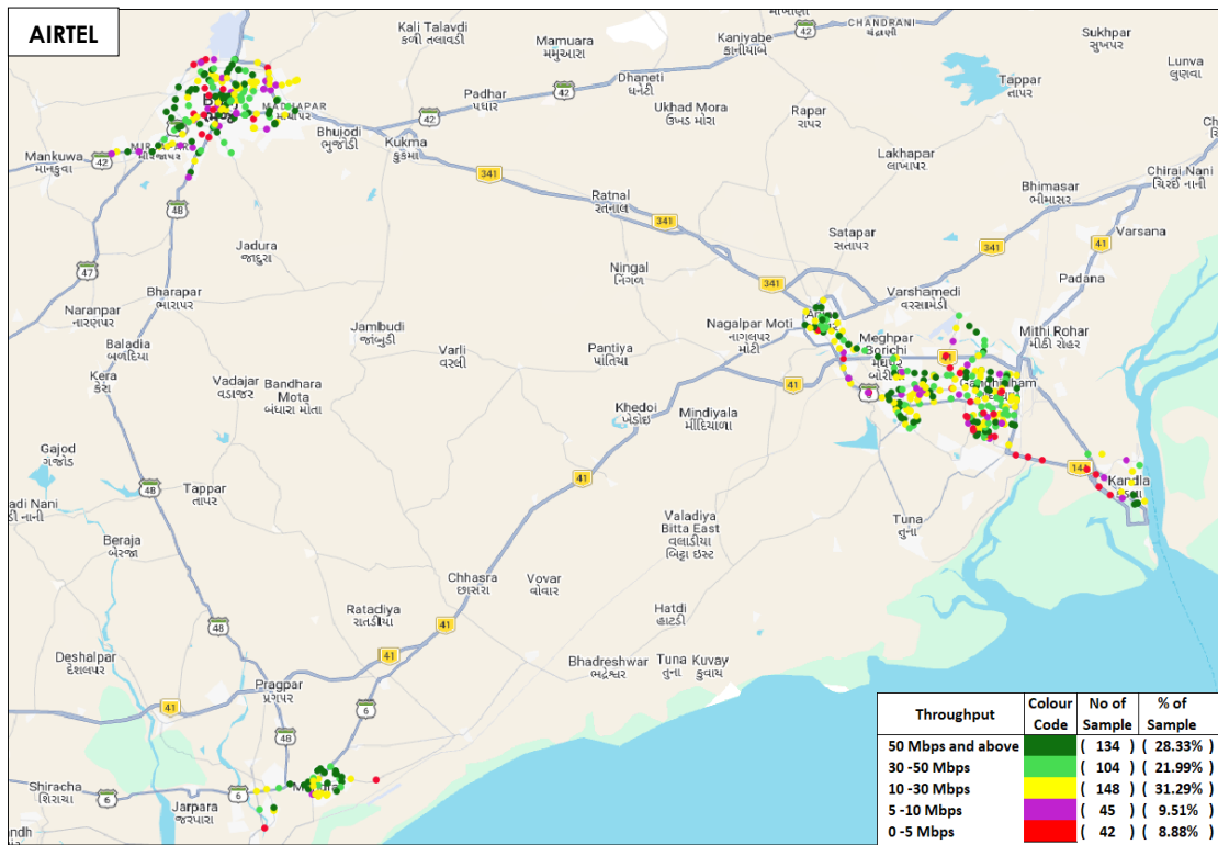
Figure-35: Upload throughput distribution auto-selection mode (5G/4G/3G/2G) - AIRTEL.
