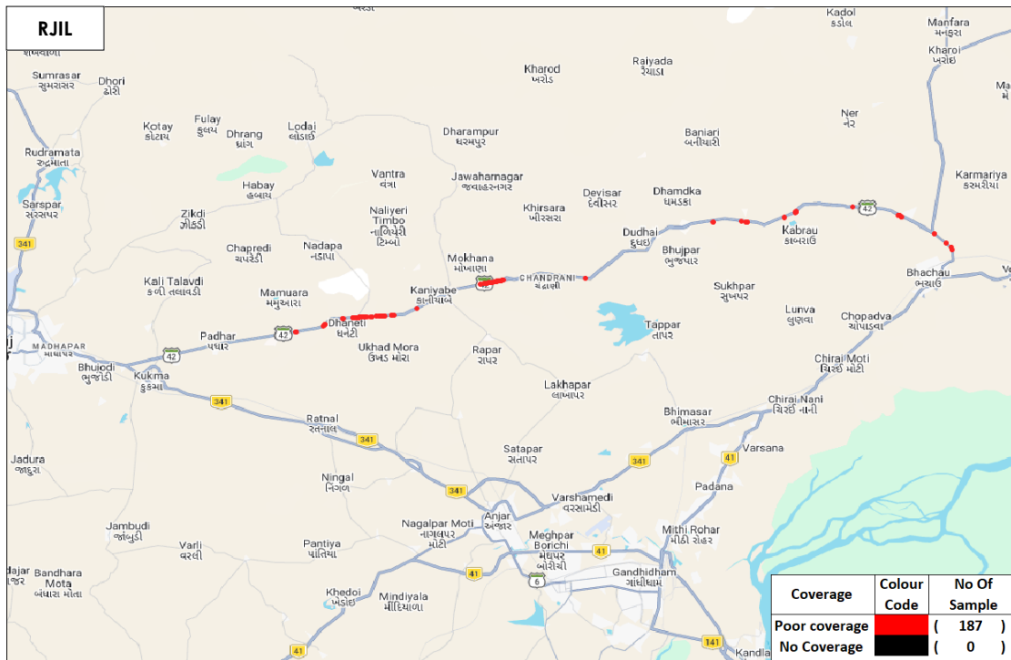
Figure-66: Poor coverage & no coverage locations in auto-selection mode (5G/4G/3G/2G) voice-RJIL.
