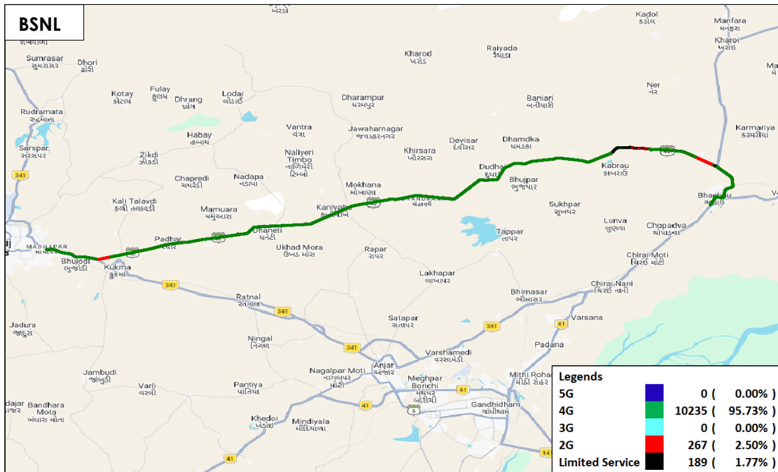
Figure-60: Serving technology plots in auto-selection mode (5G/4G/3G/2G) voice - BSNL.
