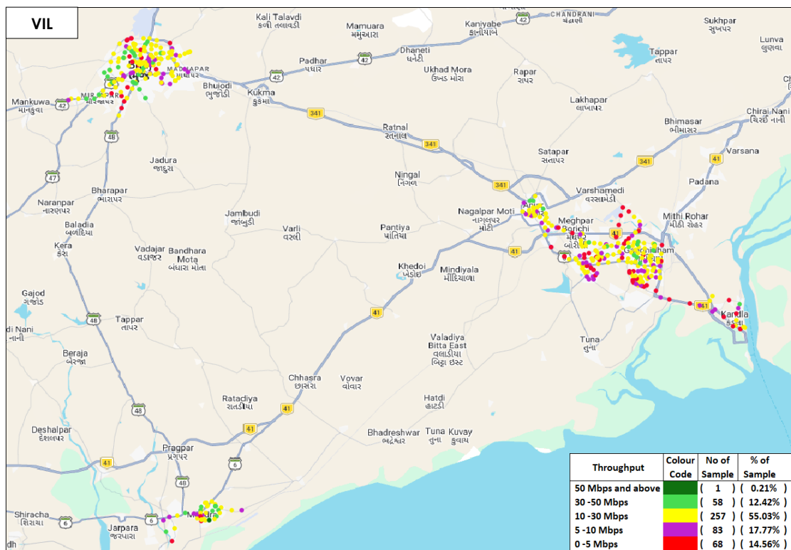
Figure-38: Upload throughput distribution auto-selection mode (5G/4G/3G/2G) - VIL.
