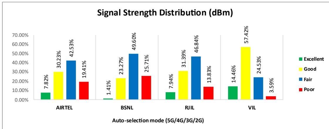
Figure-81: Signal strength distribution auto-selection mode (5G/4G/3G/2G) data.
