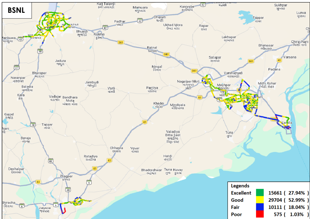
Figure-86: Signal strength auto-selection mode (5G/4G/3G/2G) voice - BSNL.
