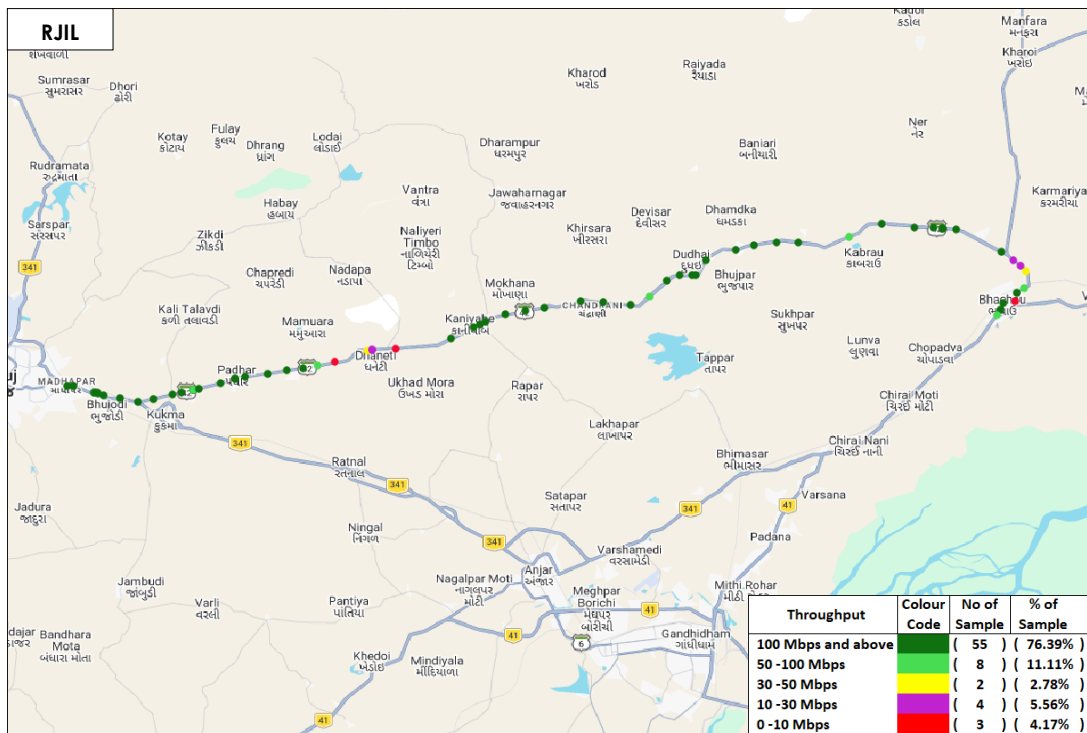
Figure-71: Download throughput distribution auto-selection mode (5G/4G/3G/2G) - RJIL.
