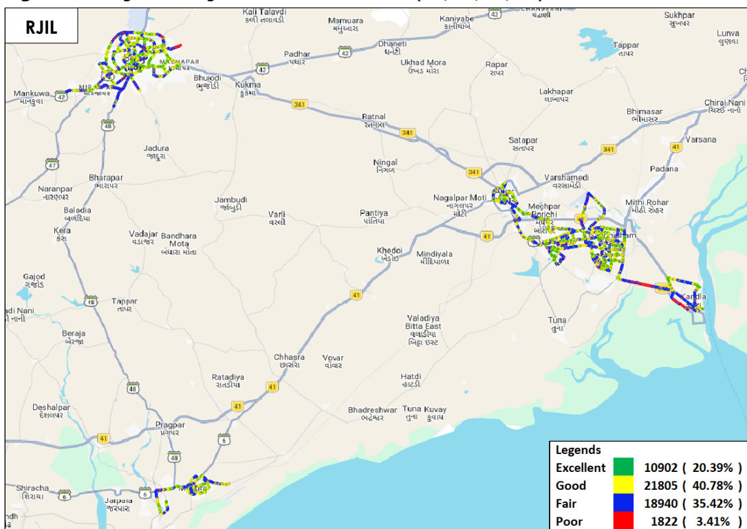
Figure-91: Signal strength auto-selection mode (5G/4G/3G/2G) data - RJIL.
