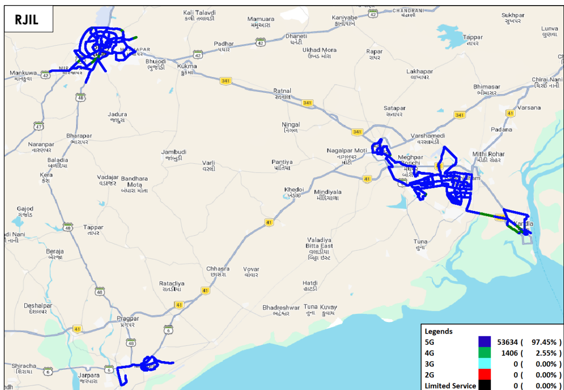
Figure-41: Serving technology plots in auto-selection mode (5G/4G/3G/2G) data - RJIL.
