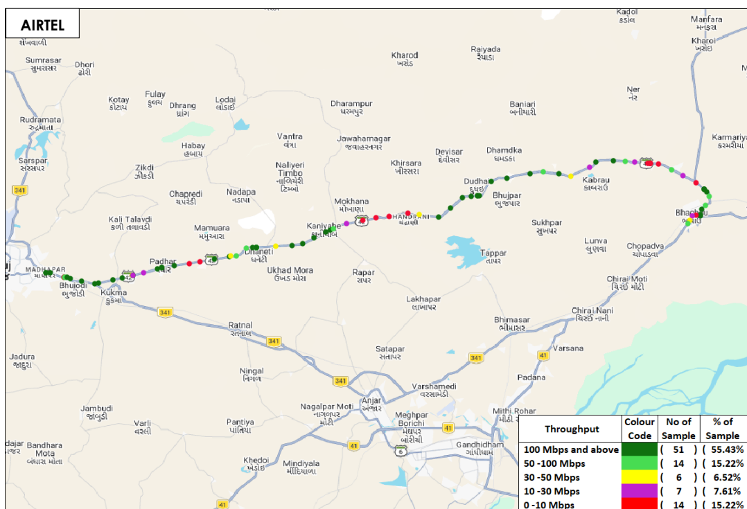
Figure-69: Download throughput distribution auto-selection mode (5G/4G/3G/2G) - AIRTEL.
