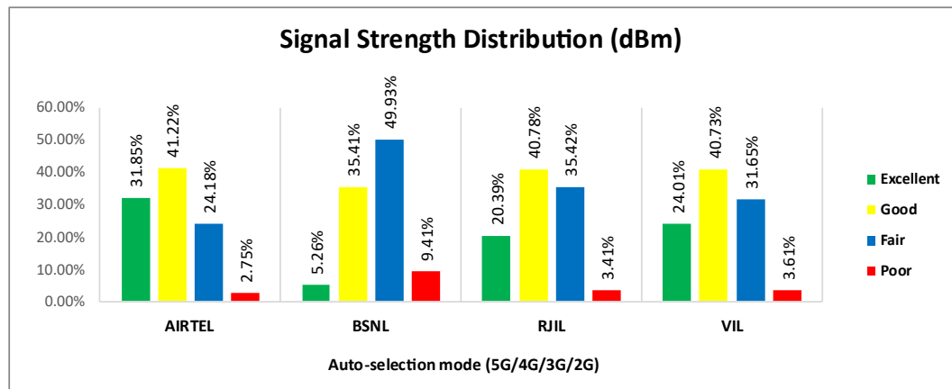
Figure-43: Signal strength distribution auto-selection mode (5G/4G/3G/2G) data.
