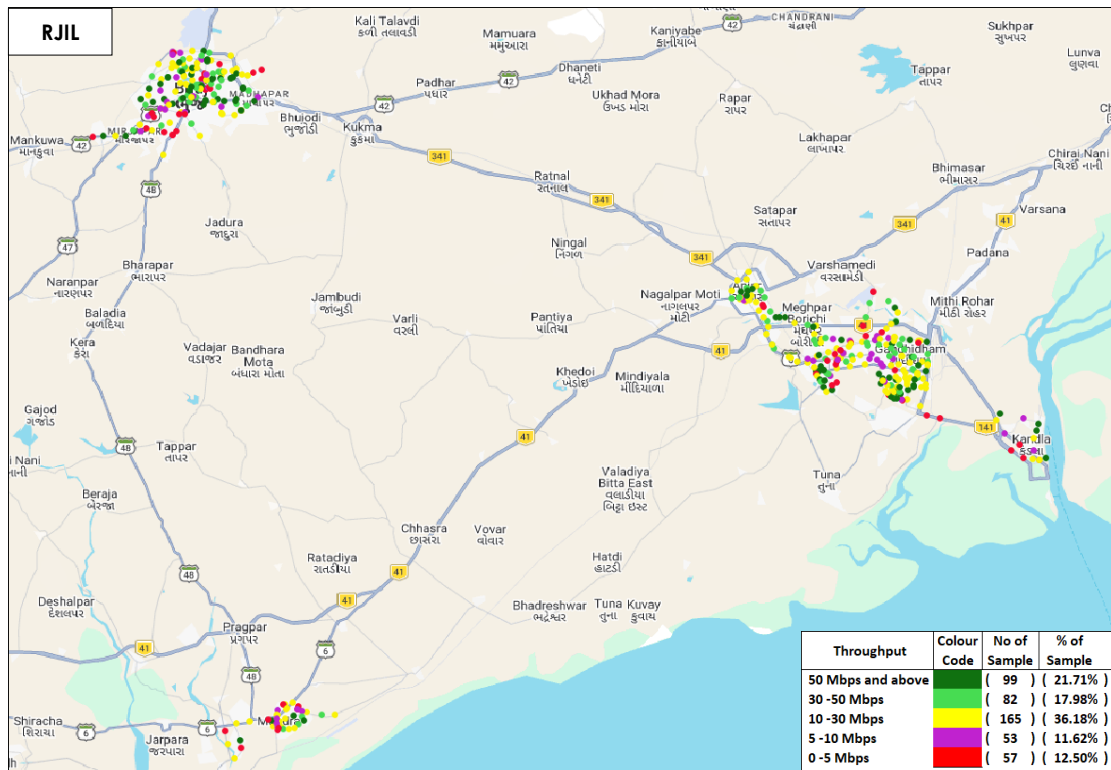
Figure-37: Upload throughput distribution auto-selection mode (5G/4G/3G/2G) - RJIL.
