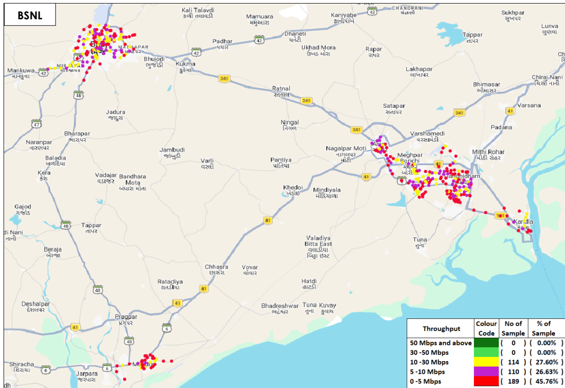
Figure-36: Upload throughput distribution auto-selection mode (5G/4G/3G/2G) - BSNL.
