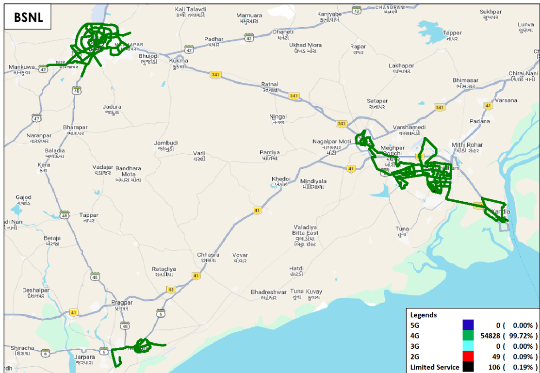
Figure-40: Serving technology plots in auto-selection mode (5G/4G/3G/2G) data - BSNL.
