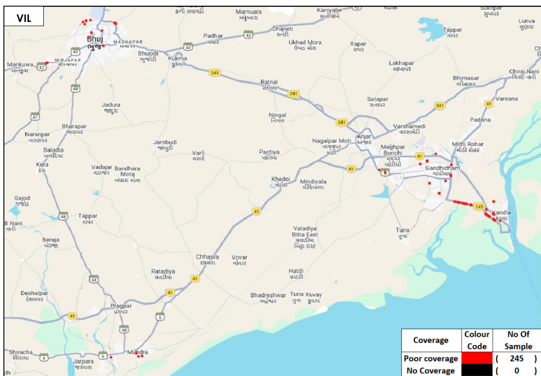
Figure-29: Poor coverage & no coverage locations in auto-selection mode (5G/4G/3G/2G) voice-VIL.
