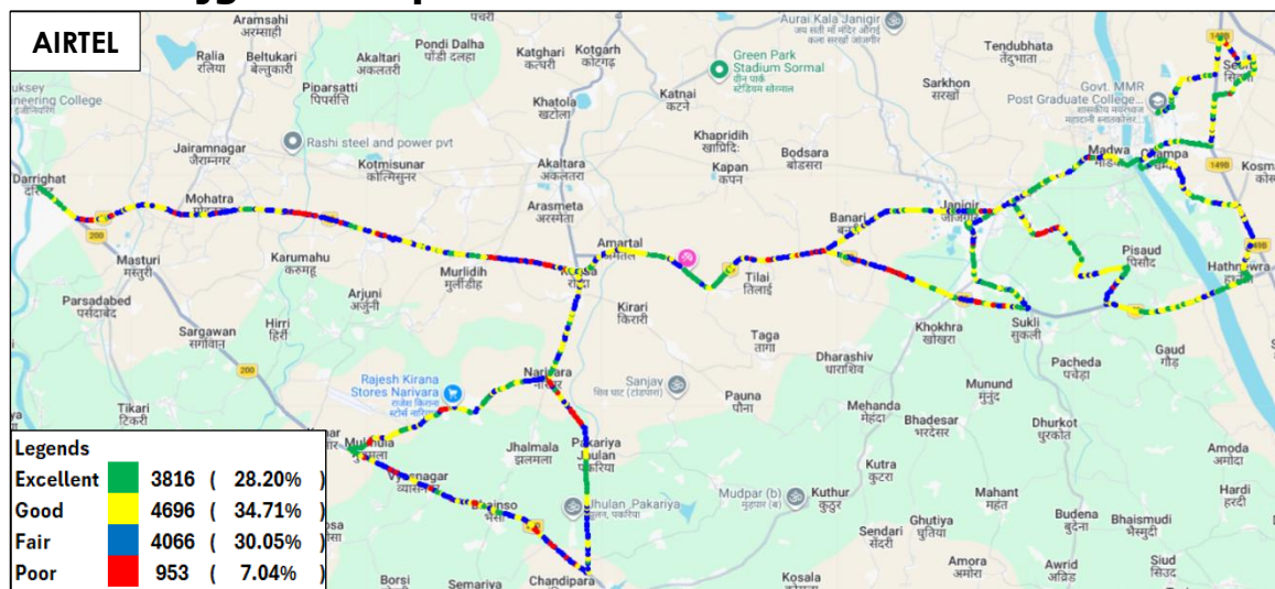
Figure-99: Signal strength 3G/2G network mode voice - AIRTEL.
