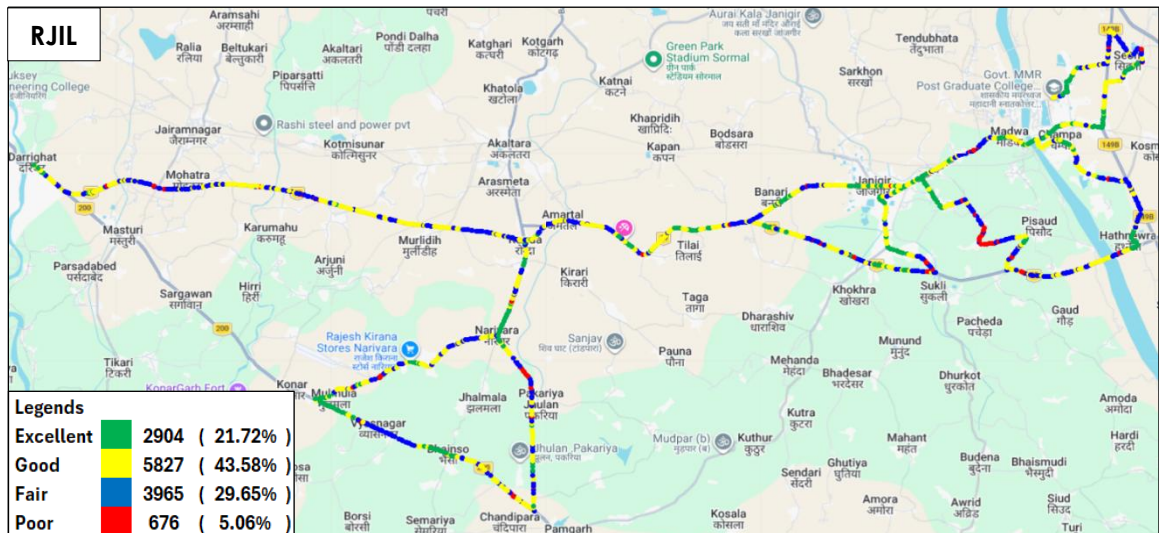
Figure-104: Signal strength auto-selection mode (5G/4G/3G/2G) voice - RJIL.
