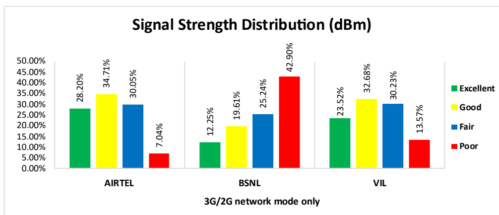
Figure-53: Signal strength distribution 3G/2G network mode only.
