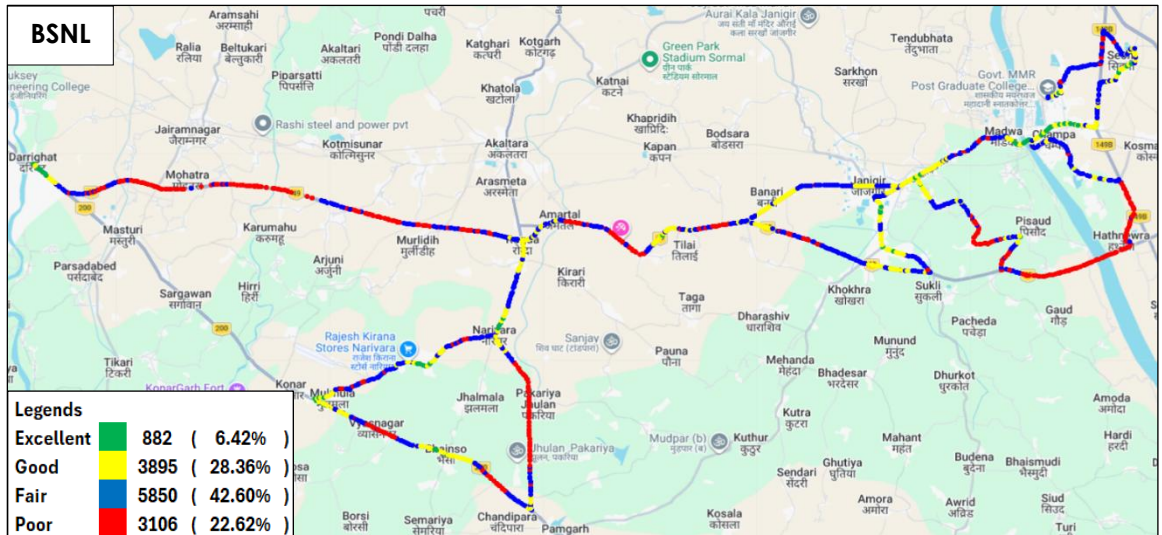
Figure-107: Signal strength auto-selection mode (5G/4G/3G/2G) data - BSNL.
