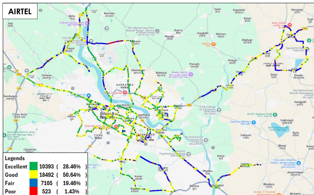
Figure-91: Signal strength auto-selection mode (5G/4G/3G/2G) voice - AIRTEL.
