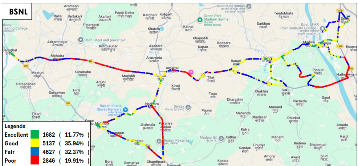
Figure-103: Signal strength auto-selection mode (5G/4G/3G/2G) voice - BSNL.
