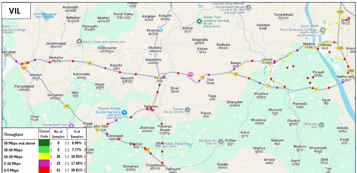
Figure-80: Upload throughput distribution auto-selection mode (5G/4G/3G/2G) - VIL.
