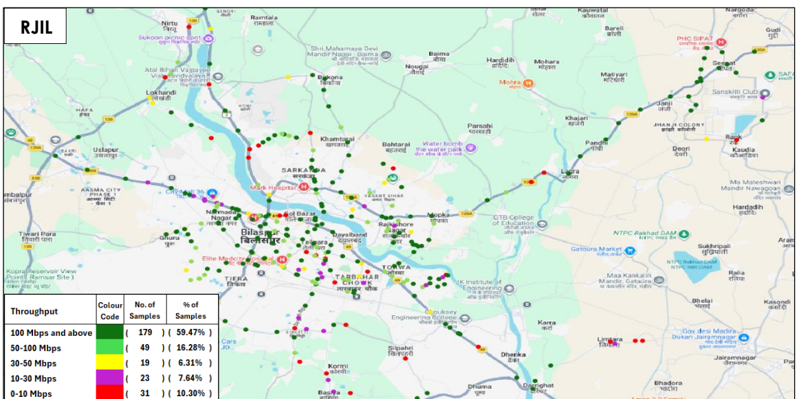
Figure-36: Download throughput distribution auto-selection mode (5G/4G/3G/2G) - RJIL.
