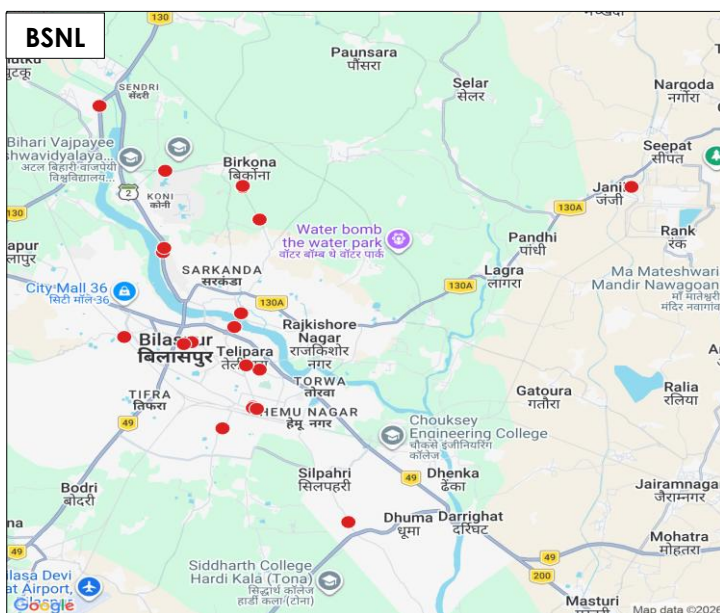
Figure-20: Number of silence instances for >3 Sec Mobile-to-Mobile (5G/4G-Open Mode) - BSNL.
