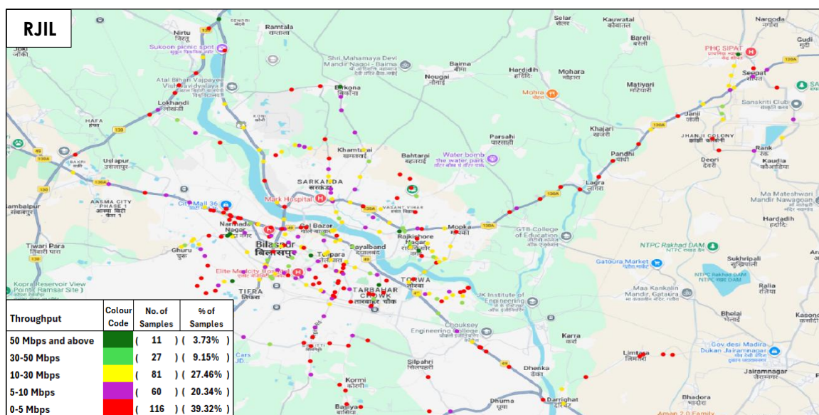
Figure-40: Upload throughput distribution auto-selection mode (5G/4G/3G/2G) - RJIL.
