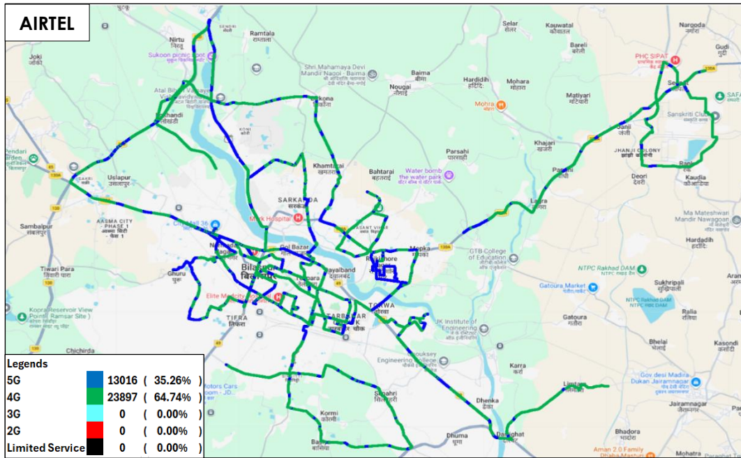
Figure-24: Serving technology plots in auto-selection mode (5G/4G/3G/2G) voice - AIRTEL.
