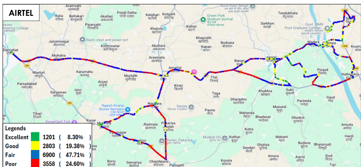
Figure-106: Signal strength auto-selection mode (5G/4G/3G/2G) data - AIRTEL.
