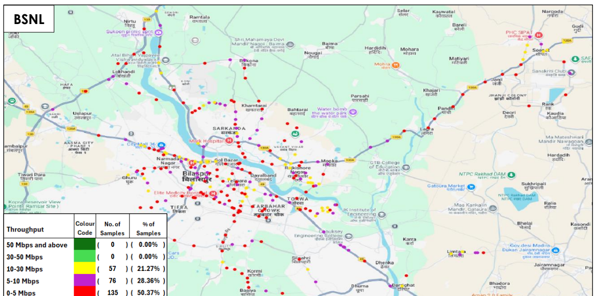
Figure-39: Upload throughput distribution auto-selection mode (5G/4G/3G/2G) - BSNL.
