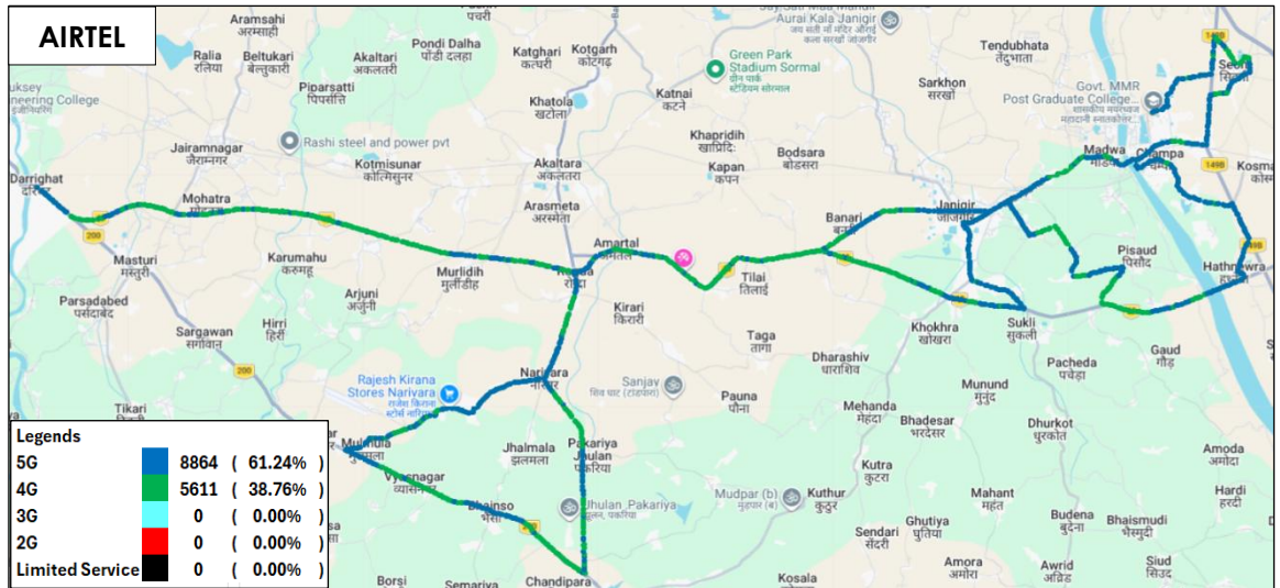
Figure-81: Serving technology plots in auto-selection mode (5G/4G/3G/2G) data -AIRTEL.
