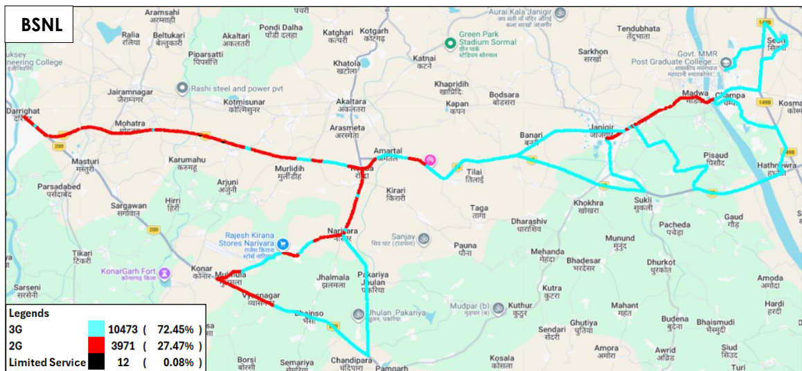
Figure-51: Serving technology plots 3G/2G network mode - BSNL.
