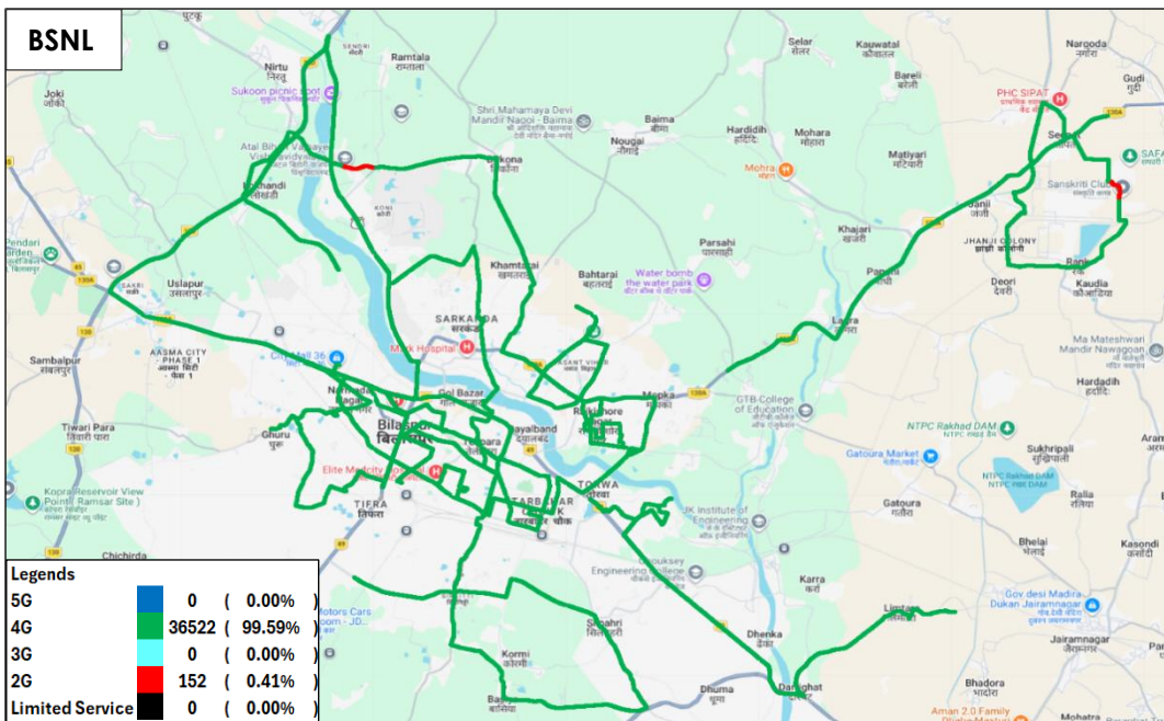
Figure-25: Serving technology plots in auto-selection mode (5G/4G/3G/2G) voice - BSNL.
