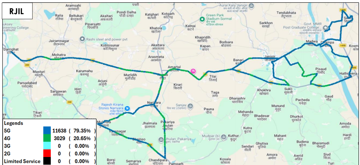
Figure-65: Serving technology plots in auto-selection mode (5G/4G/3G/2G) voice - RJIL.
