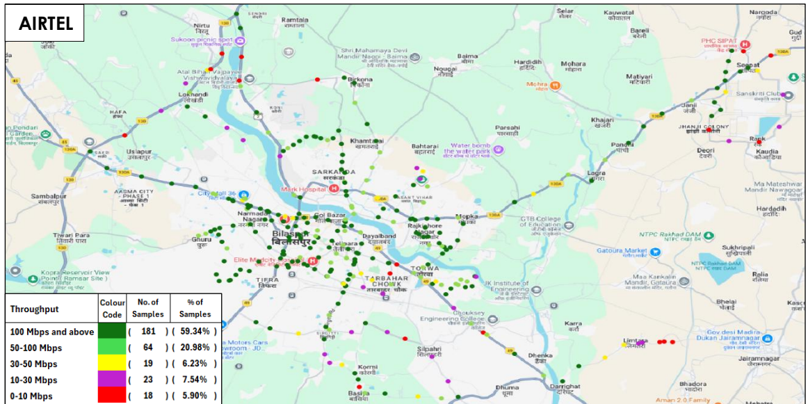
Figure-34: Download throughput distribution auto-selection mode (5G/4G/3G/2G) - AIRTEL.
