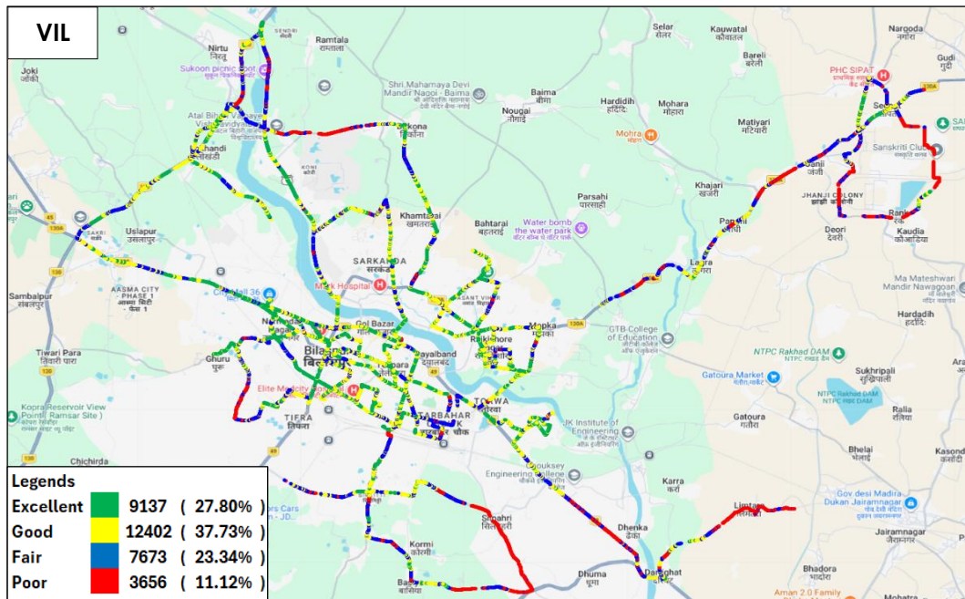
Figure-90: Signal strength 3G/2G network mode voice - VIL.
