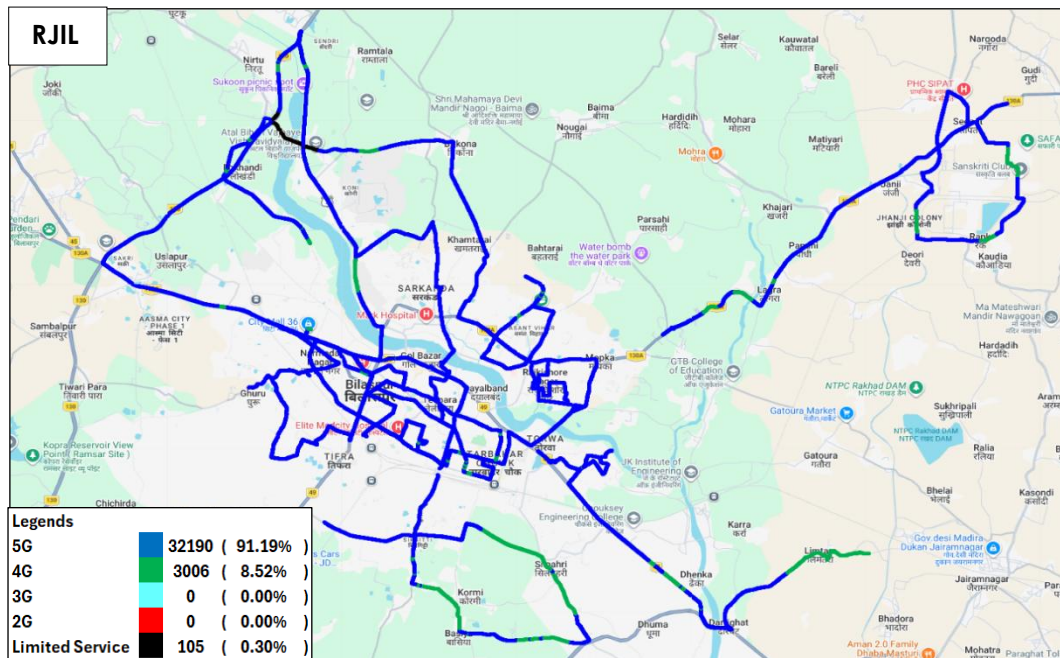
Figure-44: Serving technology plots in auto-selection mode (5G/4G/3G/2G) data- RJIL.
