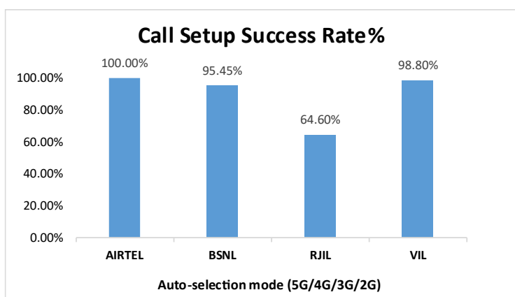
Figure-54: Performance for call setup success rate.
