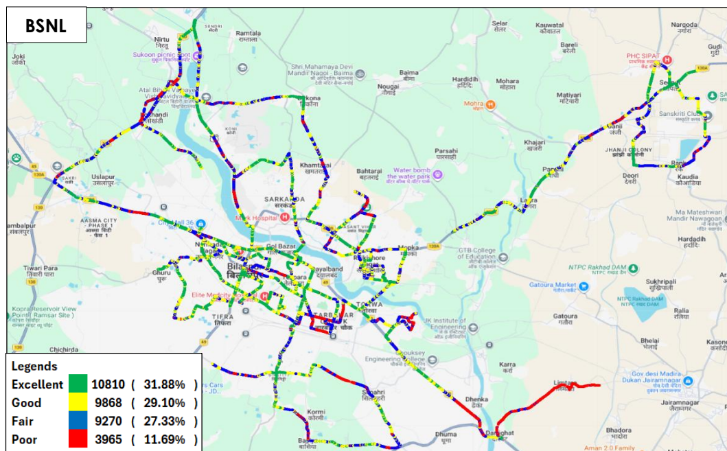
Figure-89: Signal strength 3G/2G network mode voice - BSNL.
