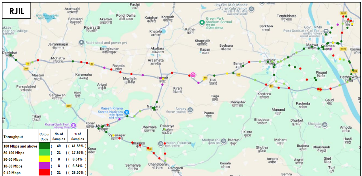
Figure-75: Download throughput distribution auto-selection mode (5G/4G/3G/2G) - RJIL.
