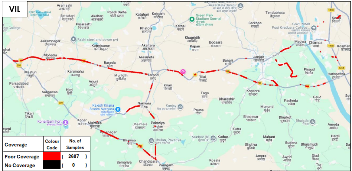
Figure-71: Poor coverage & no coverage locations in auto-selection mode (5G/4G/3G/2G) voice-VIL.
