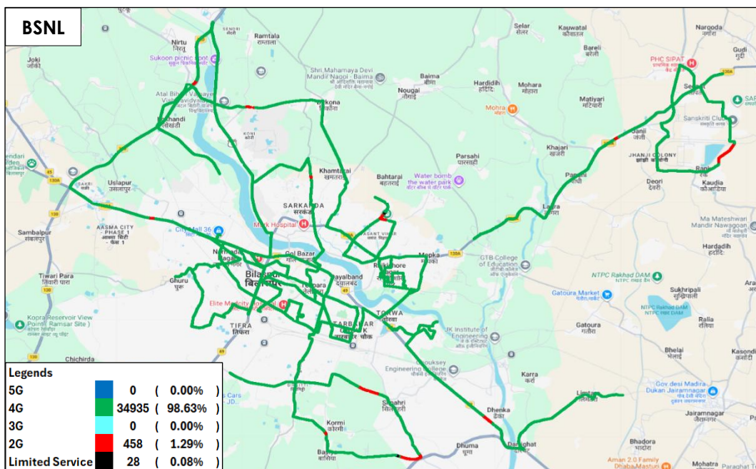
Figure-43: Serving technology plots in auto-selection mode (5G/4G/3G/2G) data-BSNL.
