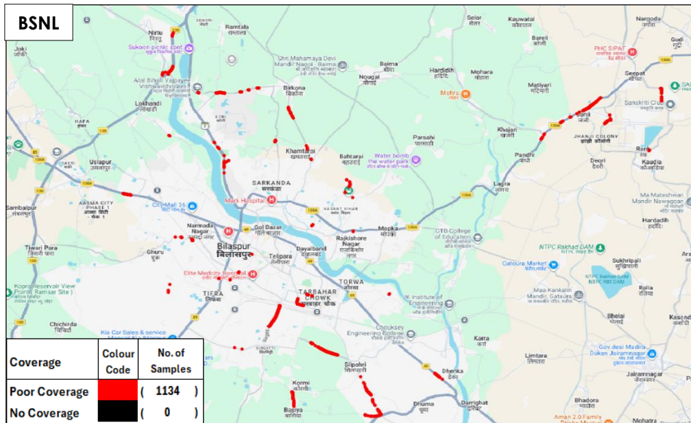
Figure-30: Poor coverage & no coverage locations in auto-selection mode (5G/4G/3G/2G) voice-BSNL.
