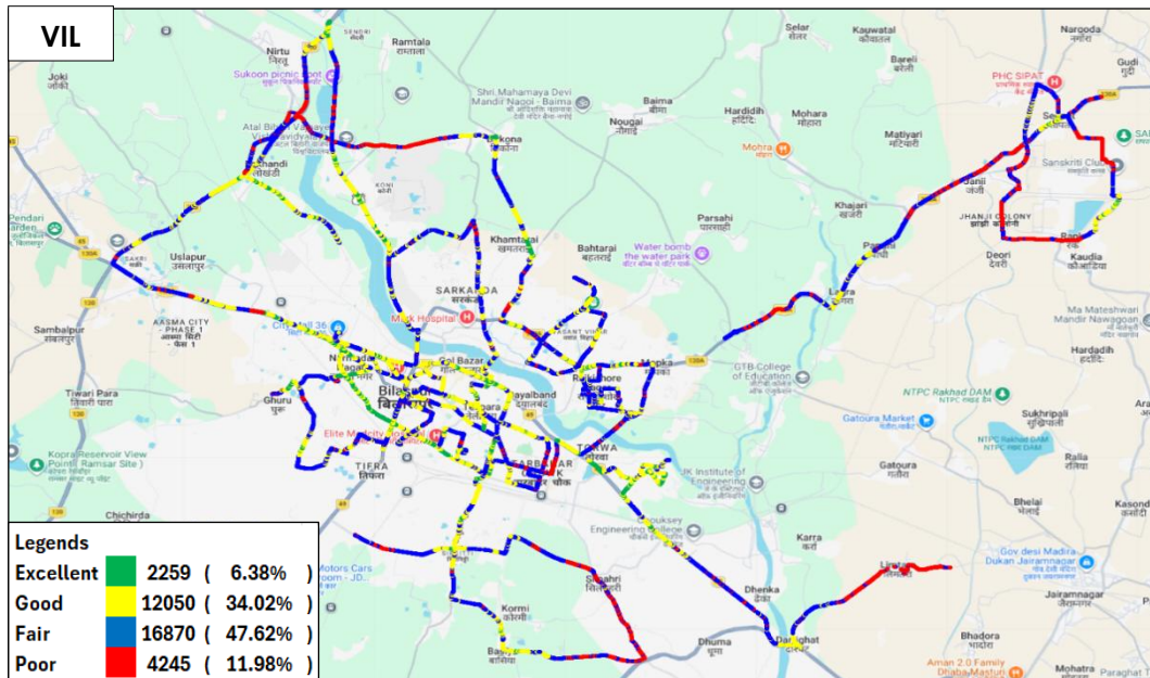
Figure-98: Signal strength auto-selection mode (5G/4G/3G/2G) data - VIL.
