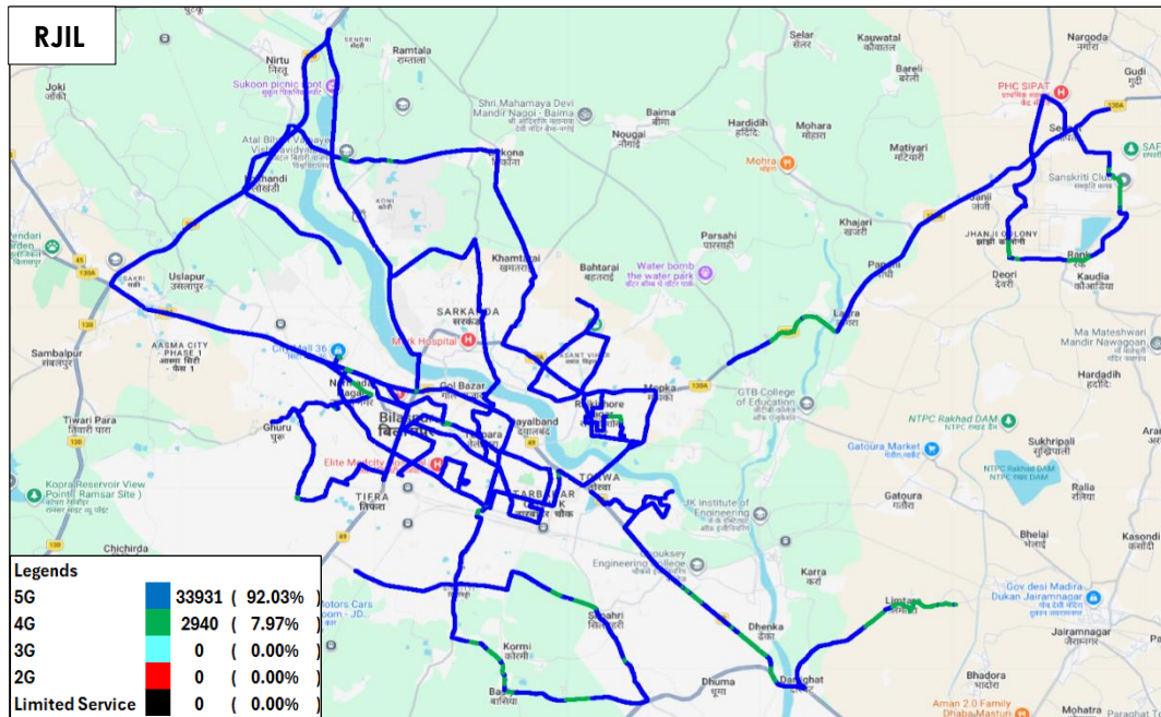
Figure-26: Serving technology plots in auto-selection mode (5G/4G/3G/2G) voice - RJIL.
