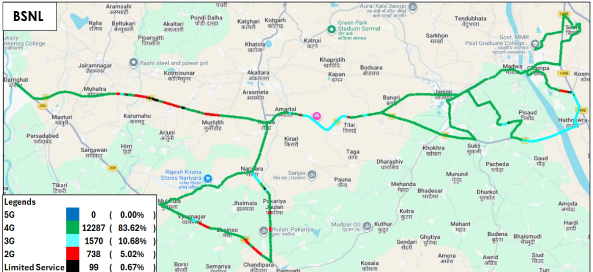
Figure-64: Serving technology plots in auto-selection mode (5G/4G/3G/2G) voice - BSNL.
