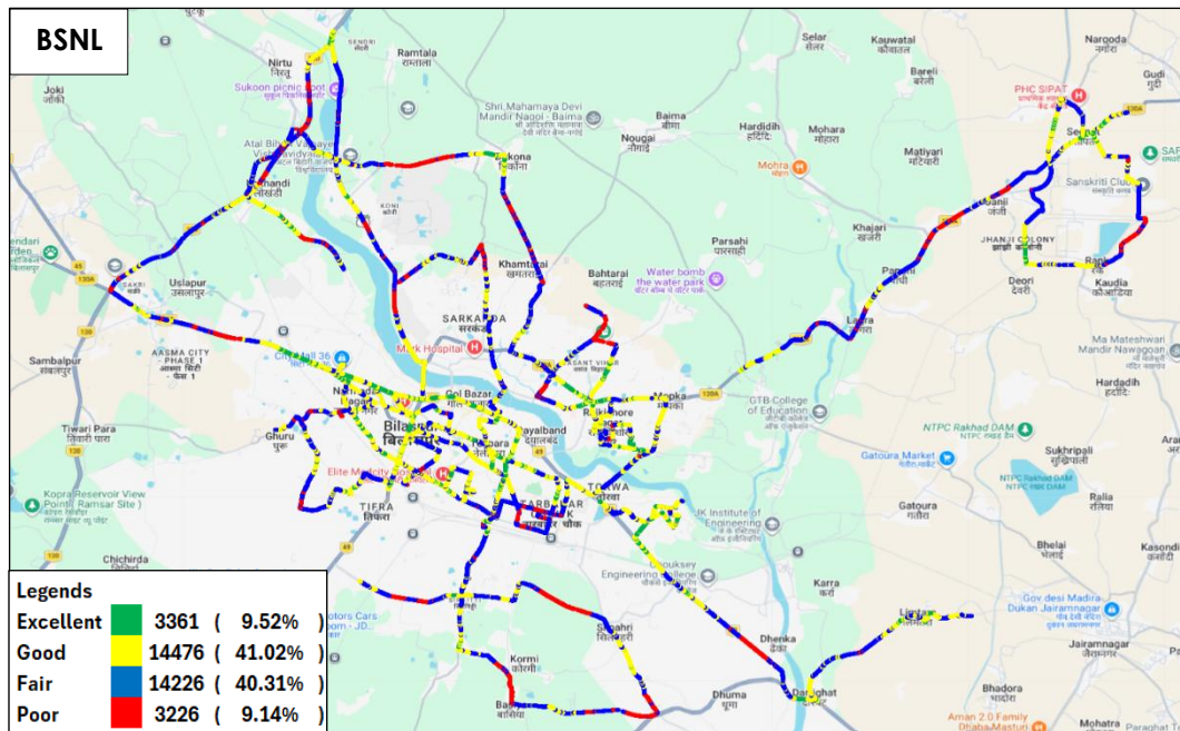
Figure-96: Signal strength auto-selection mode (5G/4G/3G/2G) data - BSNL.
