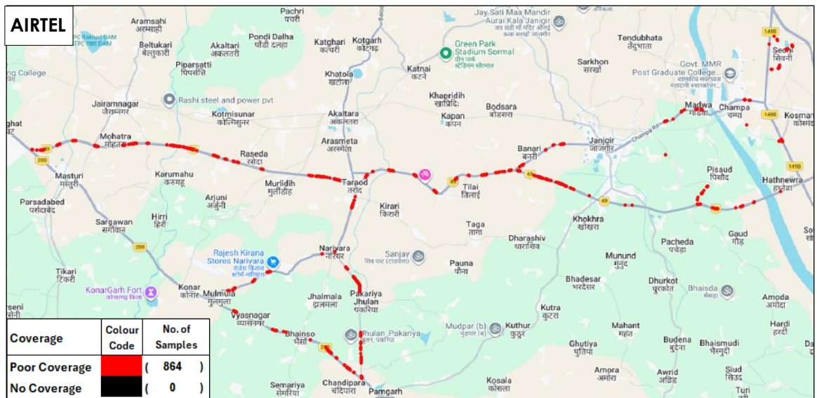
Figure-68: Poor coverage & no coverage locations in auto-selection mode (5G/4G/3G/2G) voice-AIRTEL.
