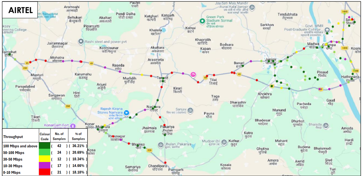
Figure-73: Download throughput distribution auto-selection mode (5G/4G/3G/2G) - AIRTEL.
