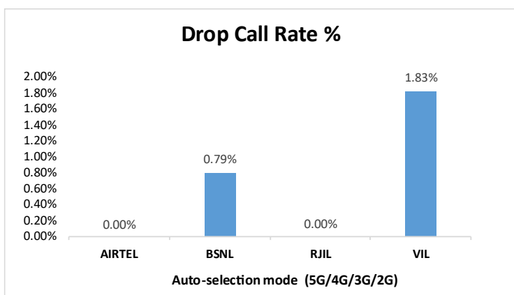
Figure-55: Performance for drop call rate.
