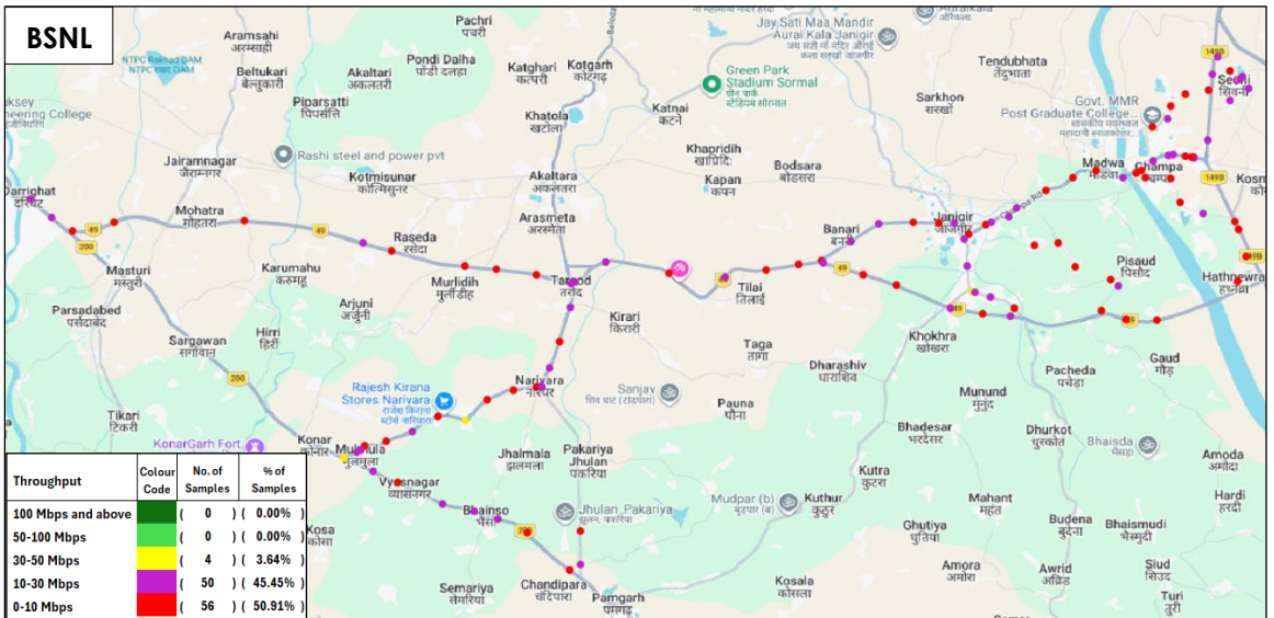
Figure-74: Download throughput distribution auto-selection mode (5G/4G/3G/2G) - BSNL.
