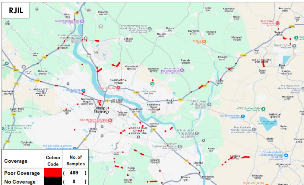
Figure-31: Poor coverage & no coverage locations in auto-selection mode (5G/4G/3G/2G) voice-RJIL.
