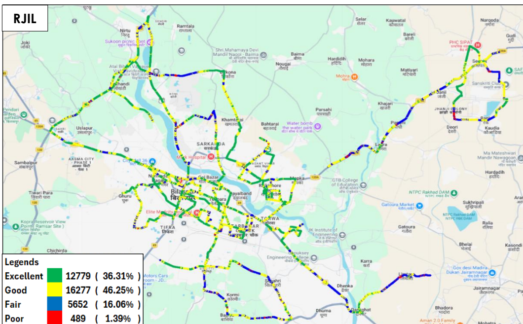
Figure-93: Signal strength auto-selection mode (5G/4G/3G/2G) voice - RJIL.
