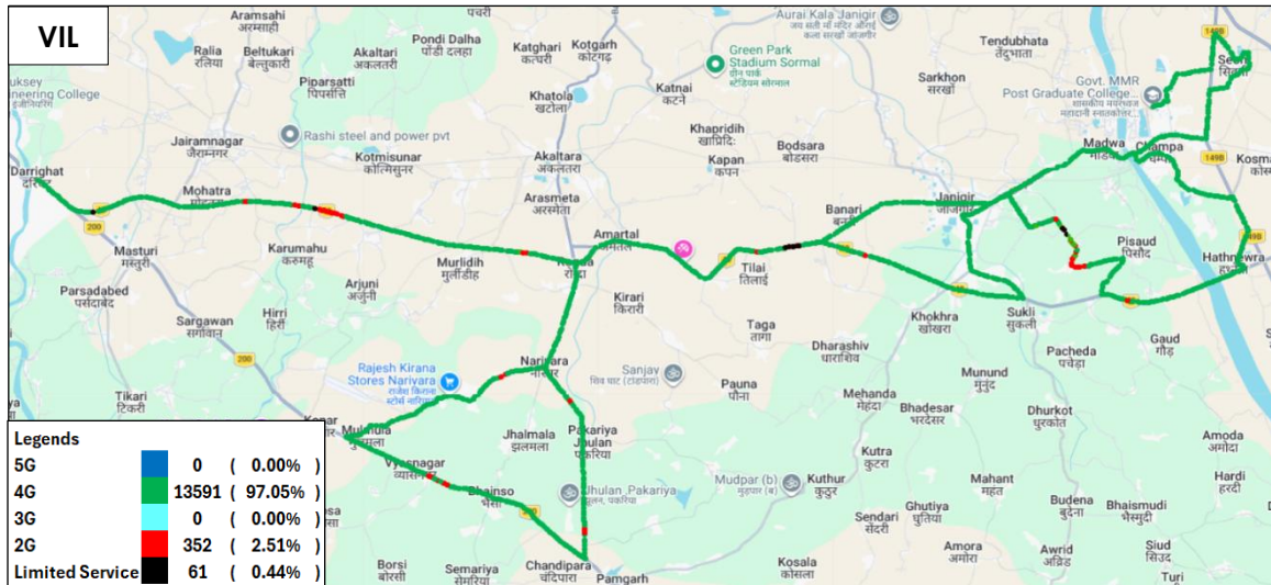
Figure-84: Serving technology plots in auto-selection mode (5G/4G/3G/2G) data- VIL.
