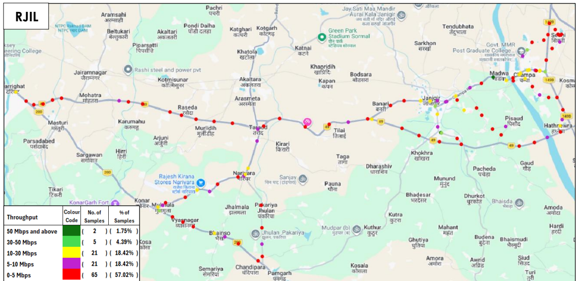
Figure-79: Upload throughput distribution auto-selection mode (5G/4G/3G/2G) - RJIL.
