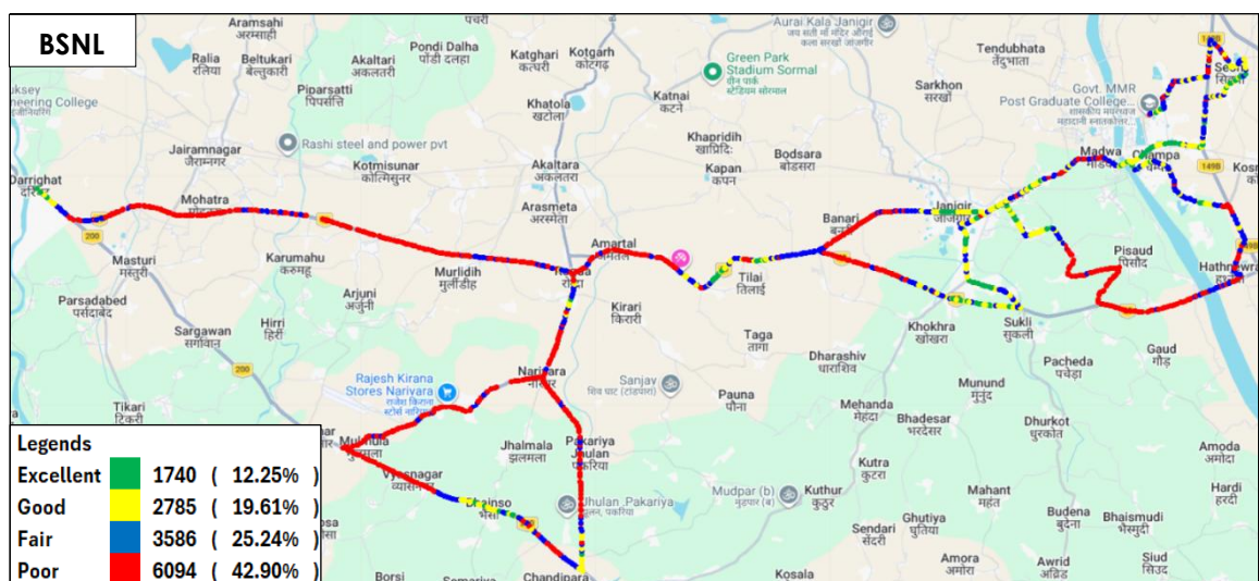
Figure-100: Signal strength 3G/2G network mode voice - BSNL.
