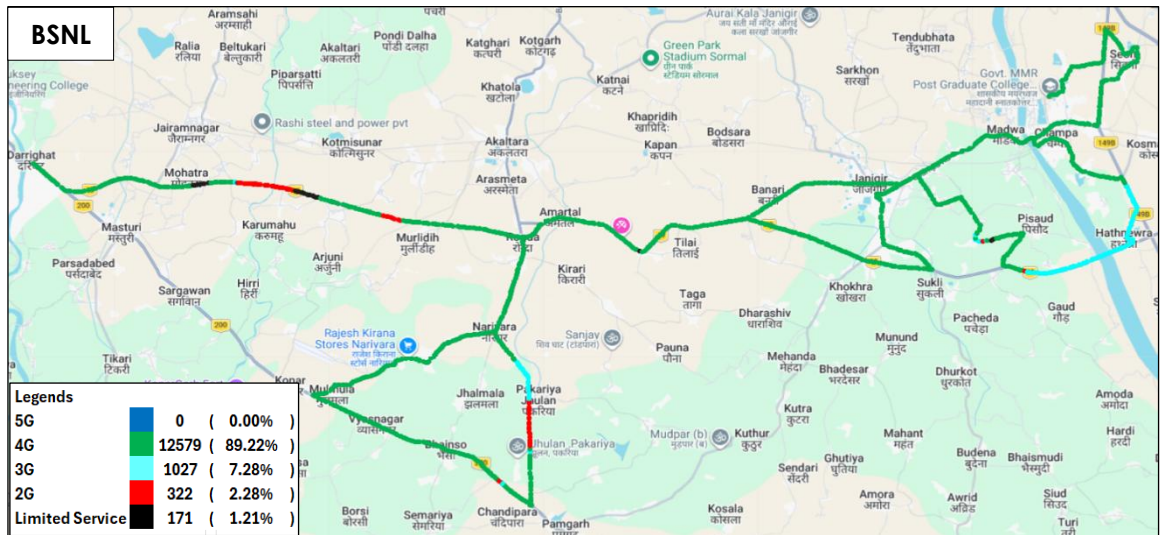
Figure-82: Serving technology plots in auto-selection mode (5G/4G/3G/2G) data-BSNL.
