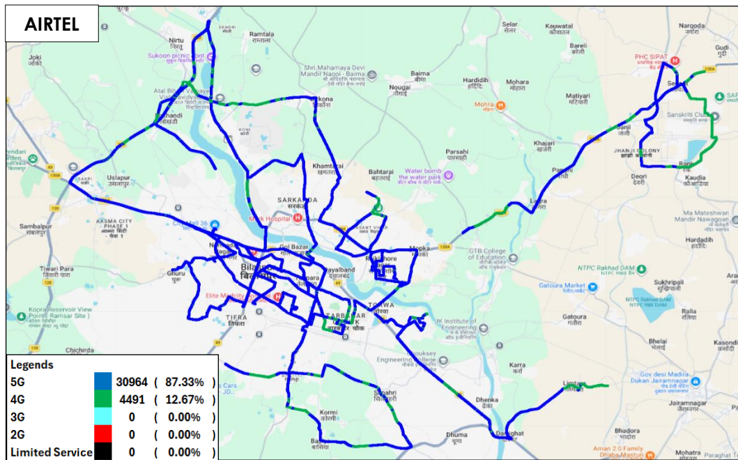
Figure-42: Serving technology plots in auto-selection mode (5G/4G/3G/2G) data -AIRTEL.
