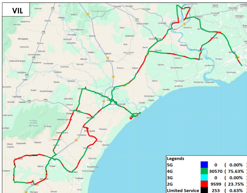
Figure-45: Serving technology plots in auto-selection mode (5G/4G/3G/2G) data – VIL.
