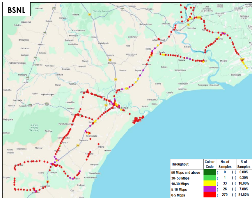
Figure-39: Upload throughput distribution auto-selection mode (5G/4G/3G/2G) – BSNL.
