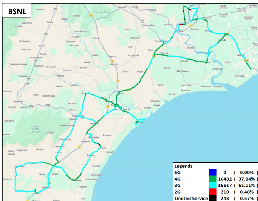
Figure-43: Serving technology plots in auto-selection mode (5G/4G/3G/2G) data – BSNL.
