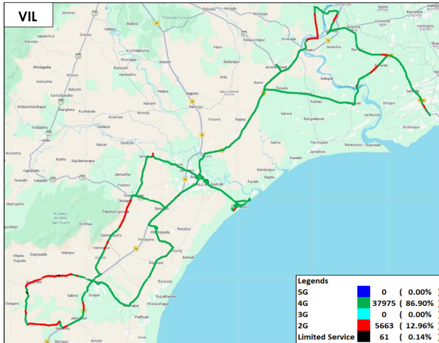
Figure-27: Serving technology plots in auto-selection mode (5G/4G/3G/2G) voice – VIL.
