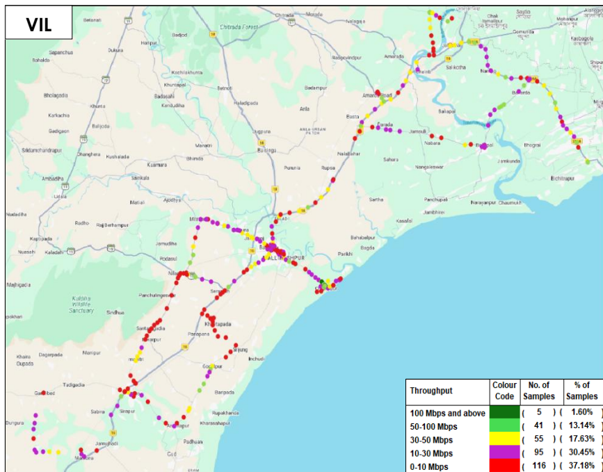
Figure-37: Download throughput distribution auto-selection mode (5G/4G/3G/2G) – VIL.
