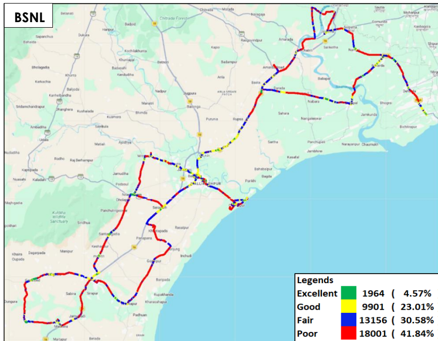
Figure-56: Signal strength auto-selection mode (5G/4G/3G/2G) data - BSNL.
