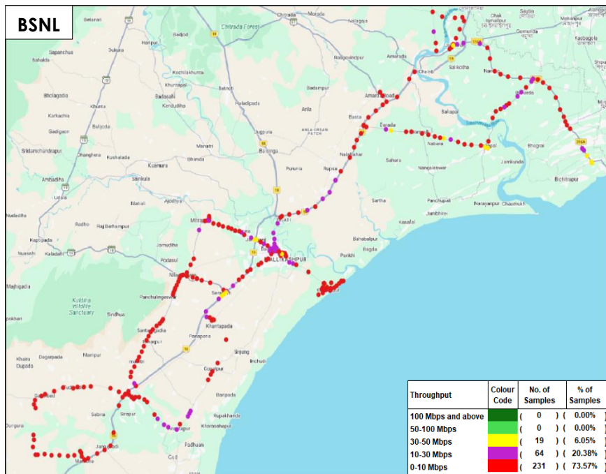
Figure-35: Download throughput distribution auto-selection mode (5G/4G/3G/2G) – BSNL.
