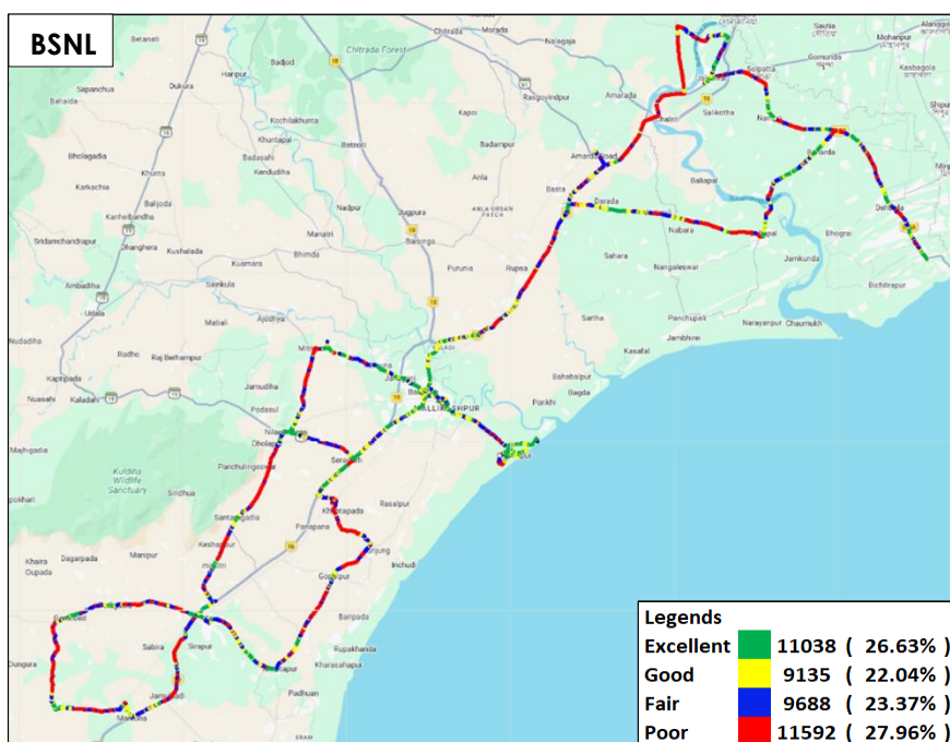
Figure-49: Signal strength 3G/2G network mode voice - BSNL.
