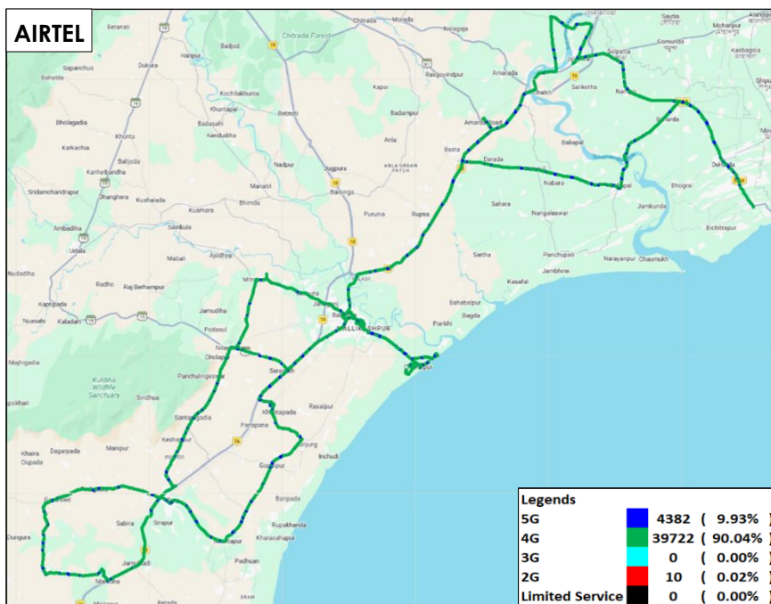
Figure-24: Serving technology plots in auto-selection mode (5G/4G/3G/2G) voice - AIRTEL.
