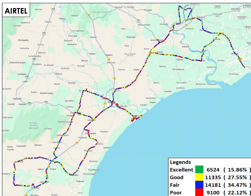
Figure-48: Signal strength 3G/2G network mode voice - AIRTEL.
