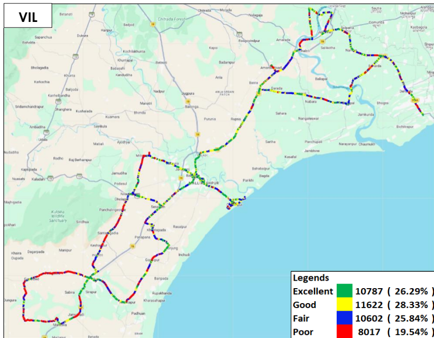
Figure-50: Signal strength 3G/2G network mode voice - VIL.
