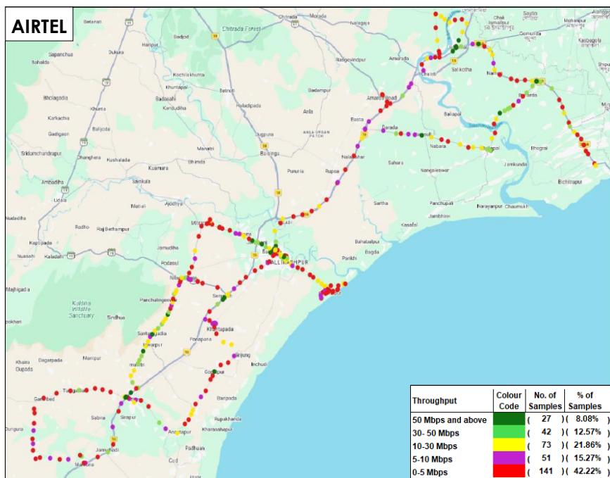
Figure-38: Upload throughput distribution auto-selection mode (5G/4G/3G/2G) – AIRTEL.
