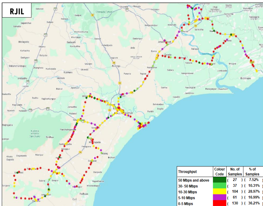
Figure-40: Upload throughput distribution auto-selection mode (5G/4G/3G/2G) – RJIL.
