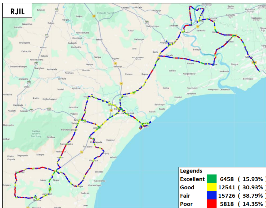
Figure-57: Signal strength auto-selection mode (5G/4G/3G/2G) data - RJIL.
