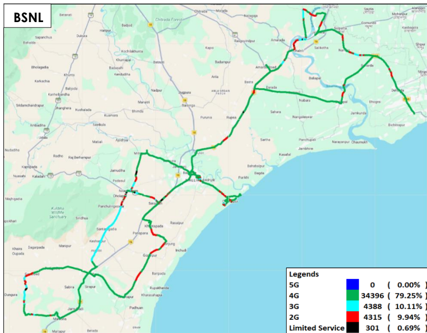
Figure-25: Serving technology plots in auto-selection mode (5G/4G/3G/2G) voice – BSNL.
