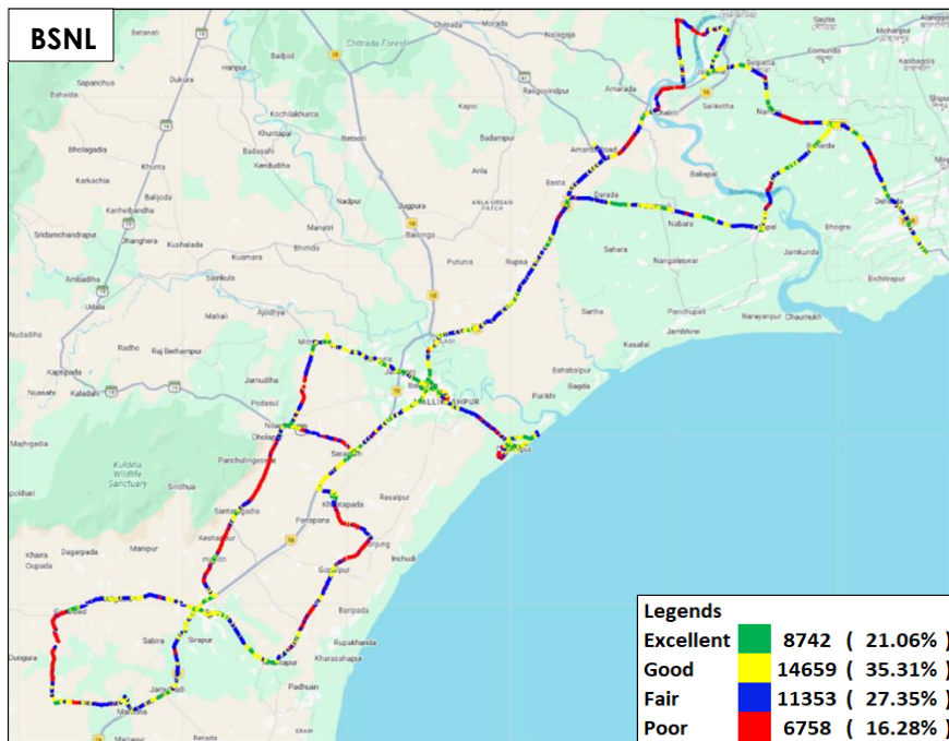
Figure-52: Signal strength auto-selection mode (5G/4G/3G/2G) voice - BSNL.
