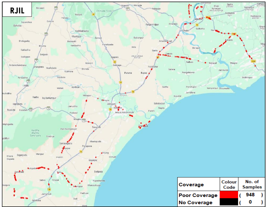
Figure-31: Poor coverage & no coverage locations in auto-selection mode (5G/4G/3G/2G) voice-RJIL.
