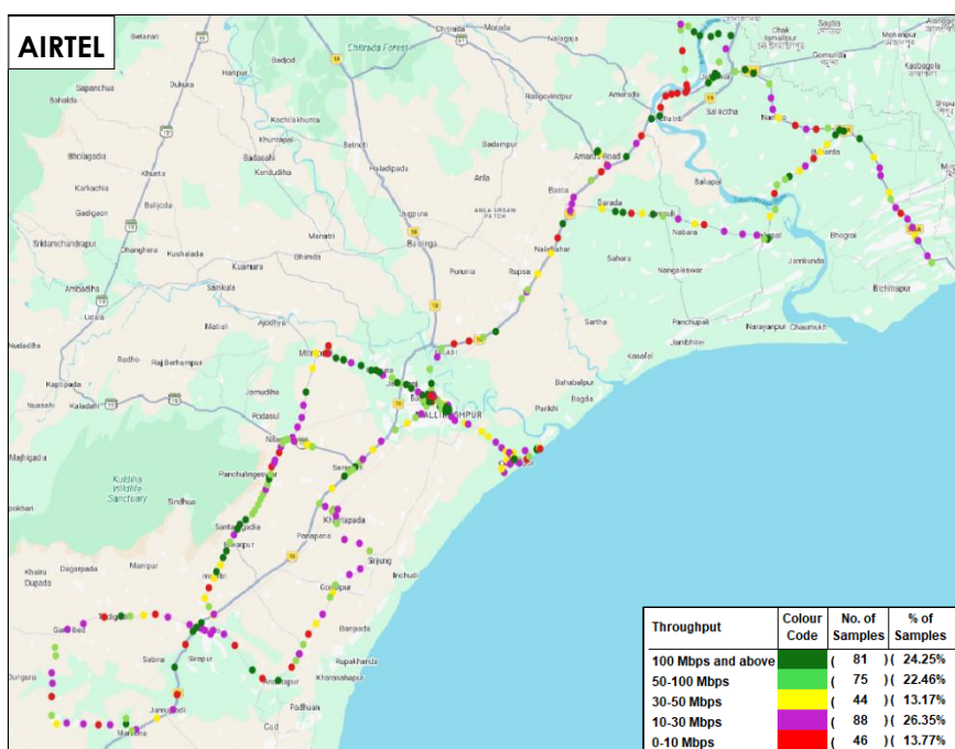
Figure-34: Download throughput distribution auto-selection mode (5G/4G/3G/2G) – AIRTEL.
