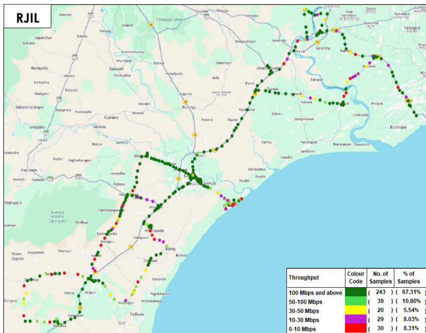
Figure-36: Download throughput distribution auto-selection mode (5G/4G/3G/2G) – RJIL.
