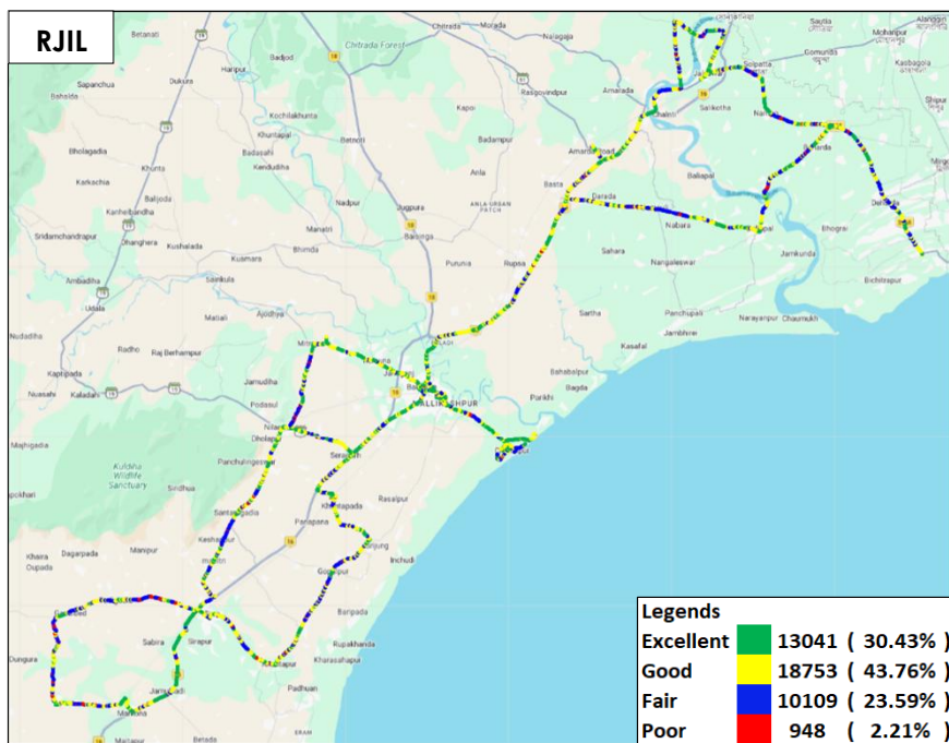
Figure-53: Signal strength auto-selection mode (5G/4G/3G/2G) voice - RJIL.
