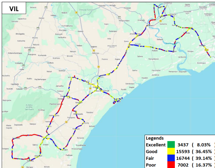
Figure-54: Signal strength auto-selection mode (5G/4G/3G/2G) voice - VIL.
