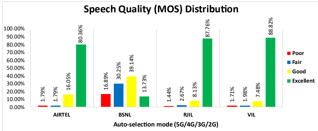
Figure-23: Distribution of samples in MOS range.
