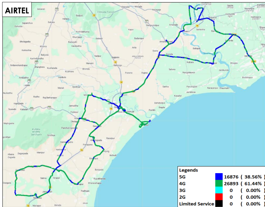
Figure-42: Serving technology plots in auto-selection mode (5G/4G/3G/2G) data – AIRTEL.
