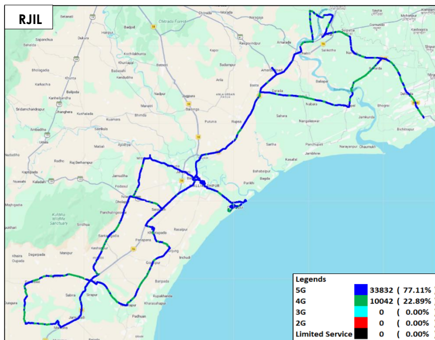
Figure-26: Serving technology plots in auto-selection mode (5G/4G/3G/2G) voice – RJIL.
