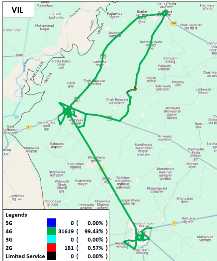
Figure-25: Serving technology plots in auto-selection mode (5G/4G/3G/2G) voice - VIL.
