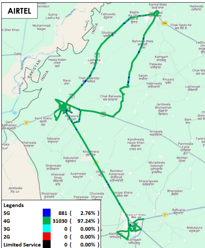
Figure-22: Serving technology plots in auto-selection mode (5G/4G/3G/2G) voice - AIRTEL.
