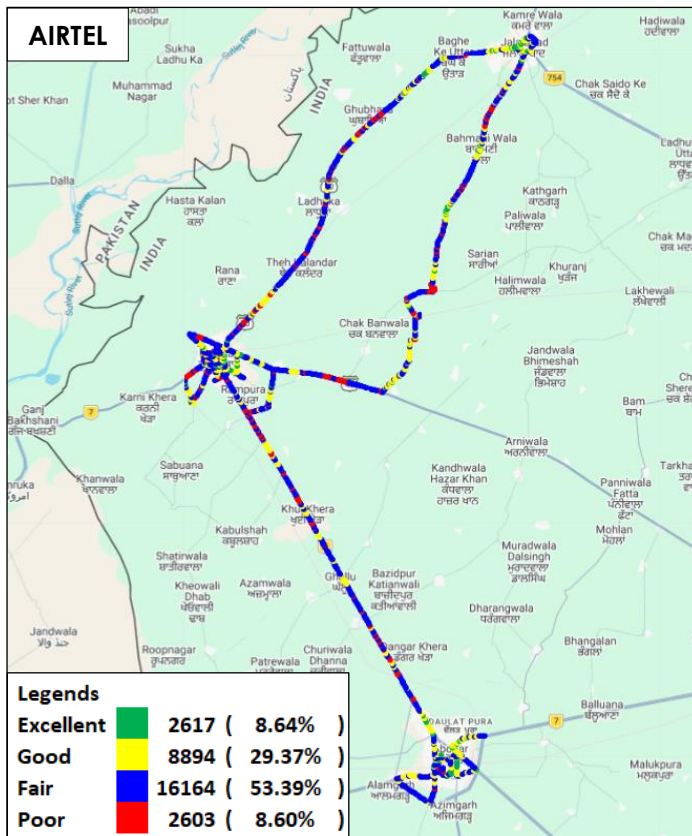
Figure-54: Signal strength auto-selection mode (5G/4G/3G/2G) data - AIRTEL.
