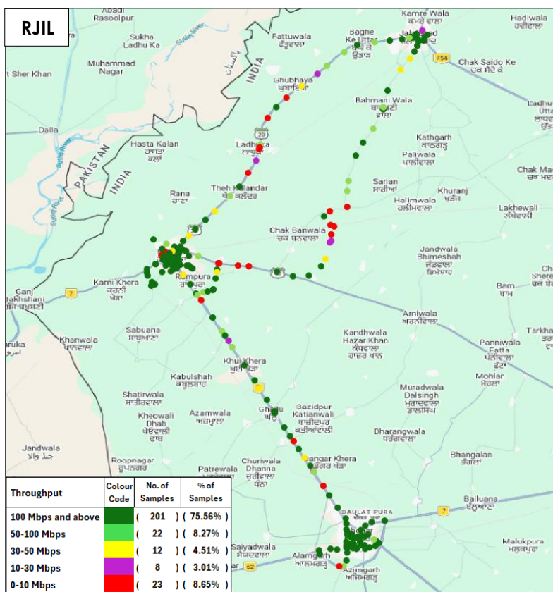
Figure-34: Download throughput distribution auto-selection mode (5G/4G/3G/2G) - RJIL.
