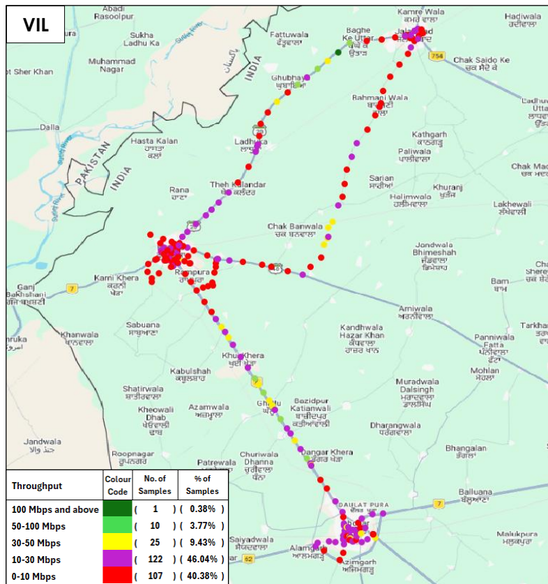
Figure-35: Download throughput distribution auto-selection mode (5G/4G/3G/2G) - VIL.
