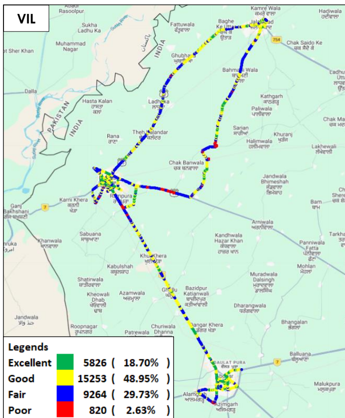
Figure-53: Signal strength auto-selection mode (5G/4G/3G/2G) voice - VIL.
