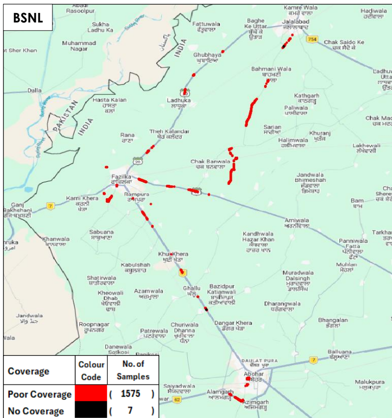
Figure-28: Poor coverage & no coverage locations in auto-selection mode 5G/4G/3G/2G voice- BSNL.
