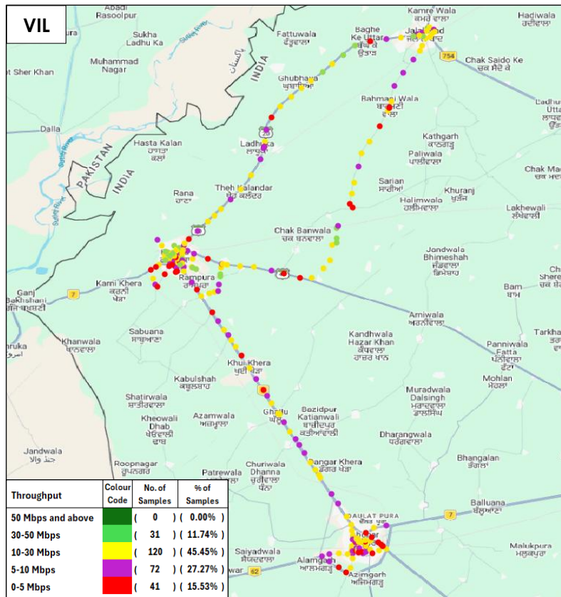
Figure-39: Upload throughput distribution auto-selection mode (5G/4G/3G/2G) - VIL.
