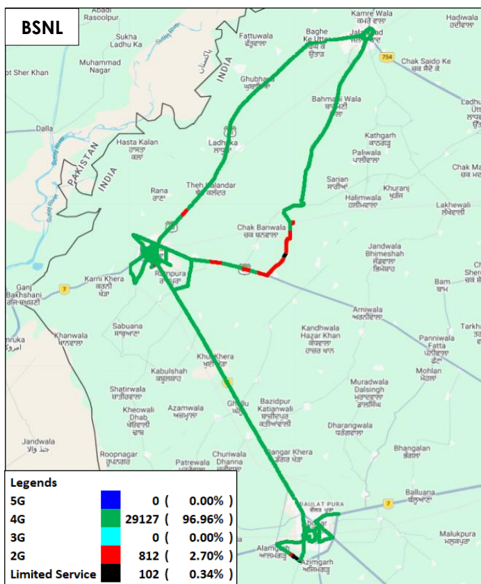
Figure-41: Serving technology plots in auto-selection mode (5G/4G/3G/2G) data-BSNL.
