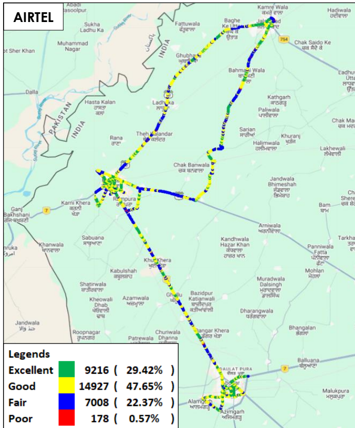
Figure-50: Signal strength auto-selection mode (5G/4G/3G/2G) voice - AIRTEL.
