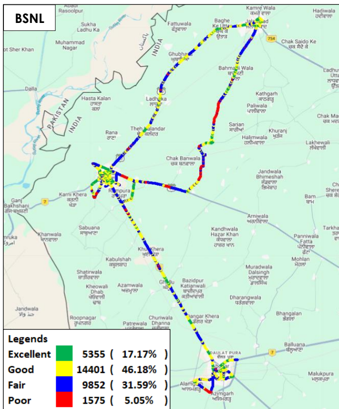
Figure-51: Signal strength auto-selection mode (5G/4G/3G/2G) voice - BSNL.
