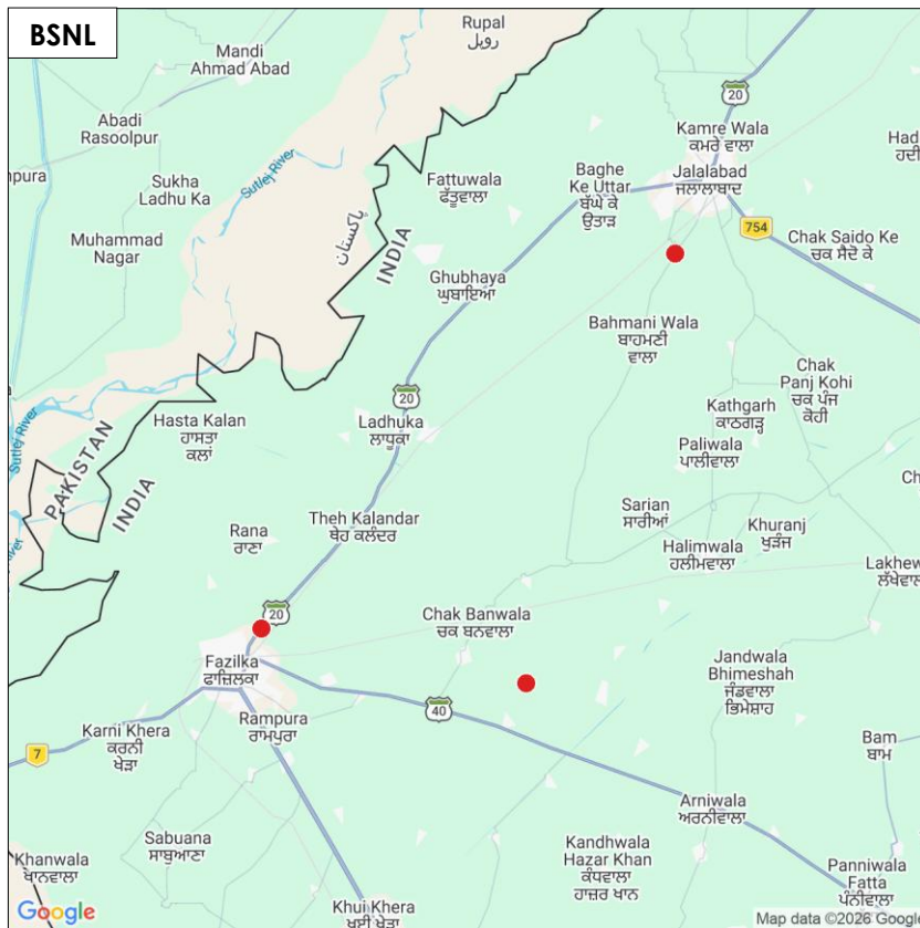
Figure-15: Drop call locations in auto-selection mode (5G/4G/3G/2G) voice - BSNL.
