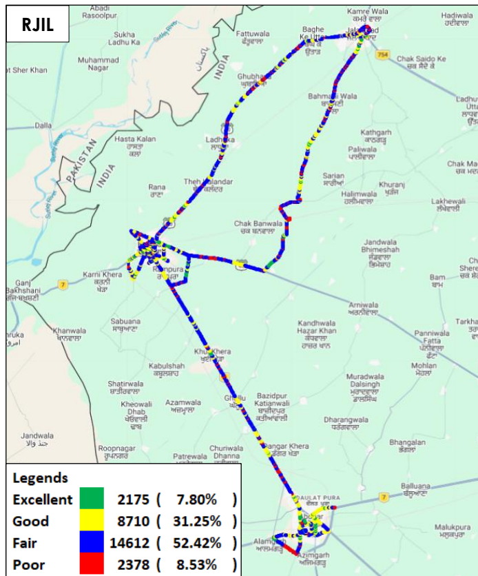
Figure-56: Signal strength auto-selection mode (5G/4G/3G/2G) data - RJIL.
