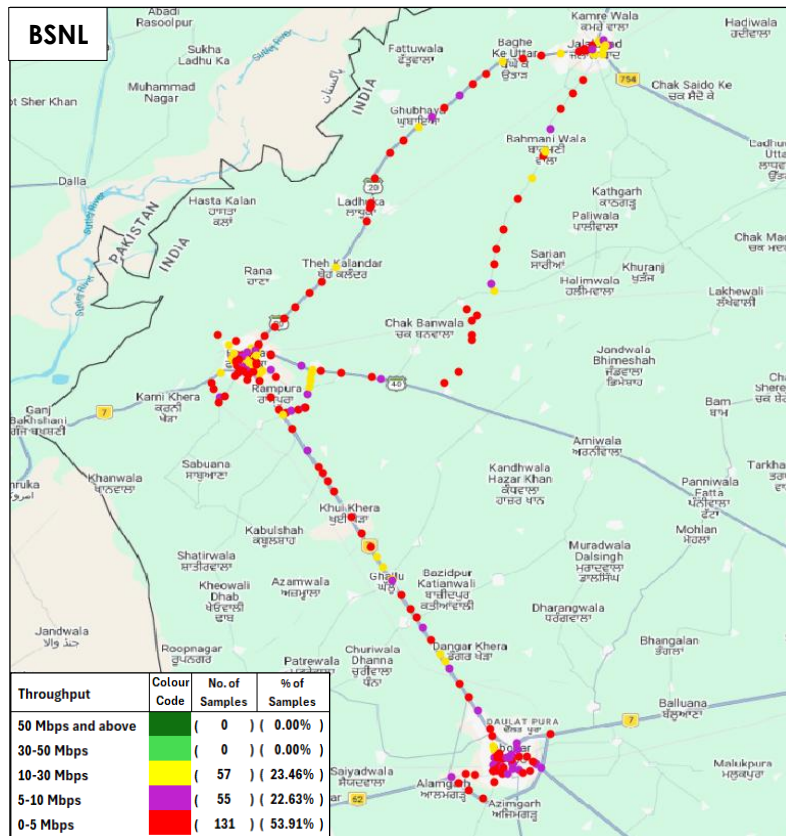
Figure-37: Upload throughput distribution auto-selection mode (5G/4G/3G/2G) - BSNL.
