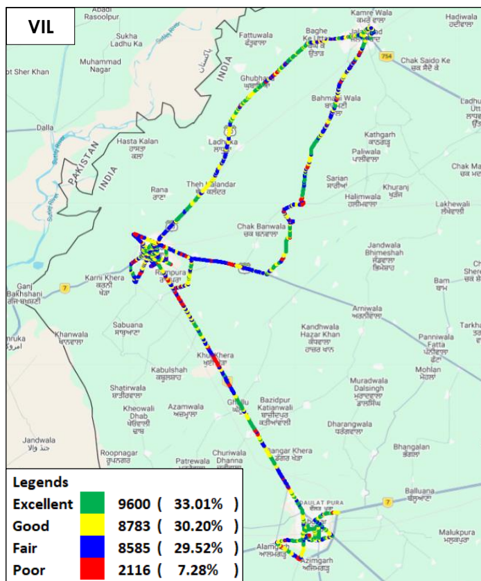
Figure-49: Signal strength 3G/2G network mode voice - VIL.
