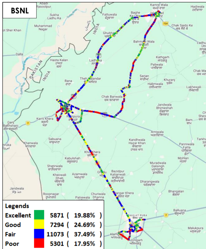
Figure-48: Signal strength 3G/2G network mode voice - BSNL.
