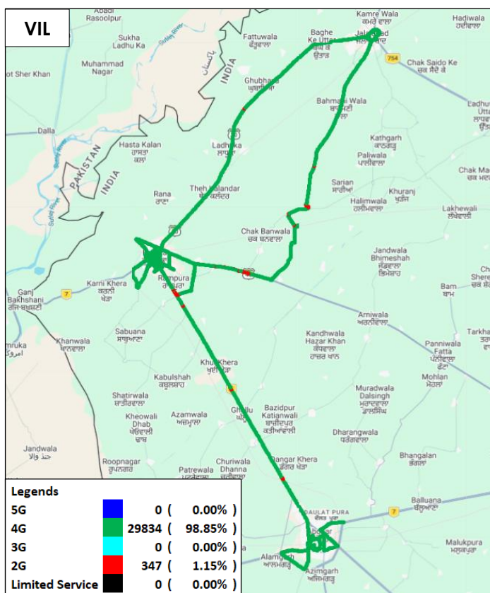
Figure-43: Serving technology plots in auto-selection mode (5G/4G/3G/2G) data- VIL.
