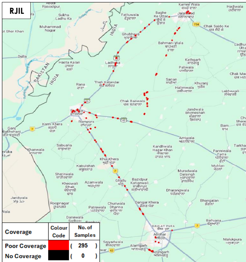
Figure-29: Poor coverage & no coverage locations in auto-selection mode 5G/4G/3G/2G voice- RJIL.
