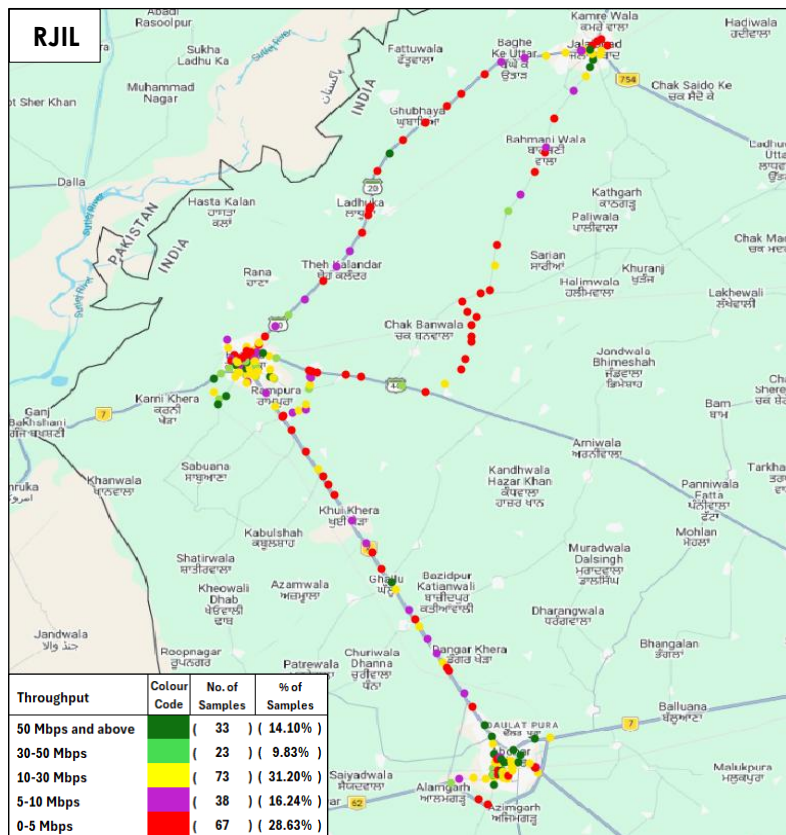
Figure-38: Upload throughput distribution auto-selection mode (5G/4G/3G/2G) - RJIL.
