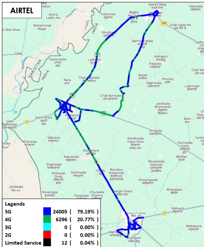
Figure-40: Serving technology plots in auto-selection mode (5G/4G/3G/2G) data -AIRTEL.
