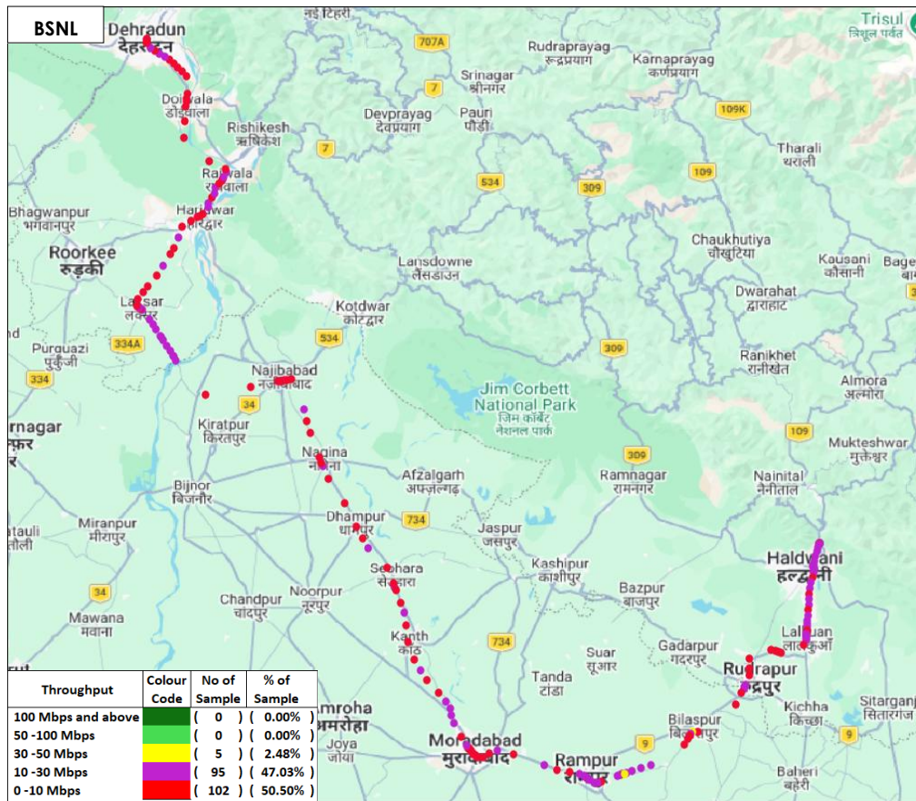
Figure-22: Download throughput distribution auto-selection mode (5G/4G/3G/2G) - BSNL.
