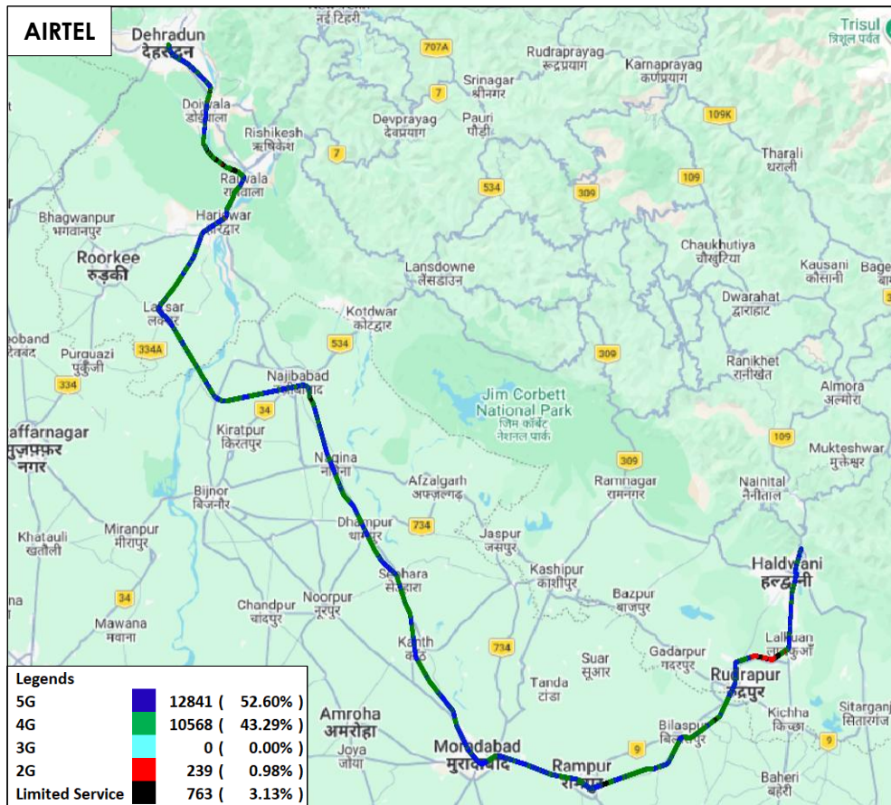
Figure-29: Serving technology plot in auto-selection mode (5G/4G/3G/2G) data – AIRTEL.
