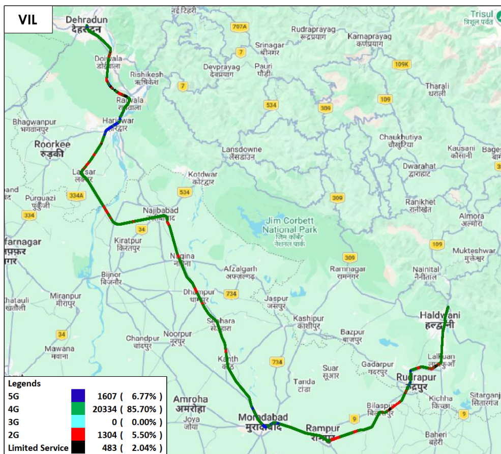
Figure-32: Serving technology plot in auto-selection mode (5G/4G/3G/2G) data - VIL.
