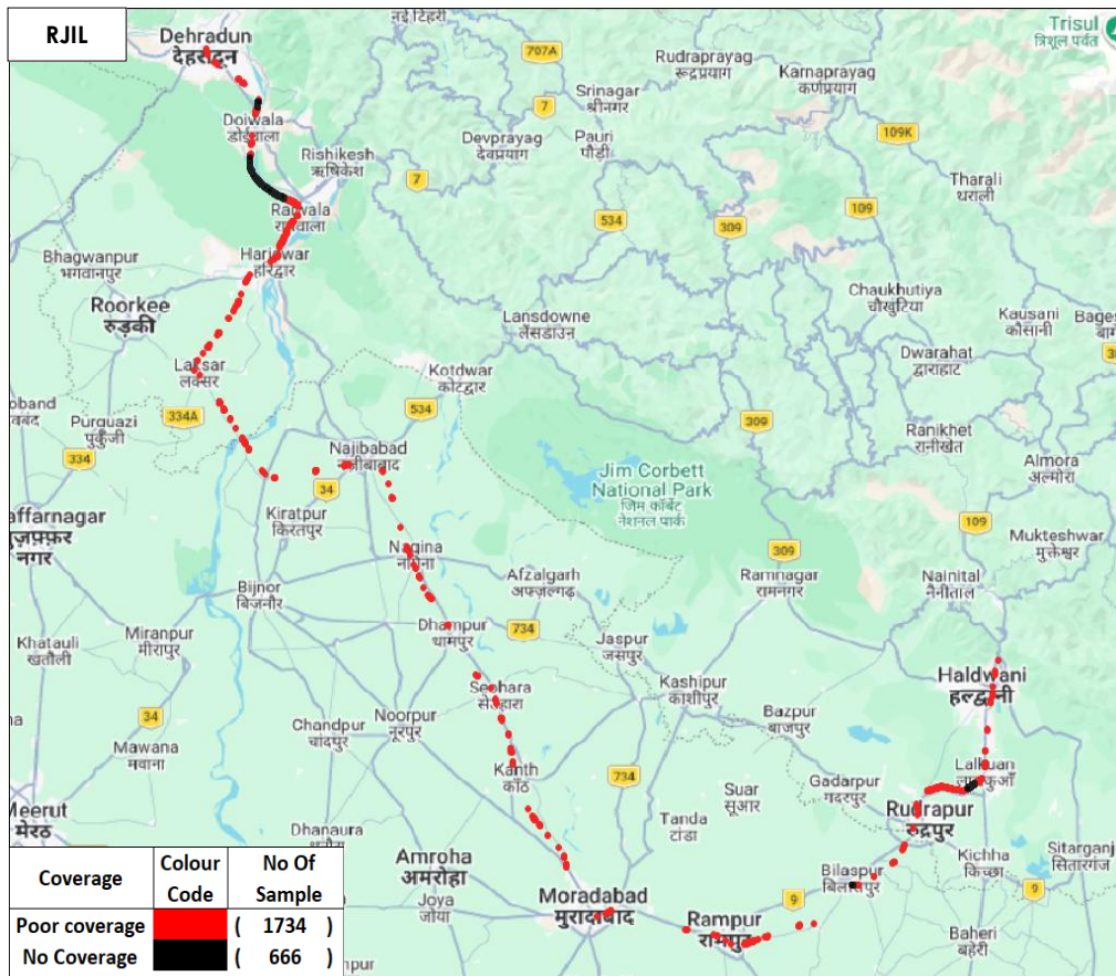
Figure-18: Poor coverage & no coverage locations in auto-selection mode (5G/4G/3G/2G) voice-RJIL.
