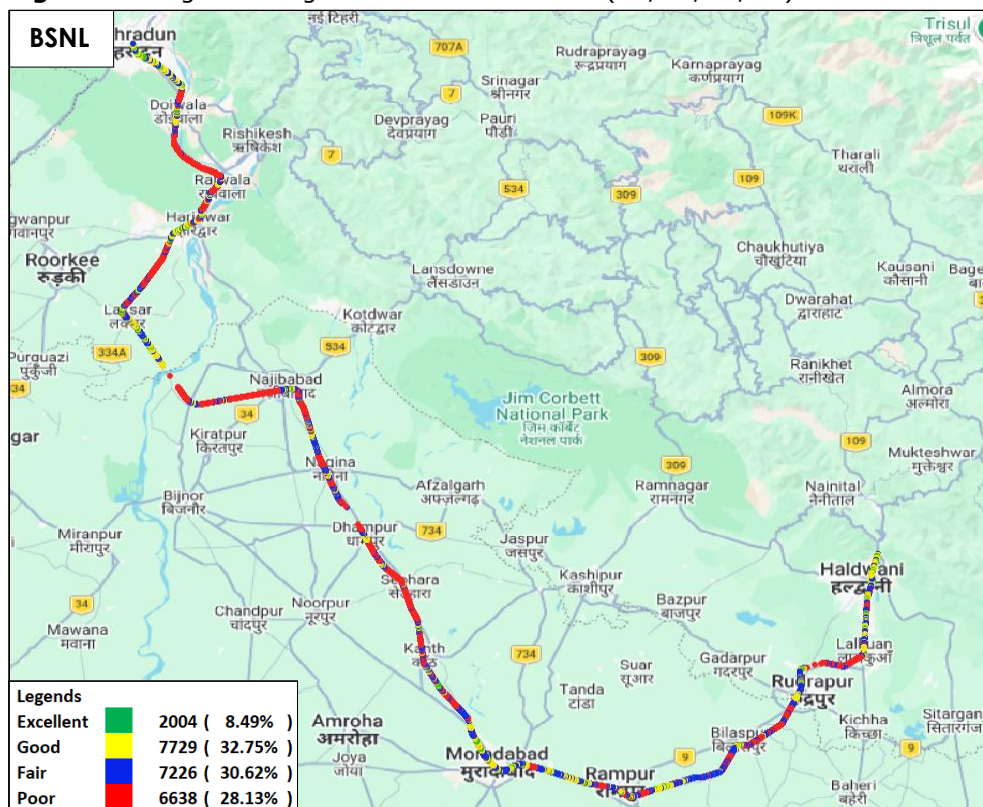
Figure-35: Signal strength auto-selection mode (5G/4G/3G/2G) voice - BSNL.
