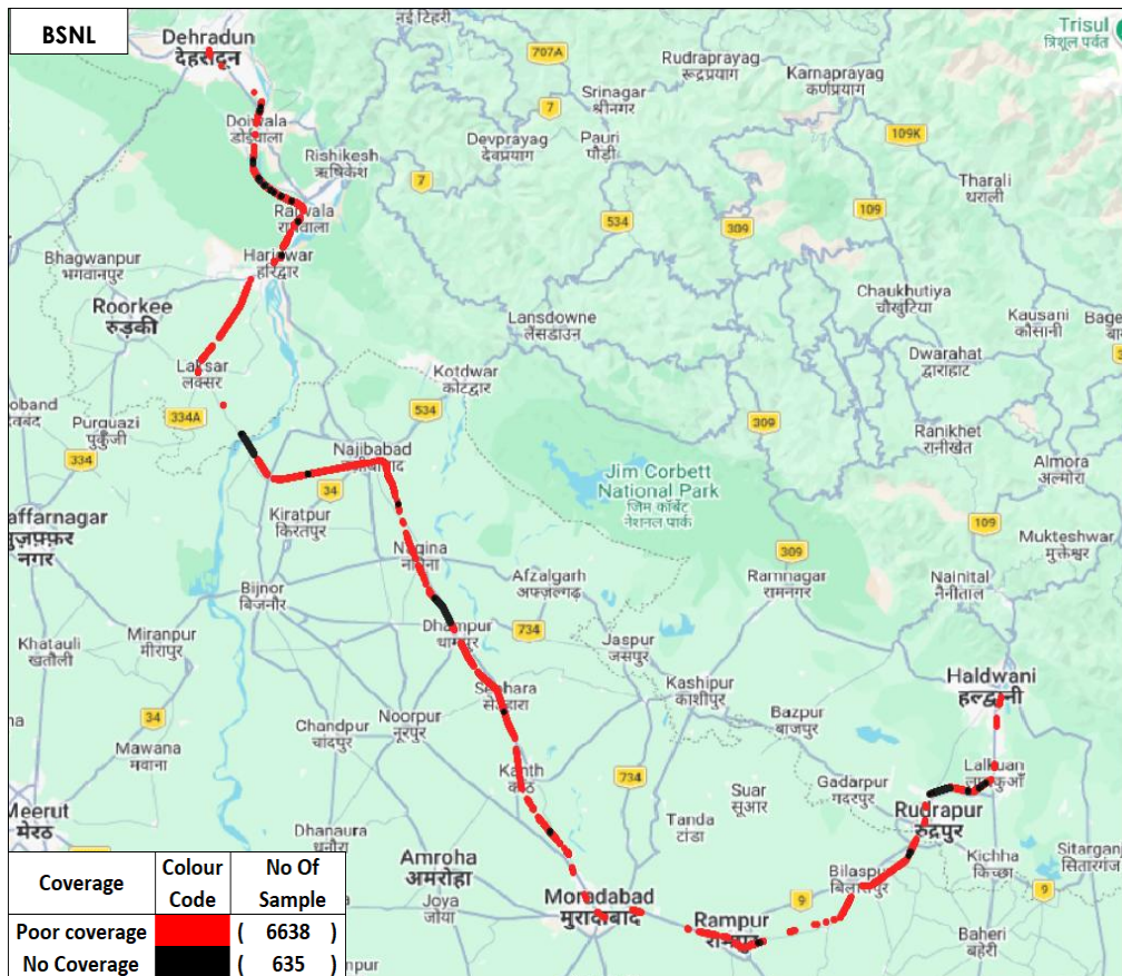
Figure-17: Poor coverage & no coverage locations in auto-selection mode (5G/4G/3G/2G) voice-BSNL.
