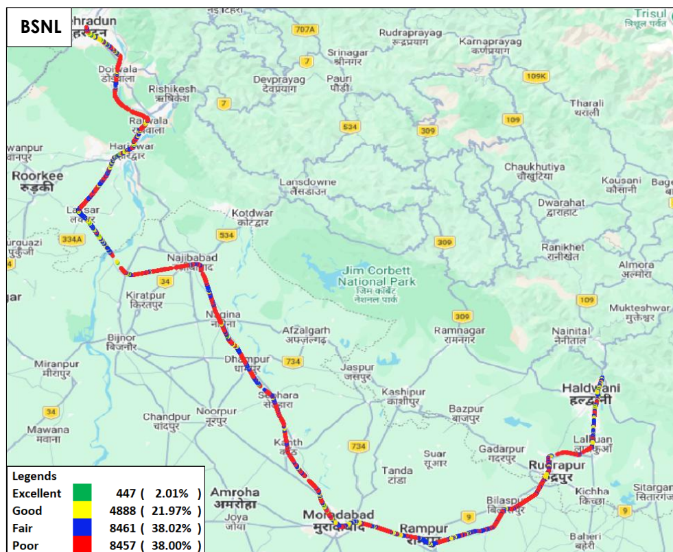
Figure-39: Signal strength auto-selection mode (5G/4G/3G/2G) data - BSNL.
