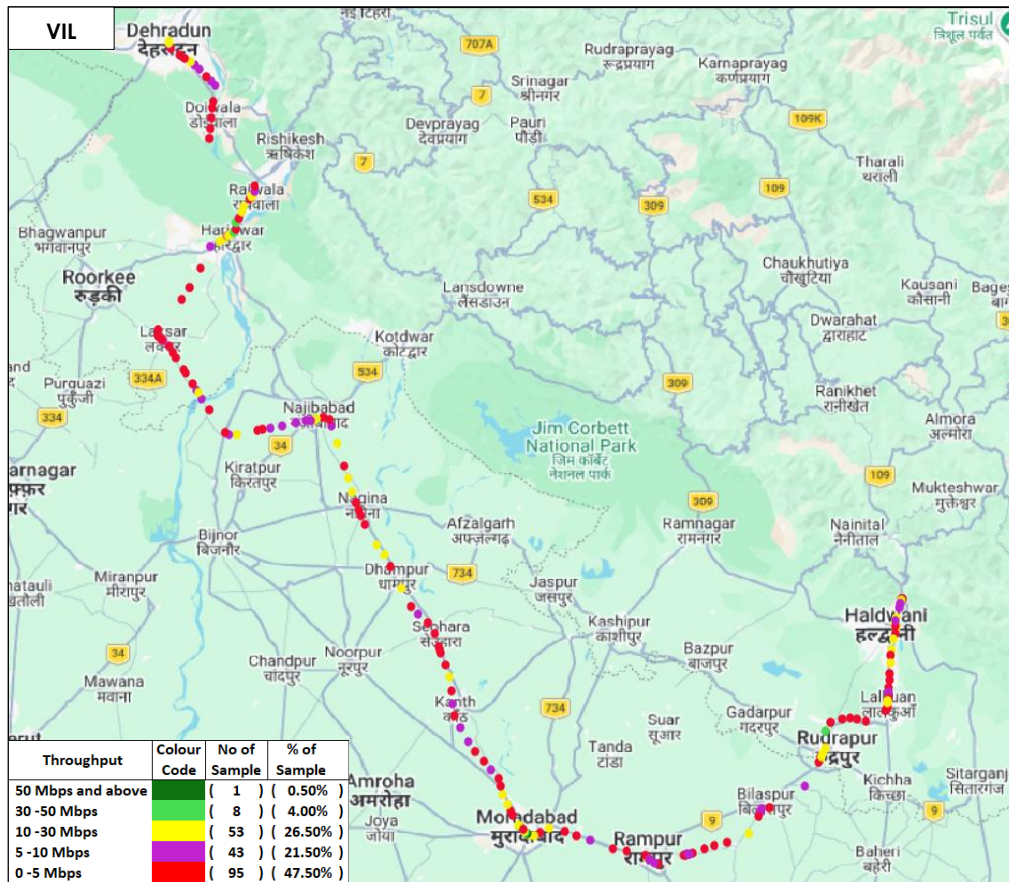
Figure-28: Upload throughput distribution auto-selection mode (5G/4G/3G/2G) - VIL.
