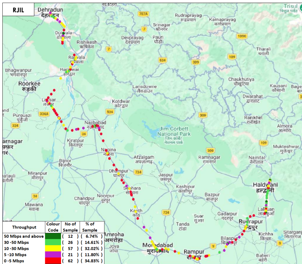
Figure-27: Upload throughput distribution auto-selection mode (5G/4G/3G/2G) - RJIL.
