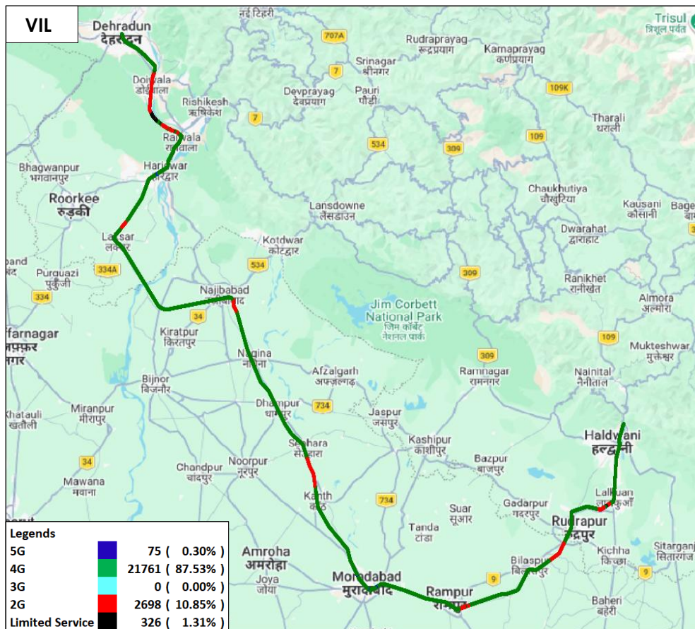
Figure-14: Serving technology plots in auto-selection mode (5G/4G/3G/2G) voice - VIL.
