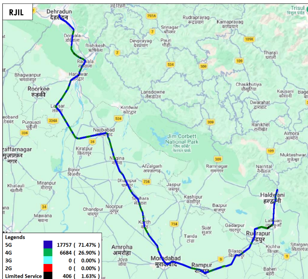
Figure-31: Serving technology plot in auto-selection mode (5G/4G/3G/2G) data - RJIL.
