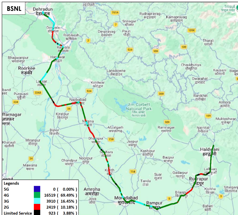
Figure-30: Serving technology plot in auto-selection mode (5G/4G/3G/2G) data - BSNL.
