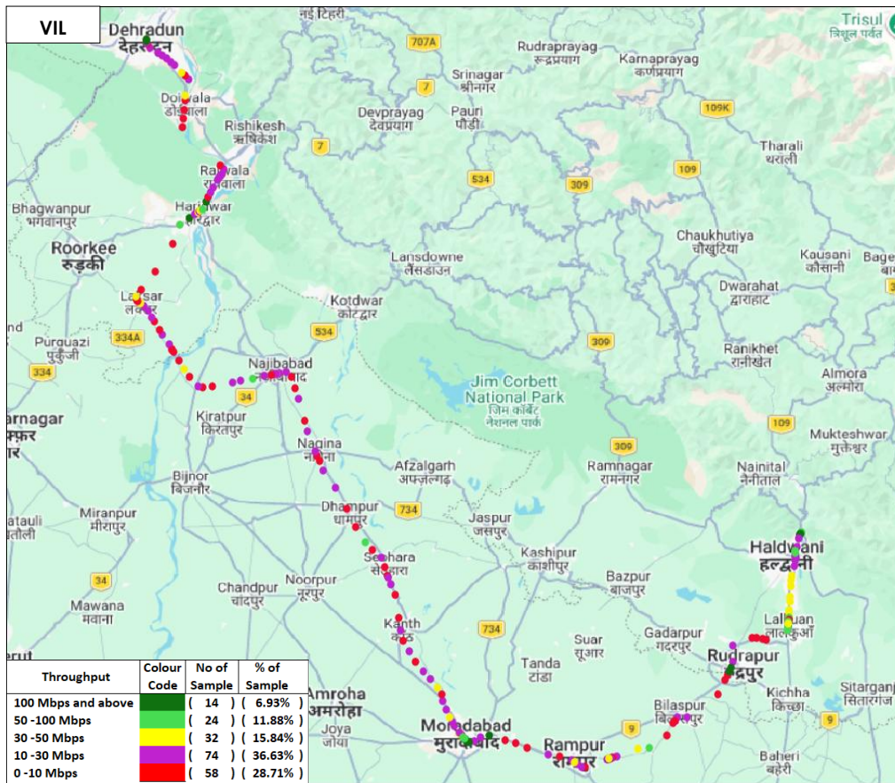
Figure-24: Download throughput distribution auto-selection mode (5G/4G/3G/2G) - VIL.
