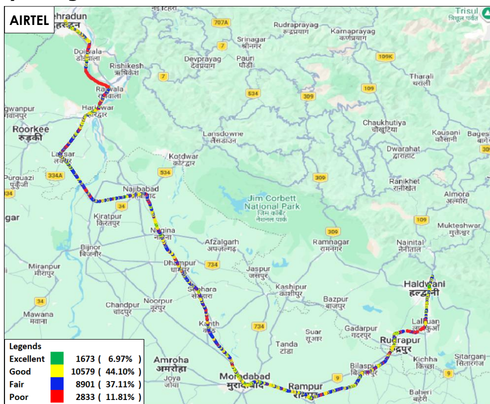
Figure-34: Signal strength auto-selection mode (5G/4G/3G/2G) voice - AIRTEL.
