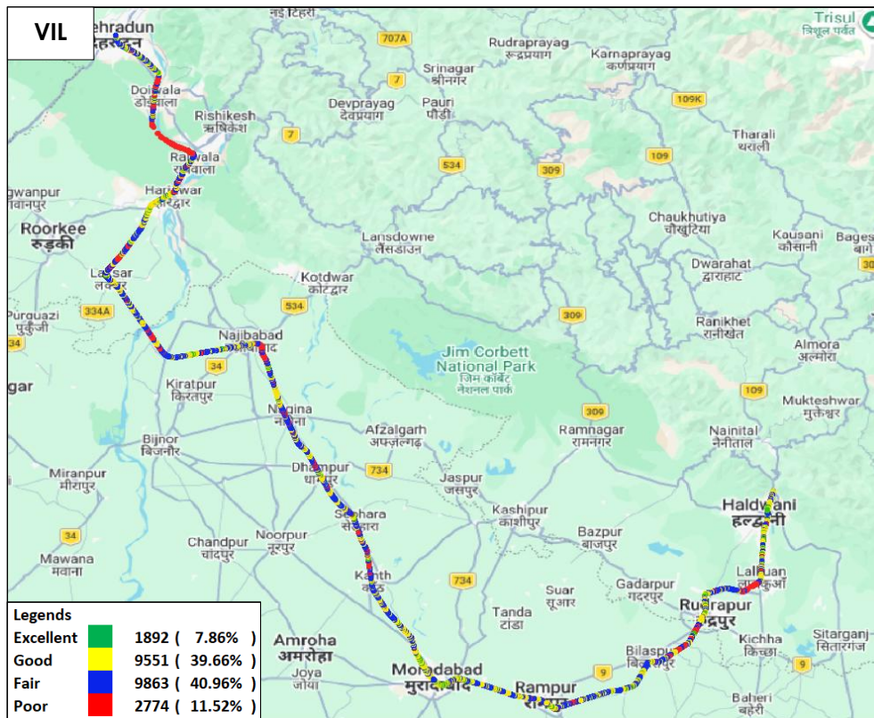
Figure-37: Signal strength auto-selection mode (5G/4G/3G/2G) voice - VIL.
