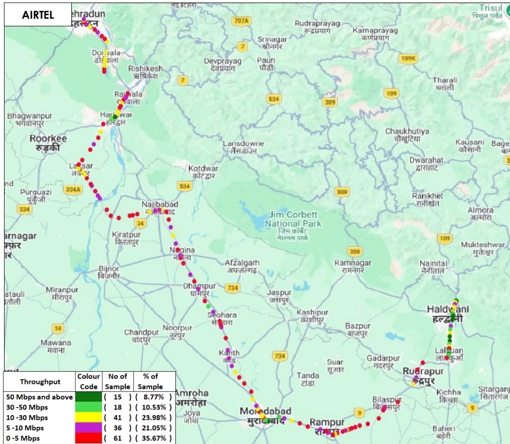
Figure-25: Upload throughput distribution auto-selection mode (5G/4G/3G/2G) - AIRTEL.
