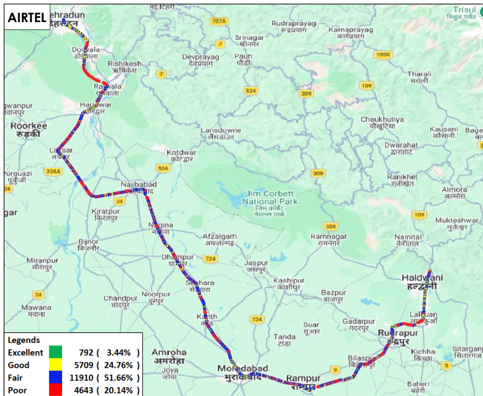
Figure-38: Signal strength auto-selection mode (5G/4G/3G/2G) data - AIRTEL.
