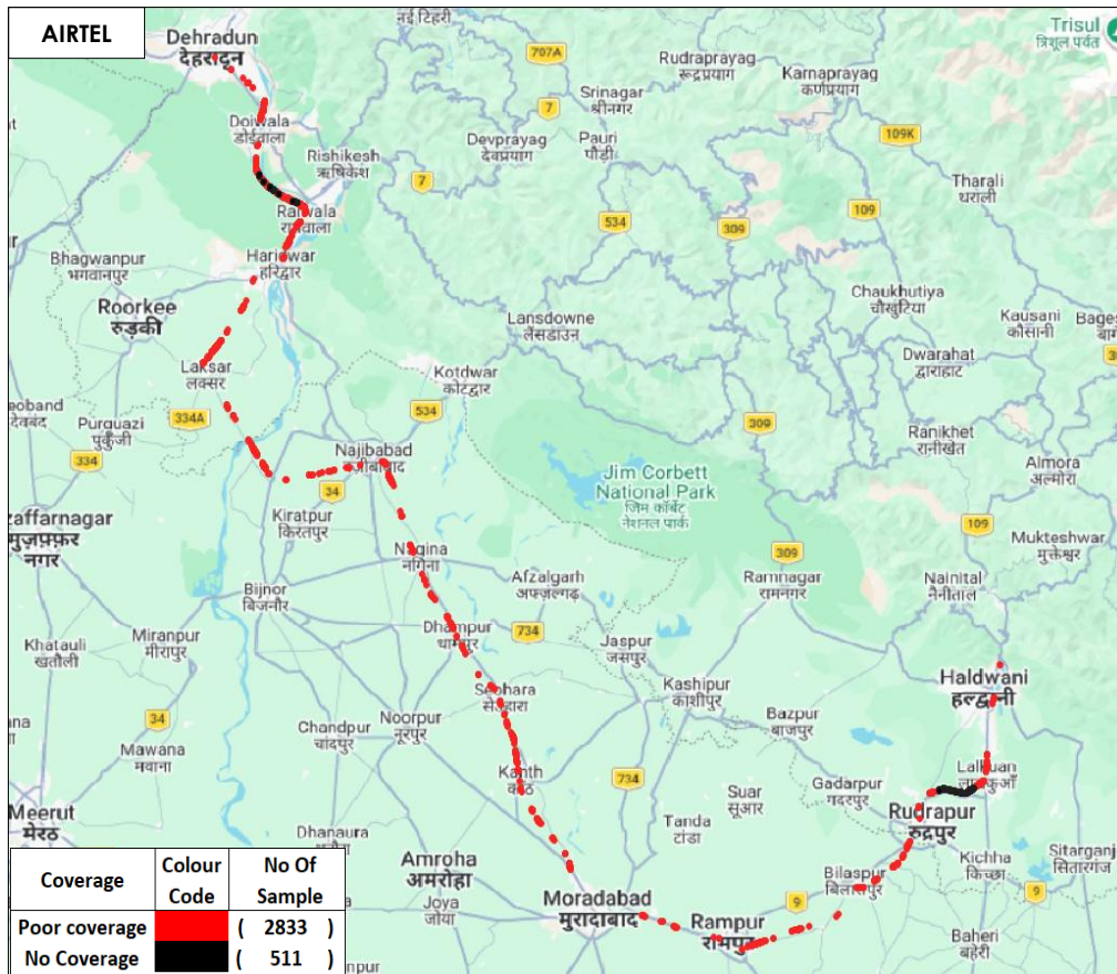
Figure-16: Poor coverage & no coverage locations in auto-selection mode (5G/4G/3G/2G) voice-Airtel.
