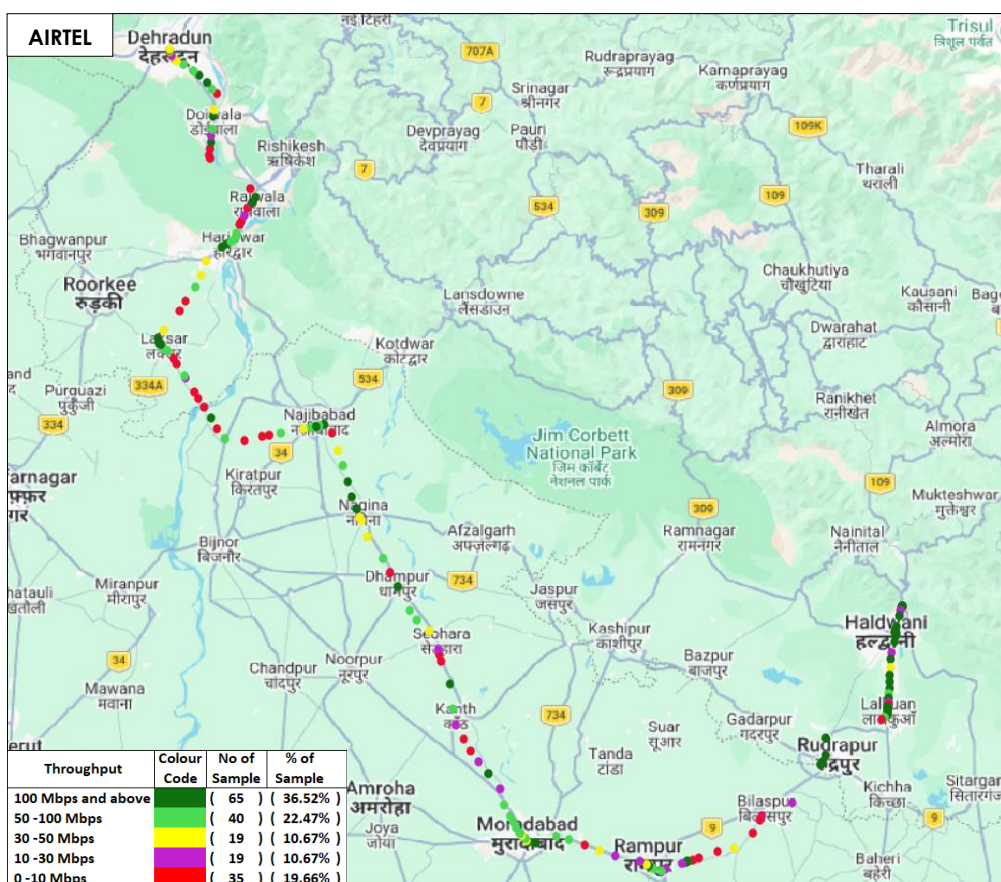
Figure-21: Download throughput distribution auto-selection mode (5G/4G/3G/2G) - AIRTEL.
