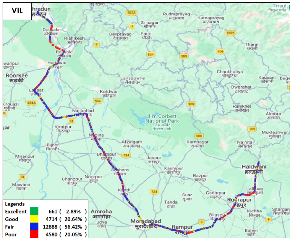
Figure-41: Signal strength auto-selection mode (5G/4G/3G/2G) data - VIL.
