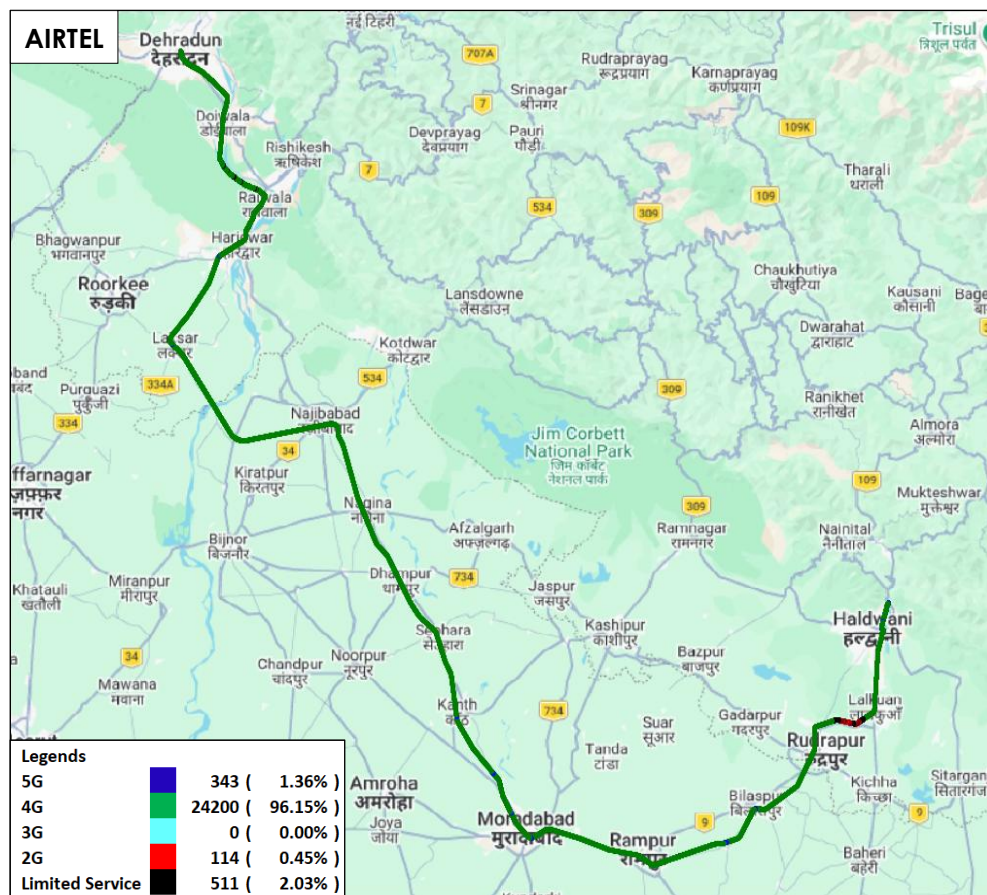
Figure-11: Serving technology plots in auto-selection mode (5G/4G/3G/2G) voice - AIRTEL.
