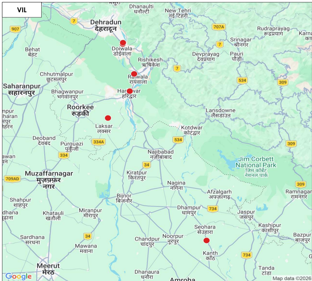
Figure-10: Drop call locations in auto-selection mode (5G/4G/3G/2G) voice – VIL
